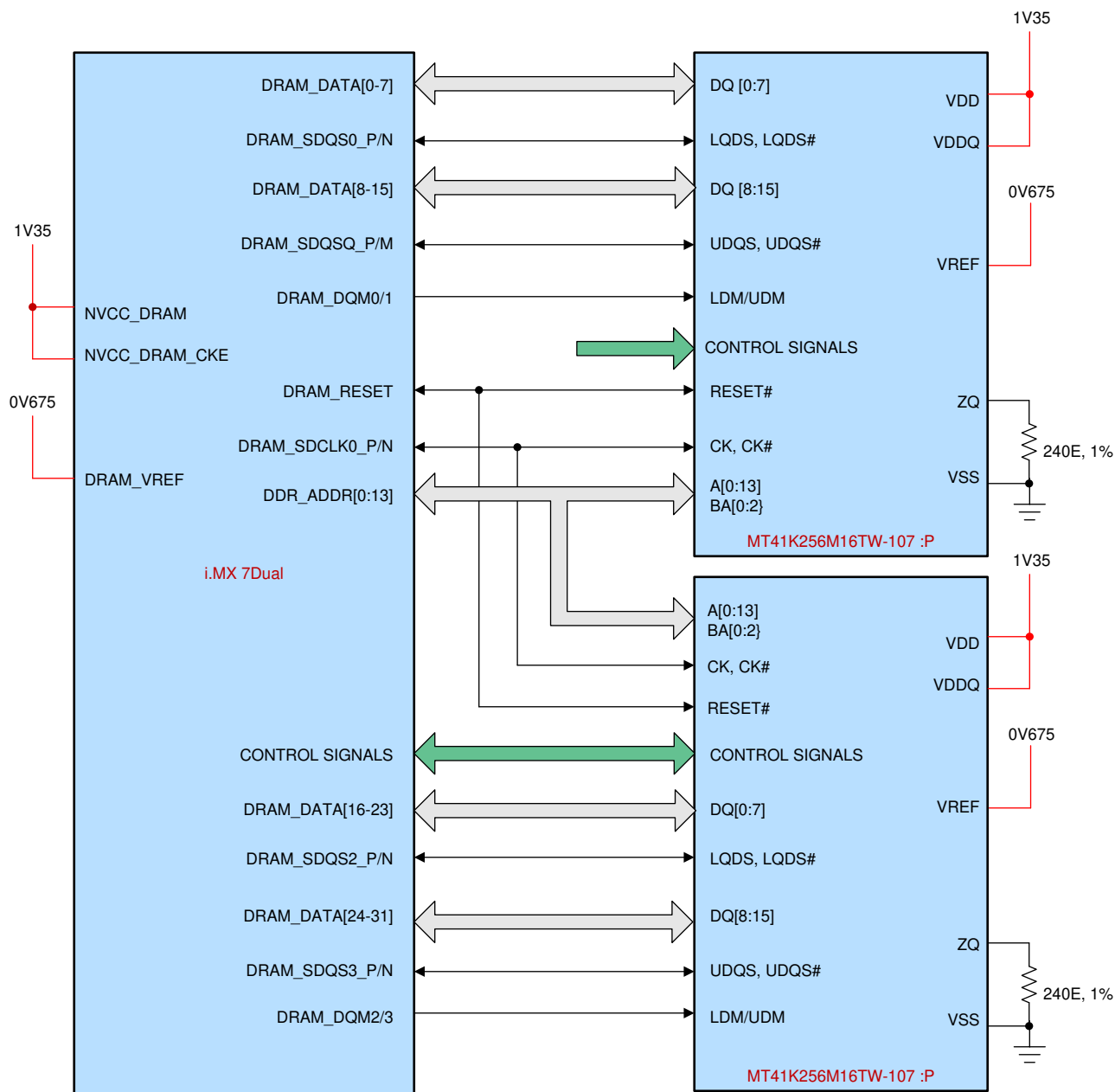
Figure 2-2. DDR3L Interface
