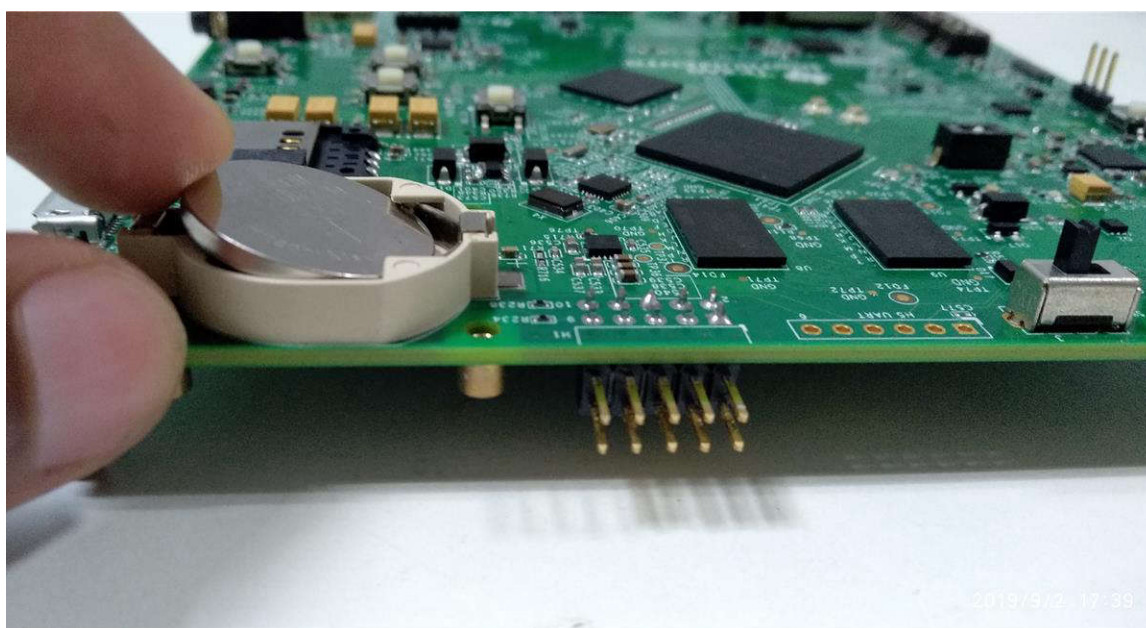
Figure 3-4. Inserting Coin Cell Battery Into BH1
