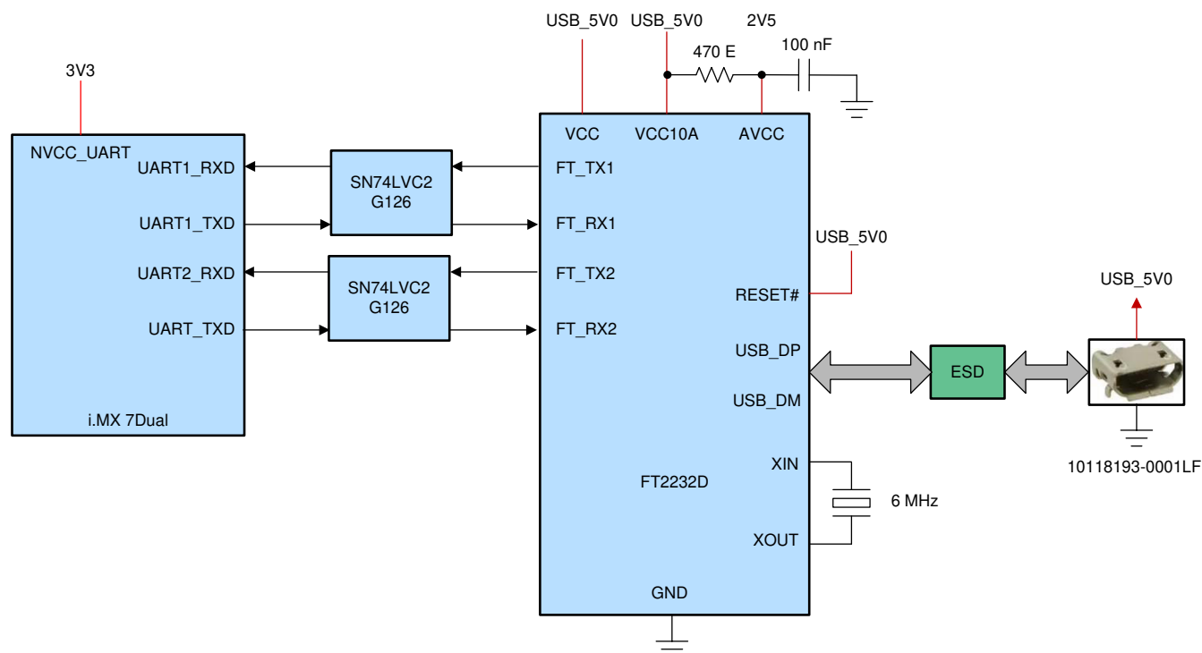
Figure 2-5. USB to Serial UART Interface With FT2232
