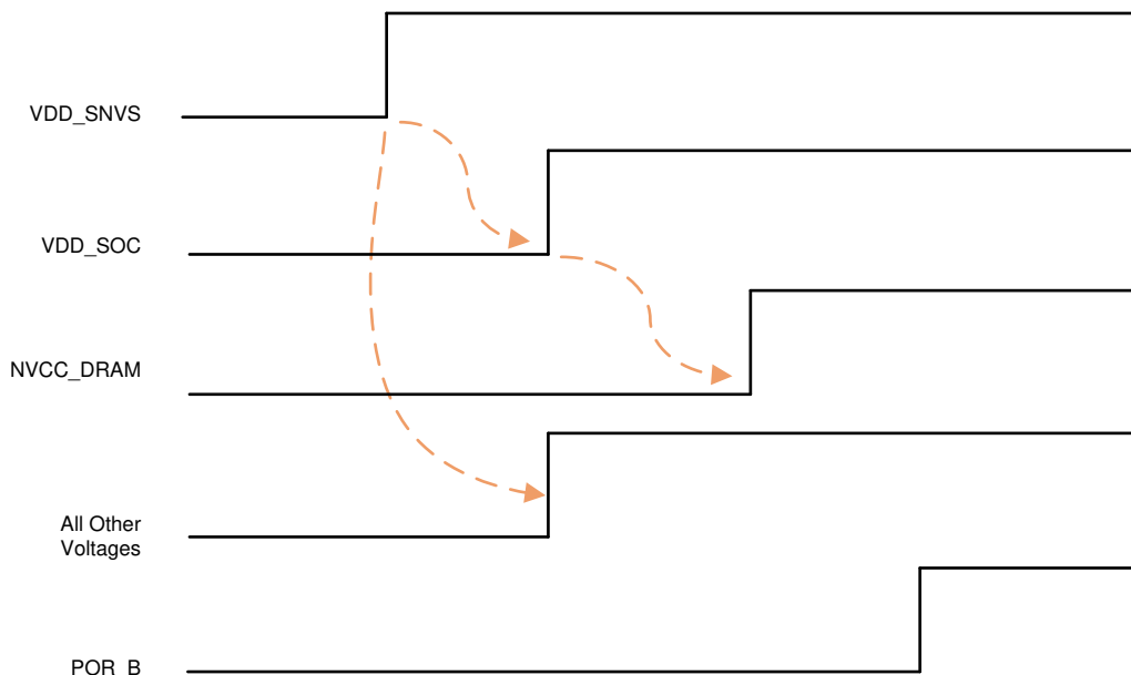
Figure 2-18. Required Power Sequence for i.MX 7D Processor
