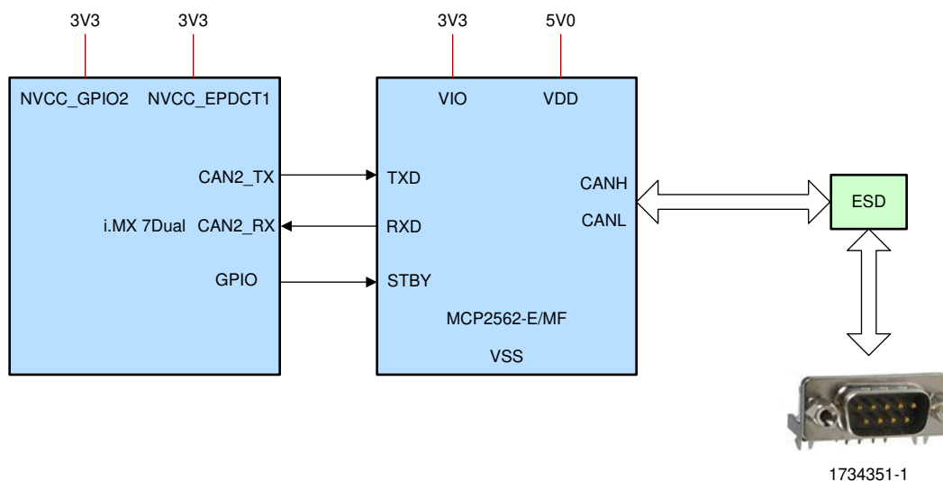
Figure 2-10. CAN Interface
