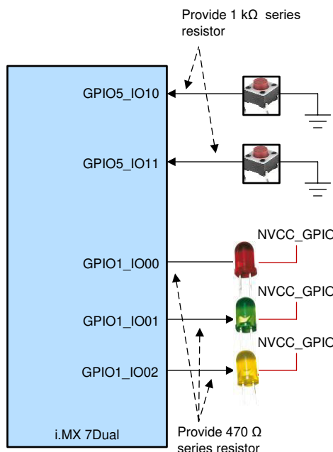
Figure 2-12. GPIO Connections to Push-buttons and LEDs
