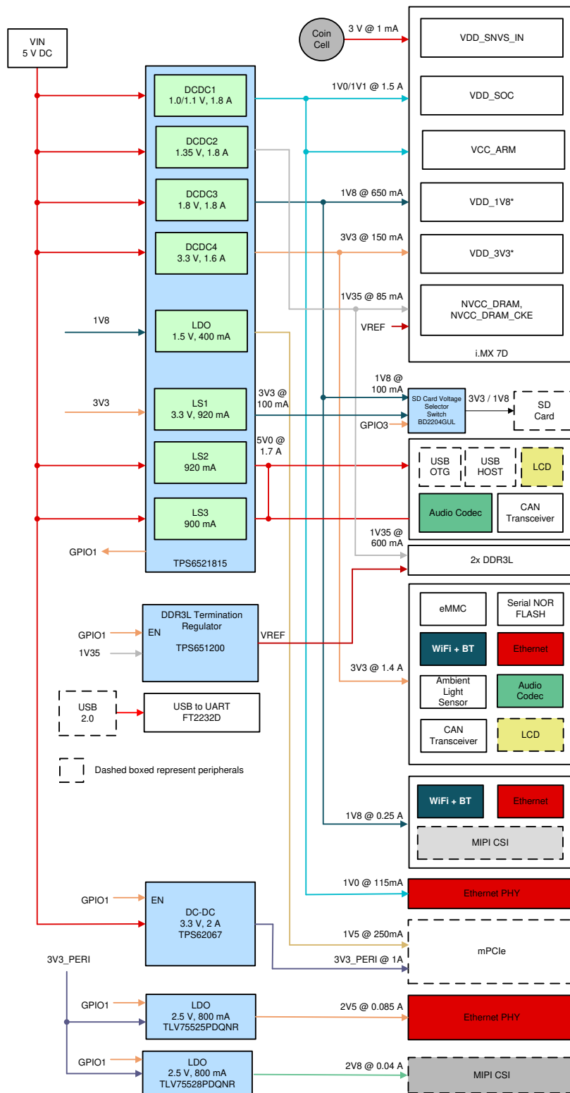
Figure 2-17. TIDA-050034 Full Power Architecture
