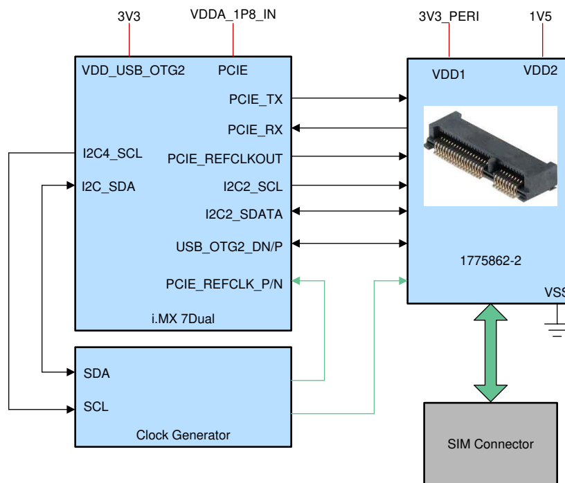
Figure 2-9. mPCIe Interface
