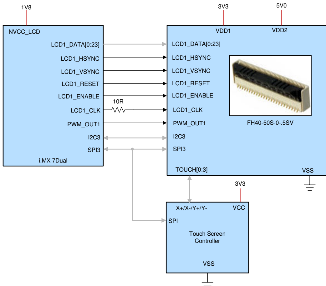
Figure 2-7. LCD Interface From i.MX 7D Processor to Connector
