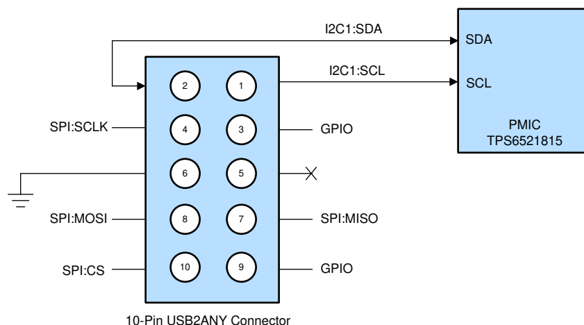
Figure 2-11. USB2ANY Header Connections to PMIC I 2 C Pins
