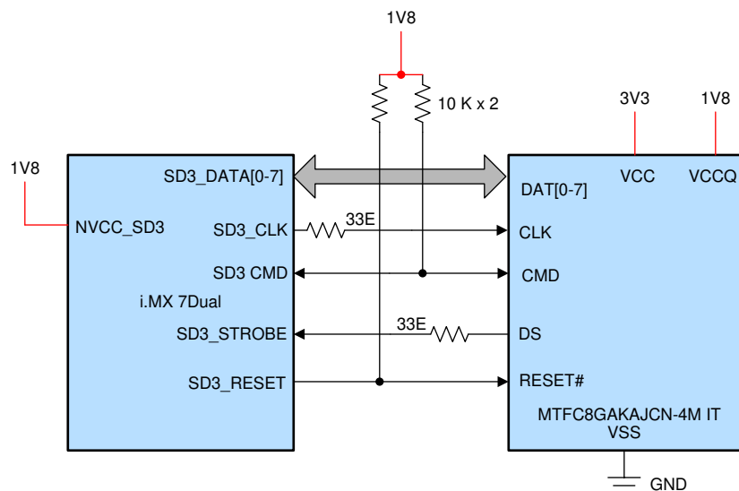
Figure 2-3. eMMC Interface
