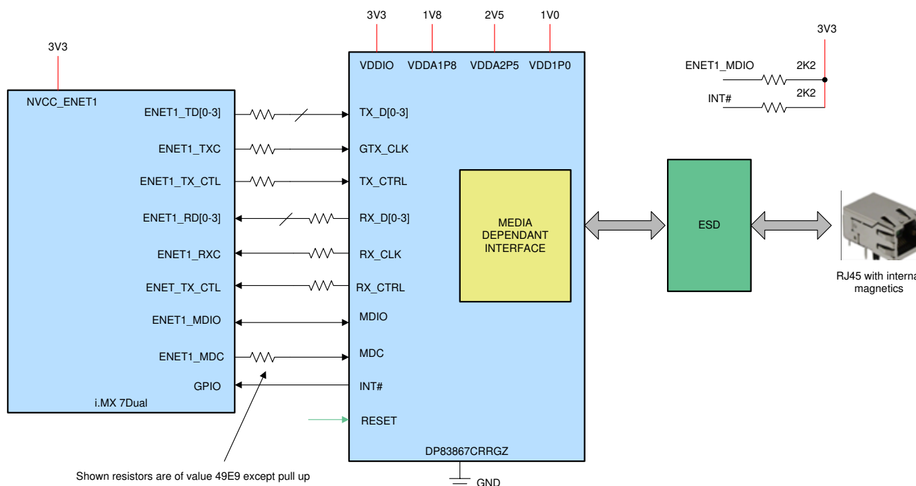
Figure 2-14. Ethernet Interface With DP83867CR PHY
