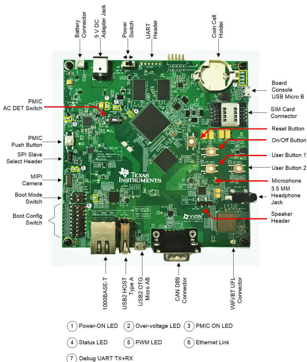
Figure 3-1. Top of TIDA-050034 PCB With Labels
