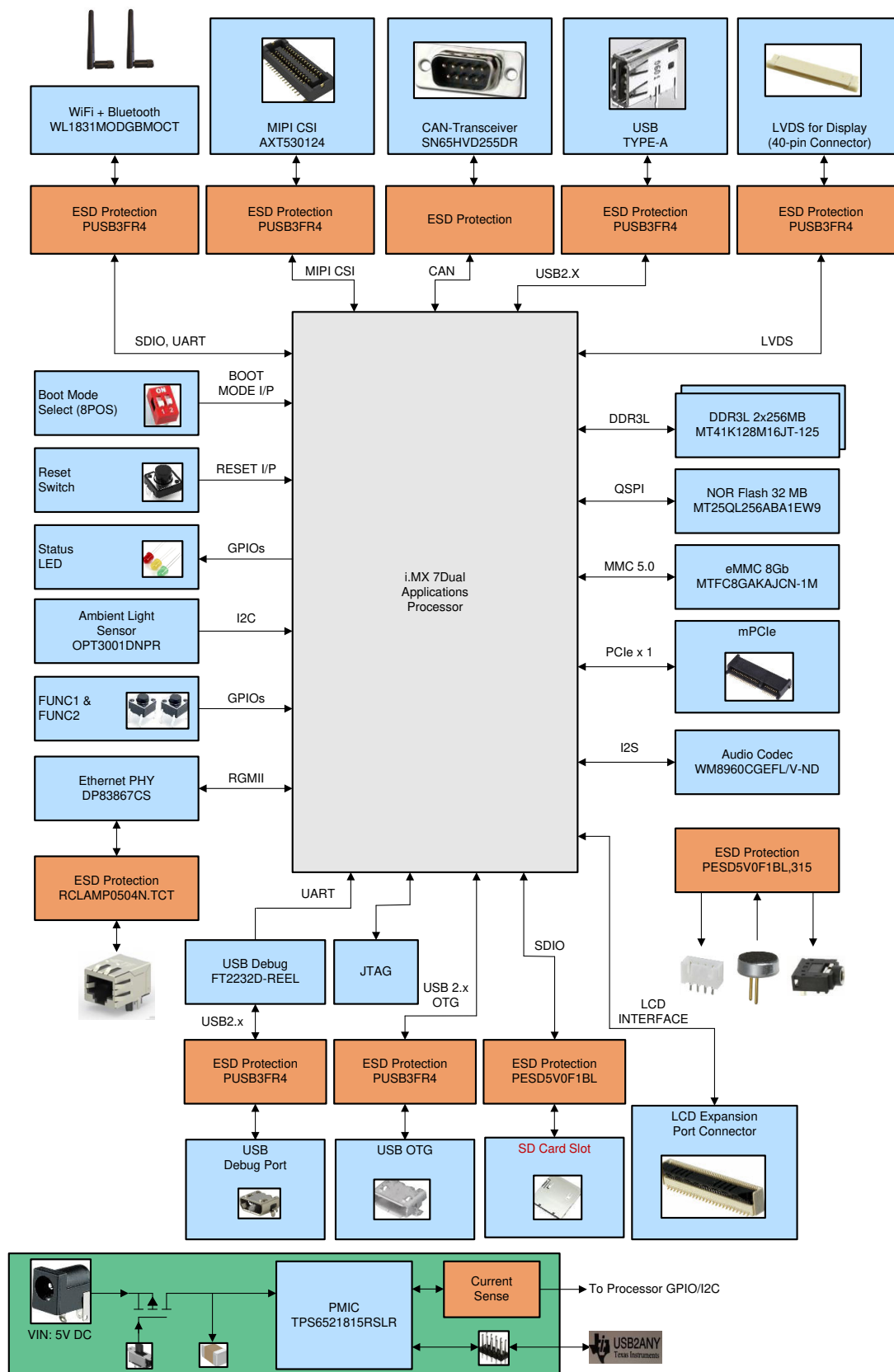
Figure 2-1. TIDA-050034 Block Diagram
