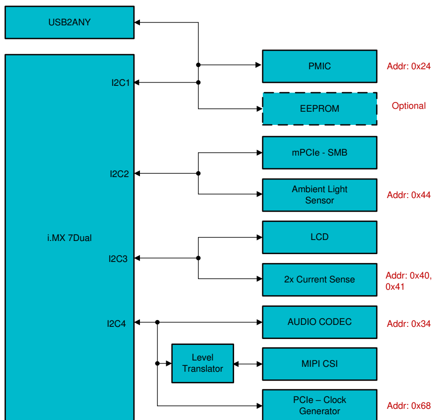
Figure 2-19. I²C Device Chain
