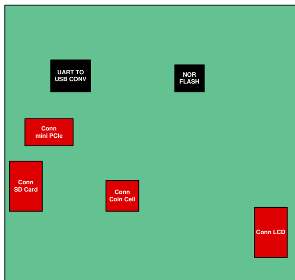
Figure 2-21. PCB Floor Planning (bottom)
