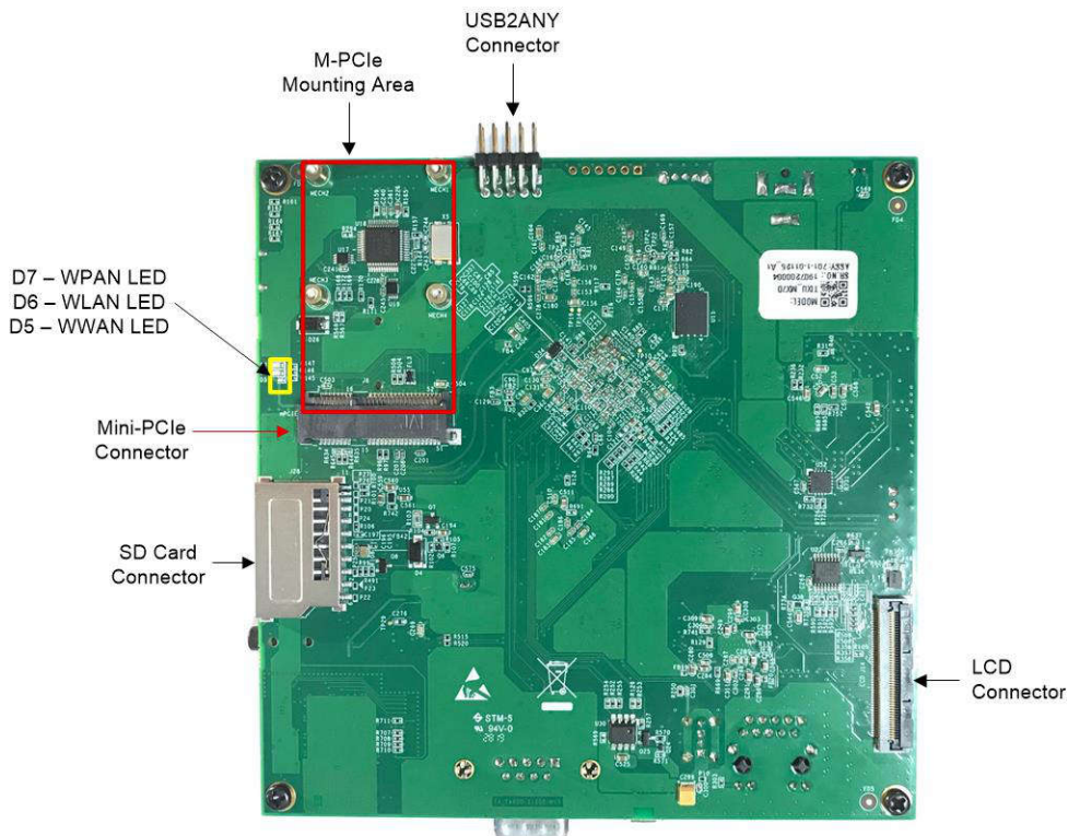
Figure 3-2. Bottom of TIDA-050034 PCB With Labels
