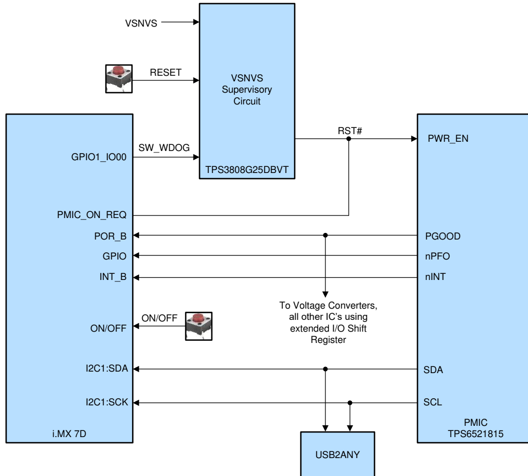
Figure 2-16. Reset Scheme With TPS3808 Supervisor
