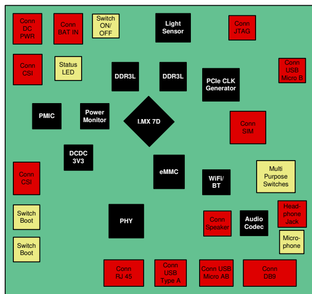
Figure 2-20. PCB Floor Planning (top)
