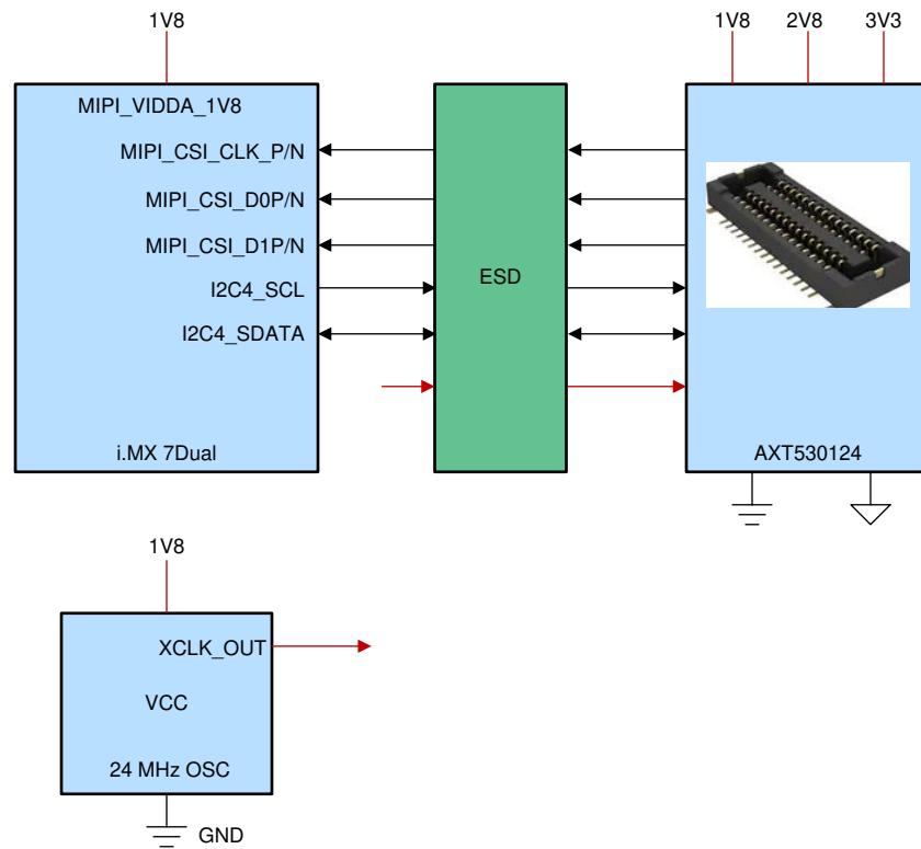
Figure 2-8. MIPI CSI Connector
