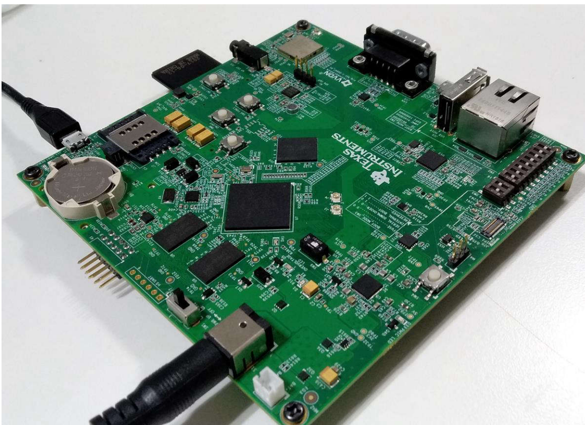
Figure 3-8. Board Connections for BOOT From SD Card With Debug Over USB
