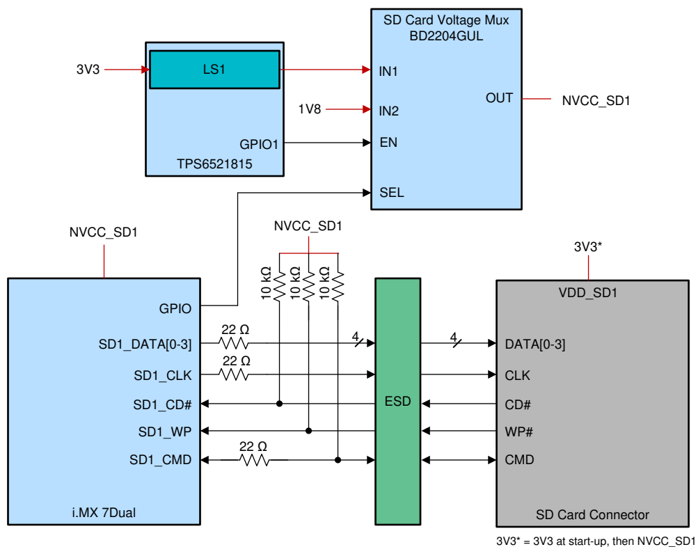
Figure 2-4. SD Card Power and Connector
