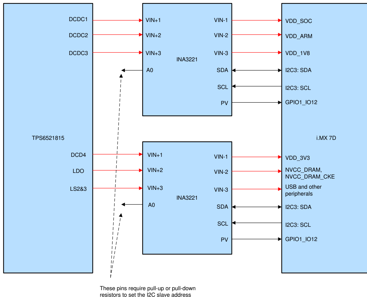
Figure 2-15. INA3221 Current Sensor Wiring From PMIC to Processor
