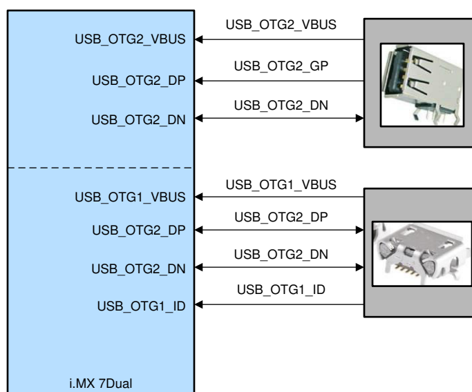
Figure 2-6. USB Interface
