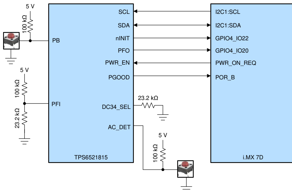
Figure 2-13. TPS6521815 PMIC I/O Wiring to i.MX 7D Processor
