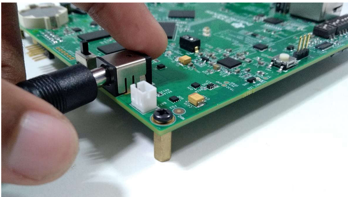
Figure 3-7. Inserting 5V DC Adapter Into J1
