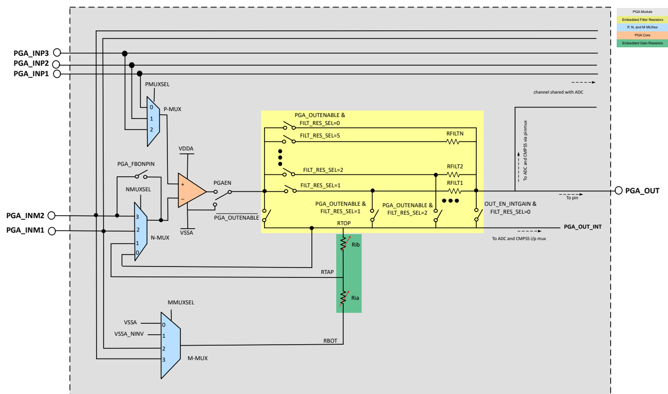
Figure 19-1. PGA Block Diagram
