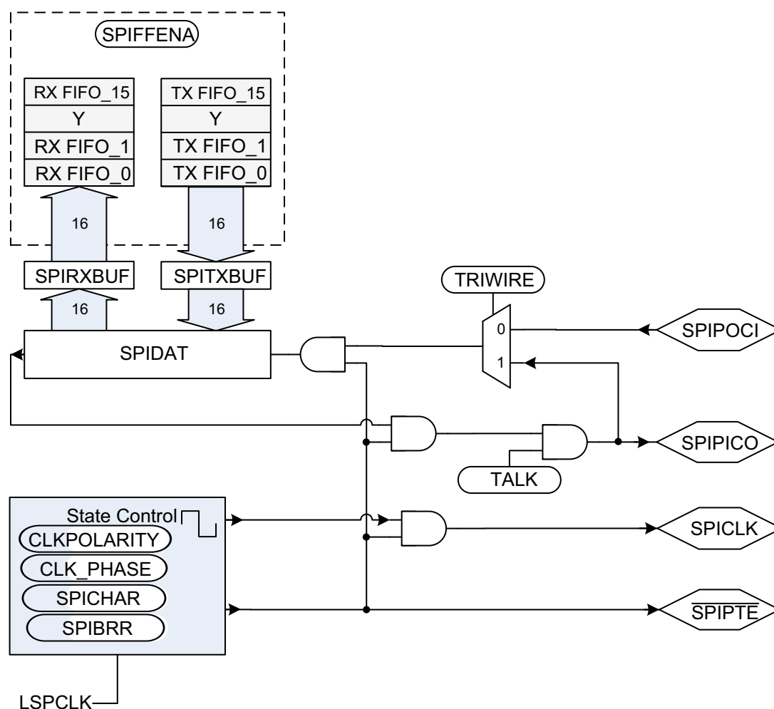
Figure 18-5. SPI Module Controller Configuration
