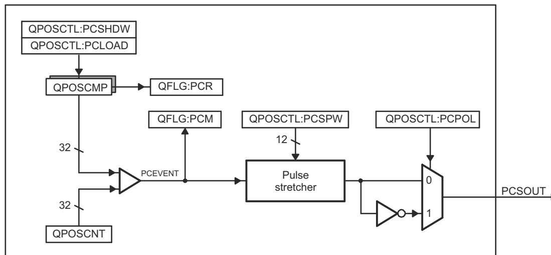
Figure 15-14. eQEP Position-compare Unit
