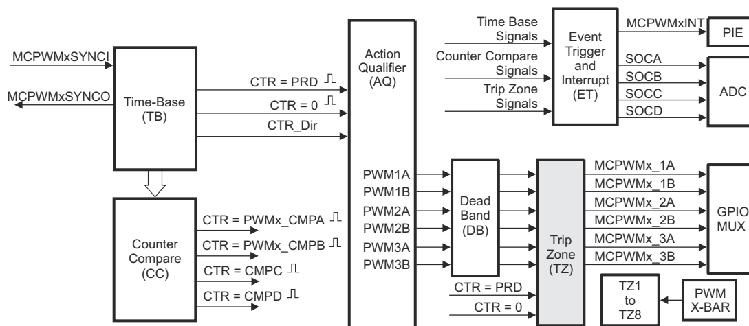
Figure 13-32. Trip-Zone Submodule
