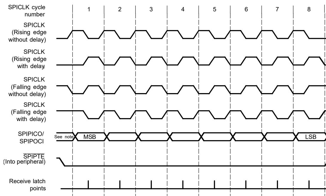
Figure 18-7. SPICLK Signal Options
