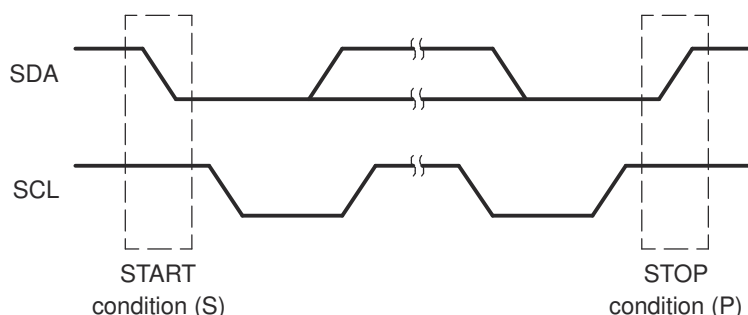
Figure 16-8. I2C Module START and STOP Conditions
