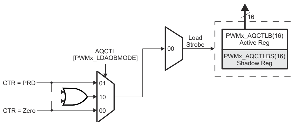
Figure 13-21. AQCTL[PWMx_LDAQBMODE]
