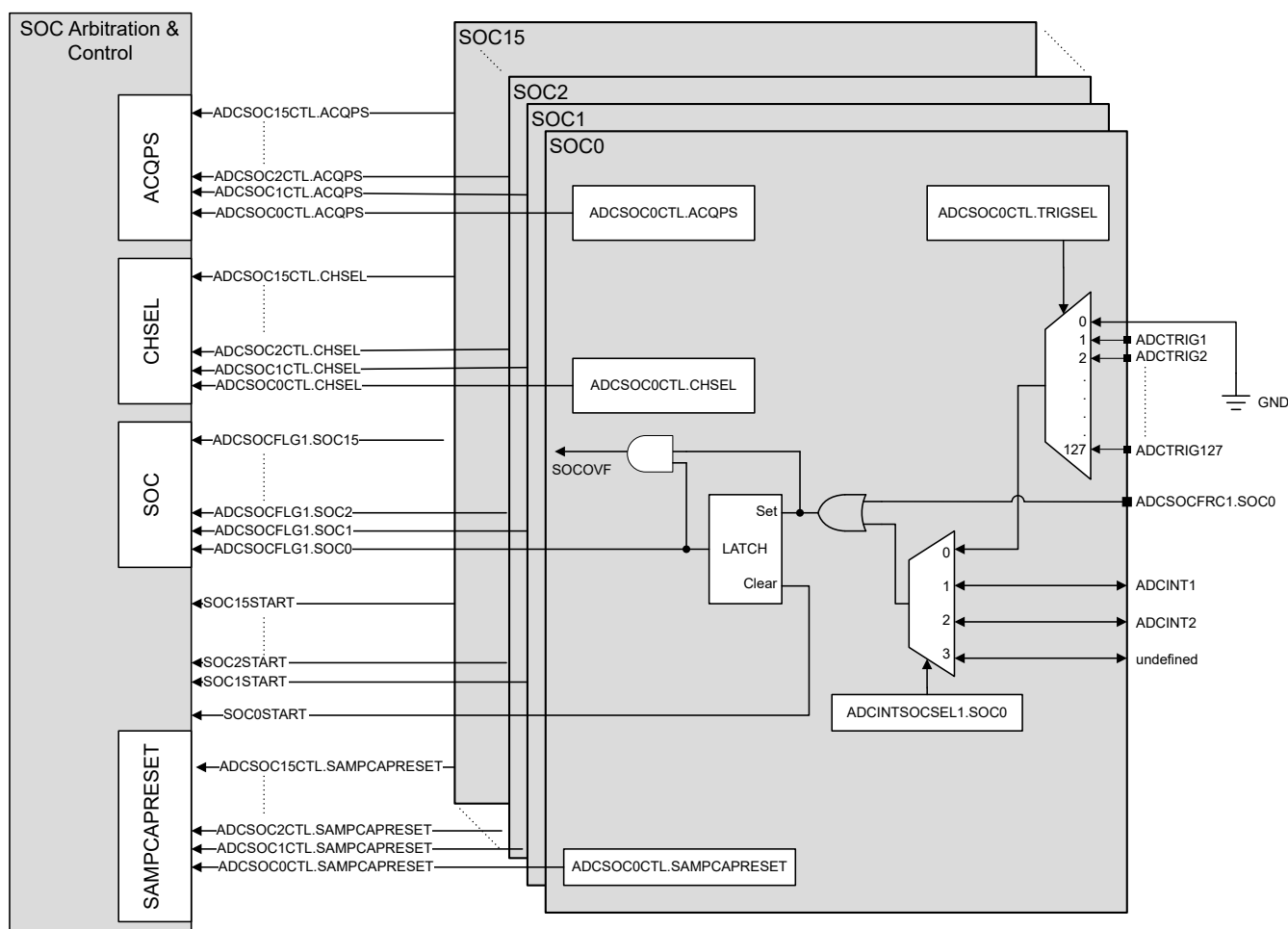
Figure 11-2. SOC Block Diagram
