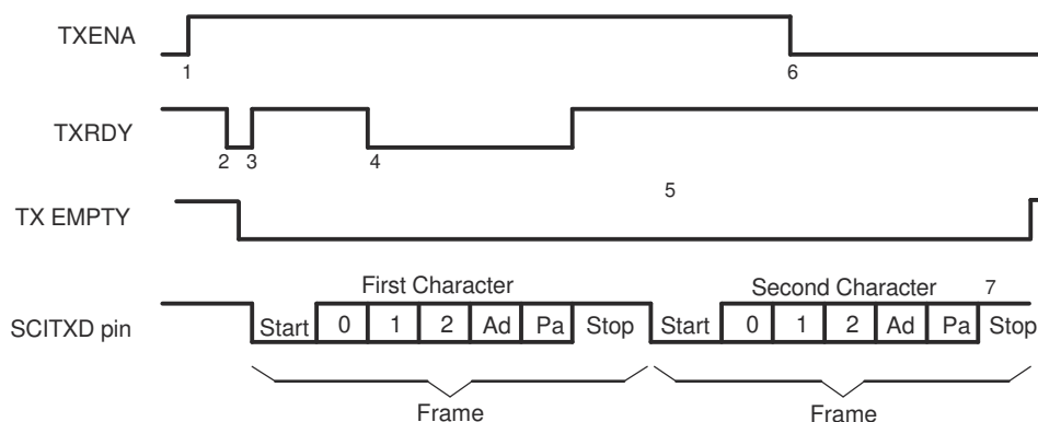
Figure 17-9. SCI TX Signals in Communications Mode
