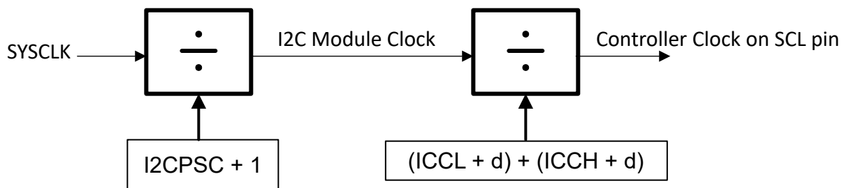
Figure 16-3. Clocking Diagram for the I2C Module
