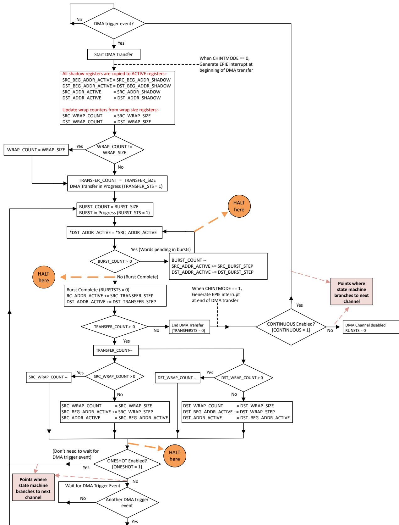
Figure 20-4. DMA State Diagram
