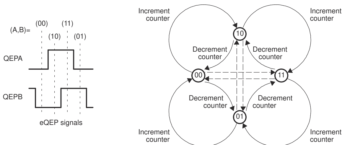
Figure 15-7. Quadrature Decoder State Machine
