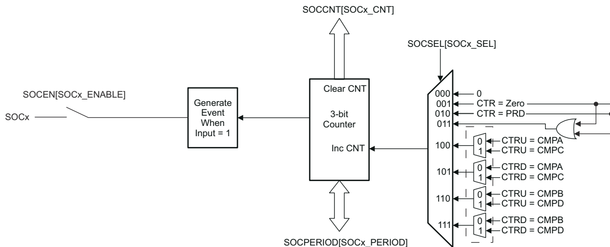
Figure 13-37. Event-Trigger Start-of-Conversion (SOC) Pulse Generator
