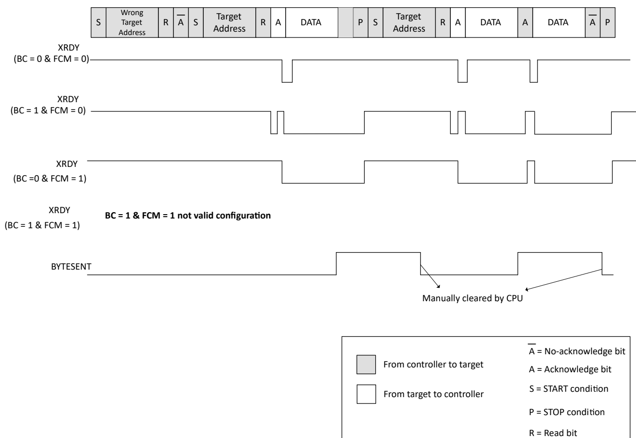
Figure 16-20. Backwards Compatibility Mode and Forward Compatibility Bit, Target Transmitter
