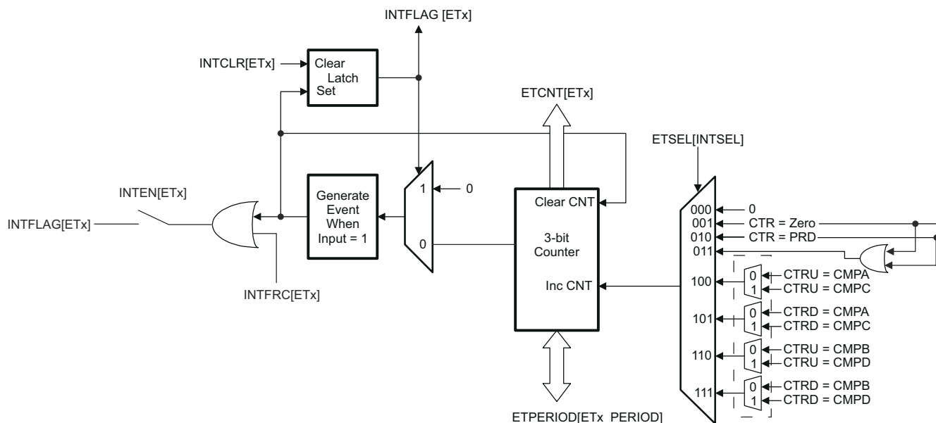
Figure 13-36. Event-Trigger Interrupt Generator
