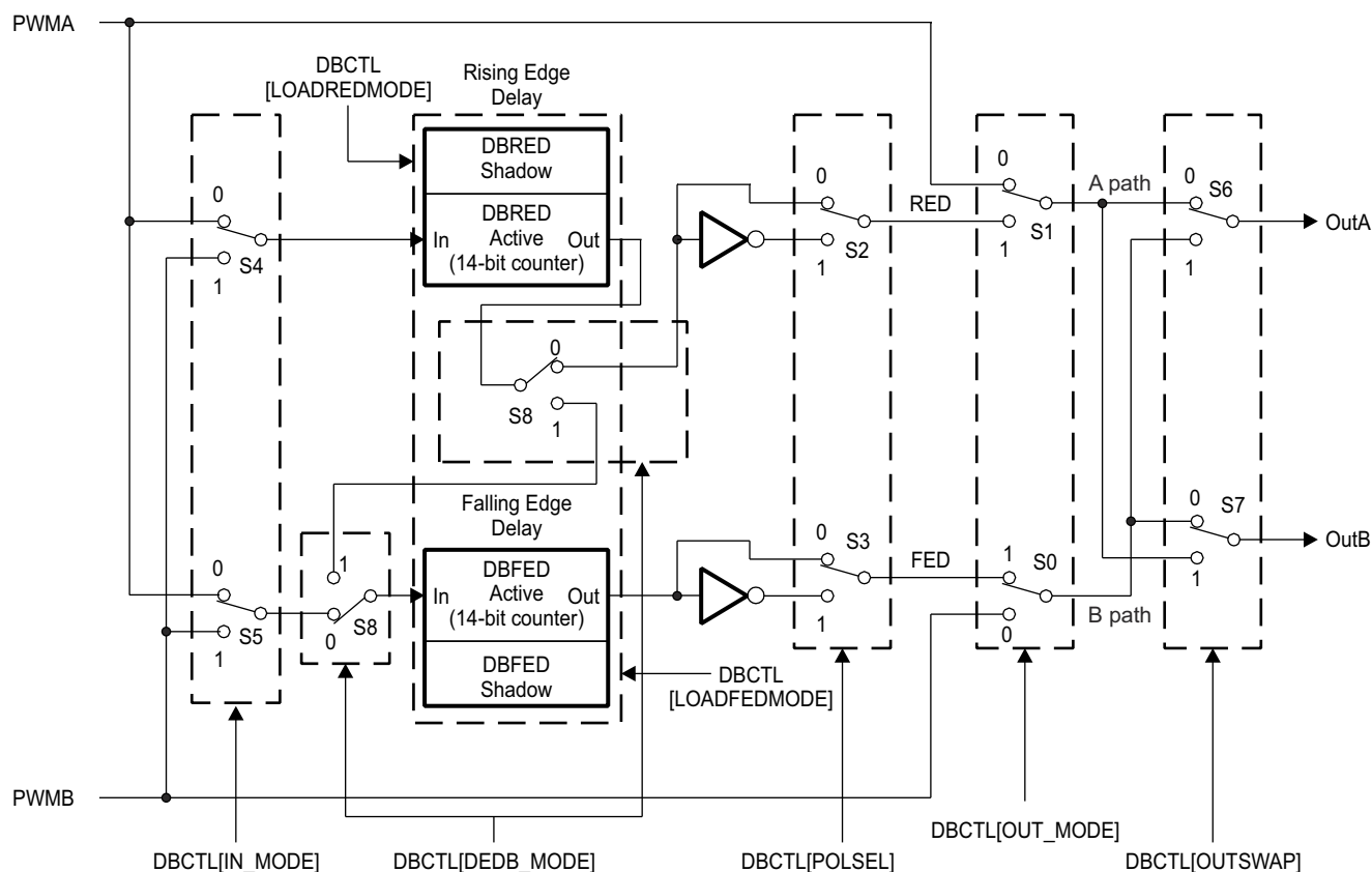
Figure 13-30. Configuration Options for the Dead-Band Submodule
