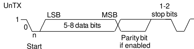
Figure 21-2. UART Character Frame
