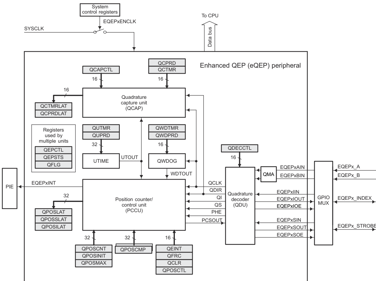
Figure 15-5. Functional Block Diagram of the eQEP Peripheral
