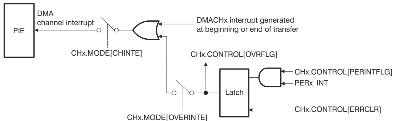
Figure 20-7. Overrun Detection Logic
