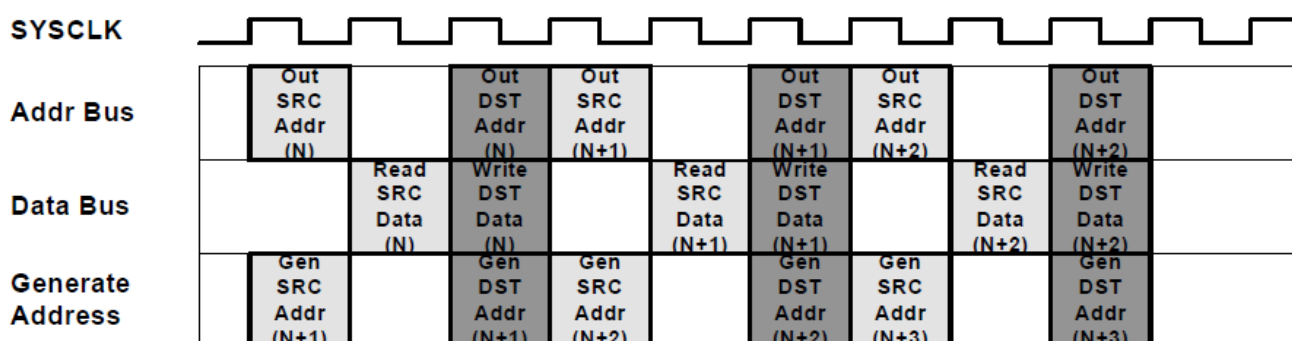
Figure 20-5. 3-Stage Pipeline DMA Transfer
