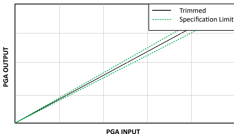
Figure 19-8. PGA Gain Error
