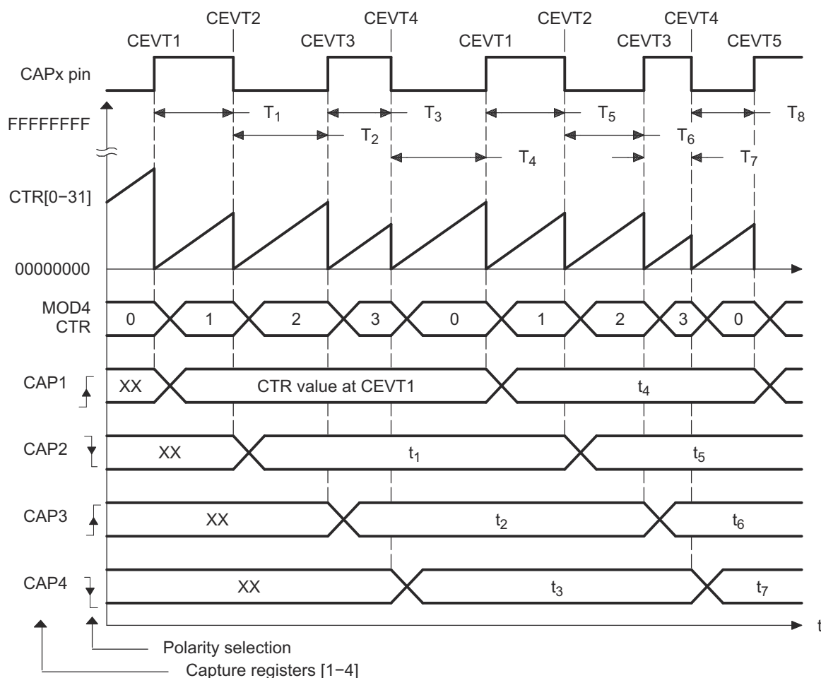
Figure 14-15. Capture Sequence for Delta Mode Time-stamp with Rising- and Falling-Edge Detect
