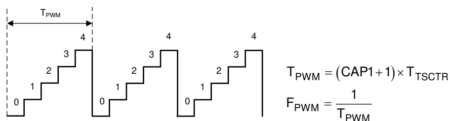
Figure 14-11. Time-Base Frequency and Period Calculation
