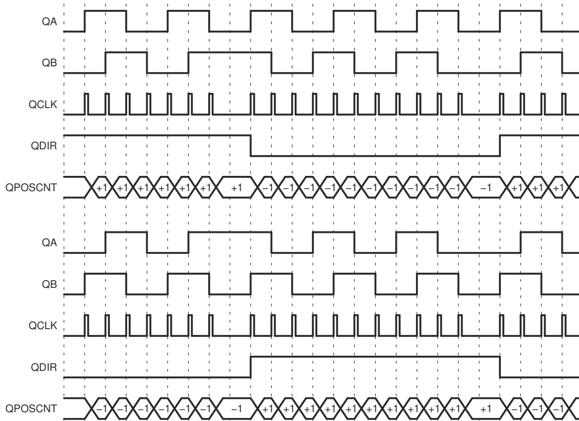
Figure 15-8. Quadrature-clock and Direction Decoding
