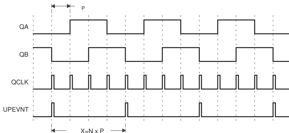
Figure 15-18. Unit Position Event for Low Speed Measurement (QCAPCTL[UPPS] = 0010)
