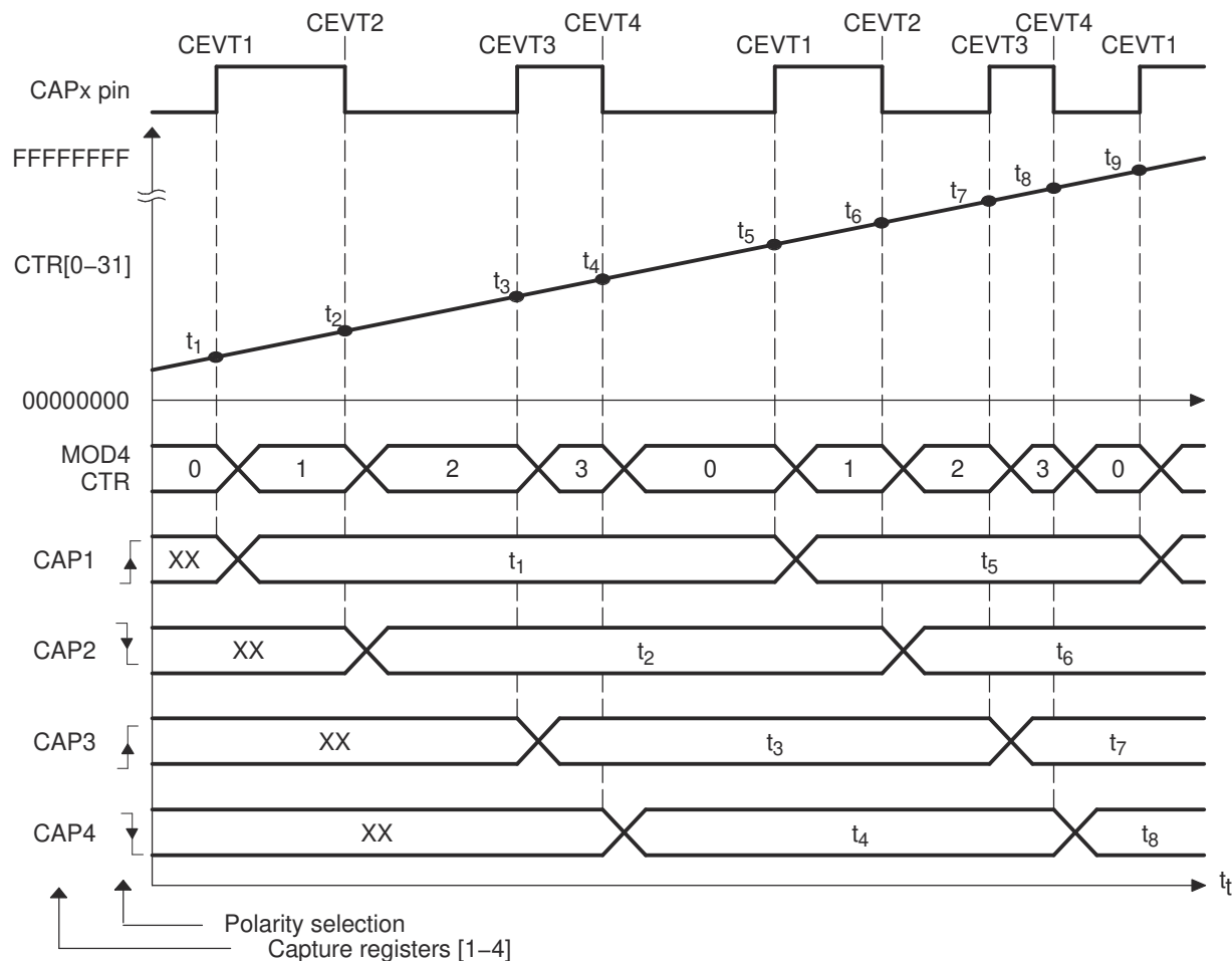
Figure 14-13. Capture Sequence for Absolute Time-stamp with Rising- and Falling-Edge Detect
