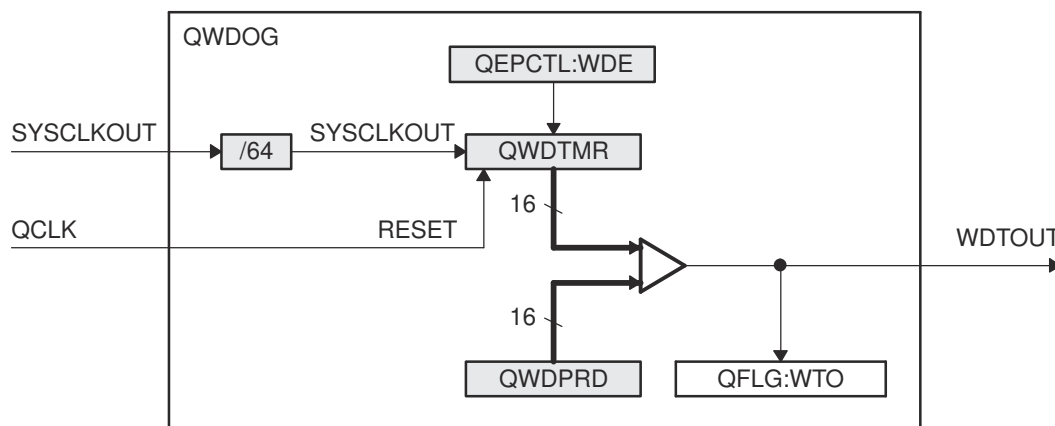
Figure 15-20. eQEP Watchdog Timer
