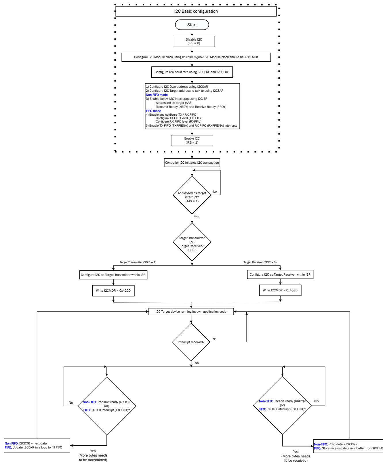
Figure 16-6. I2C Target TX / RX Flowchart
