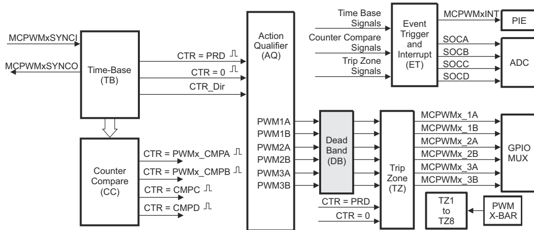
Figure 13-29. Dead_Band Submodule
