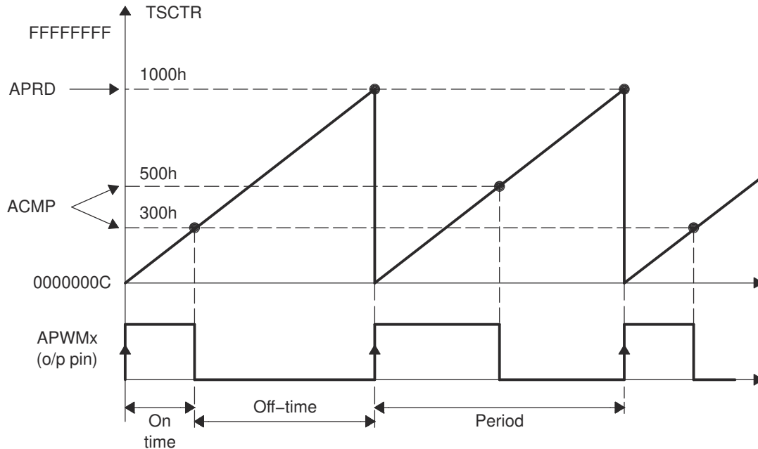
Figure 14-16. PWM Waveform Details of APWM Mode Operation
