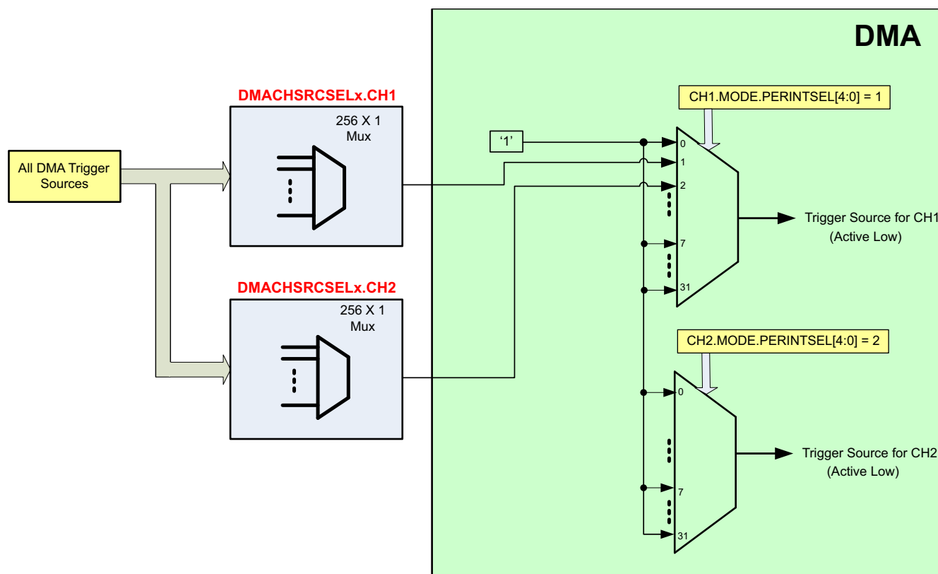
Figure 20-2. DMA Trigger Architecture
