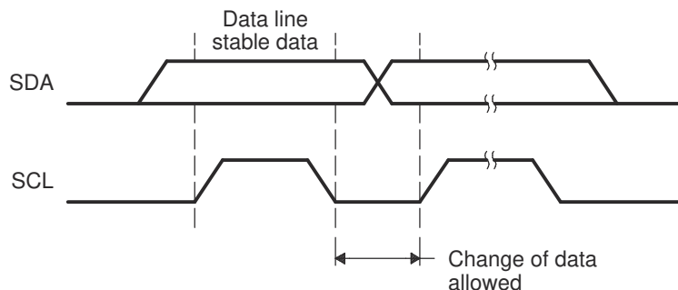
Figure 16-5. Bit Transfer on the I2C bus
