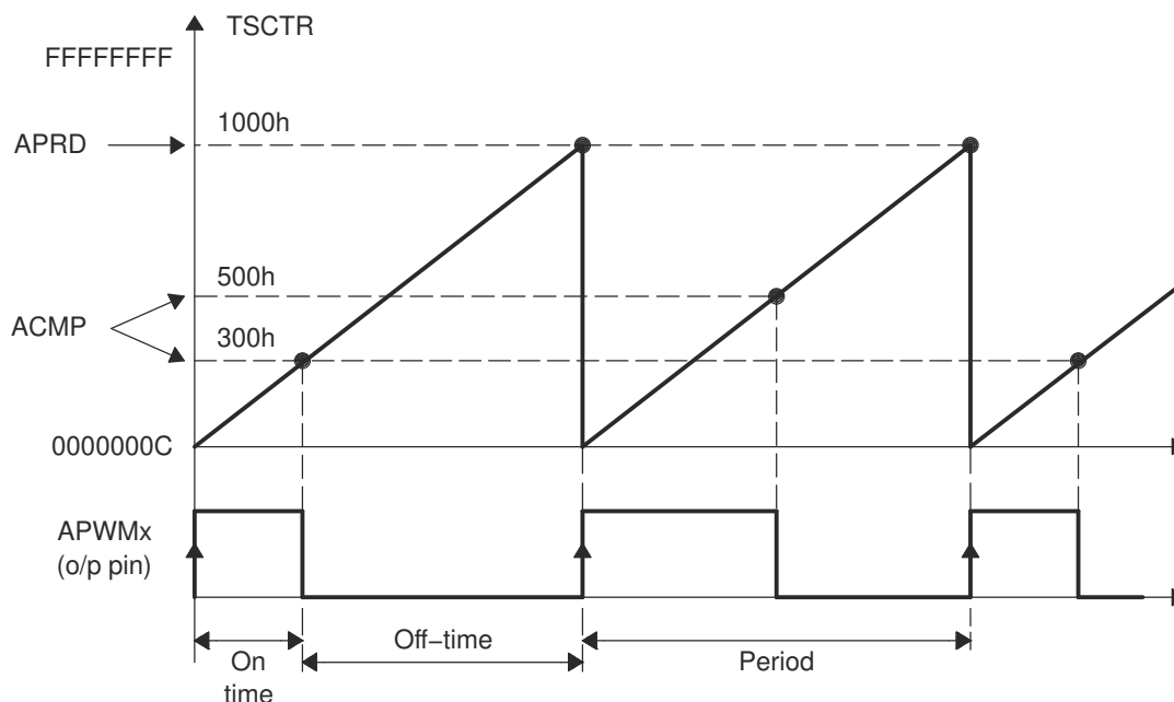
Figure 14-10. PWM Waveform Details Of APWM Mode Operation
