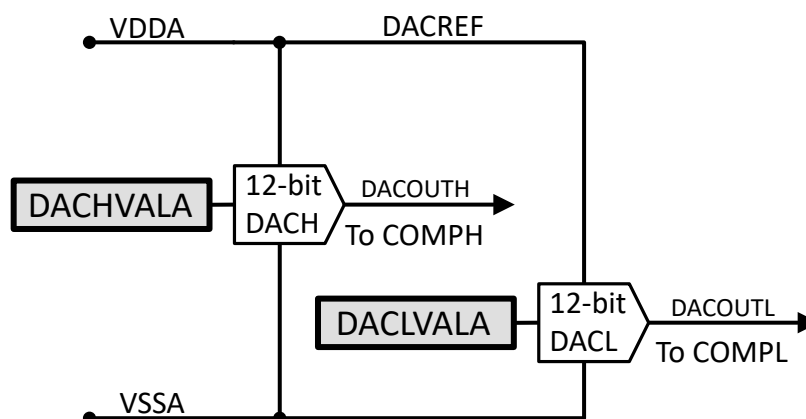
Figure 12-4. Reference DAC Block Diagram
