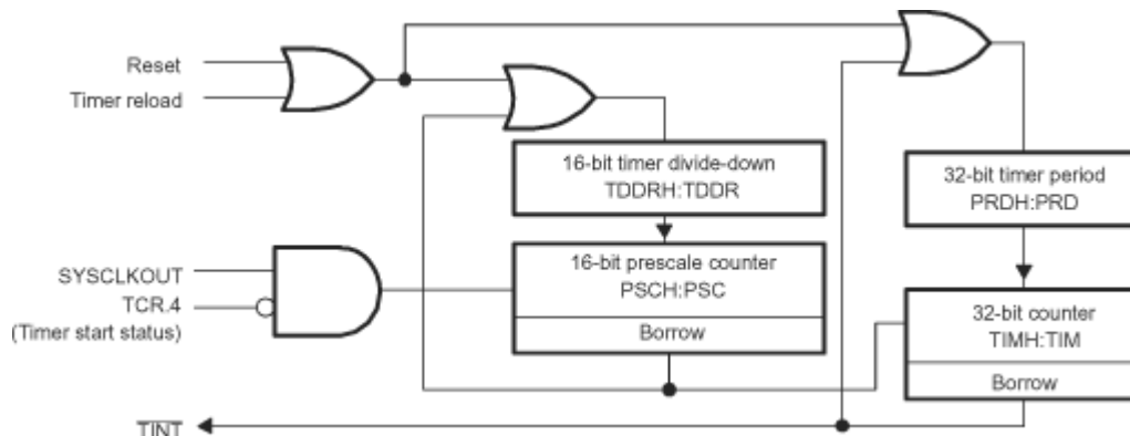
Figure 3-11. CPU Timers
