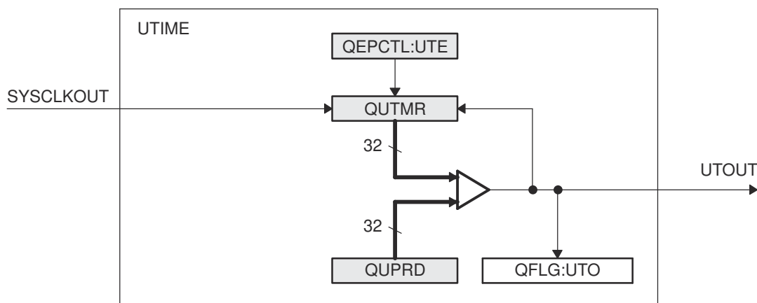
Figure 15-21. eQEP Unit Timer Base
