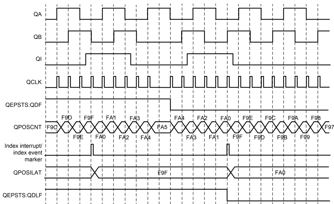
Figure 15-11. Software Index Marker for 1000-line Encoder (QEPCTL[IEL] = 1)
