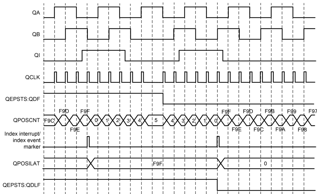
Figure 15-9. Position Counter Reset by Index Pulse for 1000-Line Encoder (QPOS MAX = 3999 or 0xF9F)
