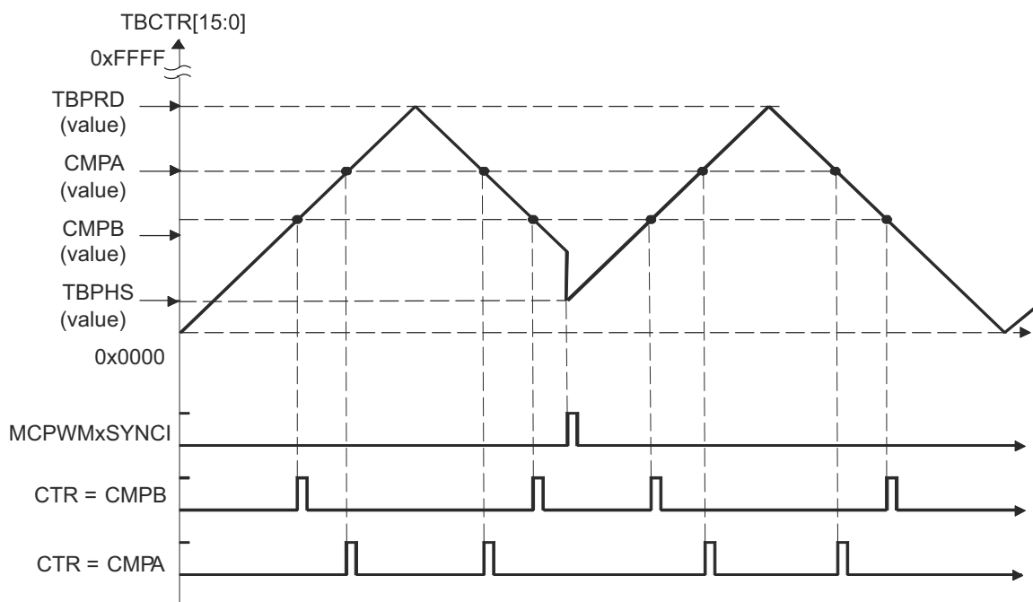
Figure 13-16. Counter-Compare Events In Up-Down Count Mode, TBCTL[PHSDIR] = 1 Count Up On Synchronization Event
