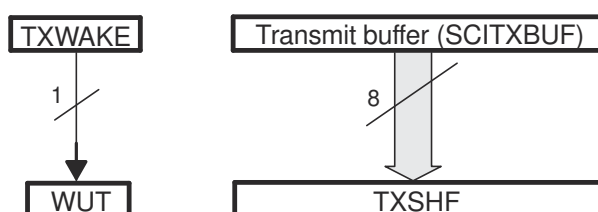
Figure 17-5. Double-Buffered WUT and TXSHF
