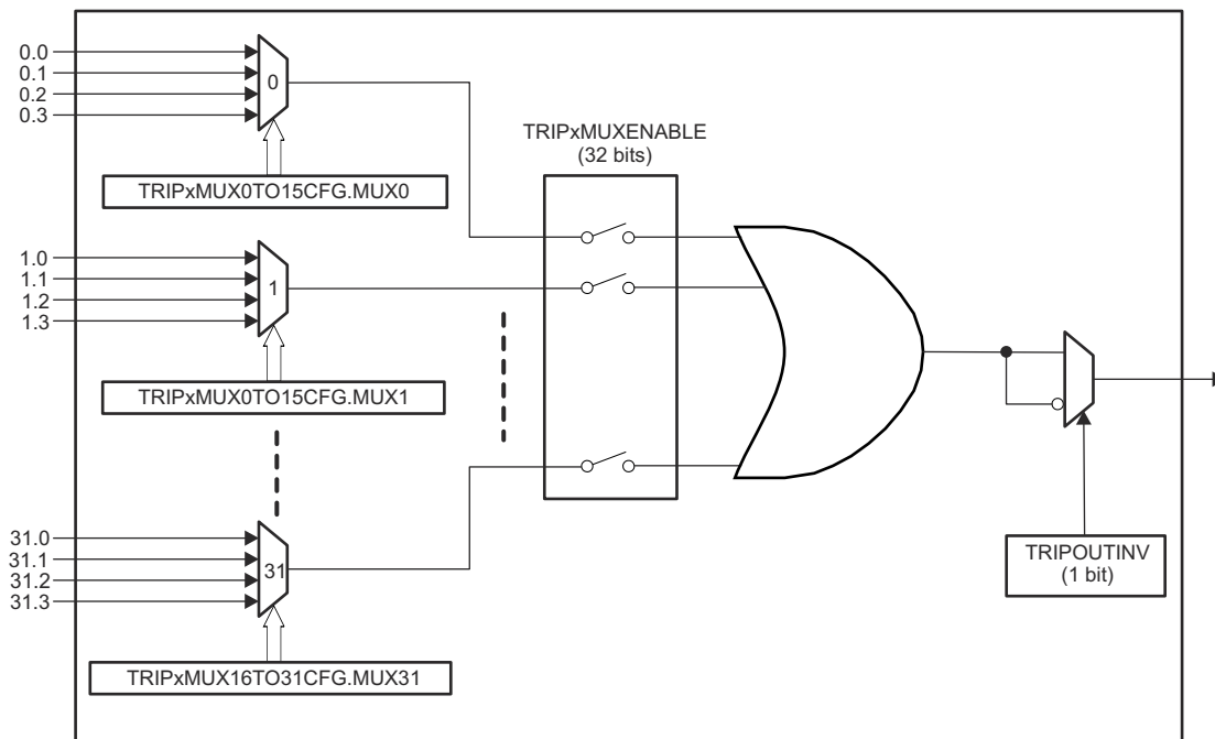
Figure 13-39. PWM X-BAR Architecture - Single Output
