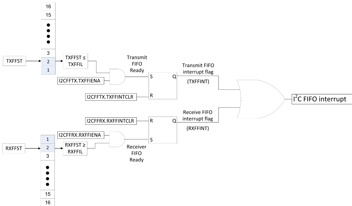
Figure 16-21. I2C FIFO Interrupt
