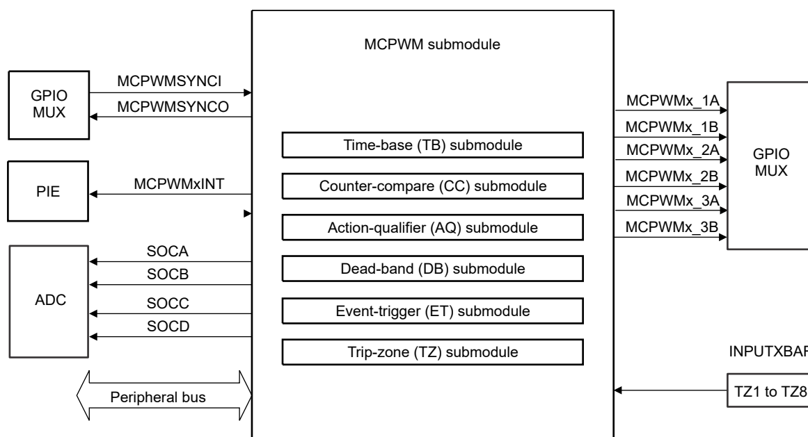
Figure 13-1. Submodules and Signal Connections for an MCPWM Module
