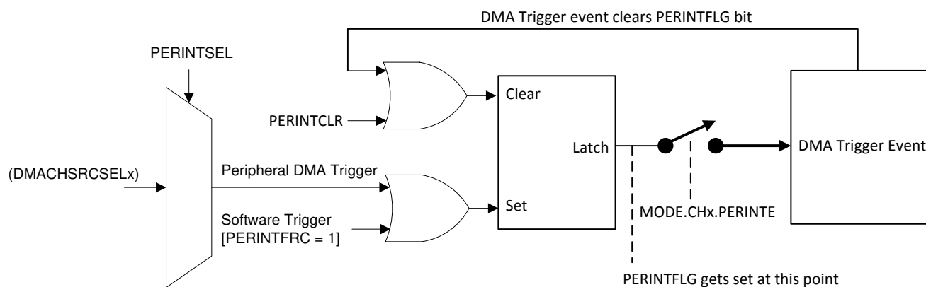
Figure 20-2. DMA Trigger Architecture
