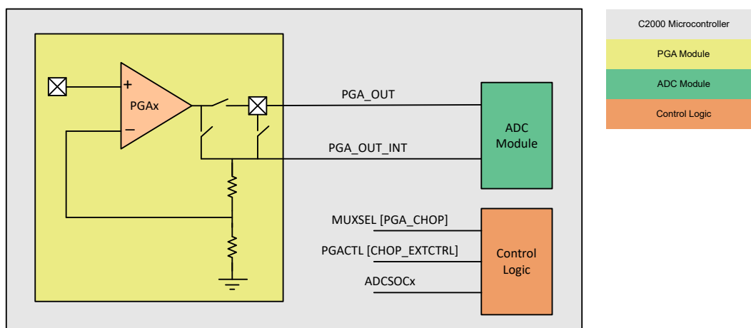
Figure 19-10. ADC-Assisted Chopping Block Diagram
