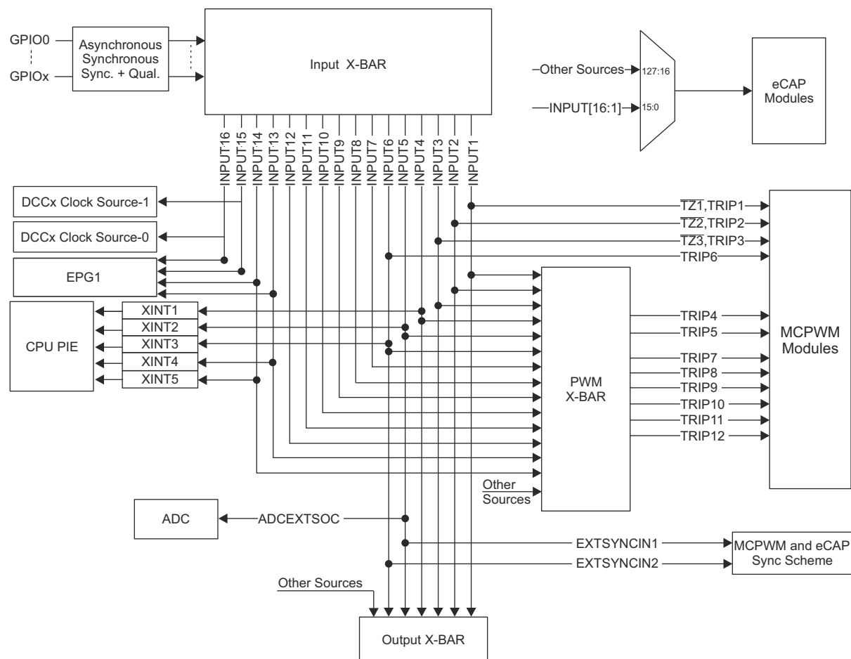
Figure 9-1. Input X-BAR
