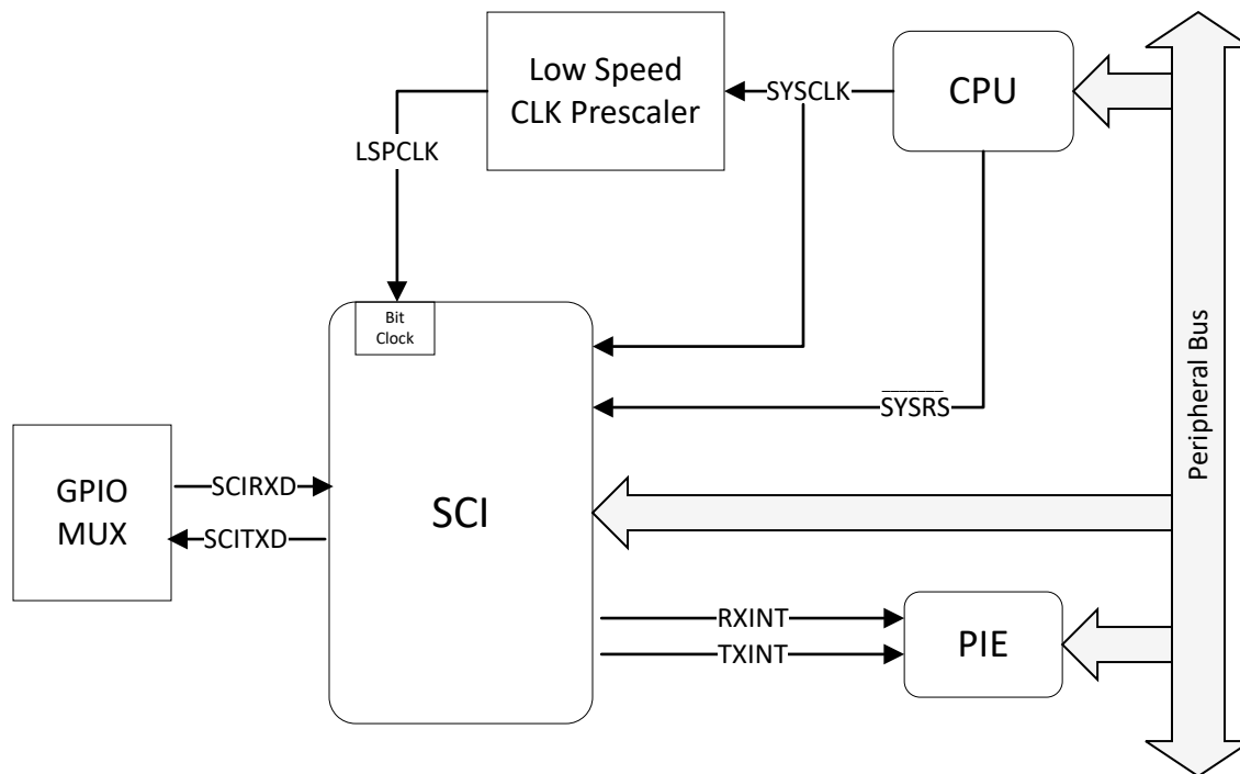
Figure 17-1. SCI CPU Interface
