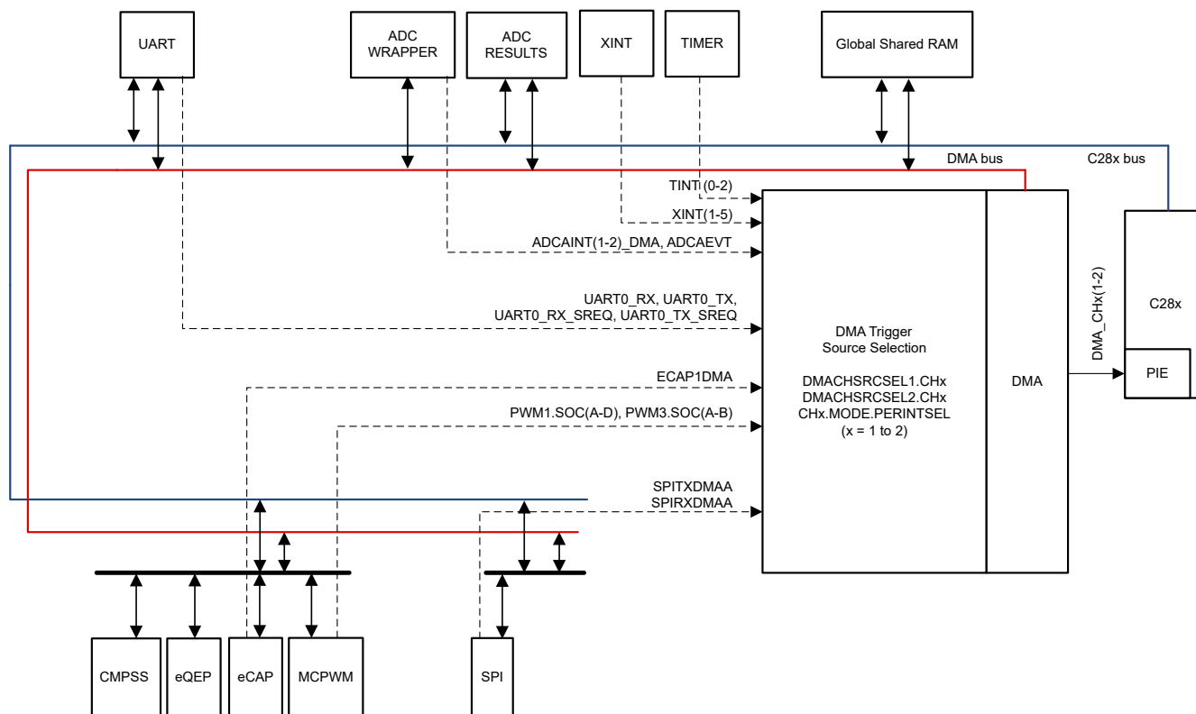
Figure 20-1. DMA Block Diagram
