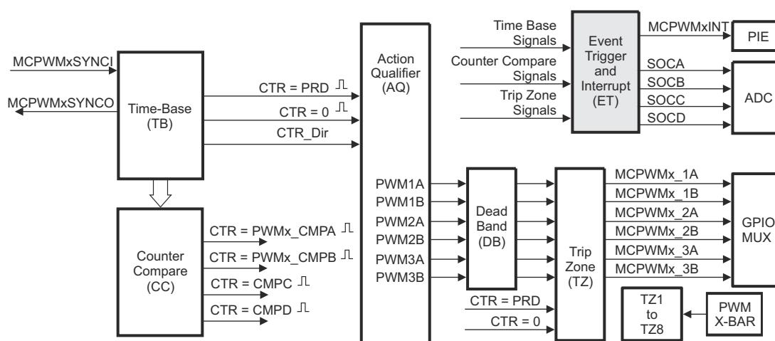
Figure 13-34. Event-Trigger Submodule
