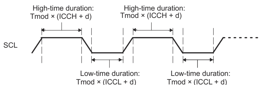
Figure 16-4. Roles of the Clock Divide-Down Values (ICCL and ICCH)
