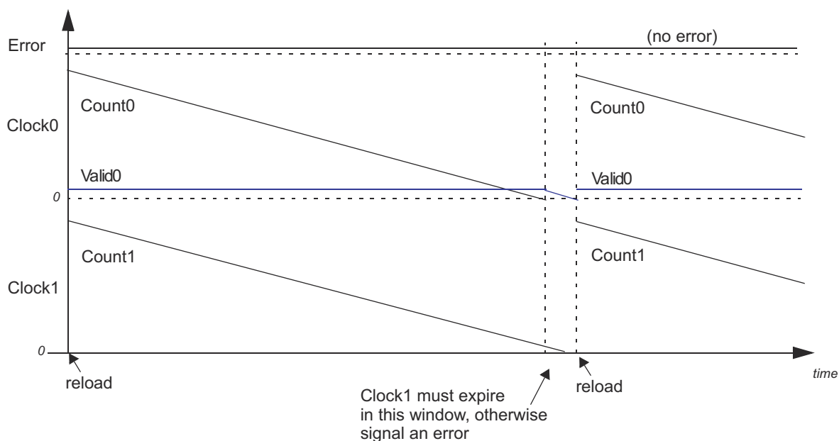
Figure 7-3. Counter Relationship
