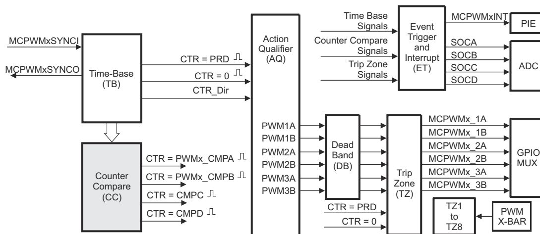
Figure 13-12. Counter-Compare Submodule
