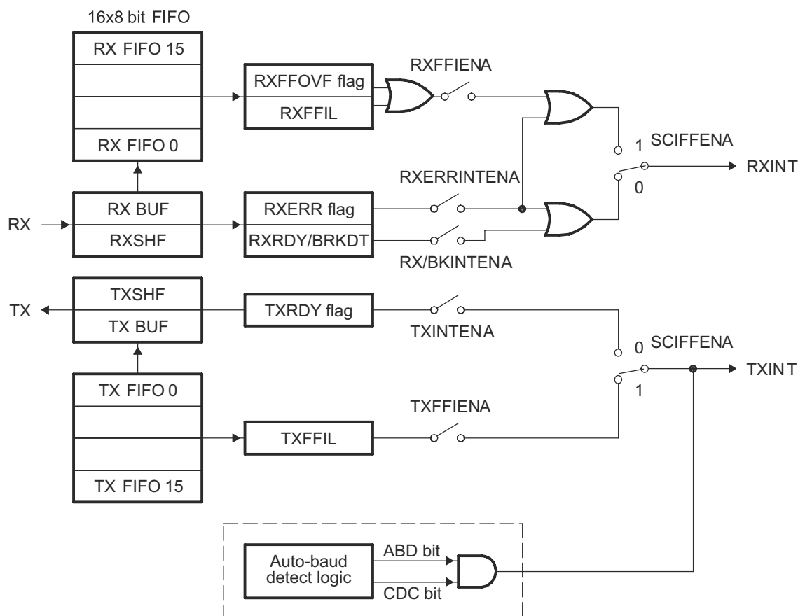
Figure 17-10. SCI FIFO Interrupt Flags and Enable Logic
