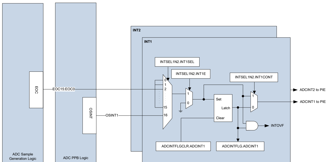
Figure 11-9. ADC End-of-Conversion (EOC) Signal Interrupts
