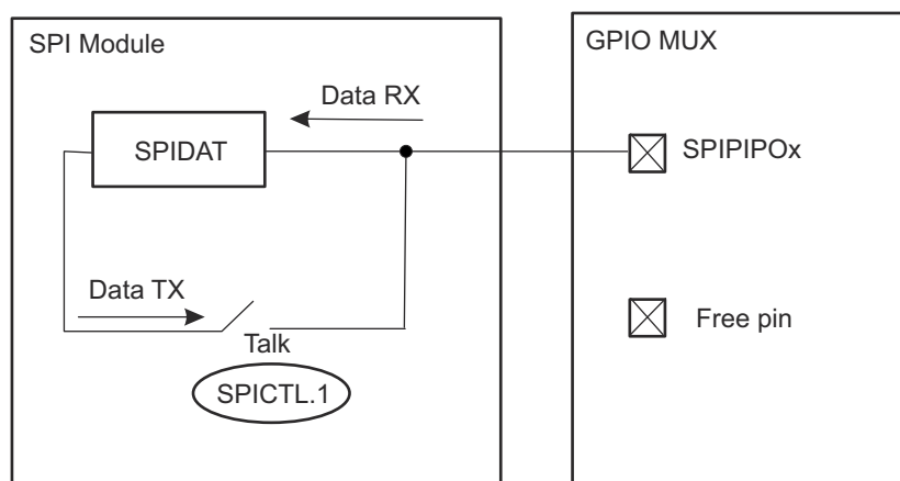
Figure 18-10. SPI 3-wire Peripheral Mode
