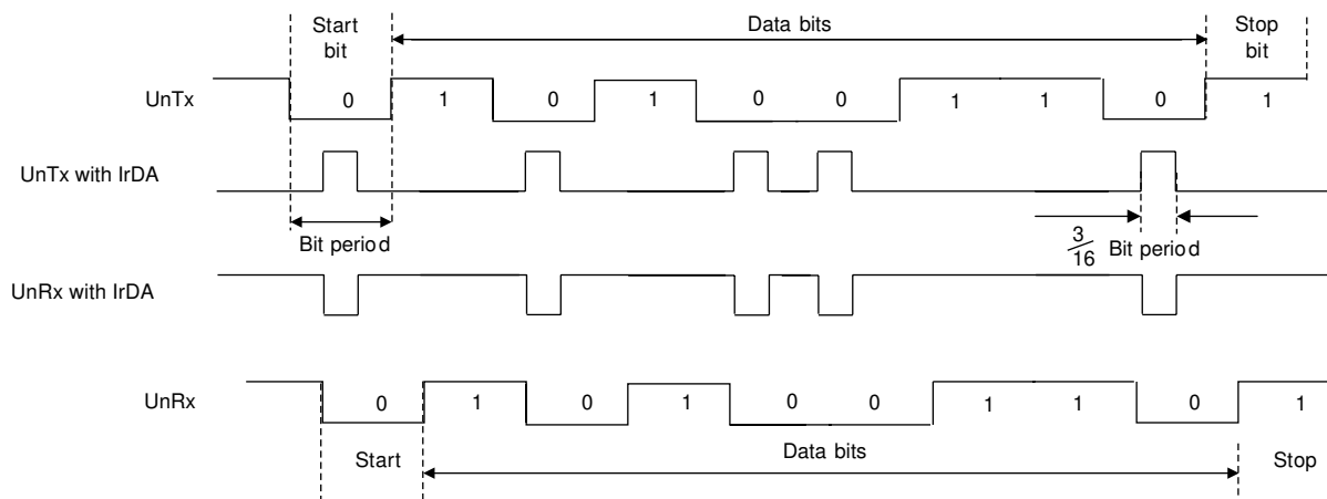
Figure 21-3. IrDA Data Modulation
