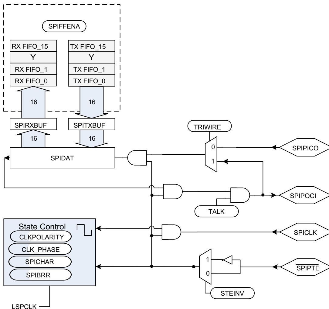
Figure 18-6. SPI Module Peripheral Configuration
