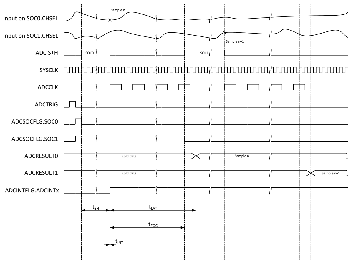
Figure 11-14. ADC Timings for 12-bit Mode in Early Interrupt Mode
