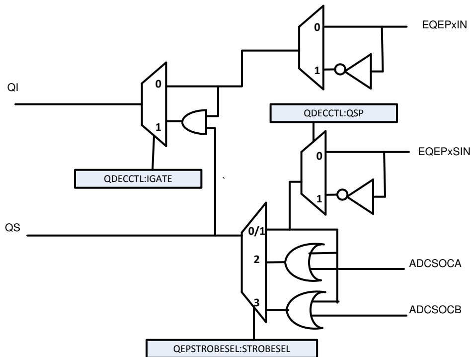
Figure 15-13. Latching Position Counter on ADCSOCA/ADCSOCB Event
