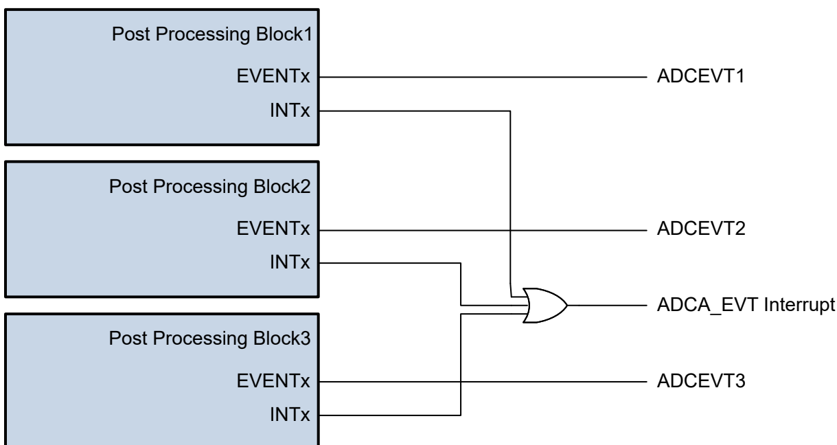
Figure 11-11. ADC Post-Processing Blocks (PPB) Interrupt Event
