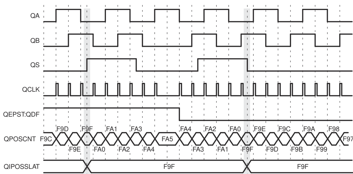
Figure 15-12. Strobe Event Latch (QEPCTL[SEL] = 1)
