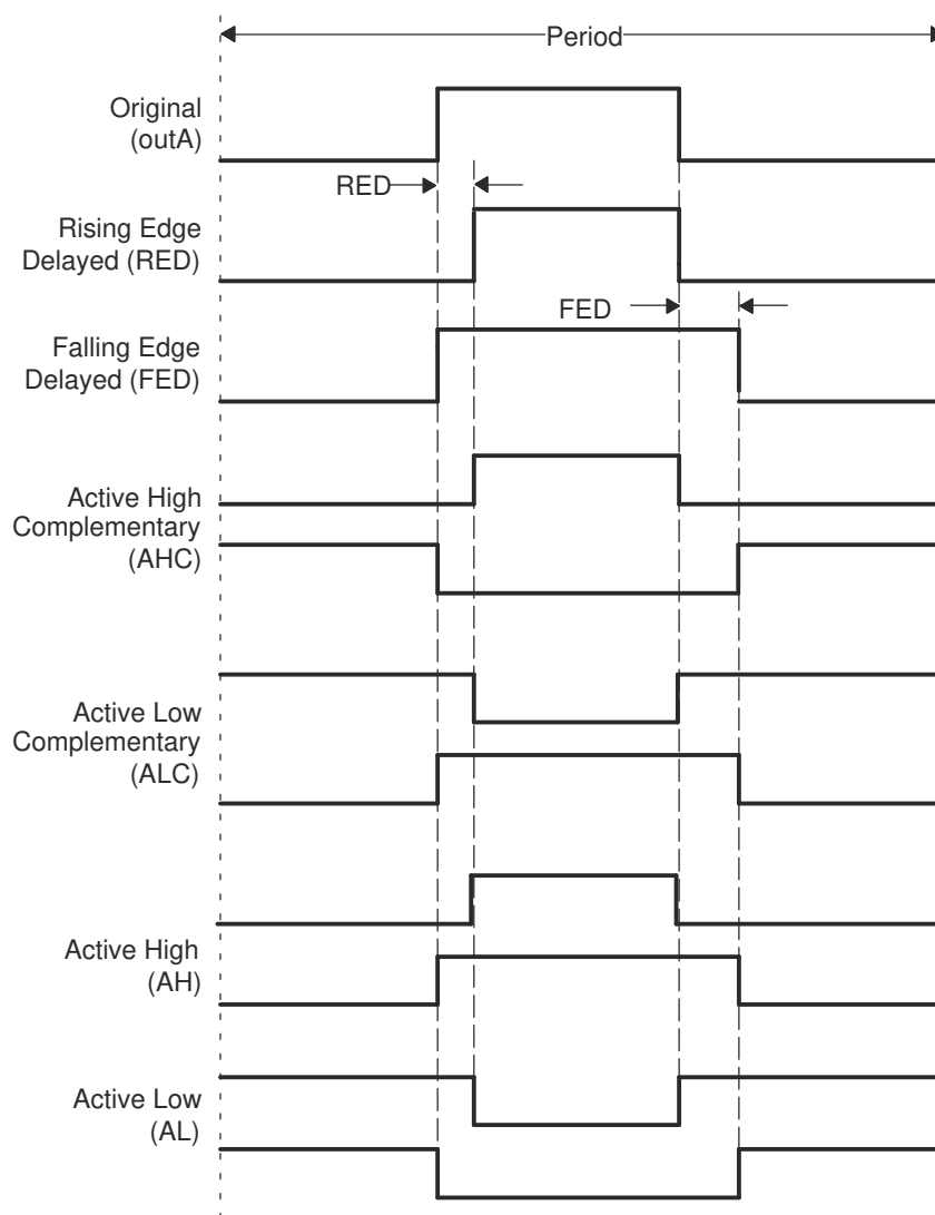
Figure 13-31. Dead-Band Waveforms for Typical Cases (0% < Duty < 100%)
