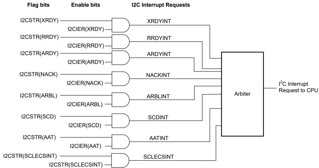
Figure 16-19. Enable Paths of the I2C Interrupt Requests
