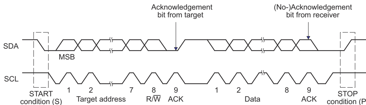
Figure 16-9. I2C Module Data Transfer (7-Bit Addressing with 8-bit Data Configuration Shown)
