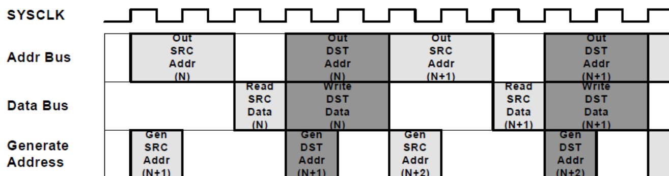
Figure 20-6. 3-stage Pipeline with One Read Stall
