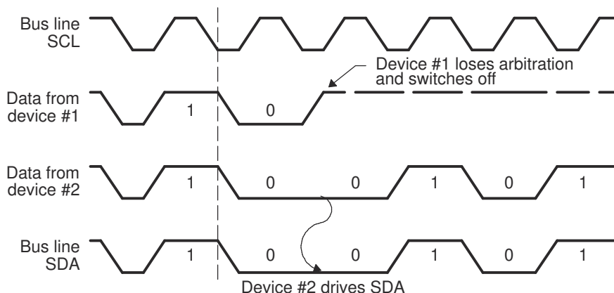
Figure 16-17. Arbitration Procedure Between Two Controller-Transmitters
