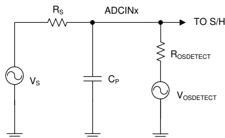
Figure 11-13. Input Circuit Equivalent with OSDETECT Enabled
