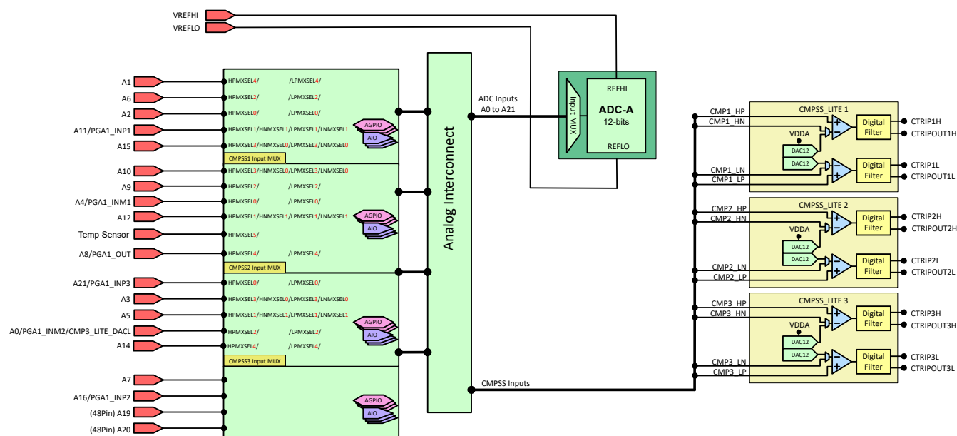
Figure 10-1. Analog Subsystem Block Diagram
