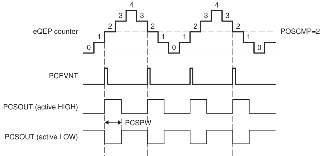
Figure 15-15. eQEP Position-compare Event Generation Points
