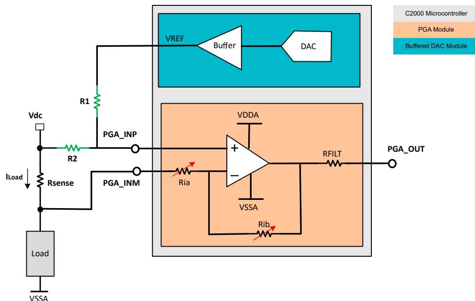
Figure 19-15. Bidirectional Current Sensing
