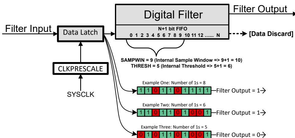
Figure 12-5. Digital Filter Behavior
