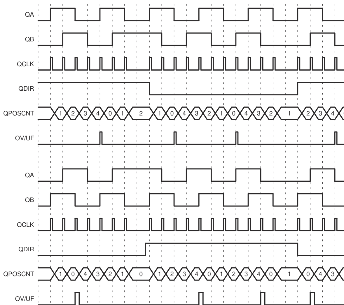
Figure 15-10. Position Counter Underflow/Overflow (QPOS MAX = 4)
