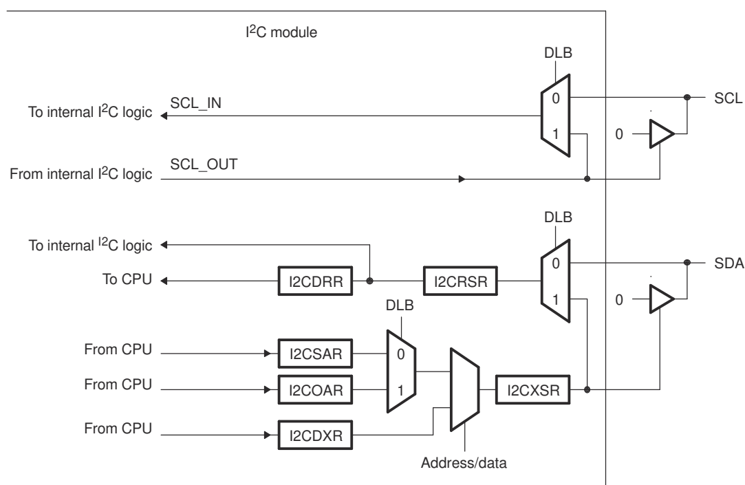
Figure 16-18. Pin Diagram Showing the Effects of the Digital Loopback Mode (DLB) Bit
