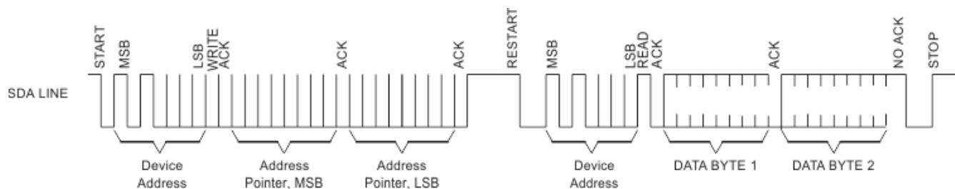
Figure 4-10. Random Read
