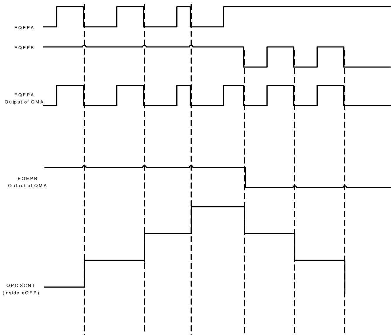
Figure 15-23. QMA Mode-1
