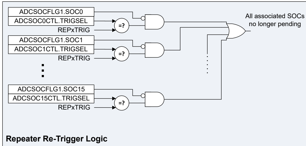
Figure 11-5. Trigger Repeater Repeat Logic
