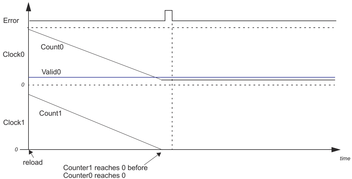
Figure 7-5. Clock1 Faster Than Clock0 - Results in an Error and Stops Counting
