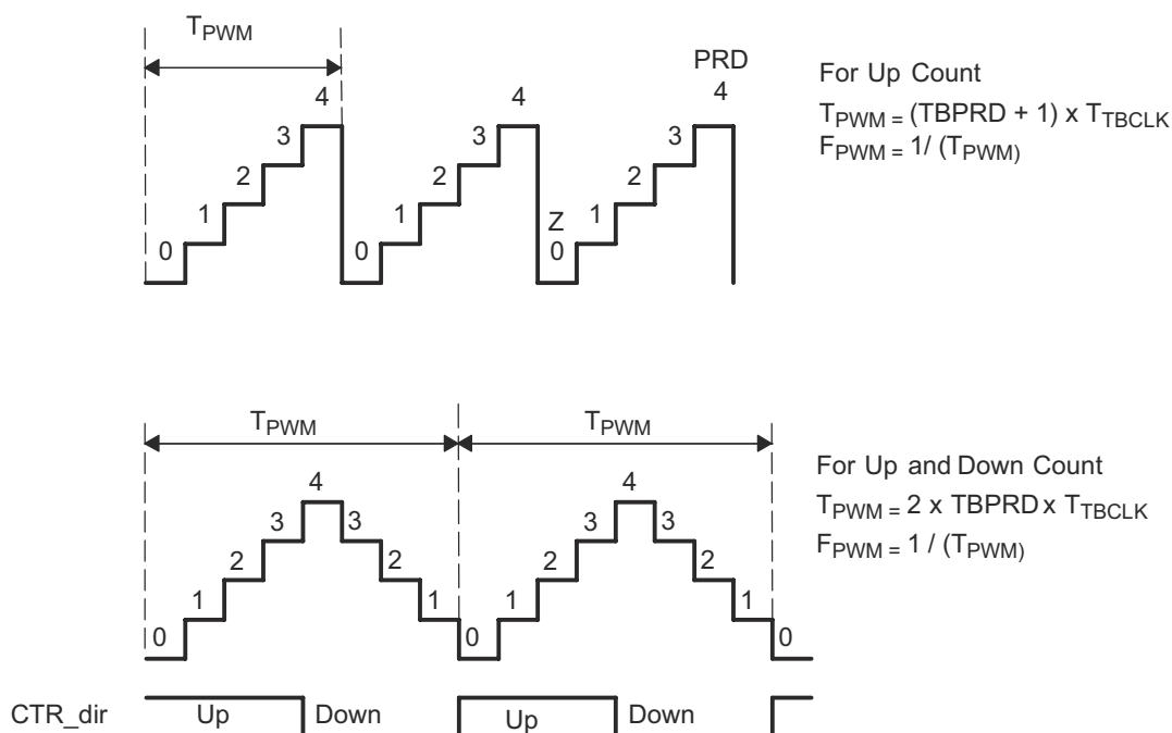
Figure 13-5. Time-Base Frequency and Period
