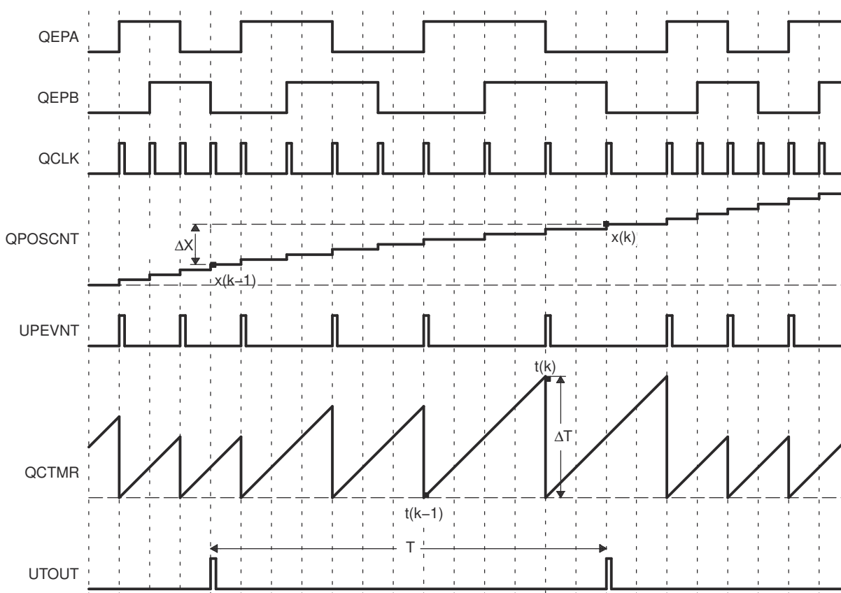
Figure 15-19. eQEP Edge Capture Unit - Timing Details
