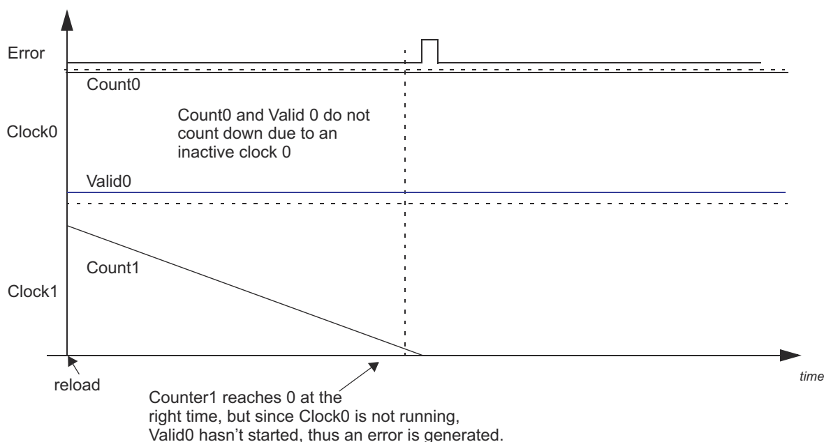
Figure 7-7. Clock0 Not Present - Results in an Error and Stops Counting
