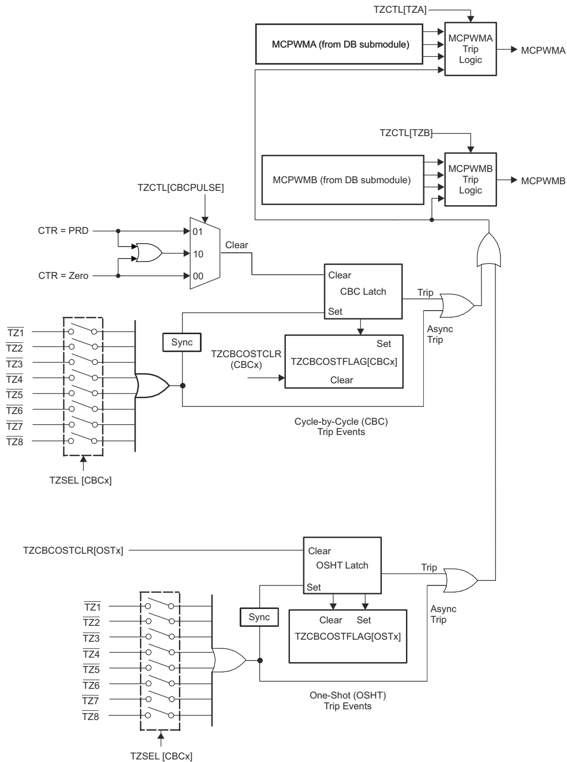
Figure 13-33. Trip-Zone Submodule Mode Control Logic
