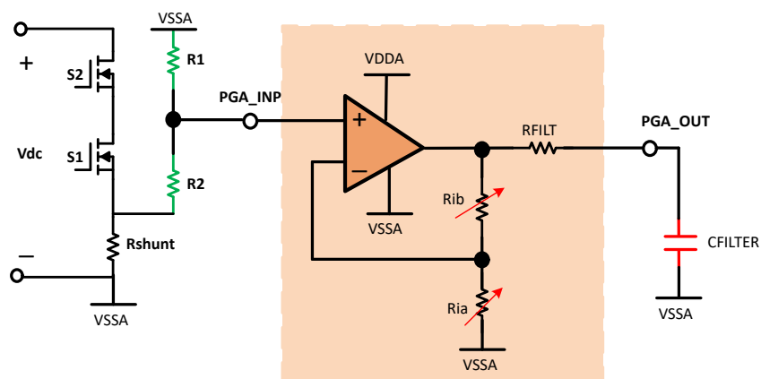
Figure 19-14. PGA Shunt Current Example
