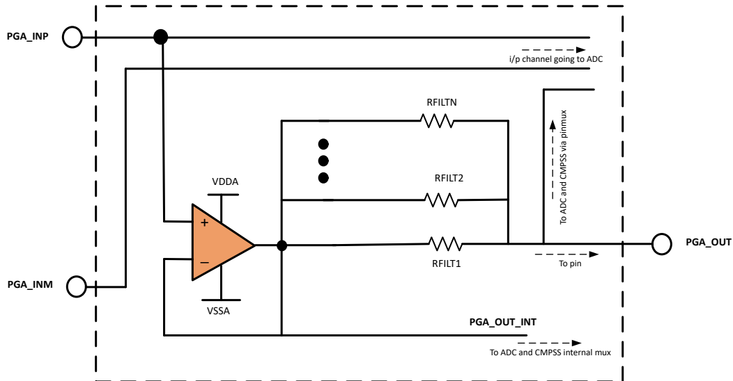
Figure 19-2. Buffer Mode
