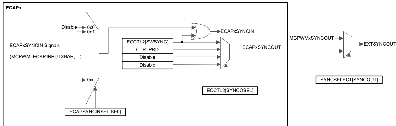
Figure 14-8. eCAP Synchronization Scheme
