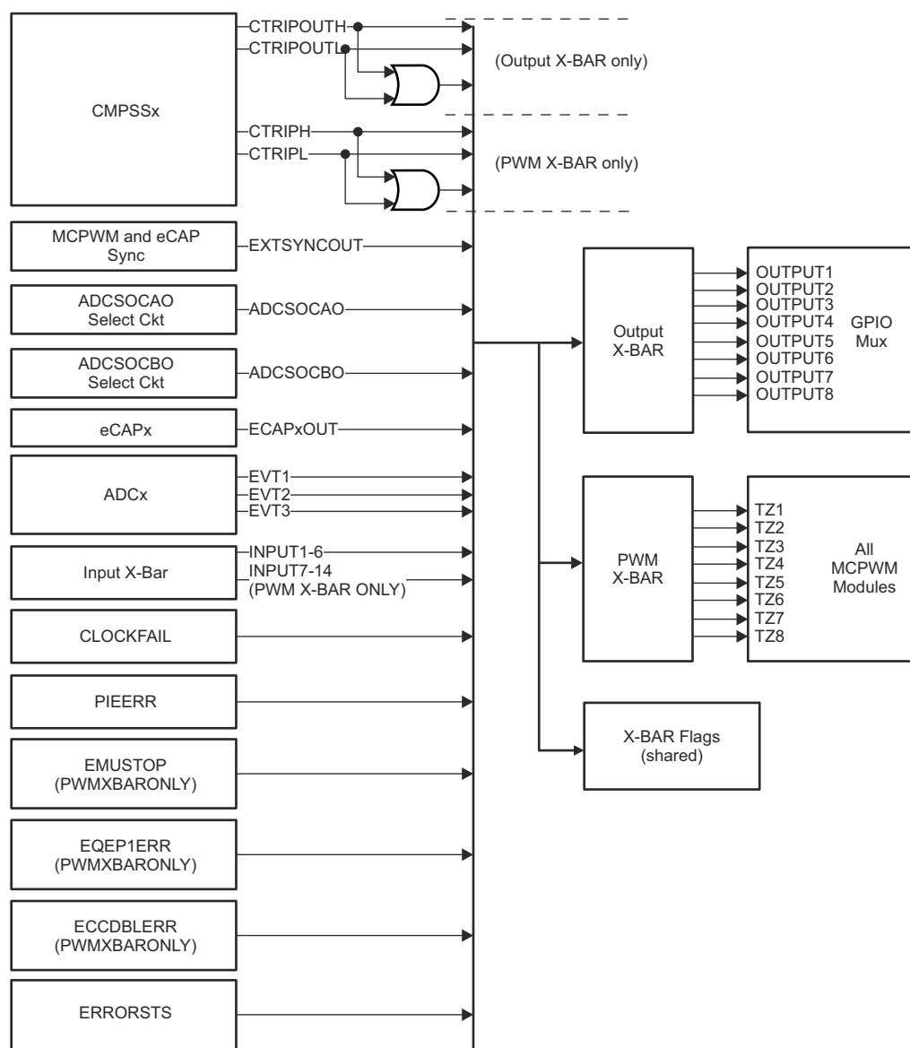
Figure 13-38. PWM X-BAR
