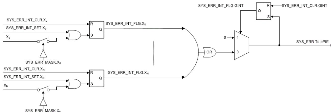
Figure 3-3. System Error
