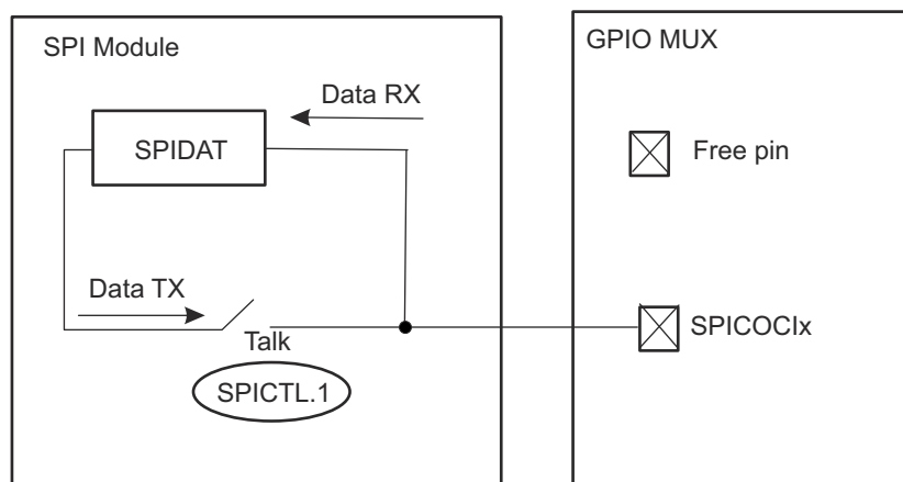
Figure 18-9. SPI 3-wire Controller Mode
