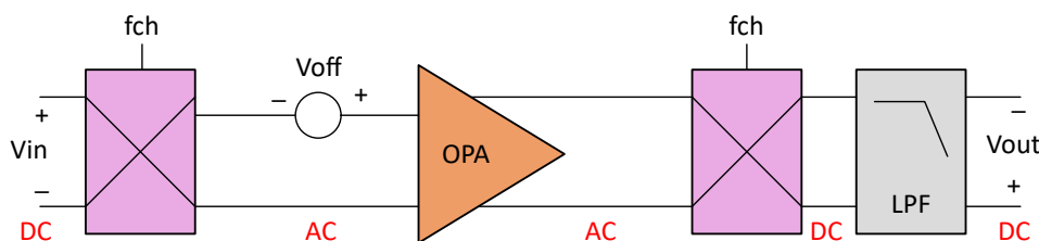
Figure 19-9. General Chopping Technique
