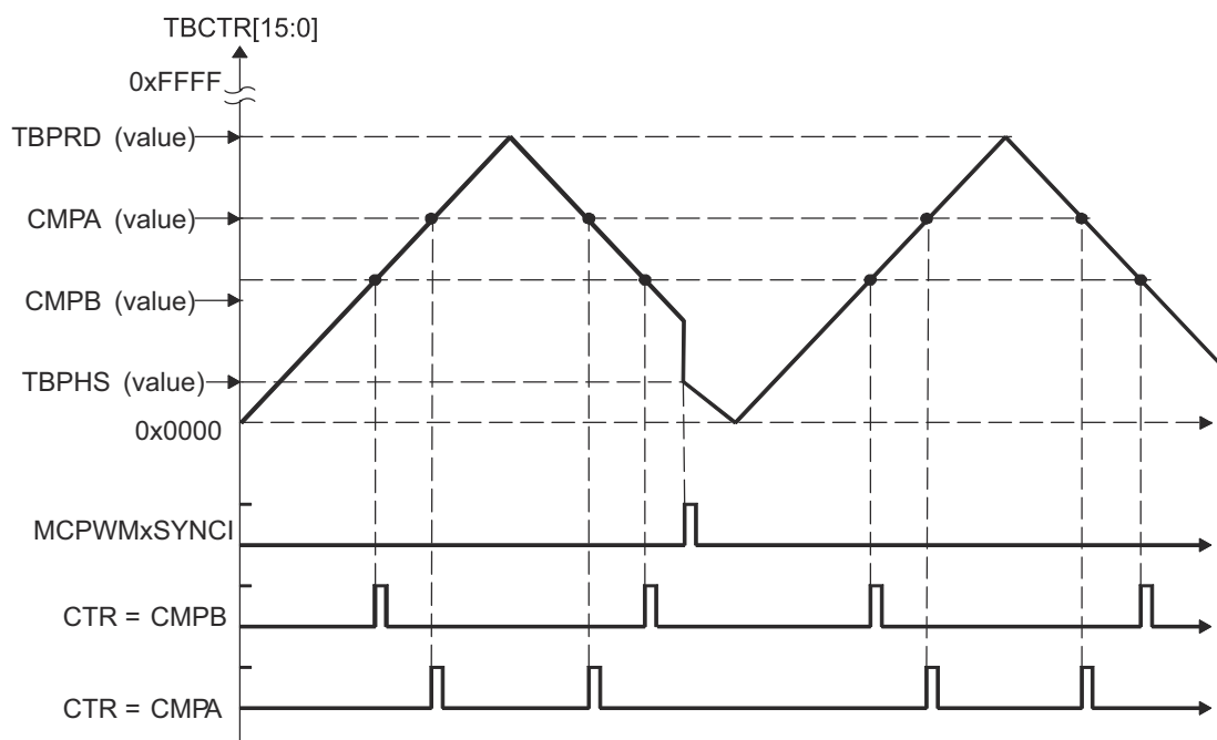
Figure 13-15. Counter-Compare Events In Up-Down Count Mode, TBCTL[PHSDIR] = 0 Count Down On Synchronization Event
