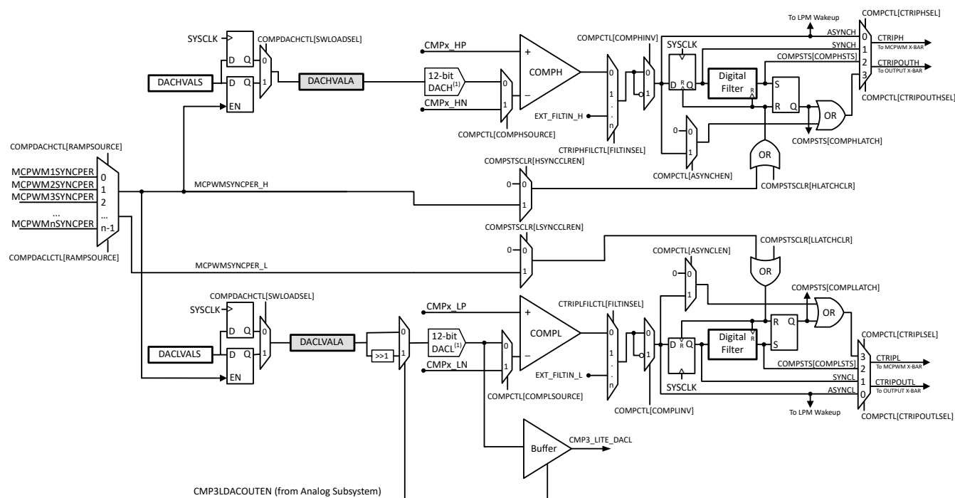
Figure 12-2. CMPSS_LITE Module Block Diagram
