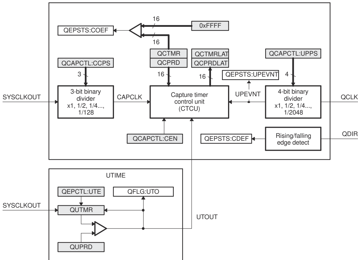
Figure 15-17. eQEP Edge Capture Unit
