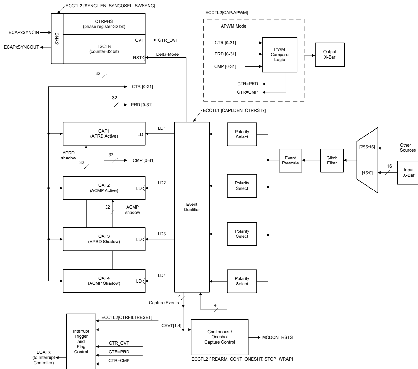
Figure 14-3. eCAP Block Diagram
