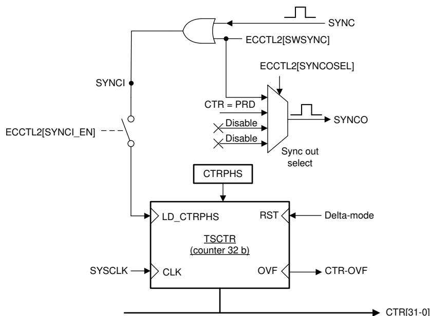
Figure 14-7. Details of the Counter and Synchronization Block
