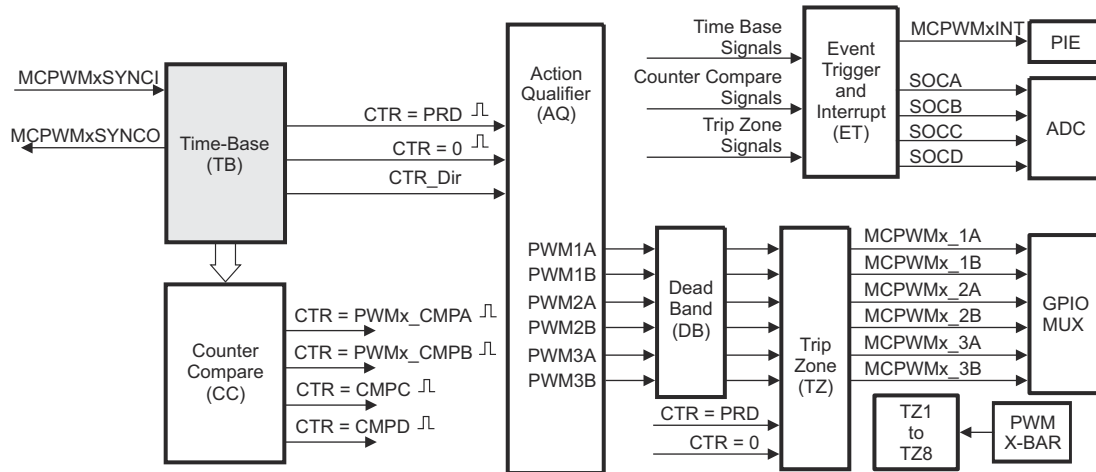
Figure 13-3. Time-Base Submodule
