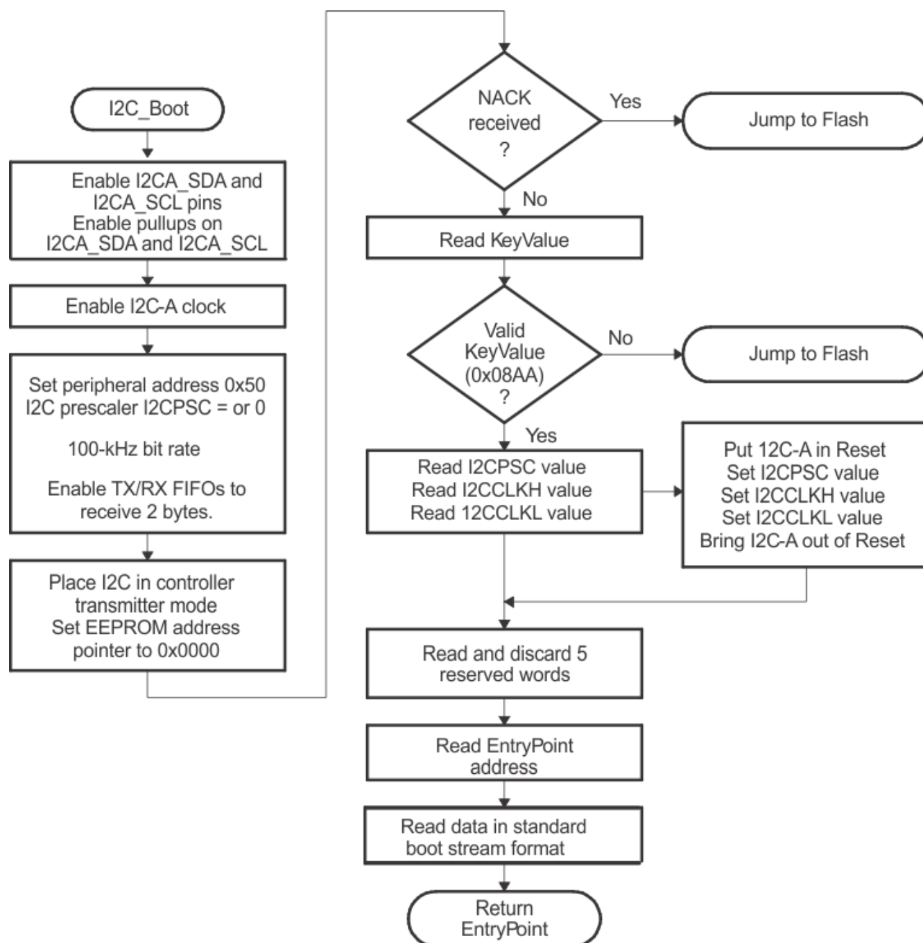
Figure 4-9. Overview of I2C Boot Function
