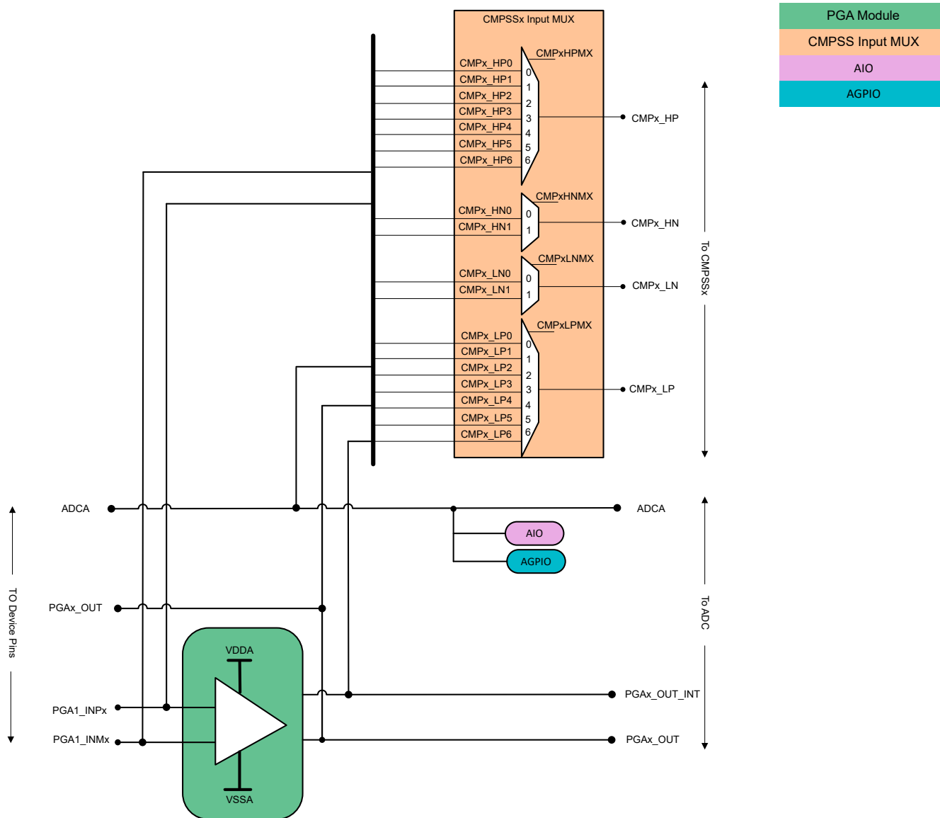
Figure 10-2. Analog Group Connections
