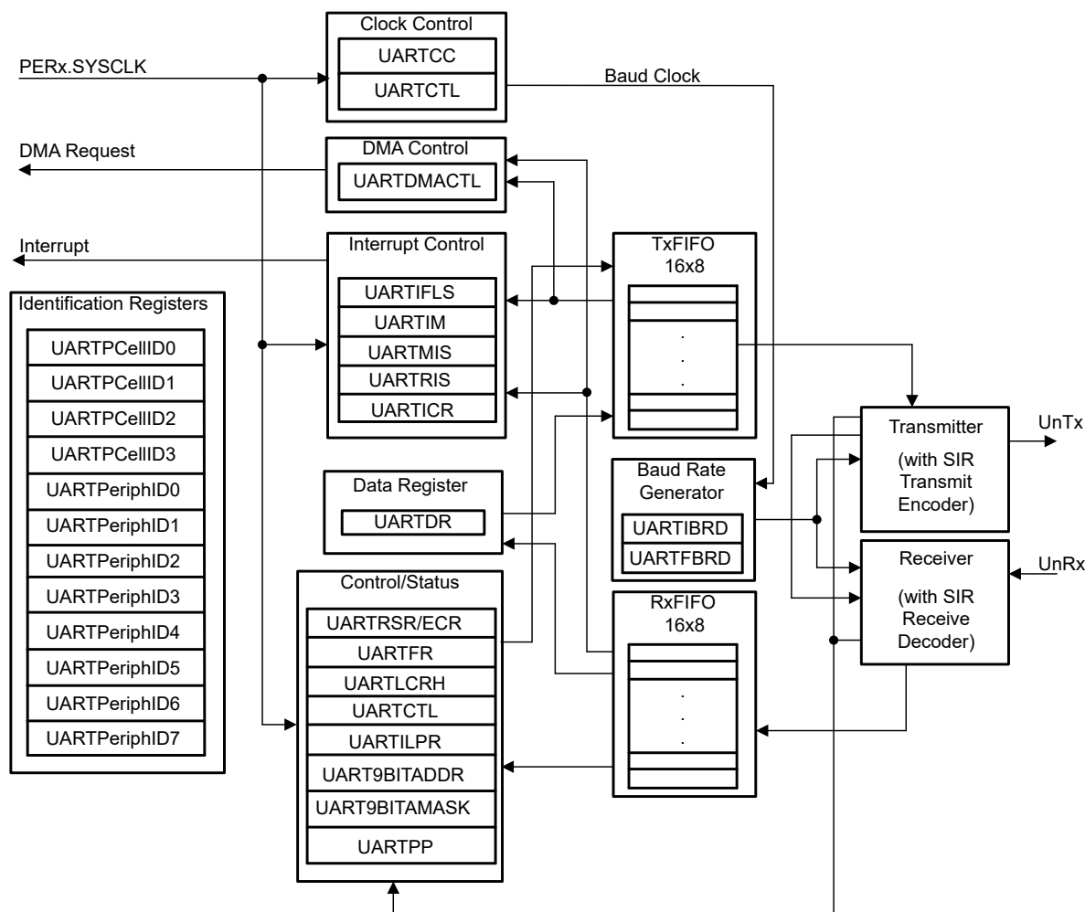
Figure 21-1. UART Module Block Diagram
