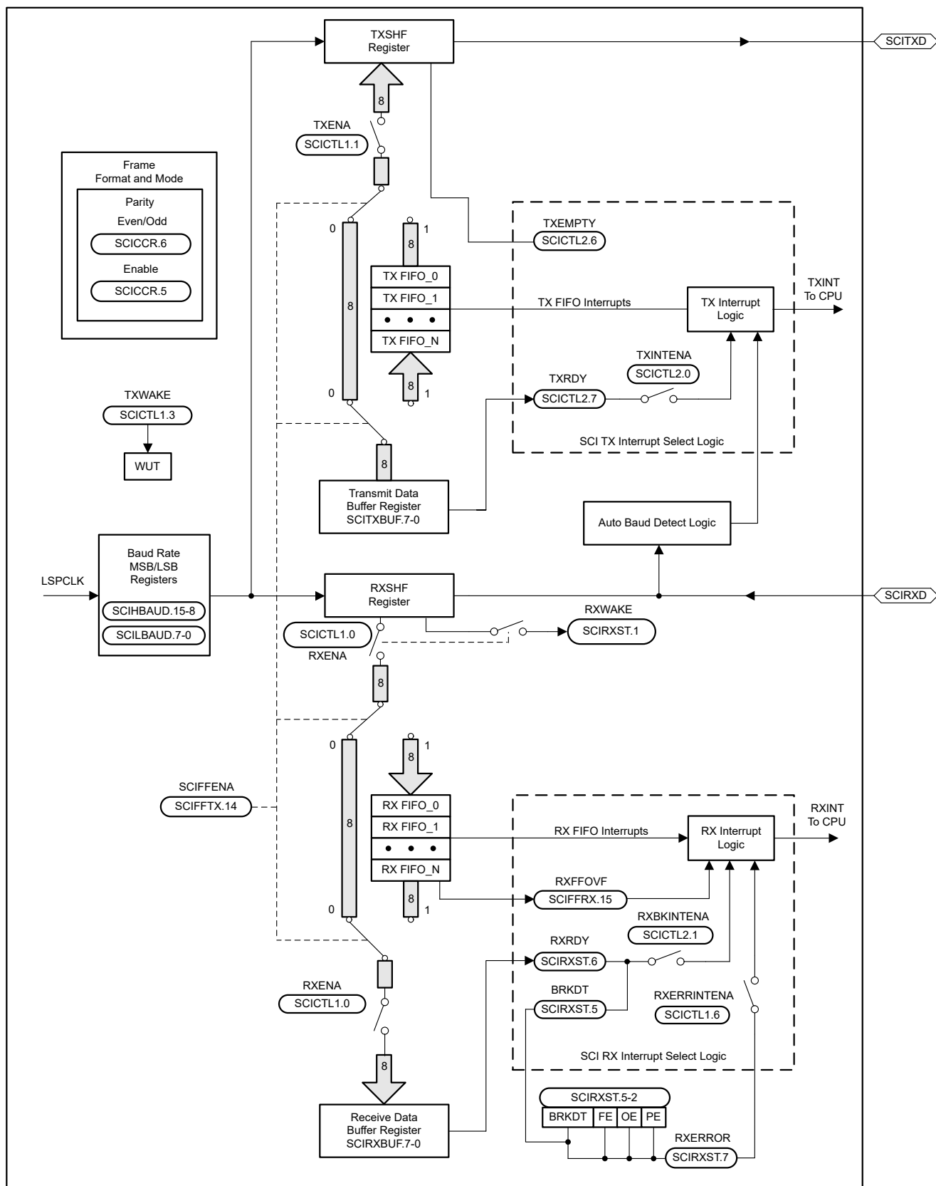
Figure 17-2. Serial Communications Interface (SCI) Module Block Diagram
