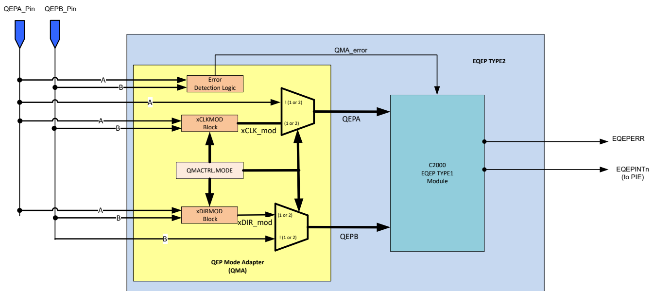
Figure 15-22. QMA Module Block Diagram
