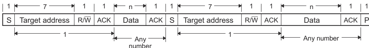
Figure 16-13. Repeated START Condition (in This Case, 7-Bit Addressing Format)
