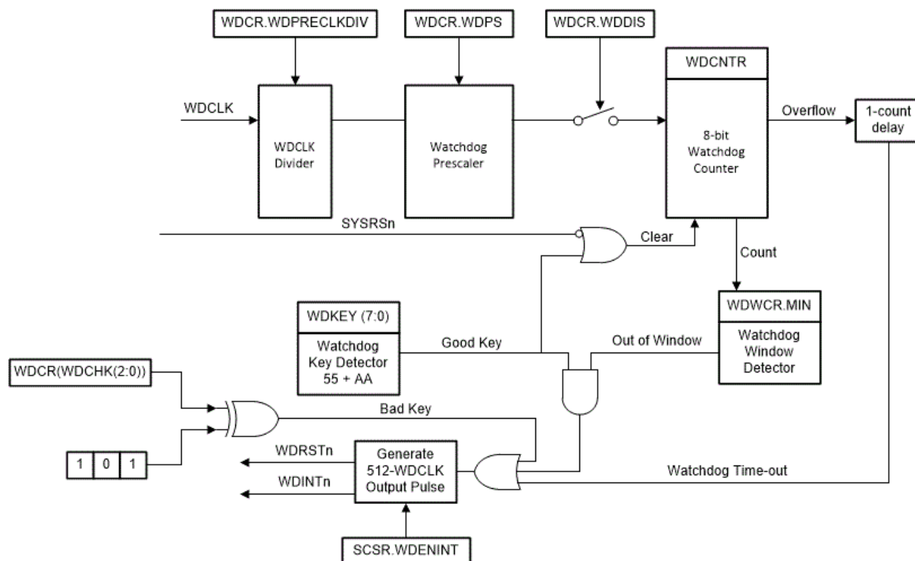
Figure 3-13. Watchdog Timer Module
