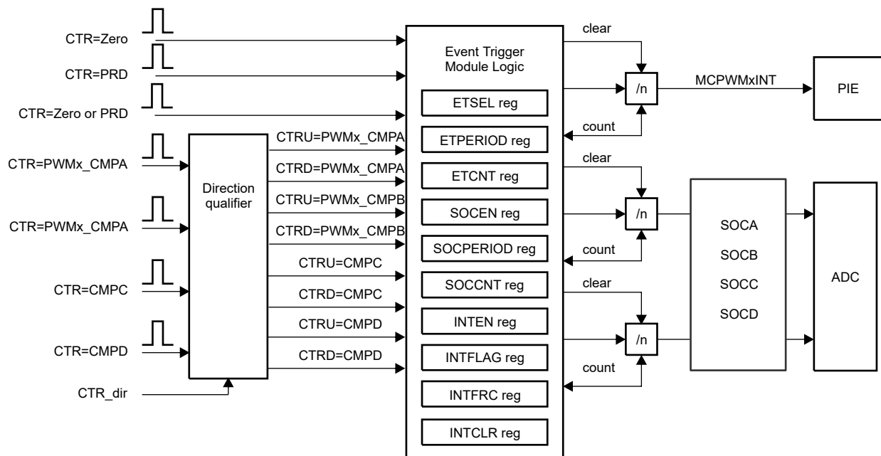
Figure 13-35. Event-Trigger Submodule Showing Event Inputs and Prescaled Outputs
