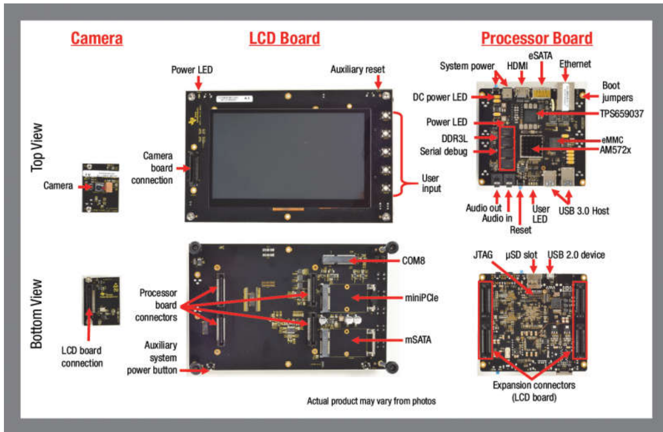
Figure 3-1. AM572x GP EVM Key Components
