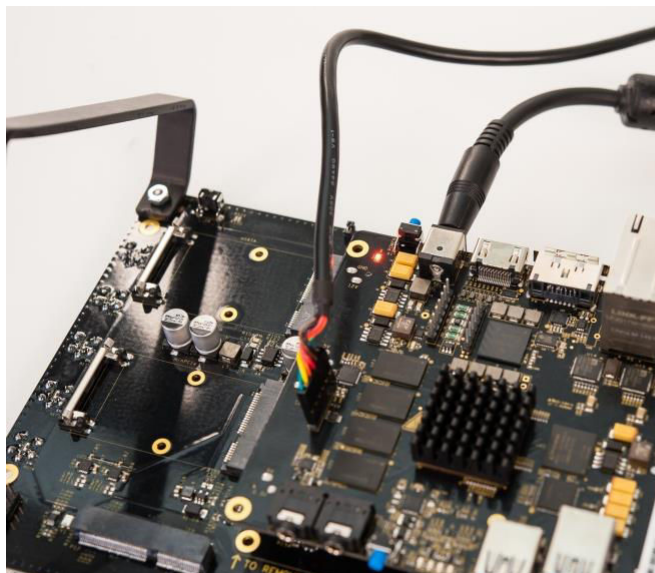
Figure 4-2. AM572x GP EVM DC Power Jack
