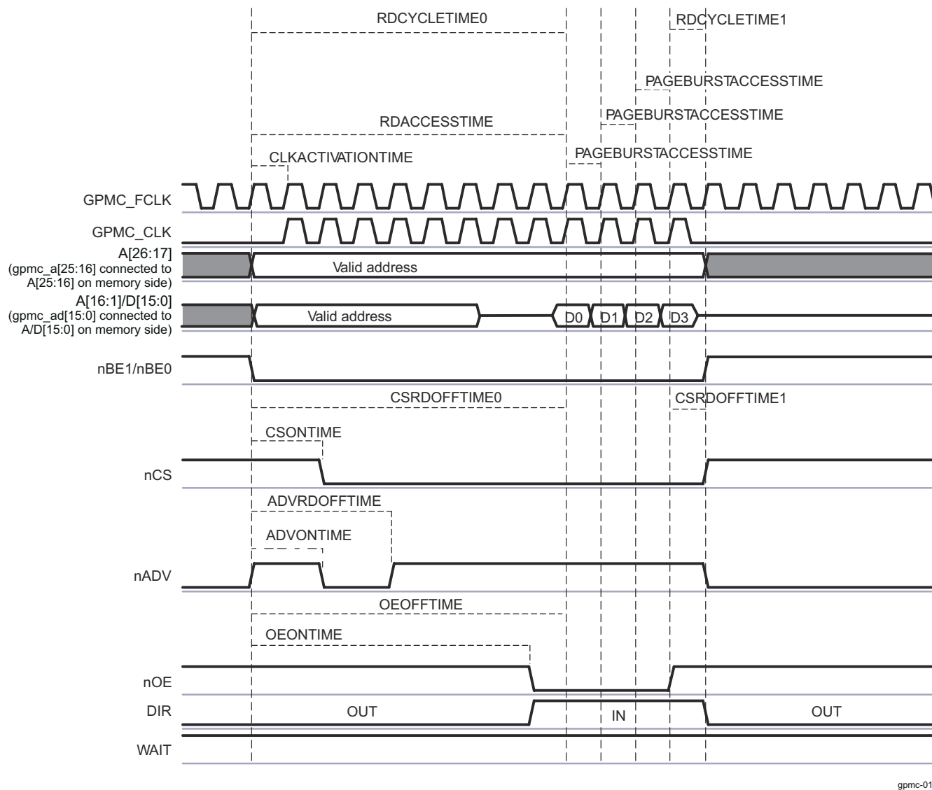
Figure 17-72. Synchronous Multiple (Burst) Read (GPMCCLKDIVIDER = 0)
