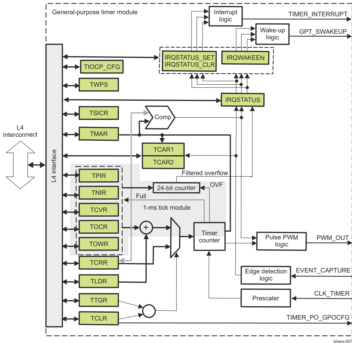
Figure 24-6. Block Diagram of TIMER1, TIMER2 and TIMER10
