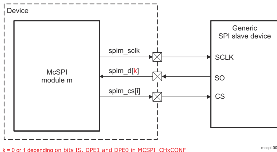
Figure 26-79. McSPI Master Single Mode (Receive Only)
