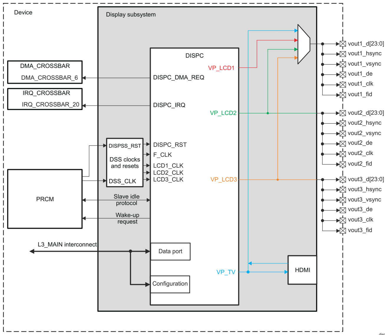
Figure 13-22. DISPC Overview
