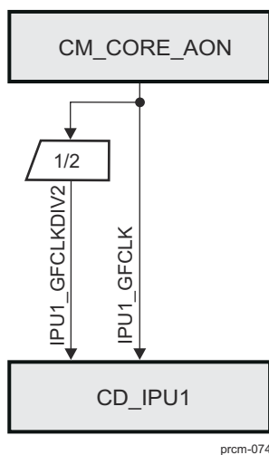
Figure 3-84. CD_IPU1 Overview
