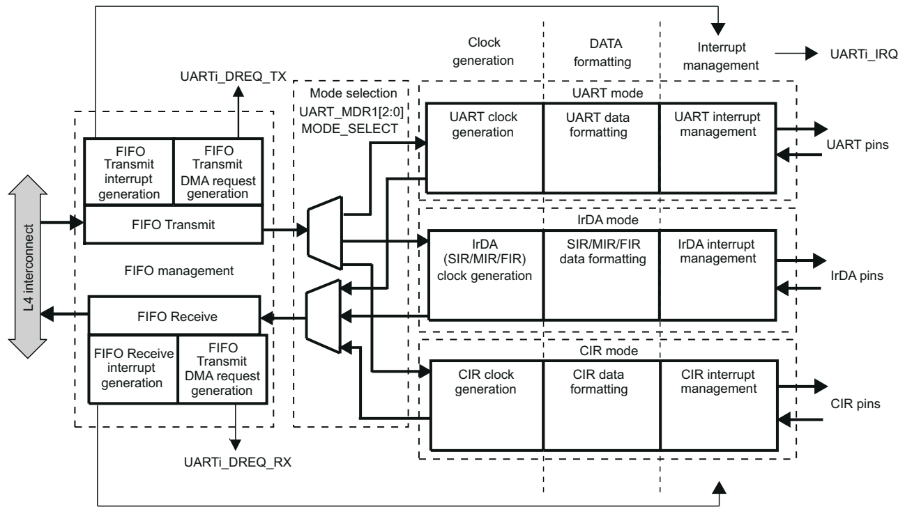
Figure 26-58. UART/IrDA/CIR Functional Block Diagram
