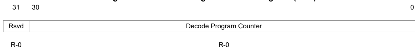
Figure 8-51. Decode Program Counter Register (DPC)
