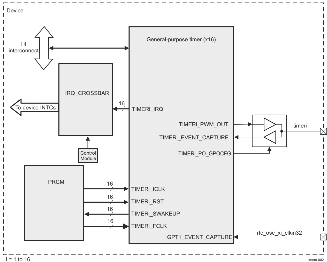
Figure 24-2. GP Timers Overview
