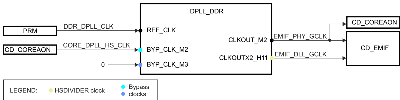
Figure 3-62. DPLL_DDR Overview
