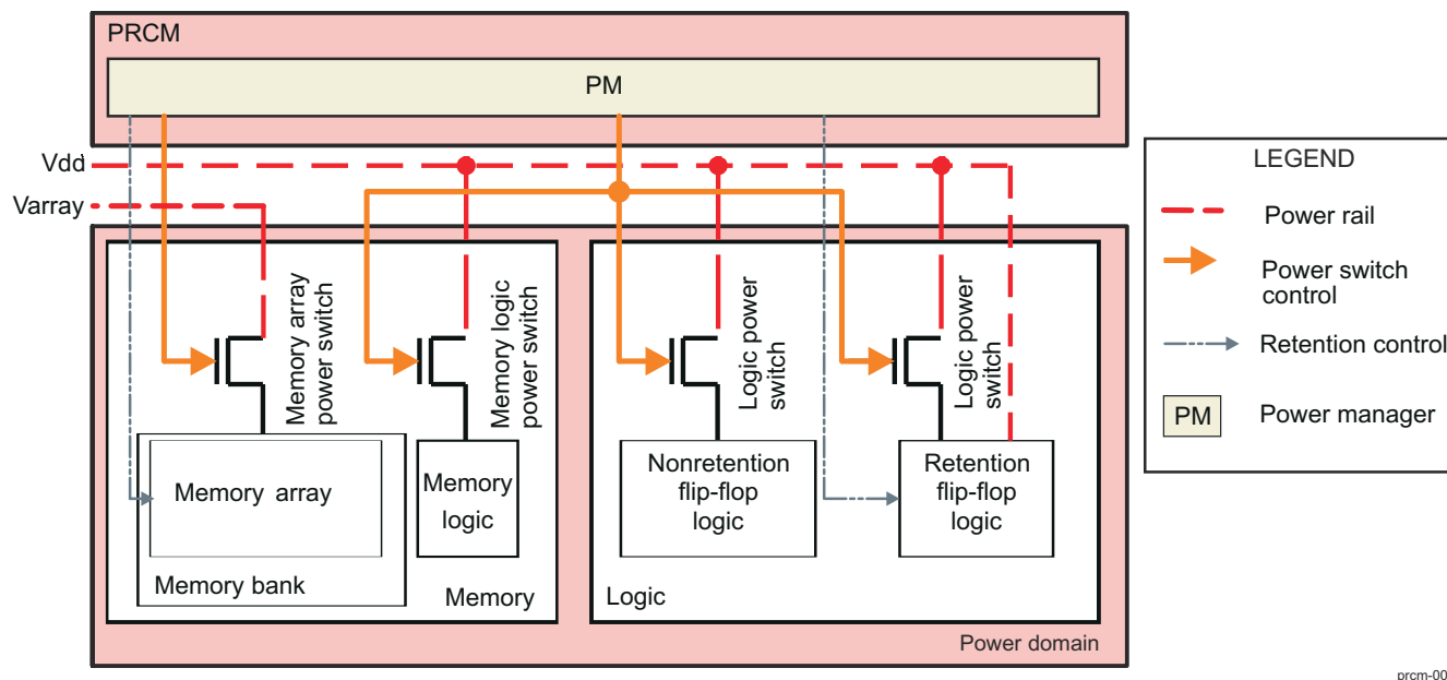
Figure 3-9. Generic Power Domain
