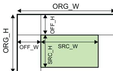
Figure 11-81. Input Image Trimming
