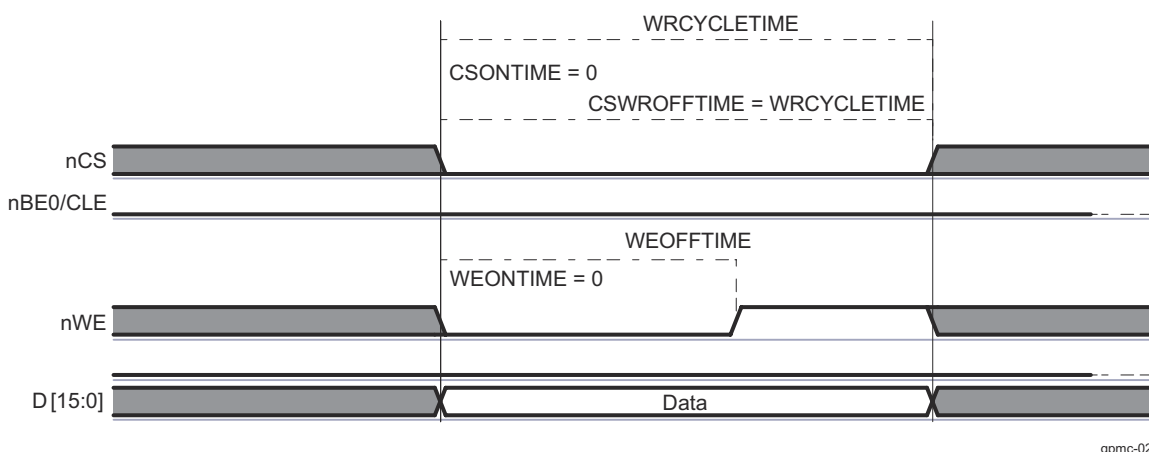
Figure 17-83. NAND Data Write Cycle
