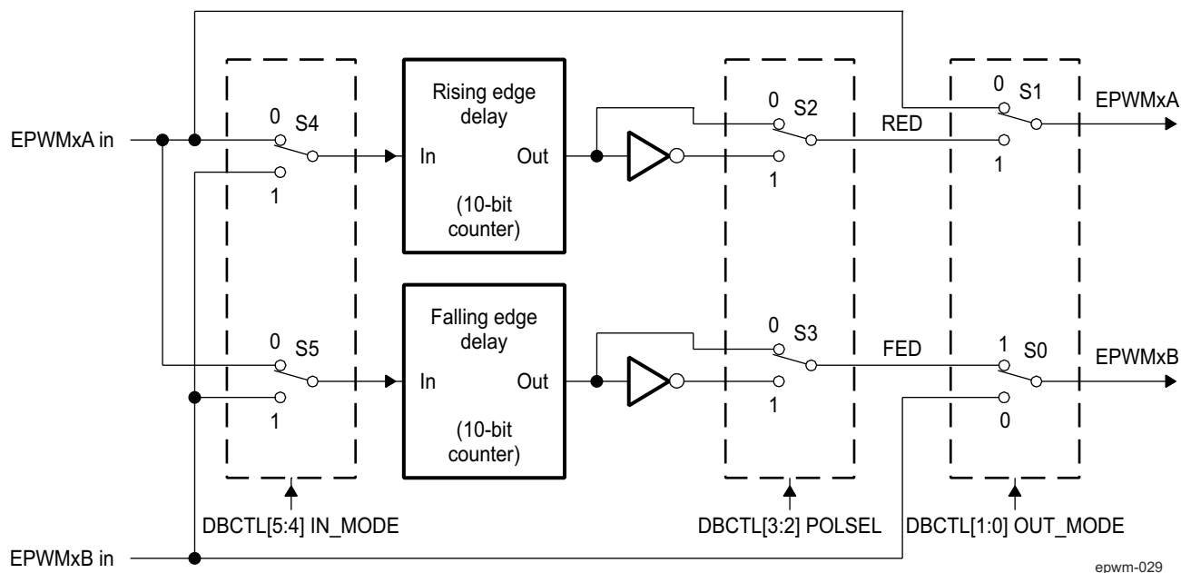
Figure 31-33. Configuration Options for the ePWM Dead-Band Generator Submodule
