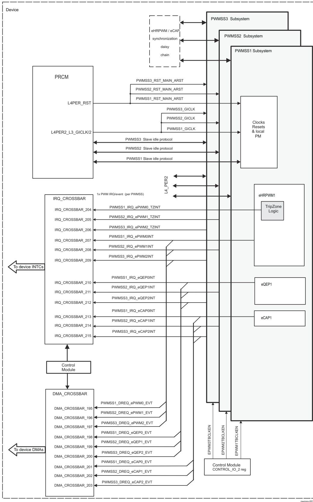
Figure 31-3. PWMSS Integration
