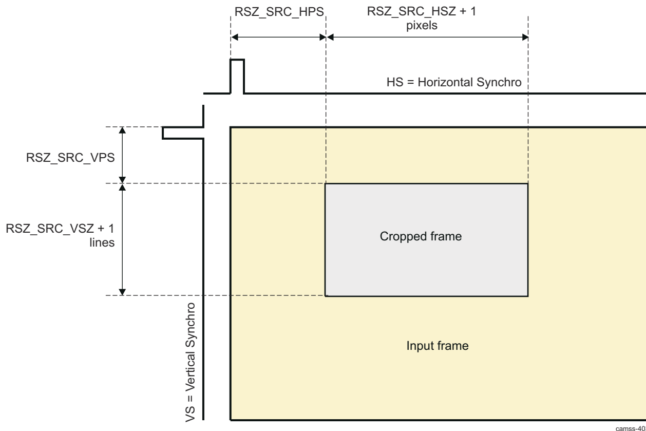
Figure 9-98. ISS ISP RSZ Input Data Cropping
