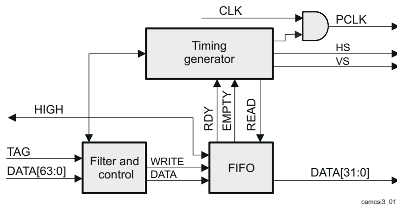
Figure 10-36. CAL Video Port and Timing Generator
