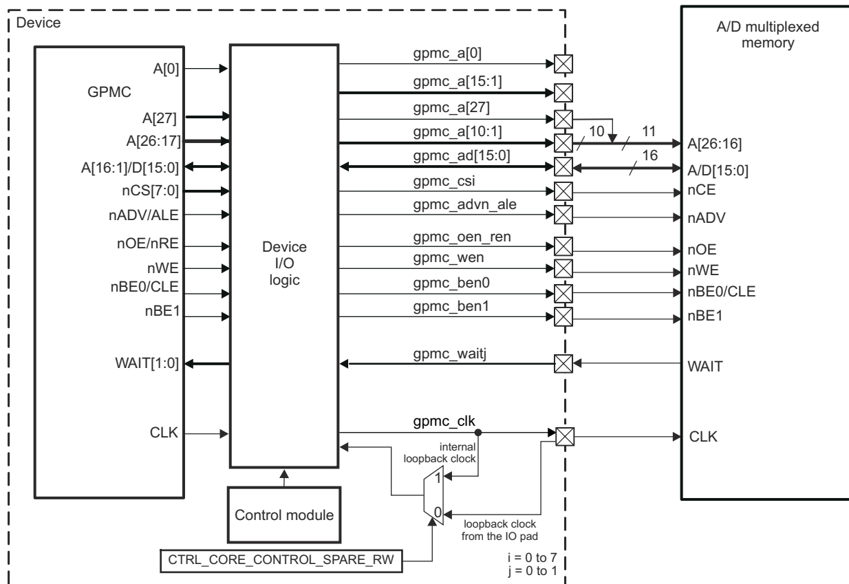
Figure 17-53. GPMC to 16-Bit Address/Data-Multiplexed Memory
