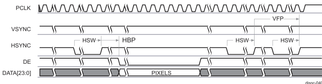
Figure 13-35. DISPC Active Matrix Timing Diagram of Configuration 2 (End of Frame)
