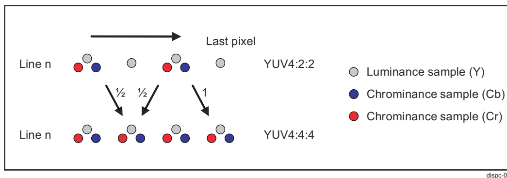
Figure 13-55. DISPC Averaging of the Chrominance Representation
