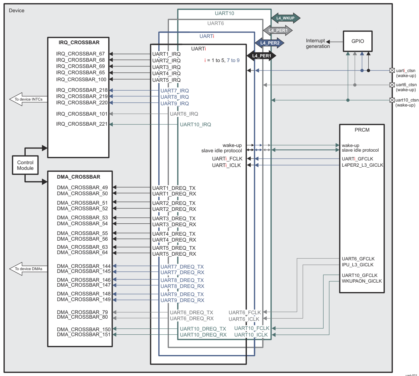
Figure 26-57. UART/IrDA/CIR Integration
