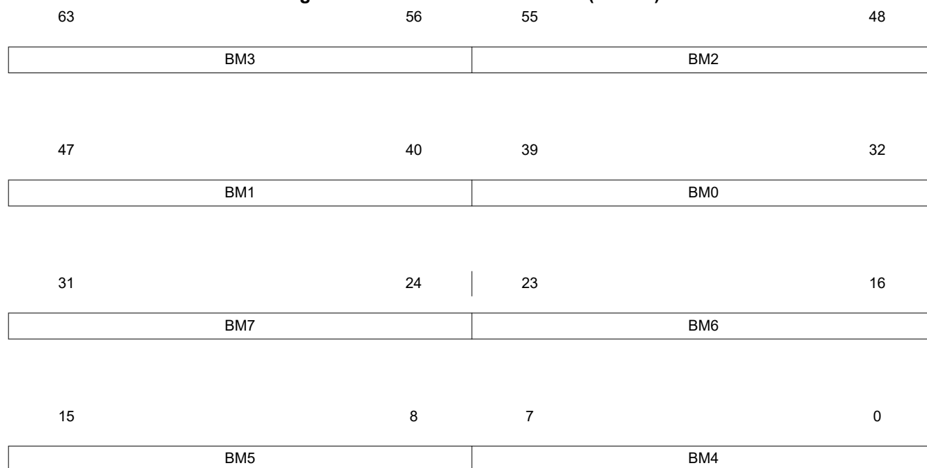
Figure 32-14. Data Source - EDMA (BM = 0)
