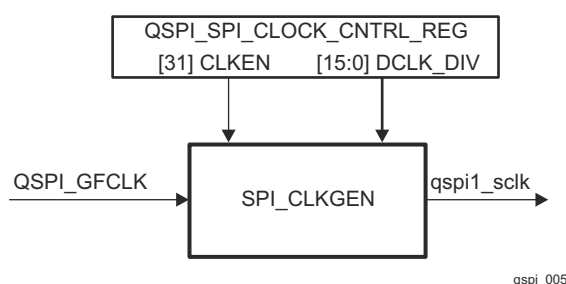
Figure 26-105. SPI_CLKGEN Block
