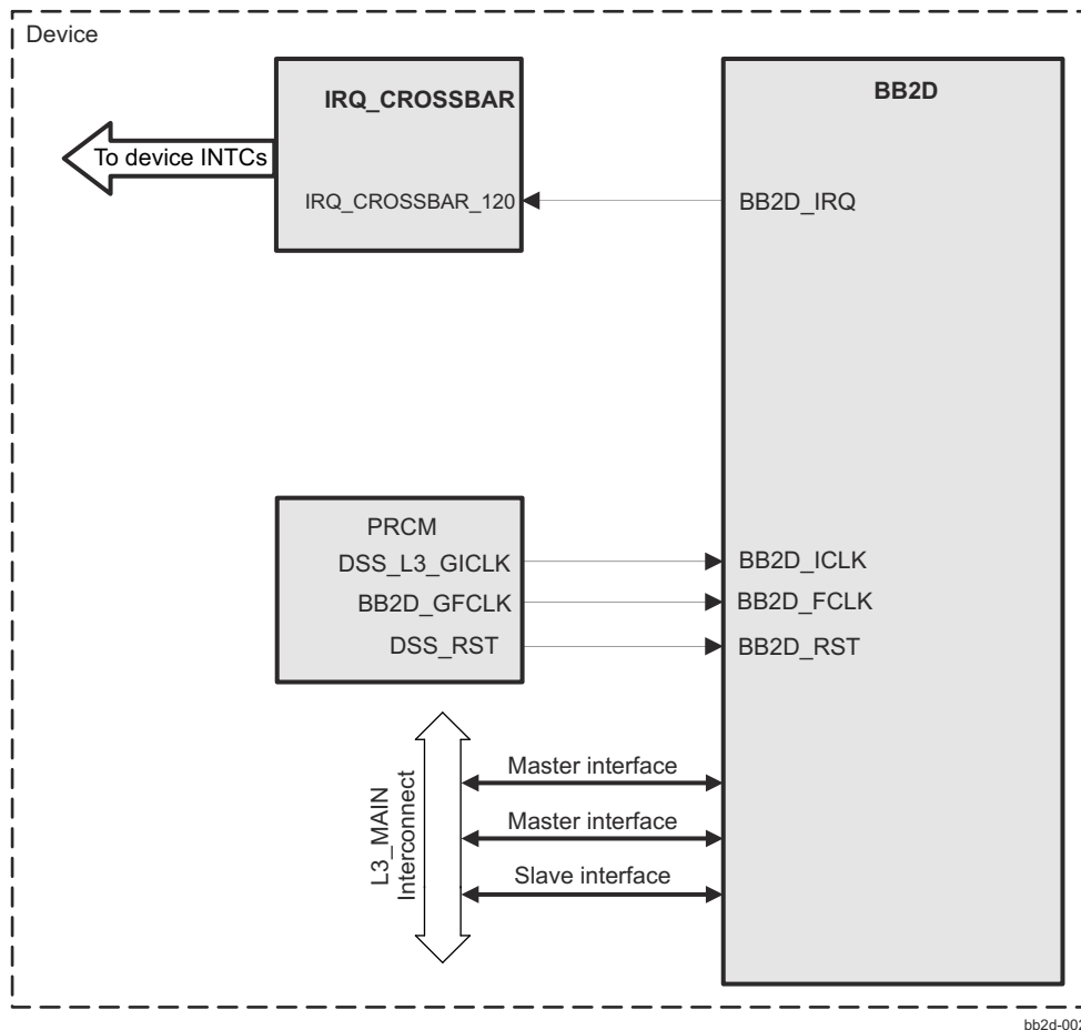
Figure 15-2. BB2D Integration
