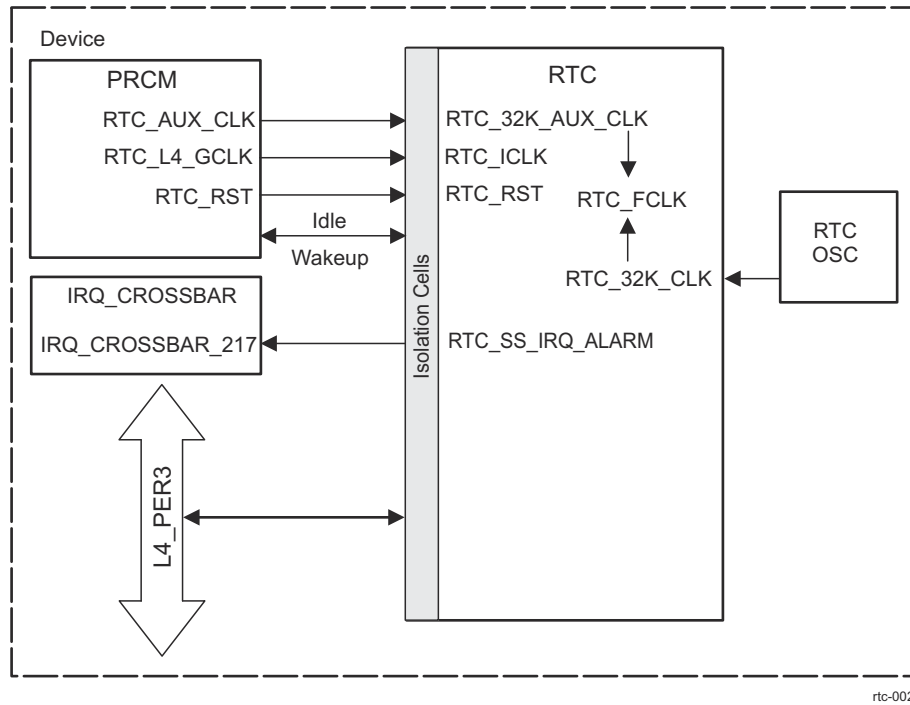
Figure 25-3. RTC Module Integration
