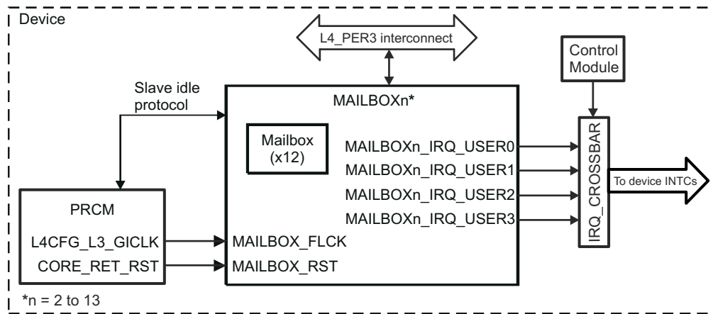
Figure 21-2. MAILBOX2..13 Integration
