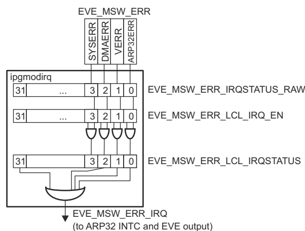
Figure 8-17. EVE Memory Switch Error Interrupt
