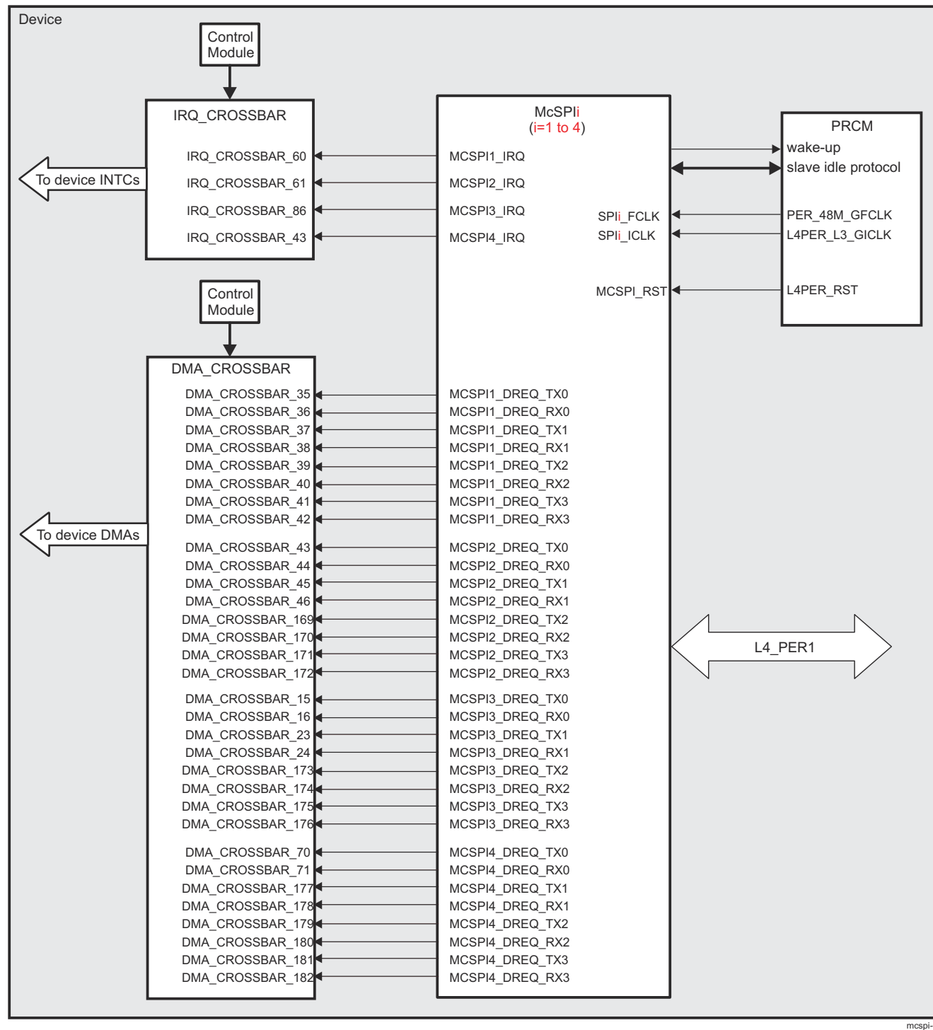
Figure 26-82. McSPI Integration
