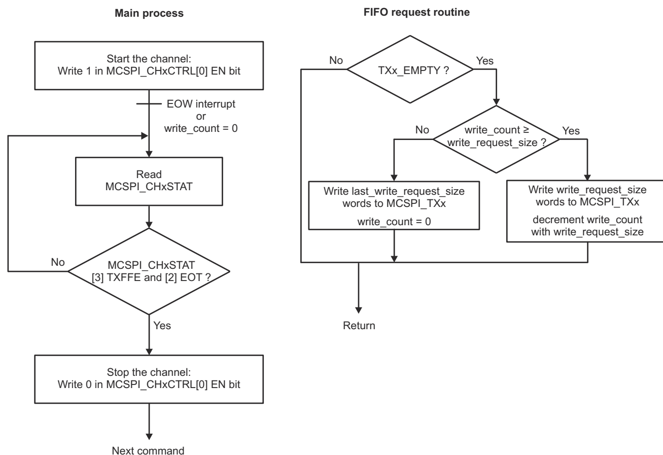
Figure 26-98. FIFO Mode Transmit-Only (Master)
