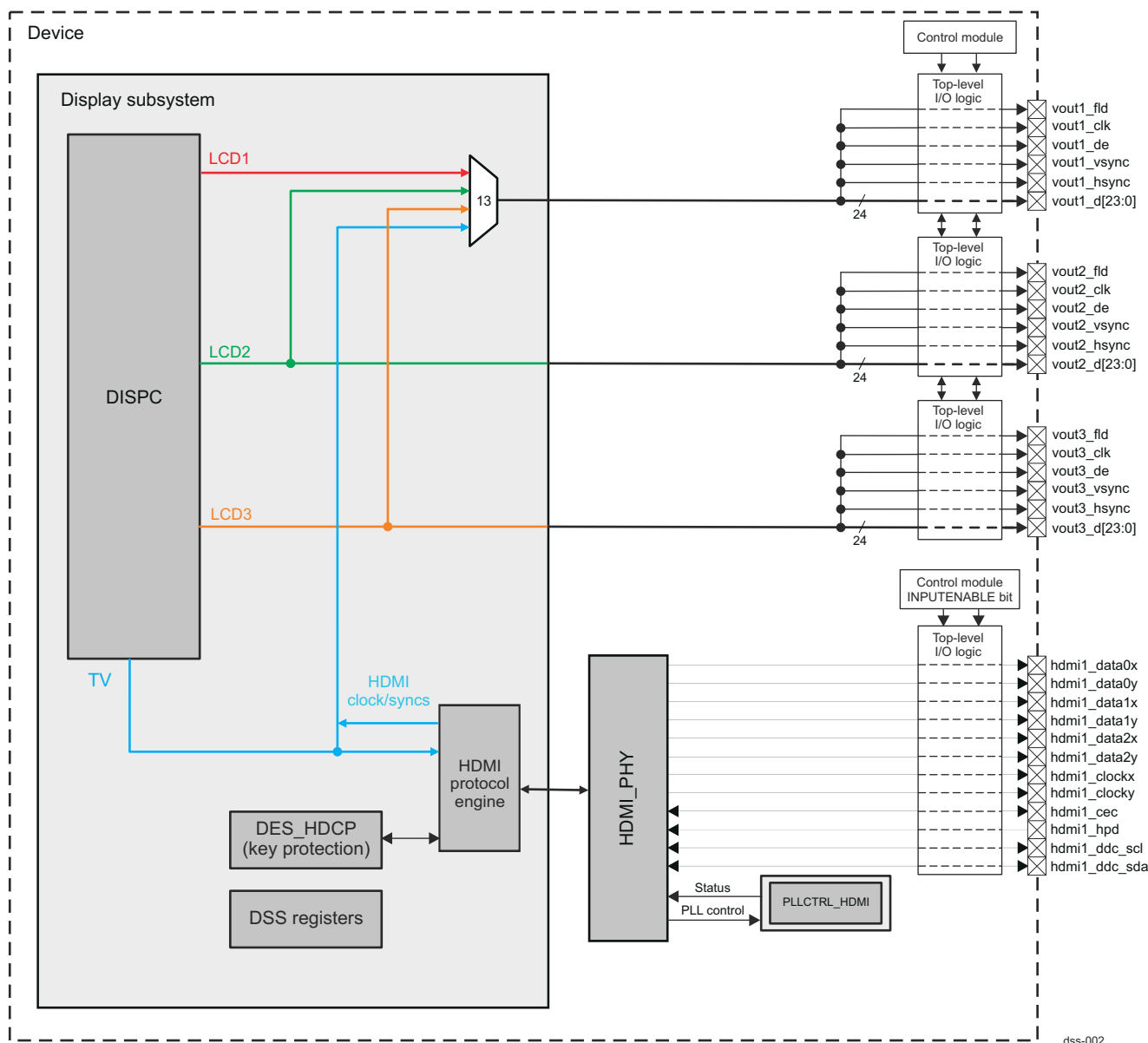
Figure 13-2. Display Subsystem Environment
