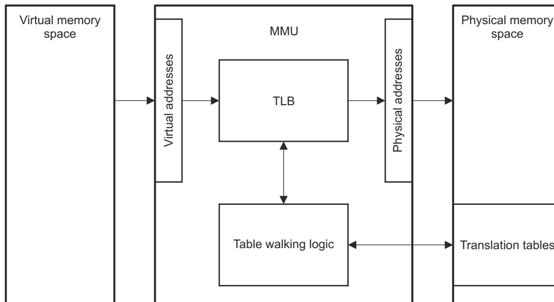
Figure 22-5. MMU Block Diagram
