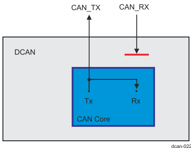
Figure 26-183. CAN Core in Loopback Mode
