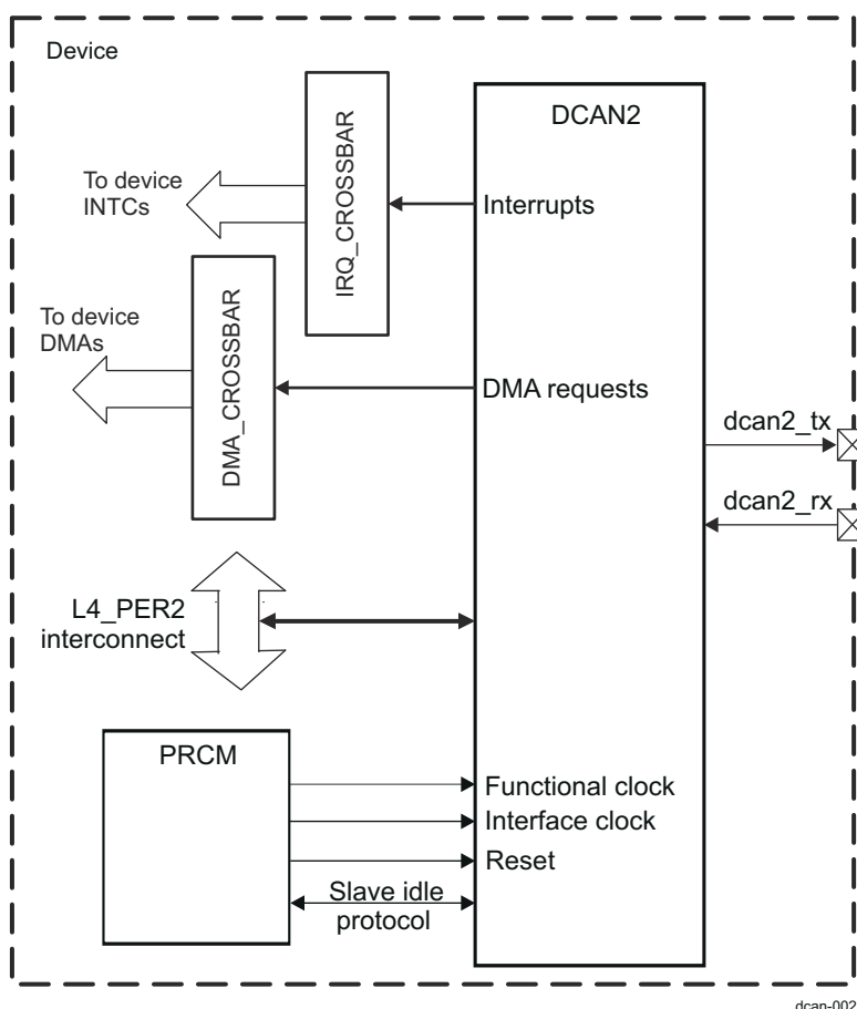
Figure 26-165. DCAN2 Overview
