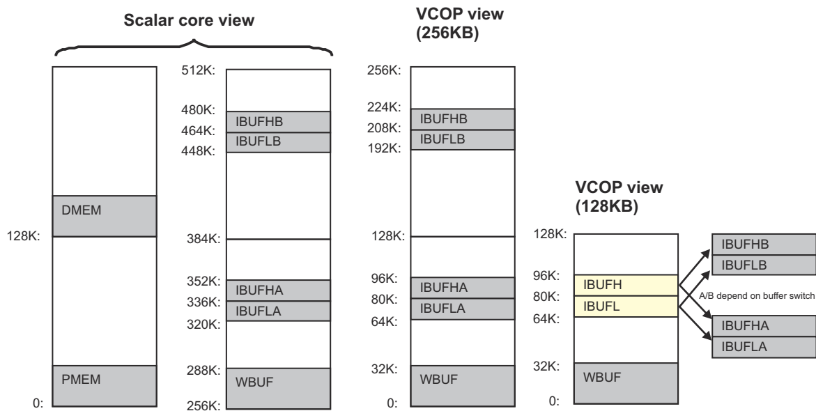
Figure 8-60. EVE Memory Map
