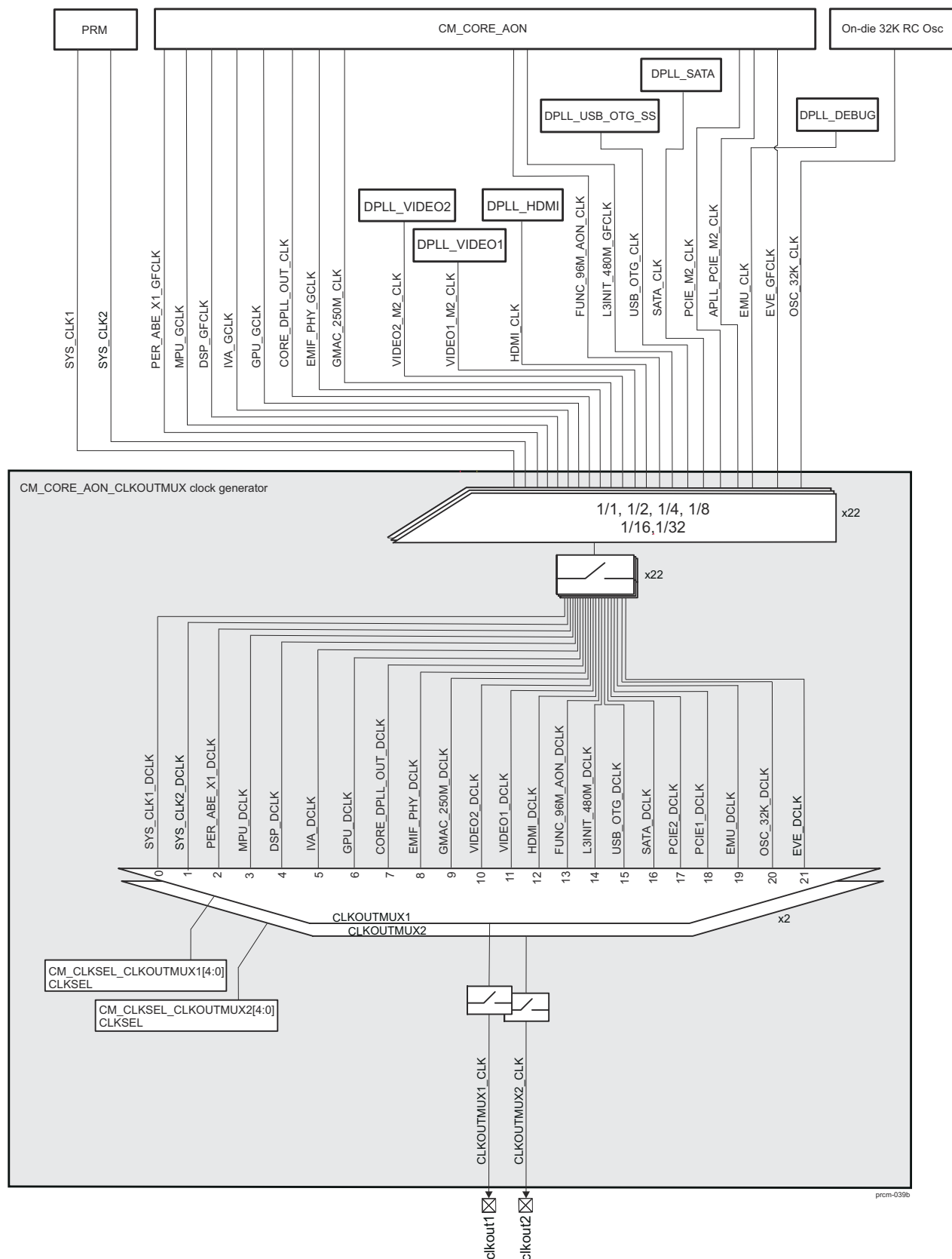
Figure 3-43. CM_CORE_AON_CLKOUTMUX Clock Manager Overview (CLKOUTMUX1 and CLKOUTMUX2)
