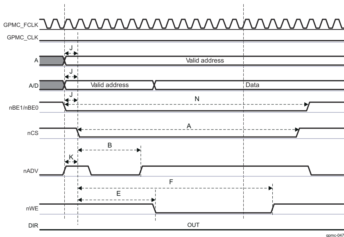
Figure 17-99. Asynchronous NOR Single Write Simplified Example
