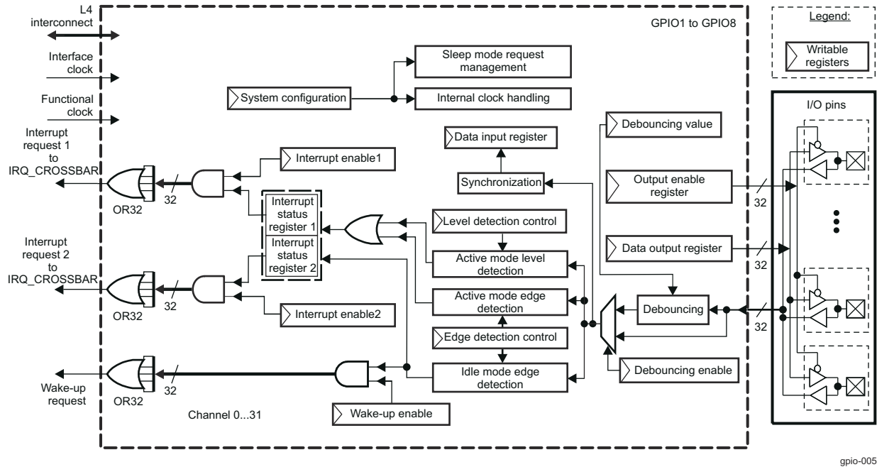
Figure 29-6. General-Purpose Interface Block Diagram
