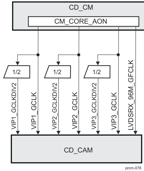
Figure 3-88. CD_CAM Overview
