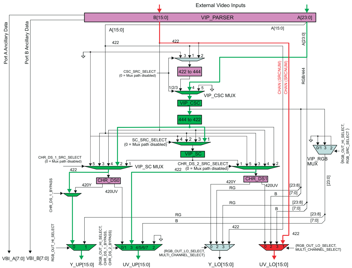
Figure 11-9. Input: A=YUV444, B=YUV422; Output: A=YUV422, A=Scaled YUV422, B=YUV422
