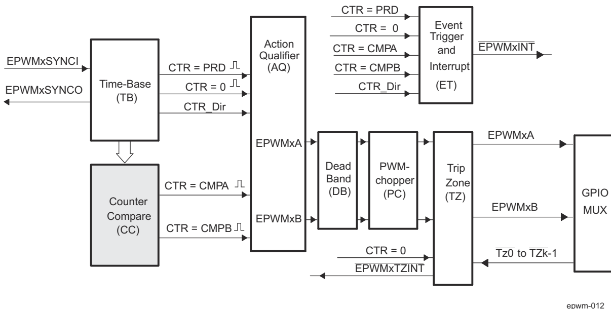
Figure 31-16. ePWM Counter-Compare Submodule
