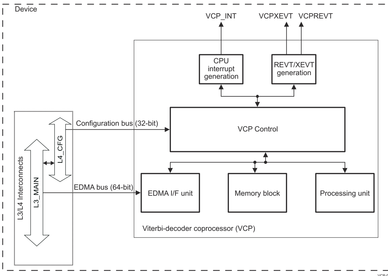
Figure 32-3. VCP Block Diagram
