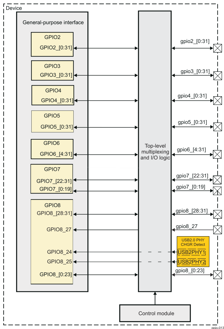
Figure 29-4. GPIO2 Through GPIO8 Signal Connections
