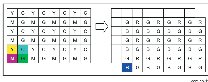
Figure 9-143. ISS ISP ISIF First Pixel/Last Line Generation
