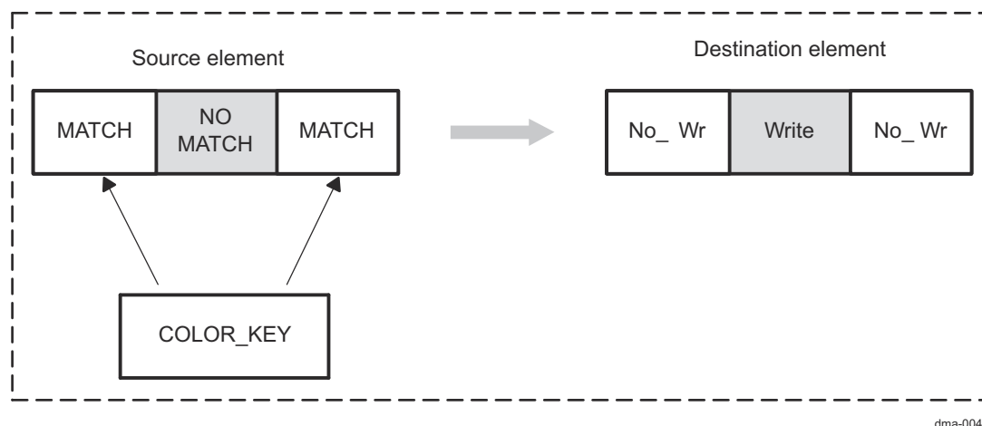
Figure 18-11. 2-D Graphic Transparent Color Block Diagram
