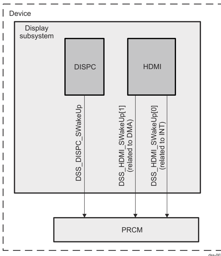
Figure 13-7. Display Subsystem Wake-Up Generation
