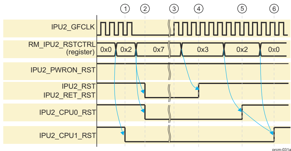
Figure 3-32. IPU2 Subsystem Software Warm Reset Sequence
