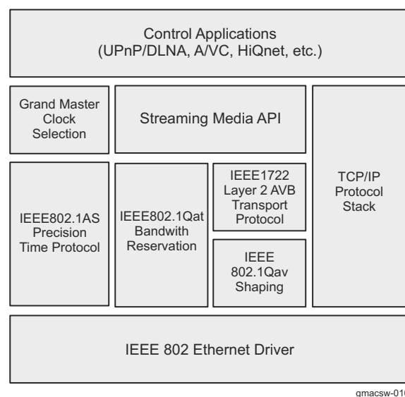
Figure 26-214. The Network Static with AVB
