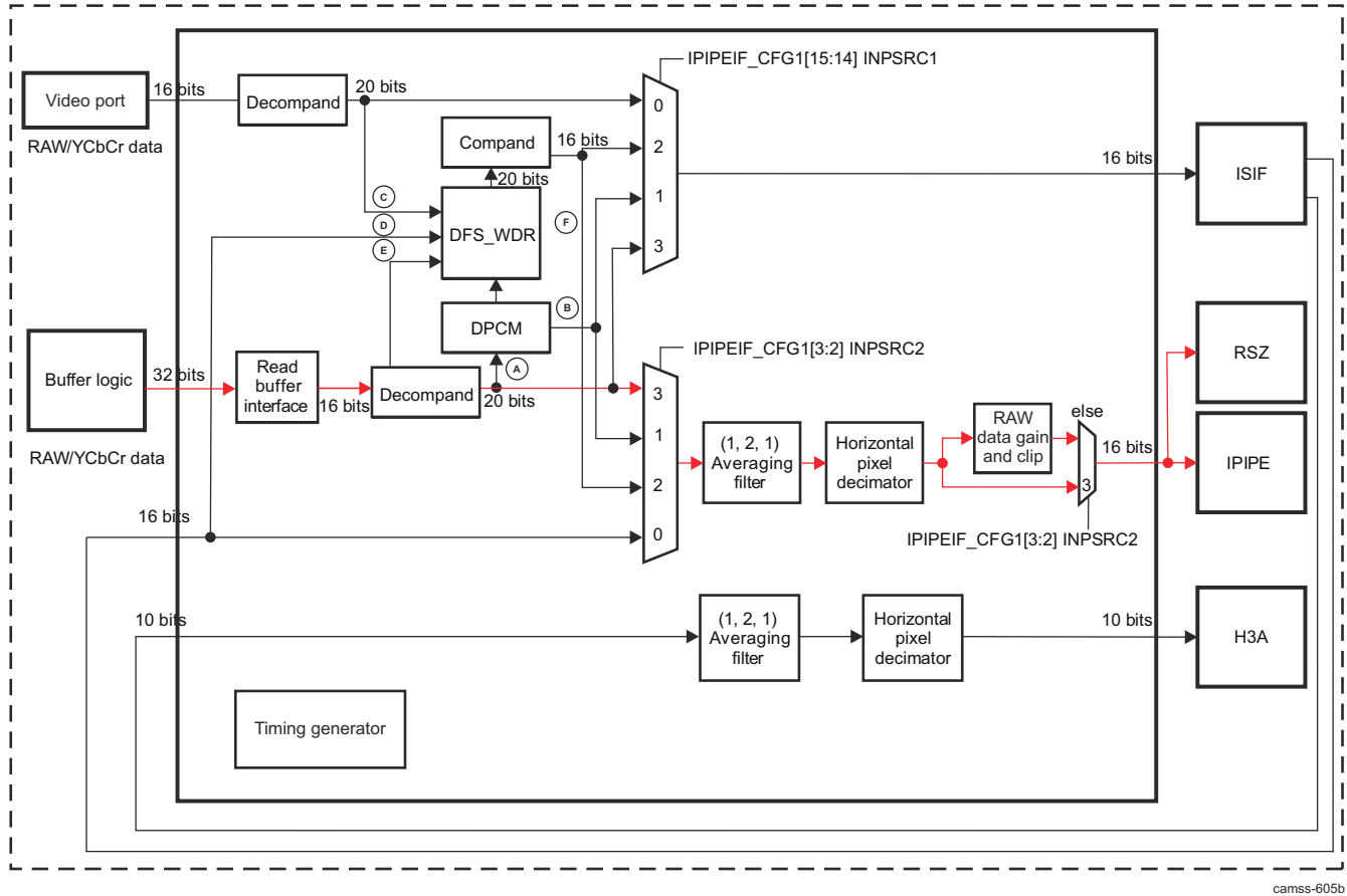
Figure 9-45. ISS ISP IPIPEIF INPSRC1 = 0 and INPSRC2 = 3 Data Paths: Second Case
