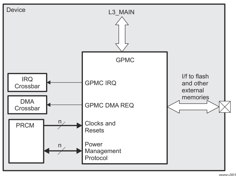
Figure 17-52. GPMC Overview
