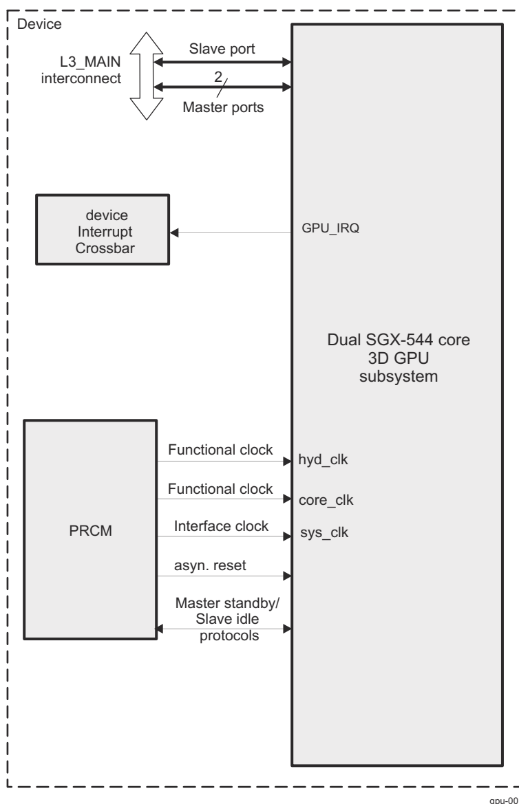
Figure 14-1. GPU Overview
