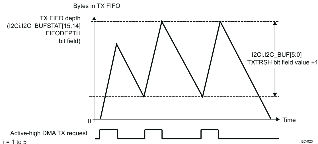
Figure 26-17. HS I 2 C Transmit FIFO Request Generation (High Threshold)
