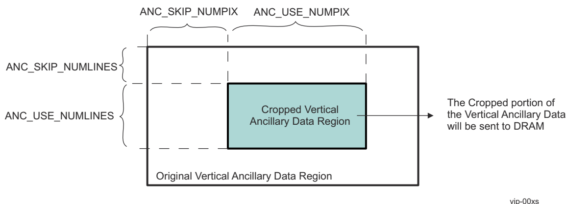
Figure 11-54. Vertical Ancillary Data Cropping
