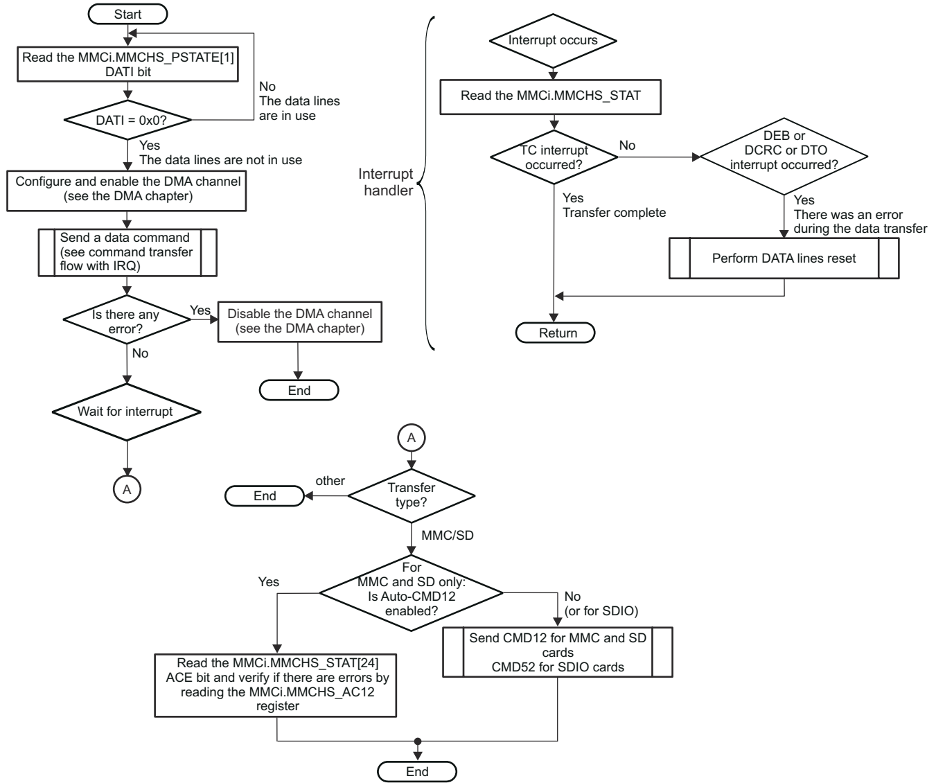
Figure 27-38. eMMC/SD/SDIO Controller Read/Write Transfer Flow in DMA Slave Mode With interrupt
