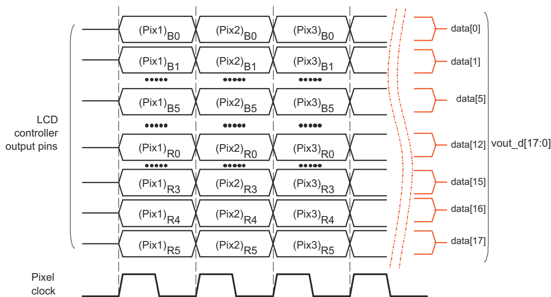
Figure 13-26. DISPC LCD Pixel Data Color18 Active Matrix
