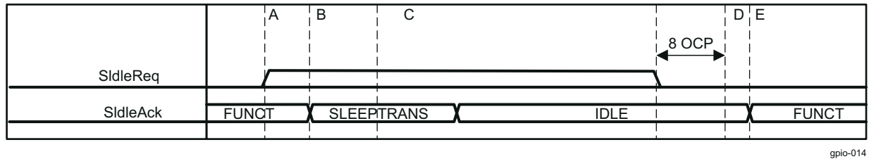
Figure 29-11. Wake-Up Event Conditions
