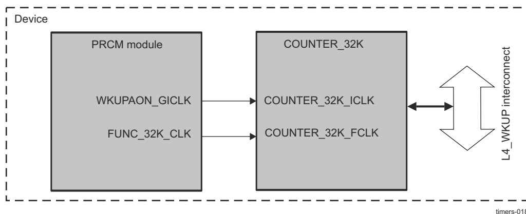
Figure 24-15. 32-kHz Synchronized Timer Block Diagram
