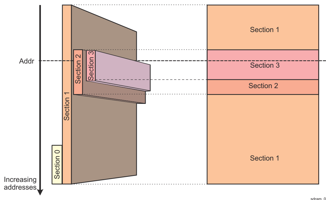
Figure 17-5. DMM Sections and Memory Mapping
