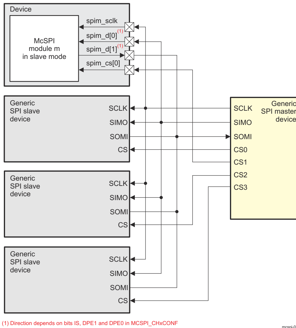
Figure 26-88. Example of McSPI Slave With One Master and Multiple Slave Devices on Channel 0
