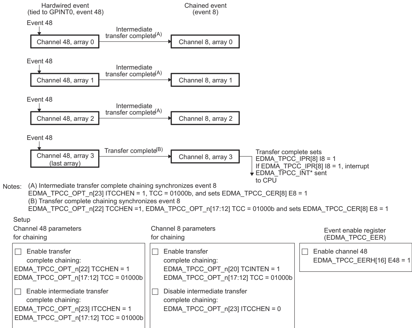
Figure 18-50. Intermediate Transfer Completion Chaining Example
