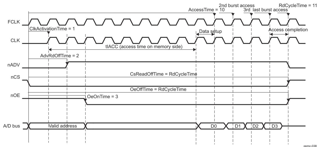
Figure 17-101. Synchronous Burst Read Access (Timing Parameters in Clock Cycles)
