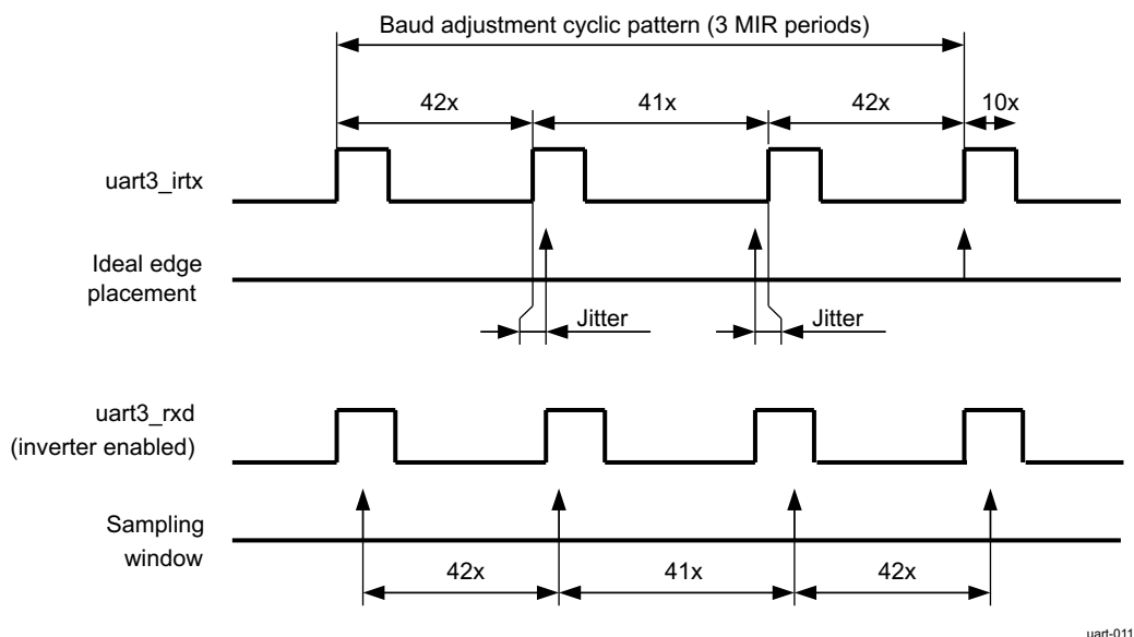
Figure 26-46. MIR Baud Rate Adjustment Mechanism
