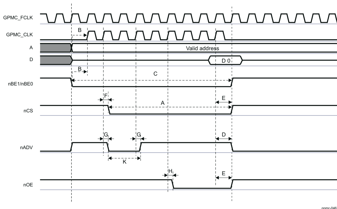
Figure 17-98. Synchronous NOR Single Read Simplified Example
