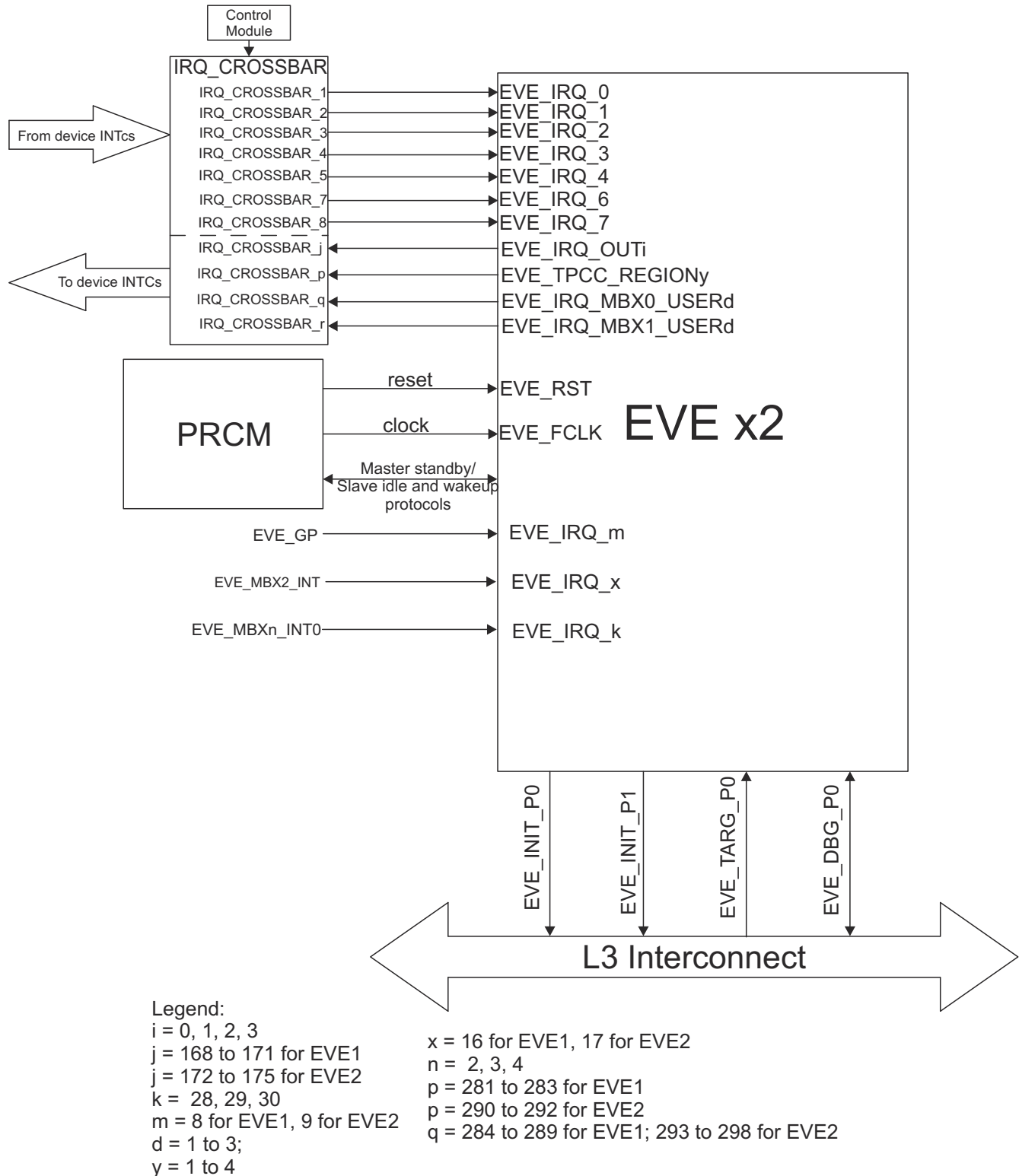
Figure 8-2. EVE Integration
