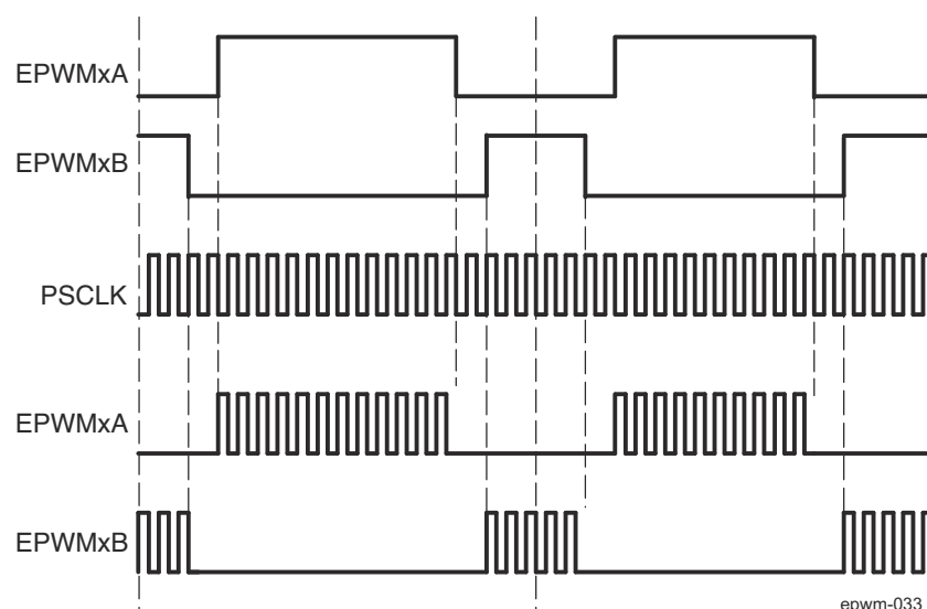
Figure 31-37. Simple PWM-Chopper Submodule Waveforms Showing Chopping Action Only
