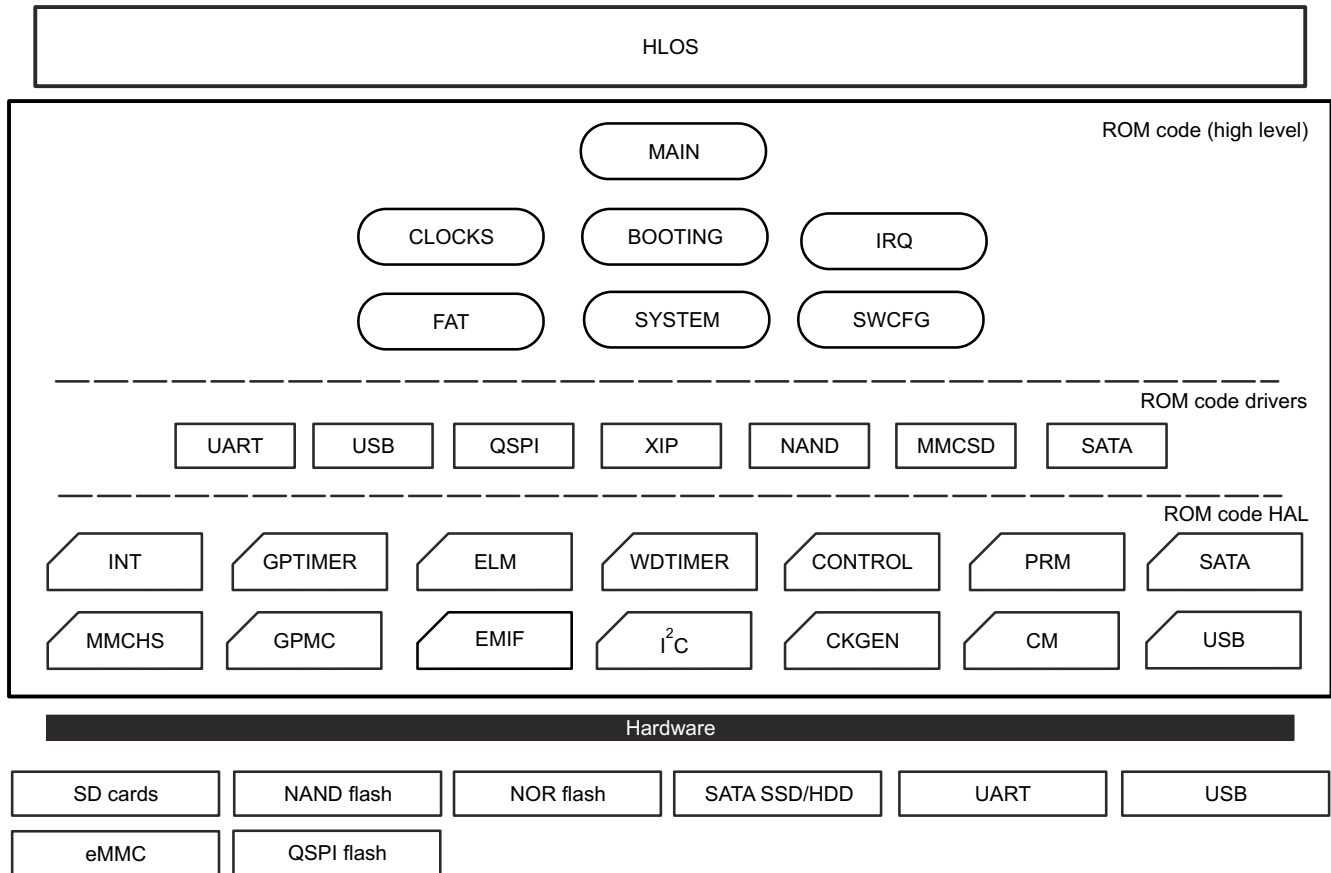
Figure 34-4. ROM Code Architecture
