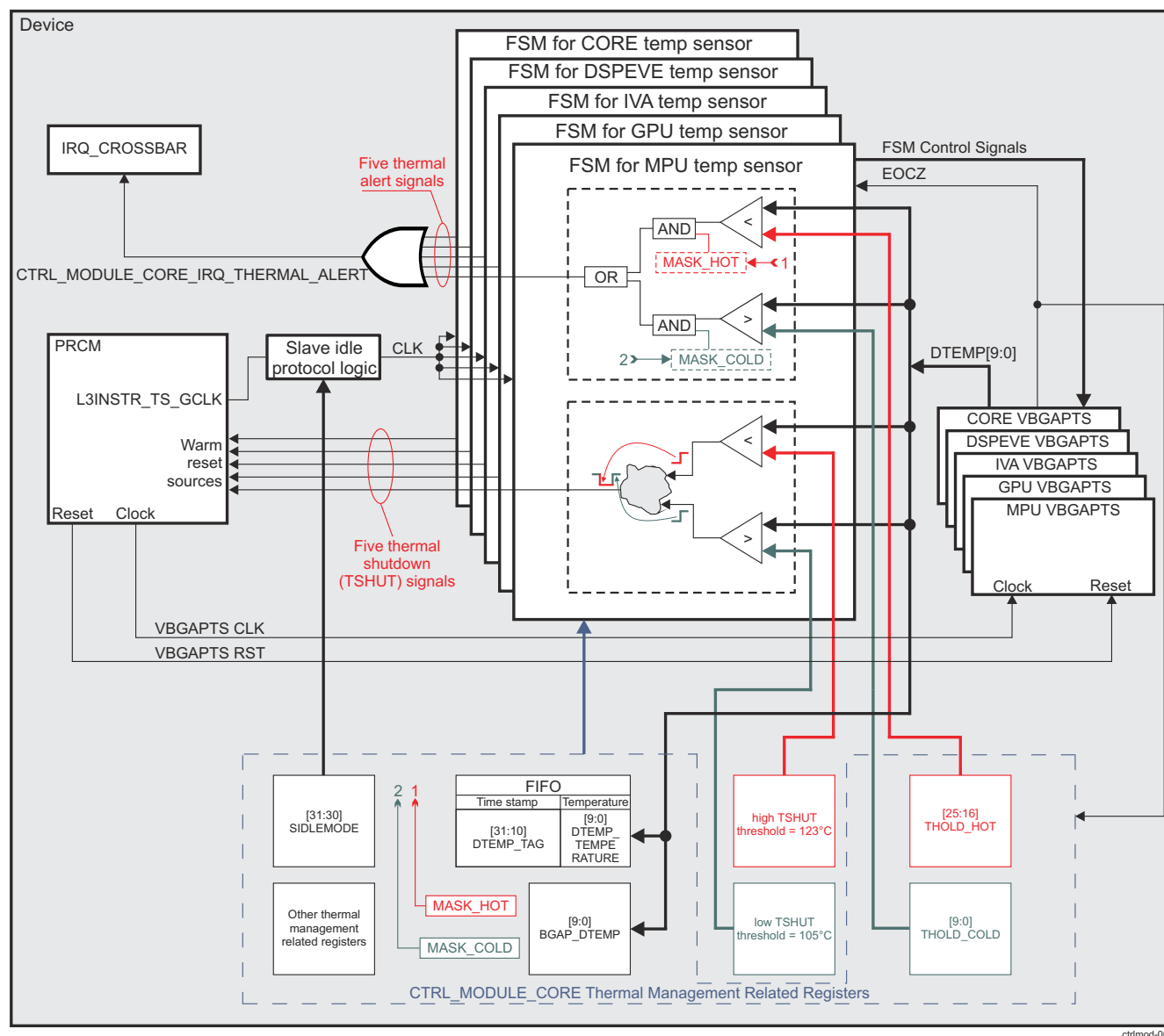
Figure 20-6. Thermal Management Functional Block Diagram
