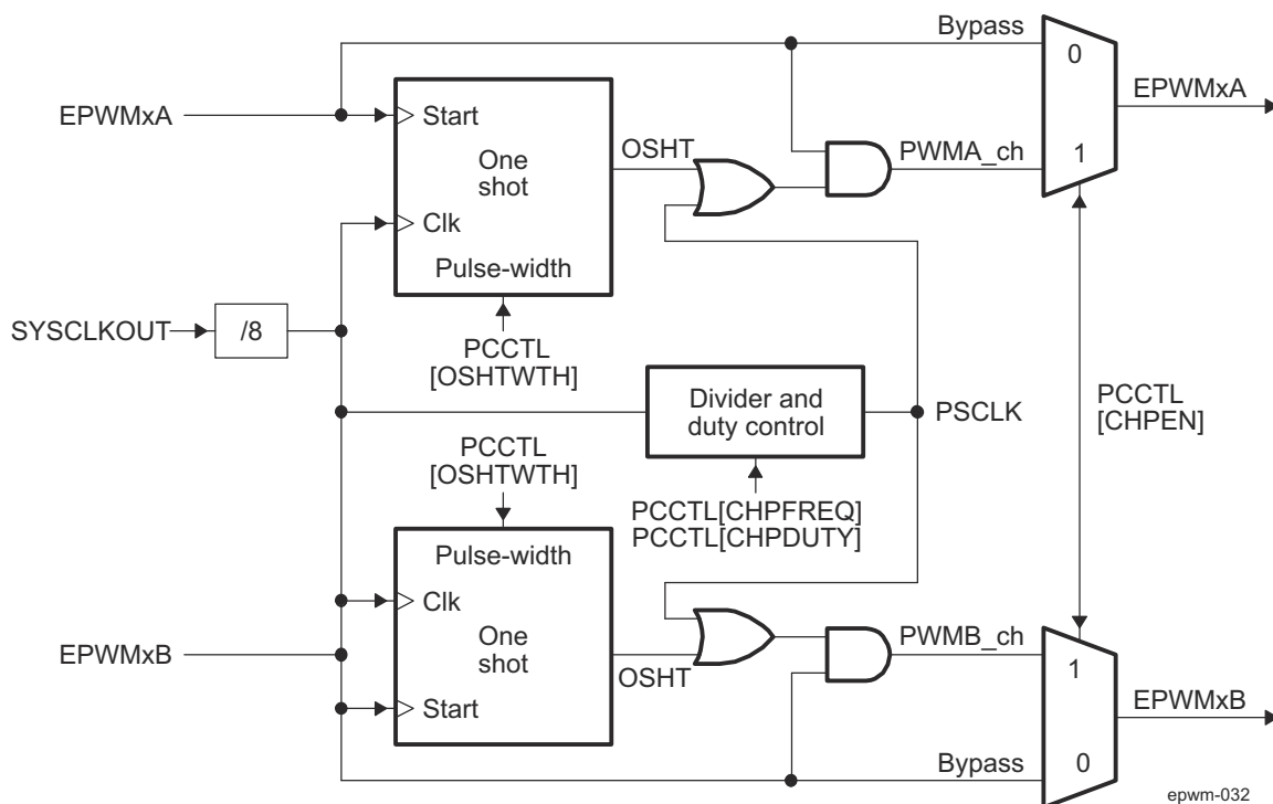
Figure 31-36. PWM-Chopper Submodule Signals and Registers
