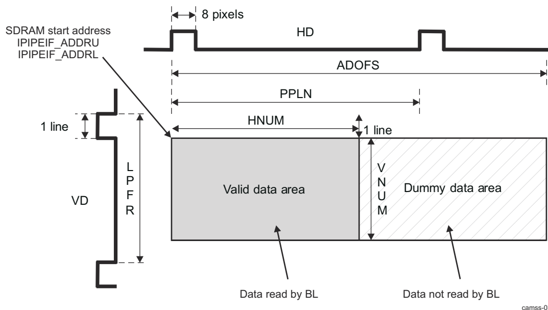
Figure 9-38. ISS ISP IPIPEIF Global Frame Definition in SDRAM Input Modes (Except Dark Frame)
