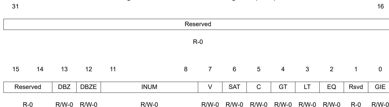
Figure 8-31. Control Status Register (CSR)
