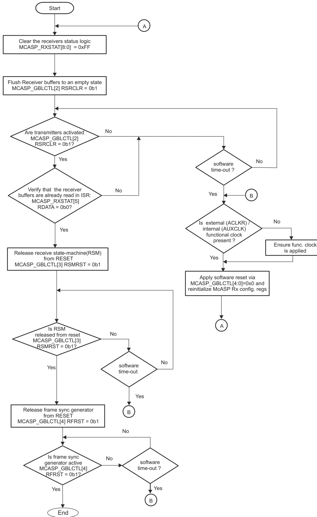
Figure 26-138. Subsequence – TDM - Reception Startup Procedure
