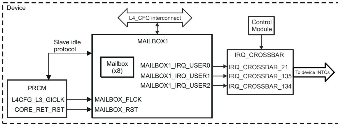
Figure 21-1. MAILBOX1 Integration
