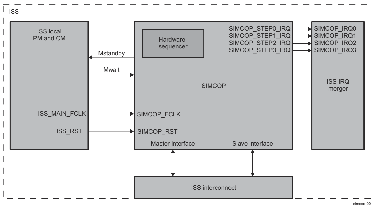
Figure 9-175. SIMCOP Integration
