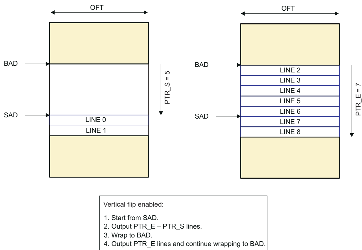
Figure 9-106. ISS ISP RSZ and Circular Buffer Settings – Example 1
