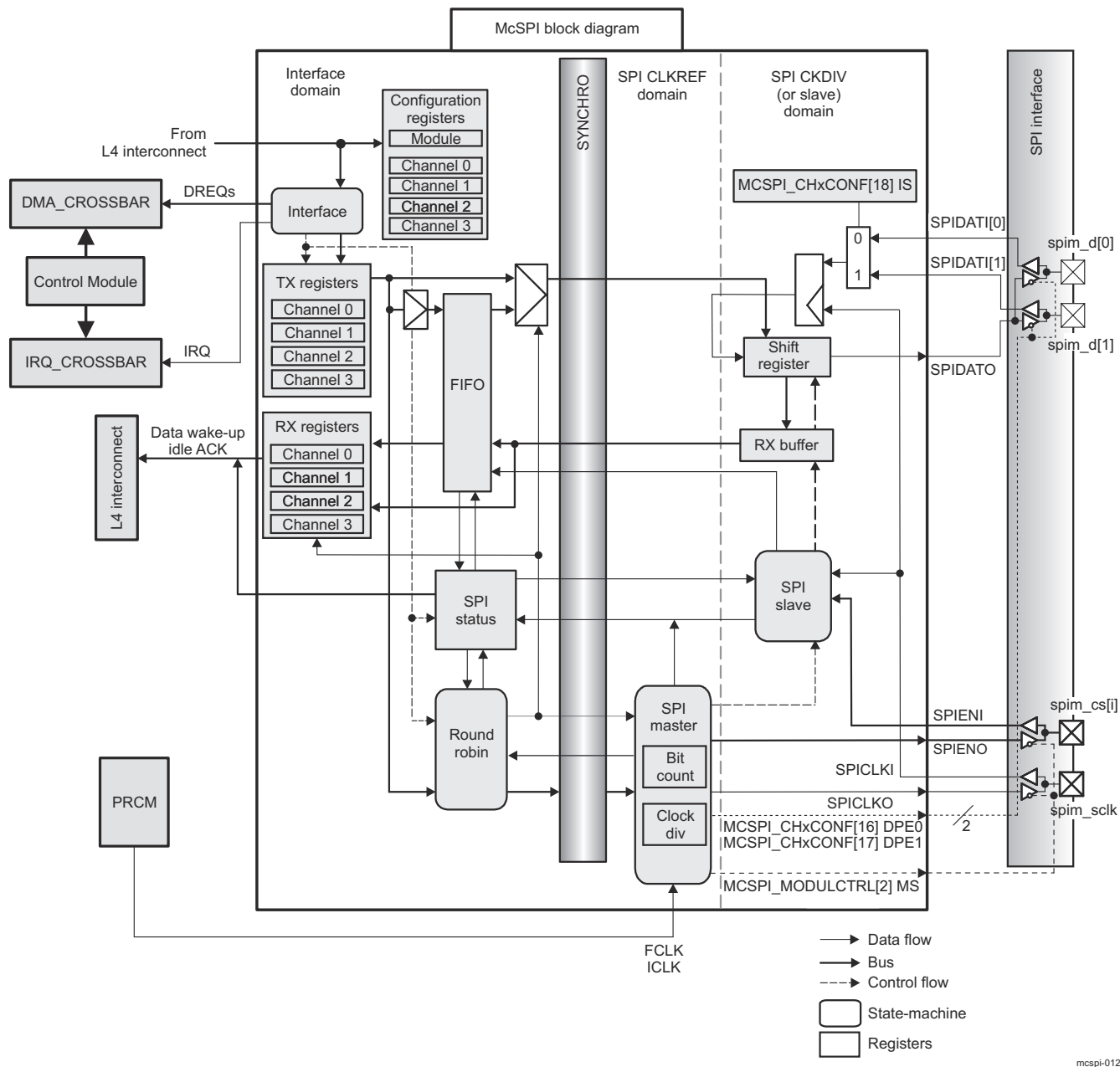
Figure 26-83. McSPI Block Diagram
