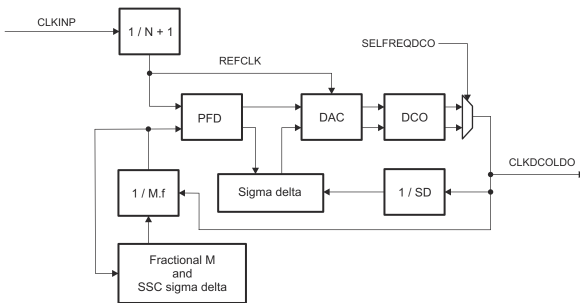
Figure 28-5. DPLL_SATA Functional Block Diagram
