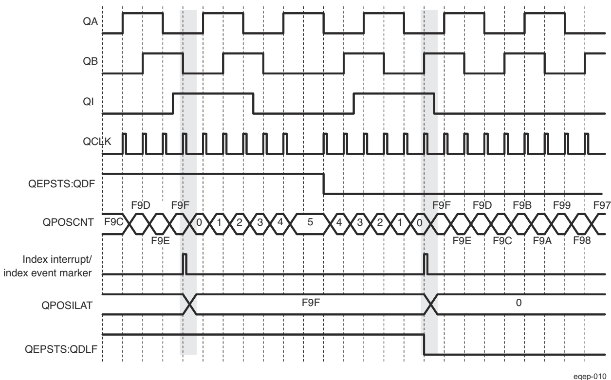
Figure 31-69. Position Counter Reset by Index Pulse for 1000 Line Encoder (QPOS MAX = 3999 or F9Fh)
