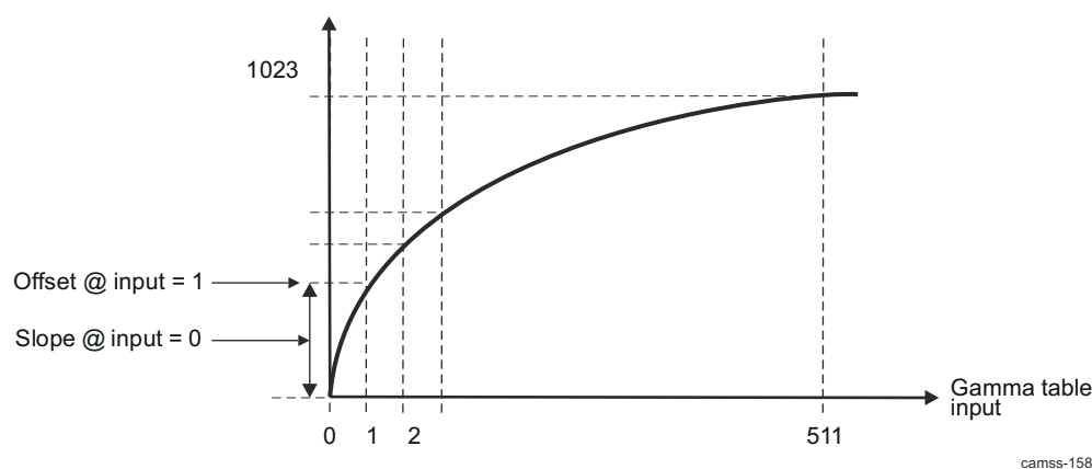
Figure 9-71. ISS ISP IPIPE Gamma Curve Example
