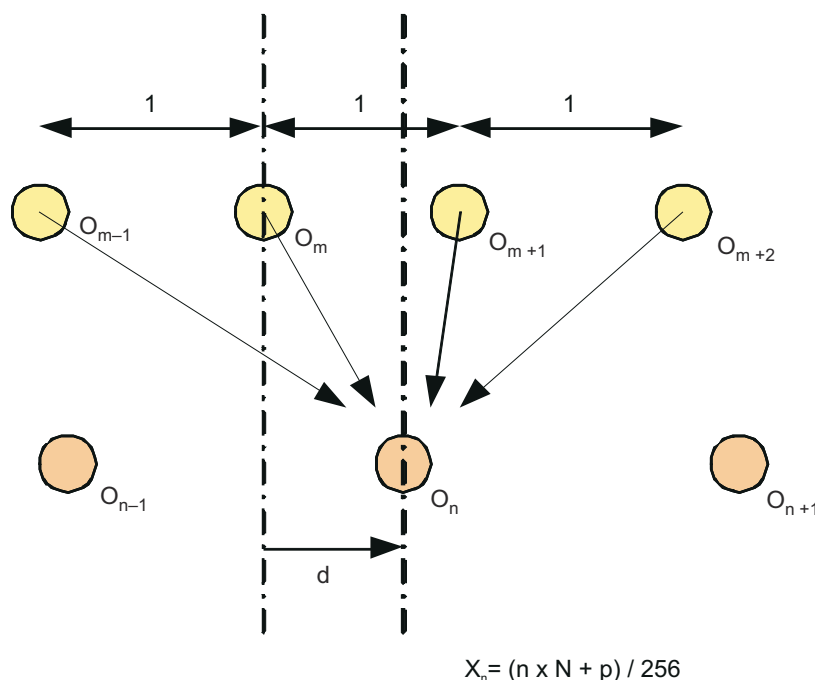
Figure 9-102. ISS ISP RSZ Interpolation Filtering
