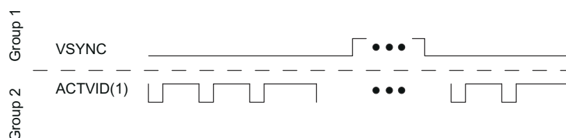
Figure 11-64. VSYNC and ACTIVID(1)
