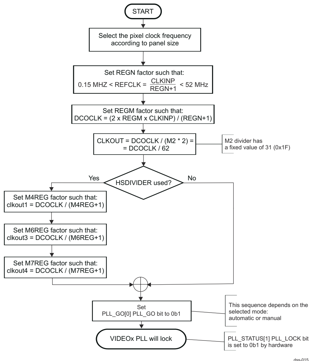
Figure 13-13. VIDEO PLL Programming Sequence
