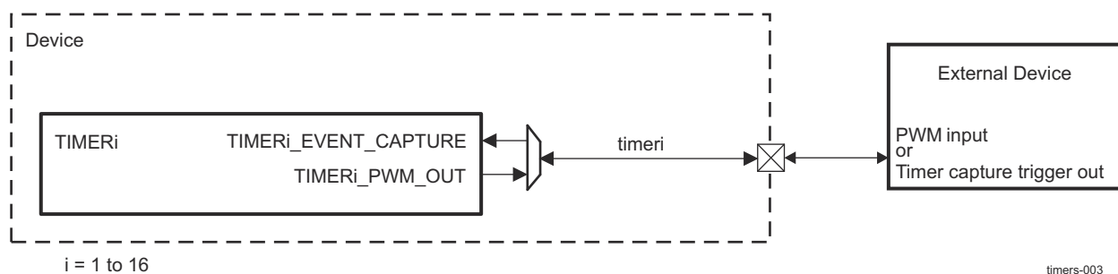
Figure 24-3. GP Timers External System Interface
