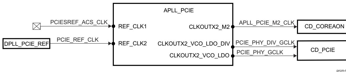
Figure 3-64. APLL_PCIE Overview
