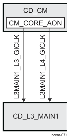
Figure 3-81. CD_L3_MAIN1 Overview
