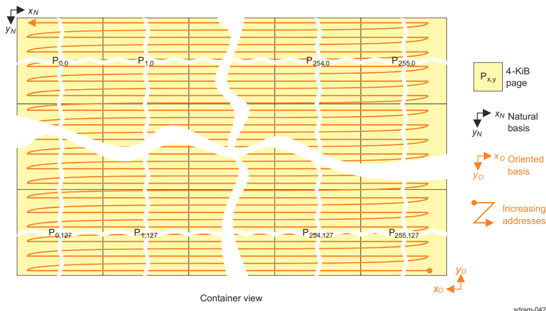
Figure 17-27. Tiled Mode Ordering of Elements in 180-Degree View
