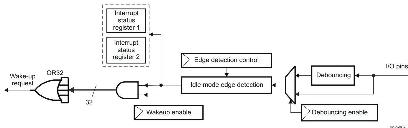
Figure 29-8. Asynchronous Path
