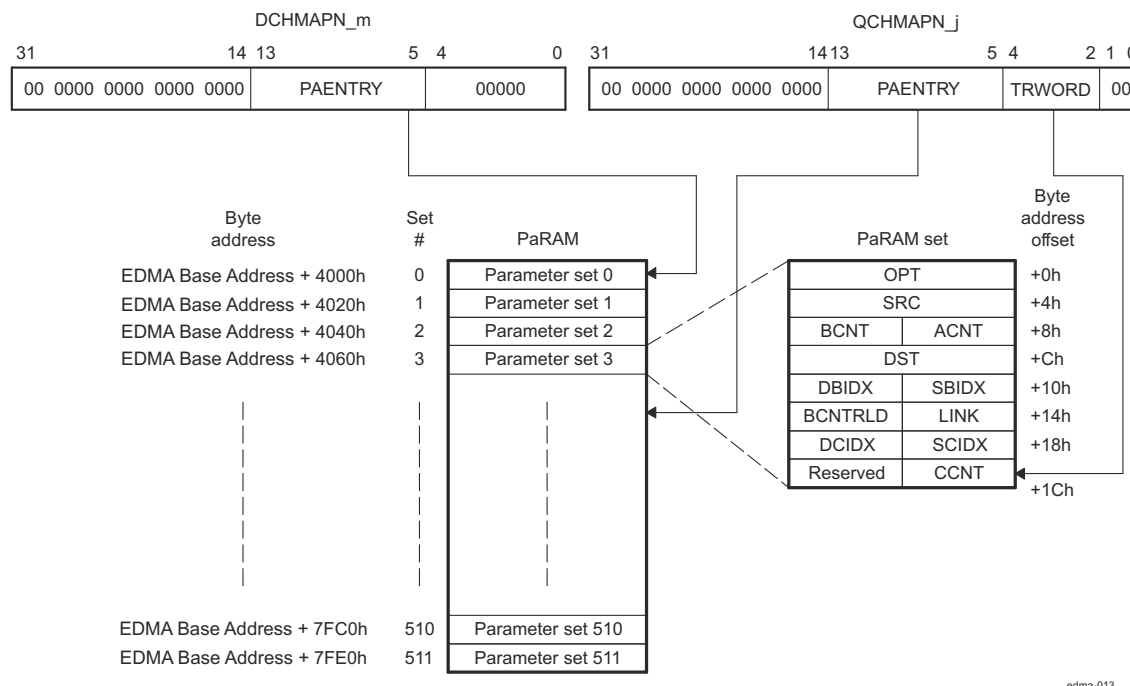
Figure 18-24. DMA Channel and QDMA Channel to PaRAM Mapping
