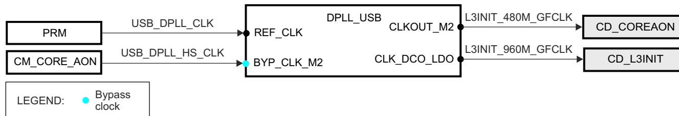
Figure 3-57. DPLL_USB Overview
