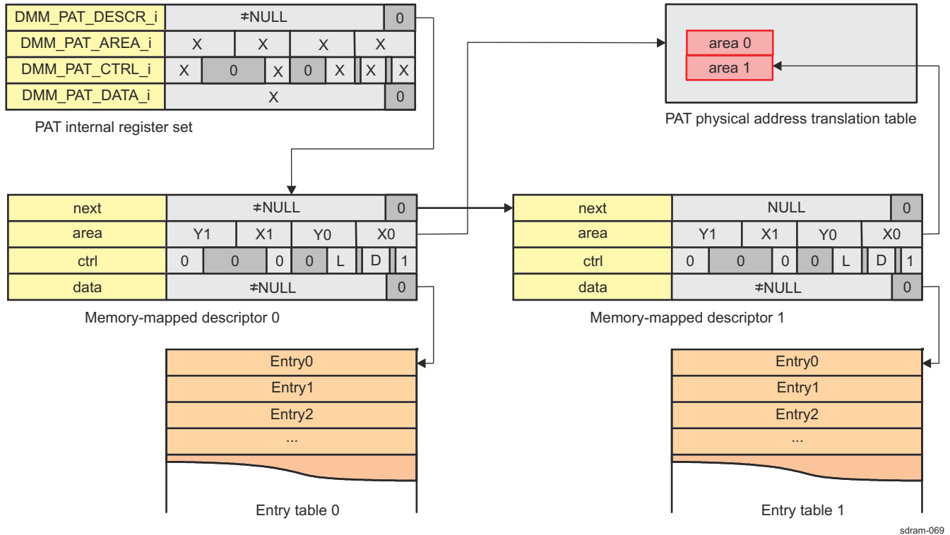
Figure 17-41. Chained Auto-Configured Area Refill Scheme
