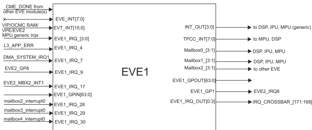
Figure 8-3. EVE1 Signals
