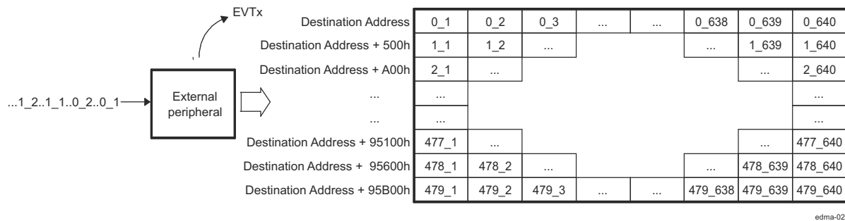
Figure 18-41. Servicing Peripheral Burst Example
