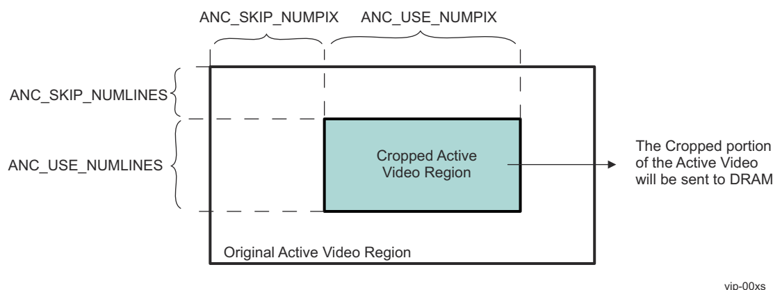
Figure 11-55. Active Video Cropping
