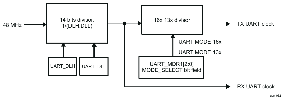
Figure 26-69. Baud Rate Generation
