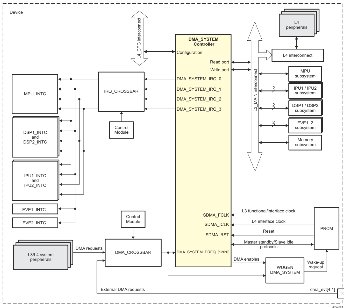
Figure 18-1. DMA_SYSTEM Overview
