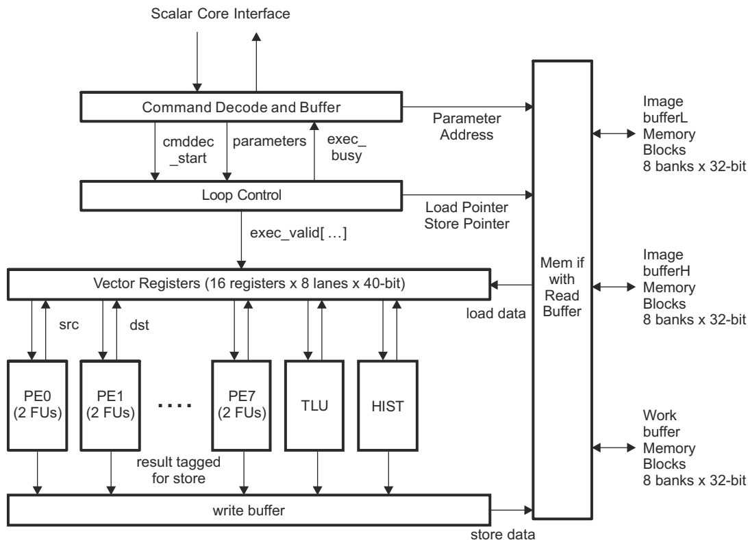
Figure 8-59. VCOP Block Diagram
