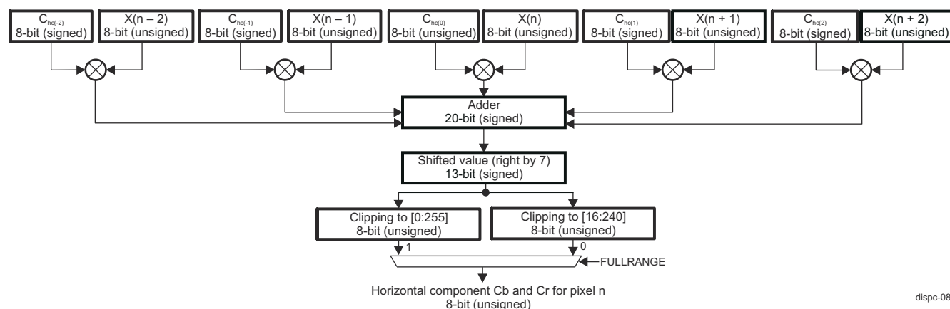
Figure 13-72. DISPC Macro-Architecture of the Horizontal Scaling for Cr and Cb Components
