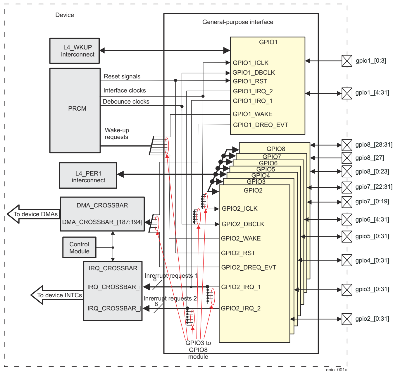
Figure 29-1. General-Purpose Interface Overview
