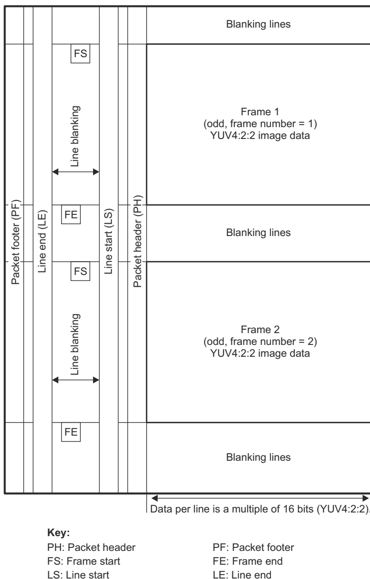
Figure 10-21. CSI2 Digital Interlaced Video Frame (Informative)
