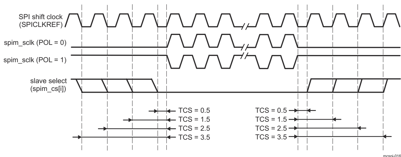
Figure 26-87. CS (SPIEN) Timing Controls
