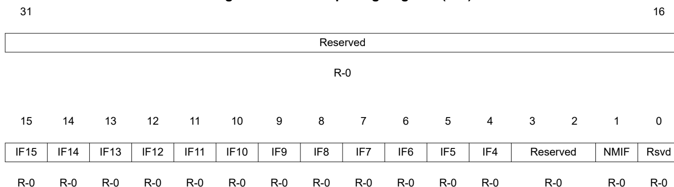
Figure 8-33. Interrupt Flag Register (IFR)
