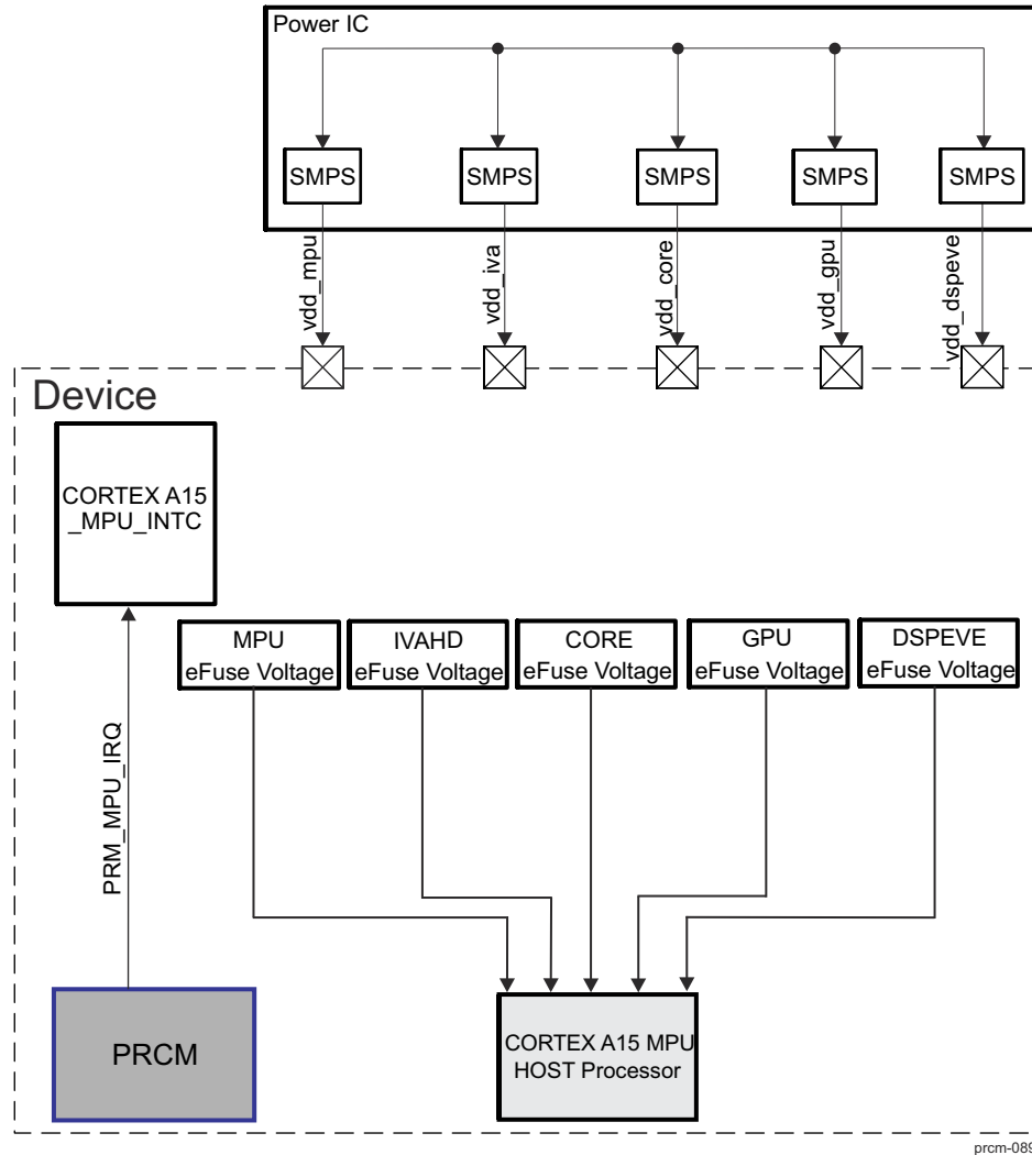
Figure 3-97. SmartReflex Integration
