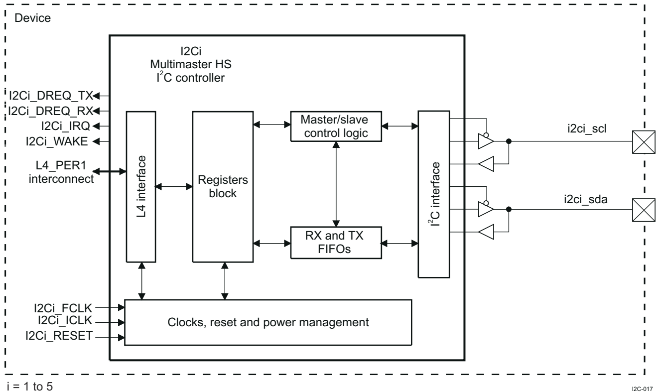
Figure 26-12. HS I 2 C Block Diagram
