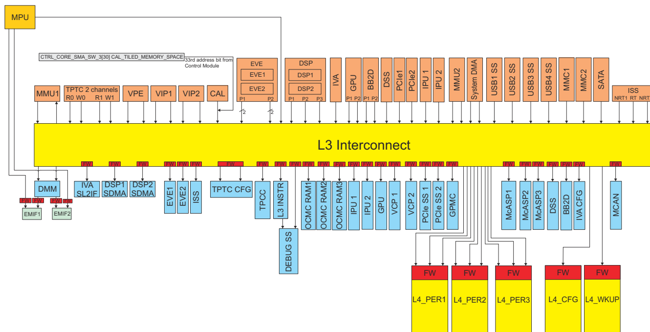
Figure 16-1. Interconnect Overview
