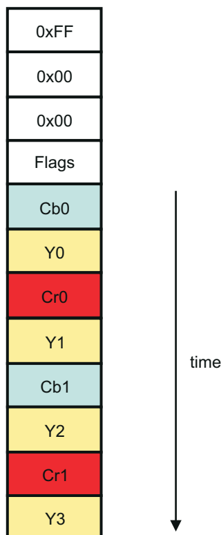
Figure 11-44. Code Word Format Example Followed by Video Data
