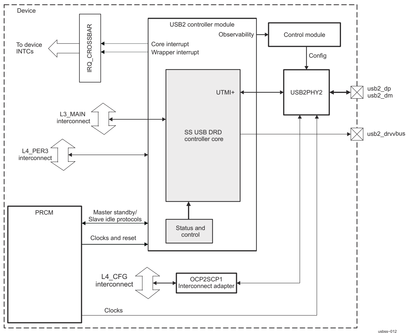
Figure 26-144. USB2 Highlight
