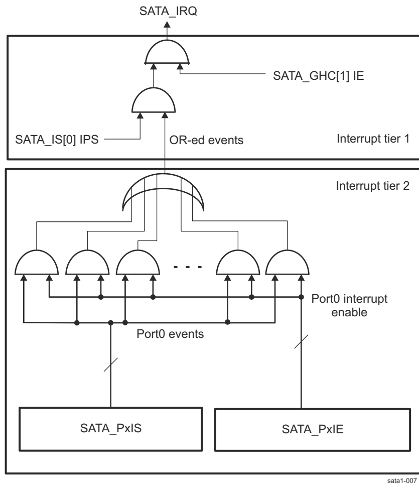
Figure 26-157. SATA Controller Interrupt Propagation Schema
