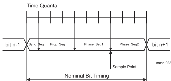
Figure 26-190. CAN Bit Timing
