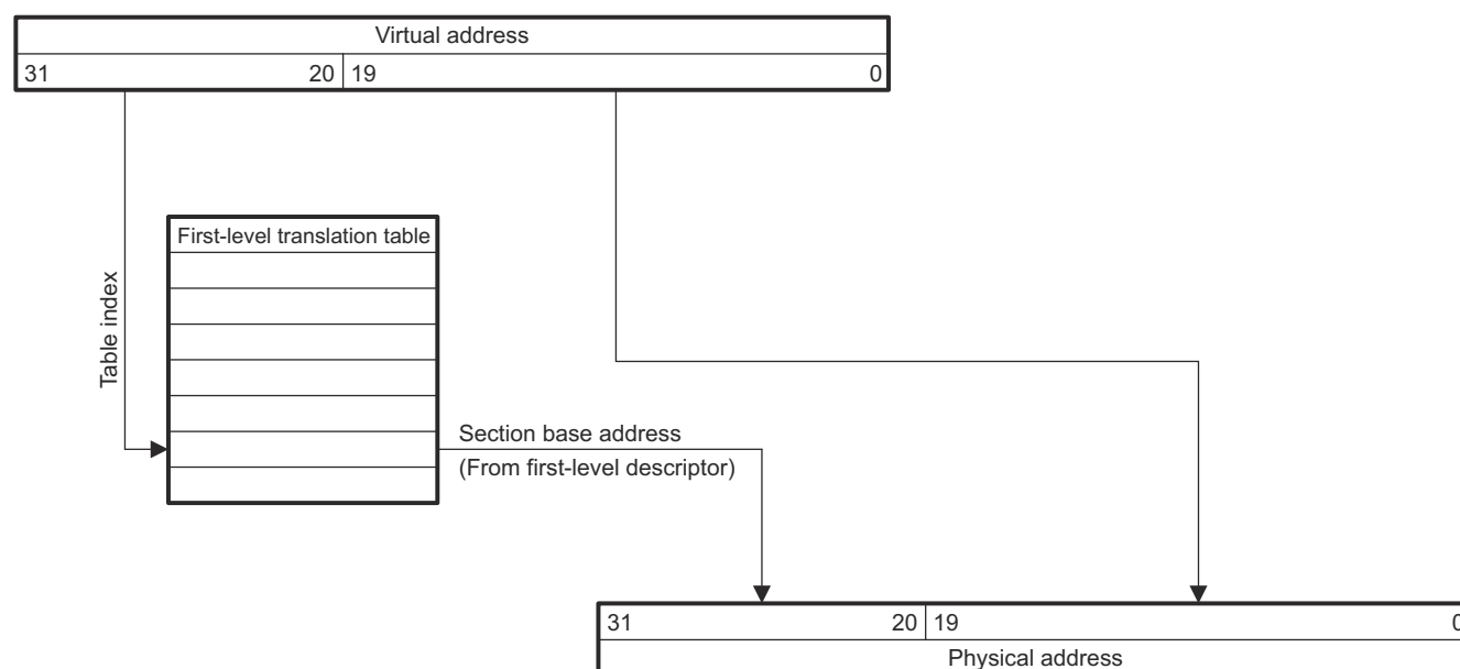
Figure 22-10. Section Translation Summary
