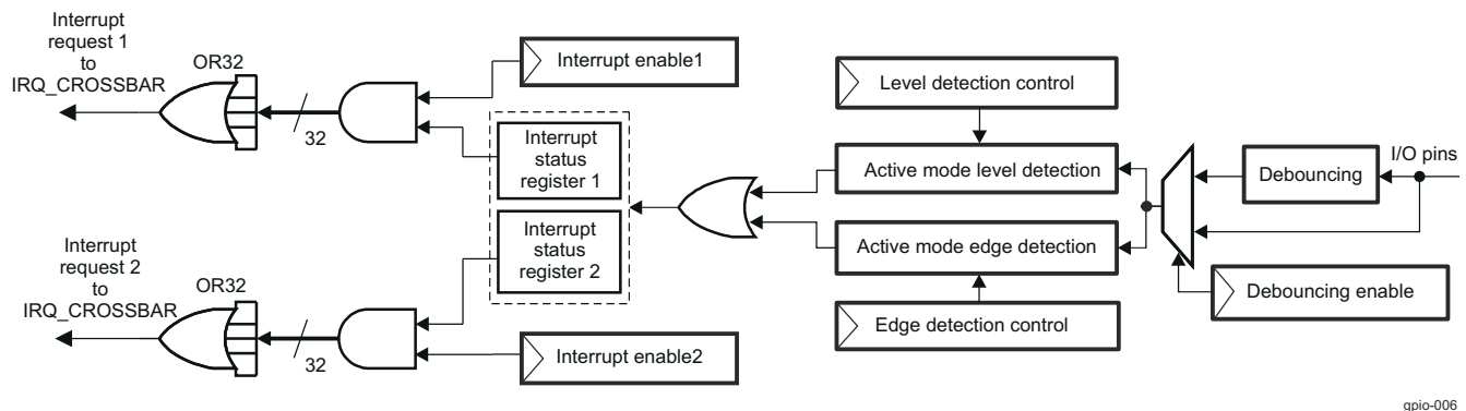
Figure 29-7. Synchronous Path
