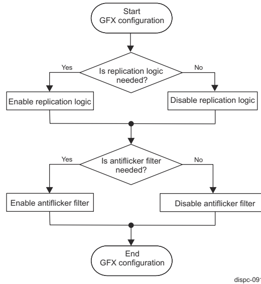
Figure 13-100. DISPC GFX Pipeline Processing Configuration
