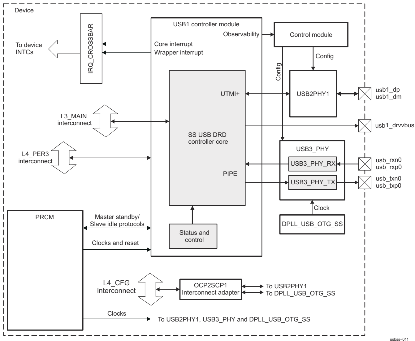
Figure 26-143. USB1 Highlight
