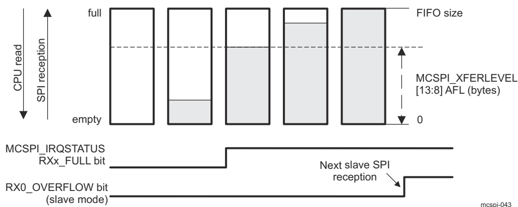
Figure 26-94. Buffer Almost Full Level (AFL)
