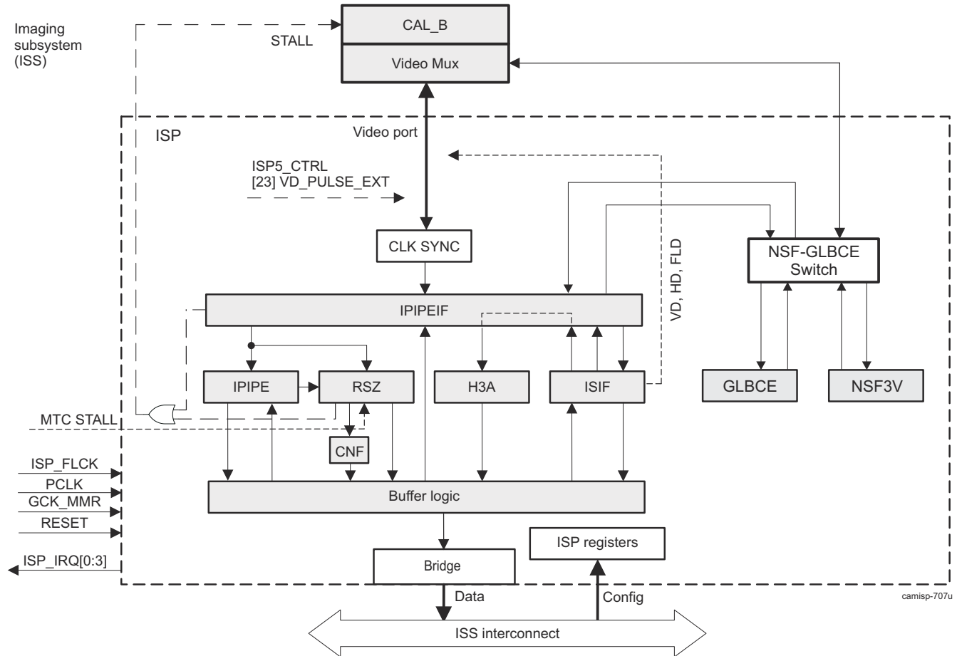
Figure 9-28. ISS ISP High-Level Diagram
