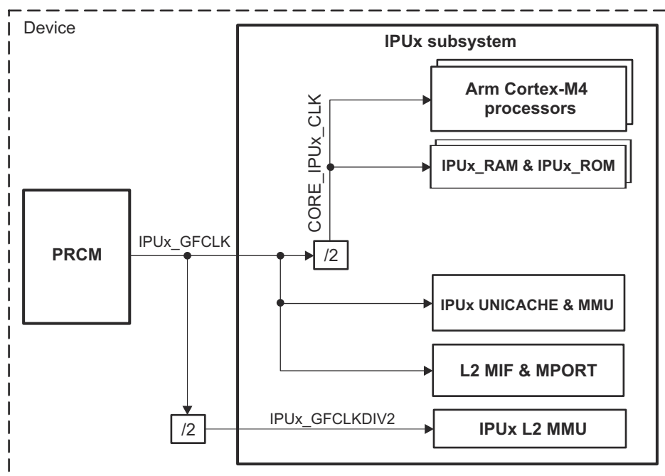
Figure 7-4. IPUx Subsystem Clocking Scheme
