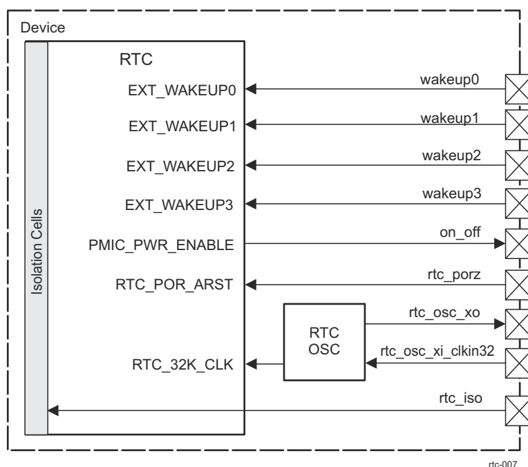
Figure 25-2. RTC External Signals
