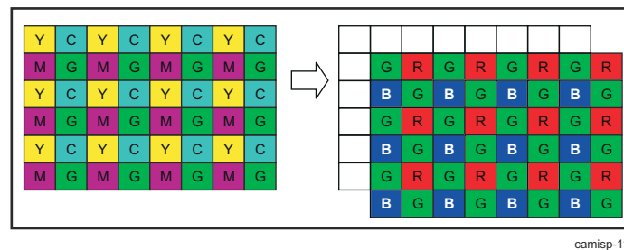
Figure 9-138. ISS ISP ISIF Color Space Conversion Example
