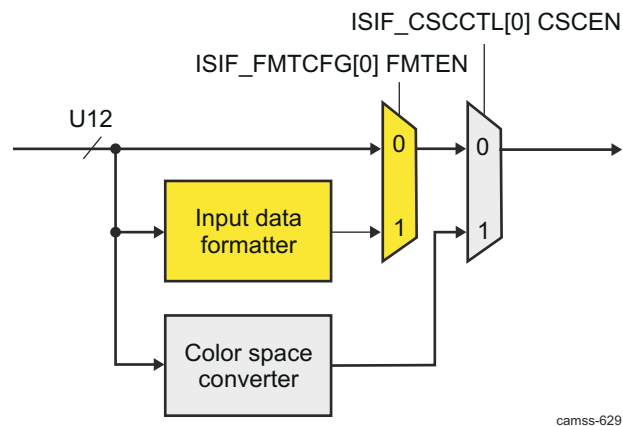
Figure 9-135. ISS ISP ISIF Color Space Converter Block Diagram
