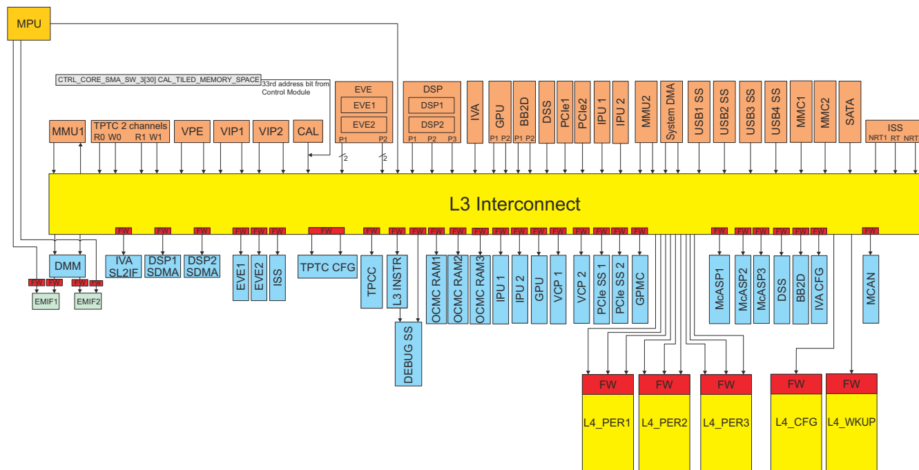
Figure 16-2. L3_MAIN Interconnect Overview
