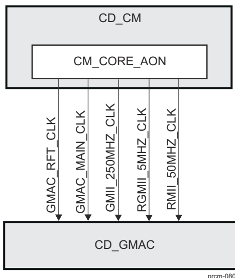
Figure 3-89. CD_GMAC Overview
