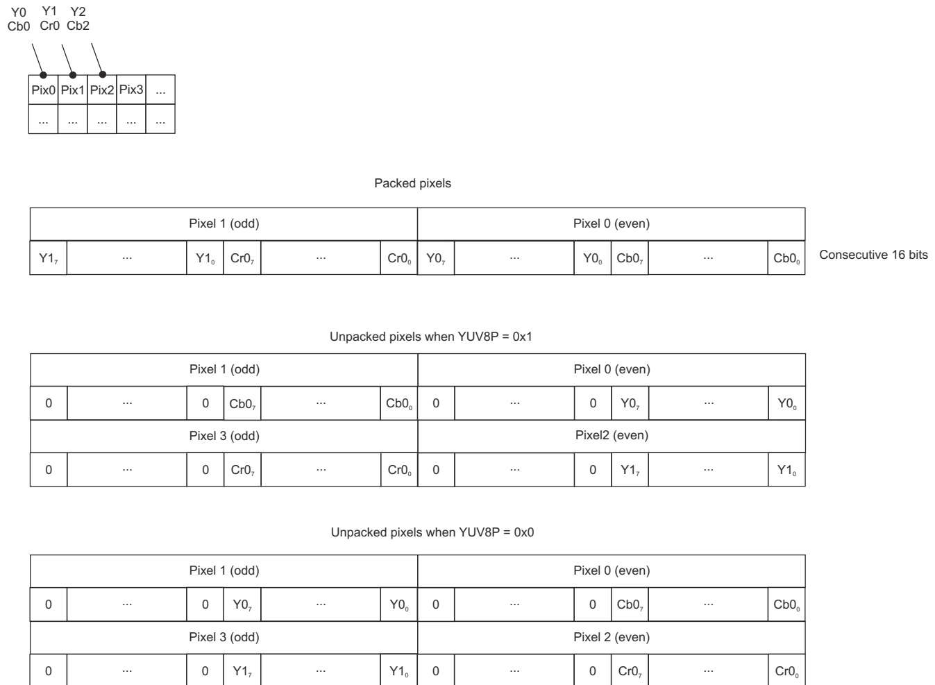
Figure 9-54. ISS ISP IPIPEIF YUV8P Settings
