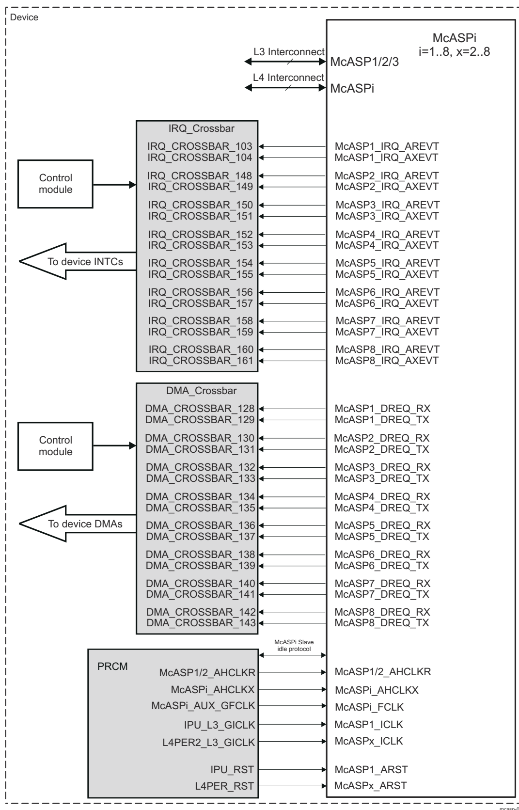
Figure 26-118. McASP Integration
