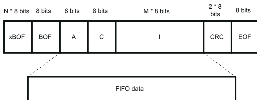
Figure 26-41. IrDA SIR Frame Format
