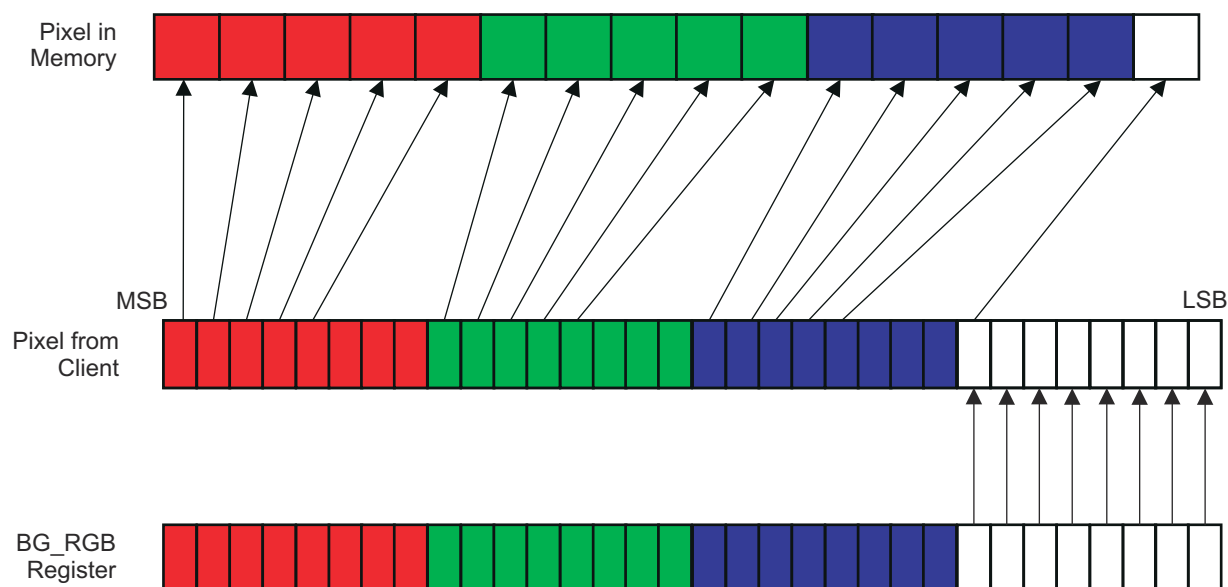
Figure 11-109. RGBA-5551 (Data Type 3)
