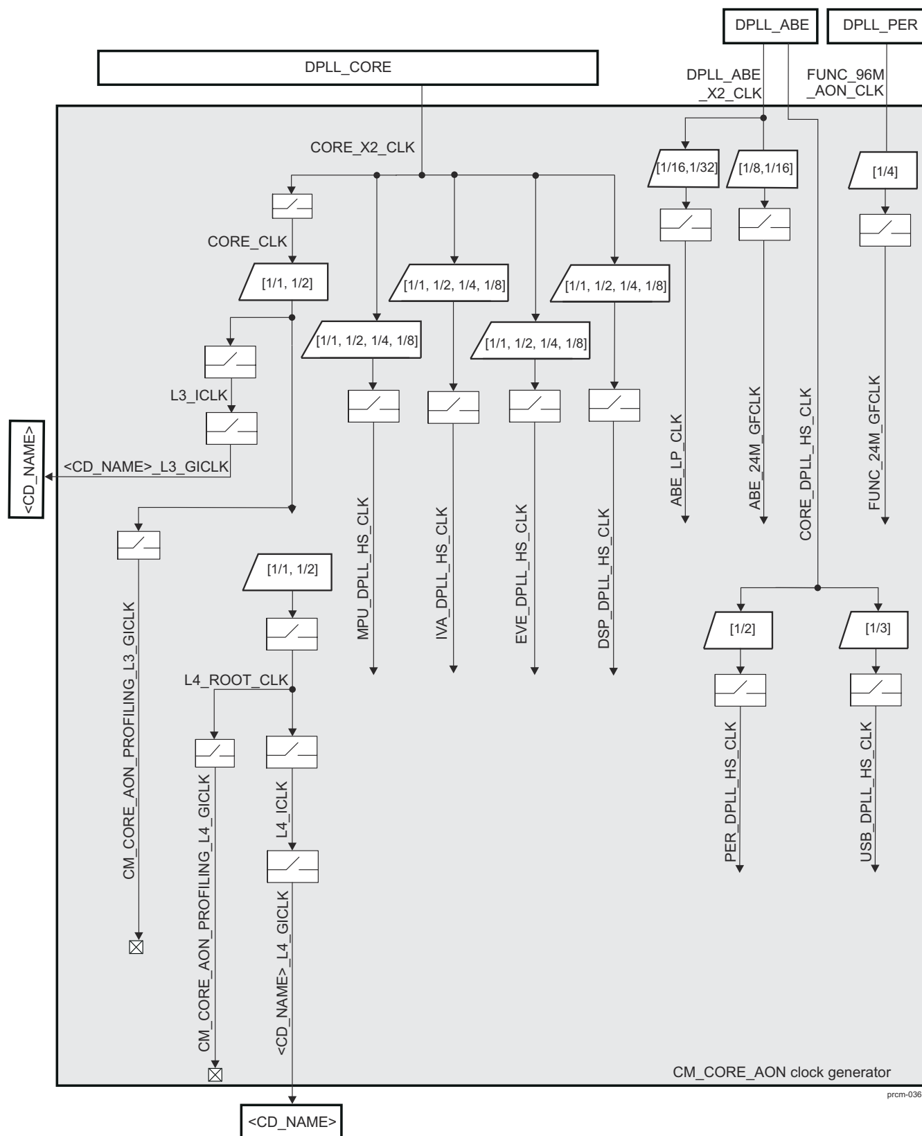
Figure 3-40. CM_CORE_AON Overview (a)
