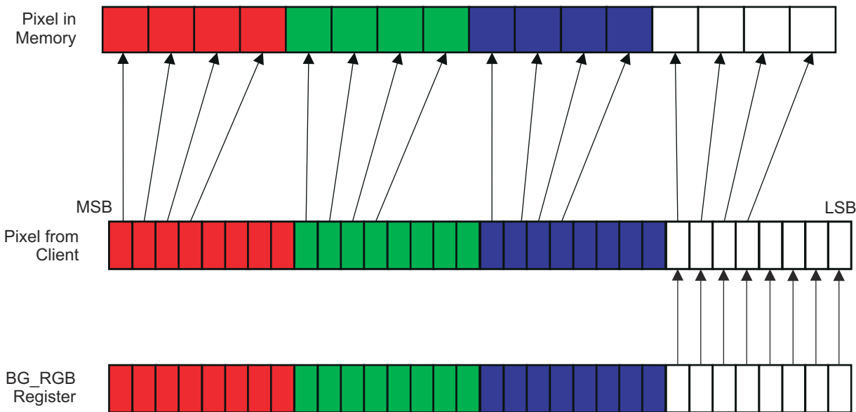
Figure 12-64. RGBA-4444 (Data Type 4)
