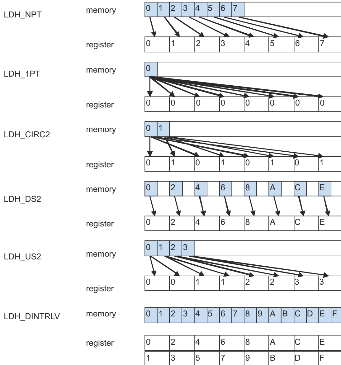
Figure 8-64. Load halfword Distribution Options
