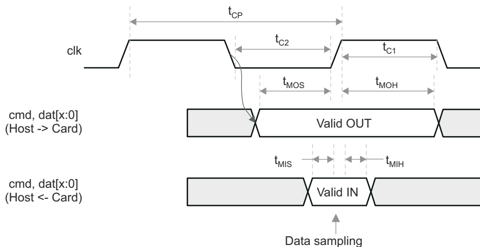
Figure 27-30. Output Driven on Falling Edge
