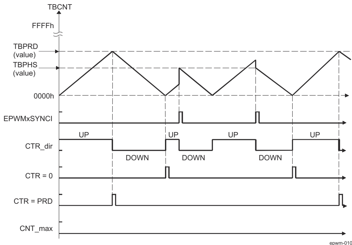
Figure 31-14. ePWM Time-Base Up-Down-Count Waveforms, EPWM_TBCTL[13] PHSDIR = 0 Count Down on
