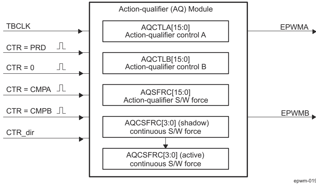
Figure 31-23. ePWM Action-Qualifier Submodule Inputs and Outputs
