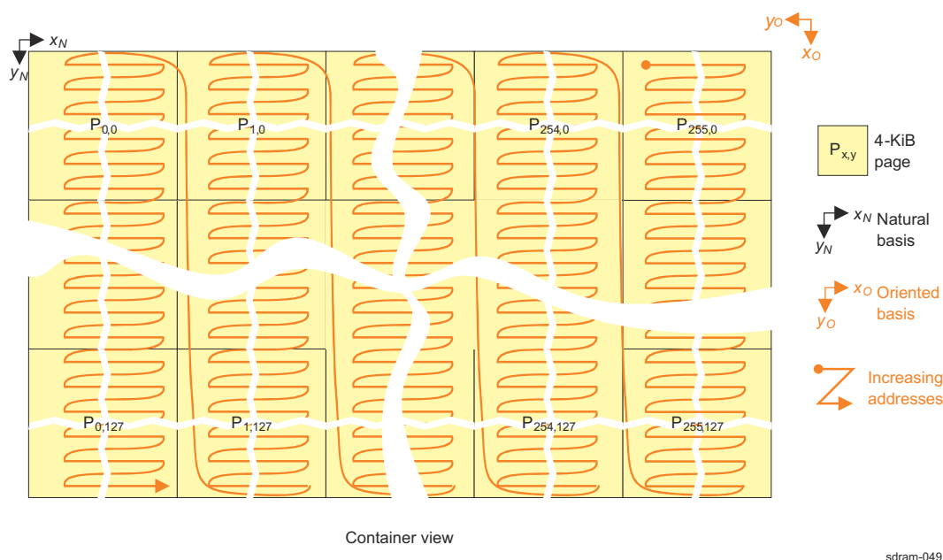
Figure 17-32. Page Mode Ordering of Elements in 270-Degree View
