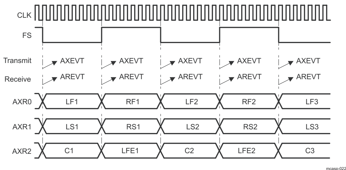
Figure 26-130. DMA Transmit and Receive Event in an Audio Example – One Event
