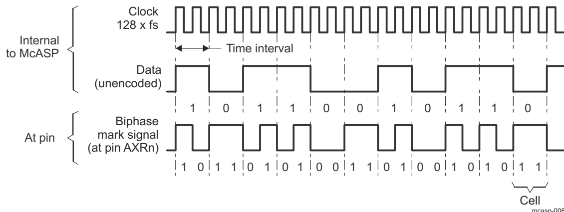
Figure 26-115. Biphase-Mark Code
