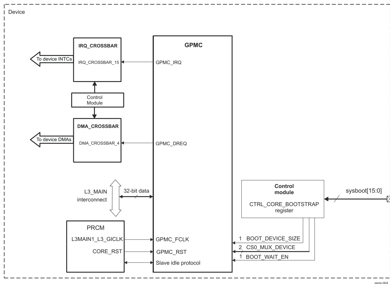
Figure 17-57. GPMC Integration
