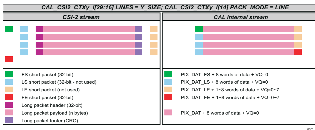
Figure 10-23. CSI-2 Packing – Example 1
