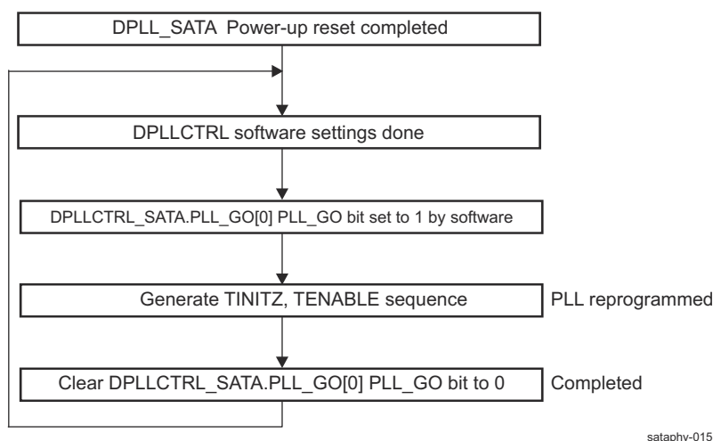
Figure 28-6. SATA PLL GO Sequence
