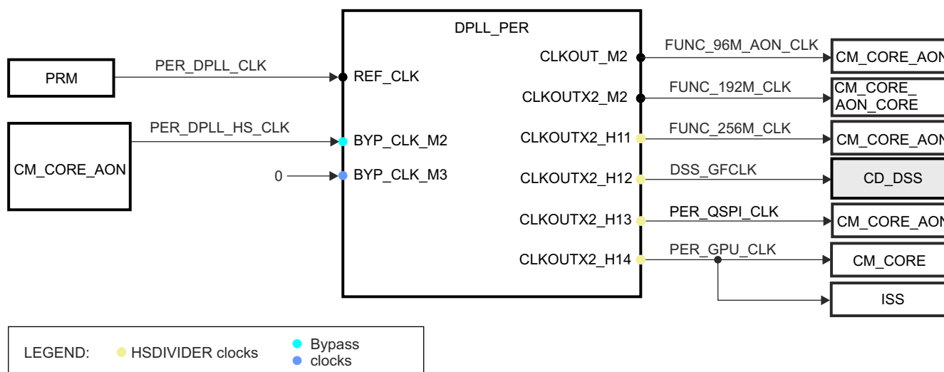
Figure 3-52. DPLL_PER Overview
