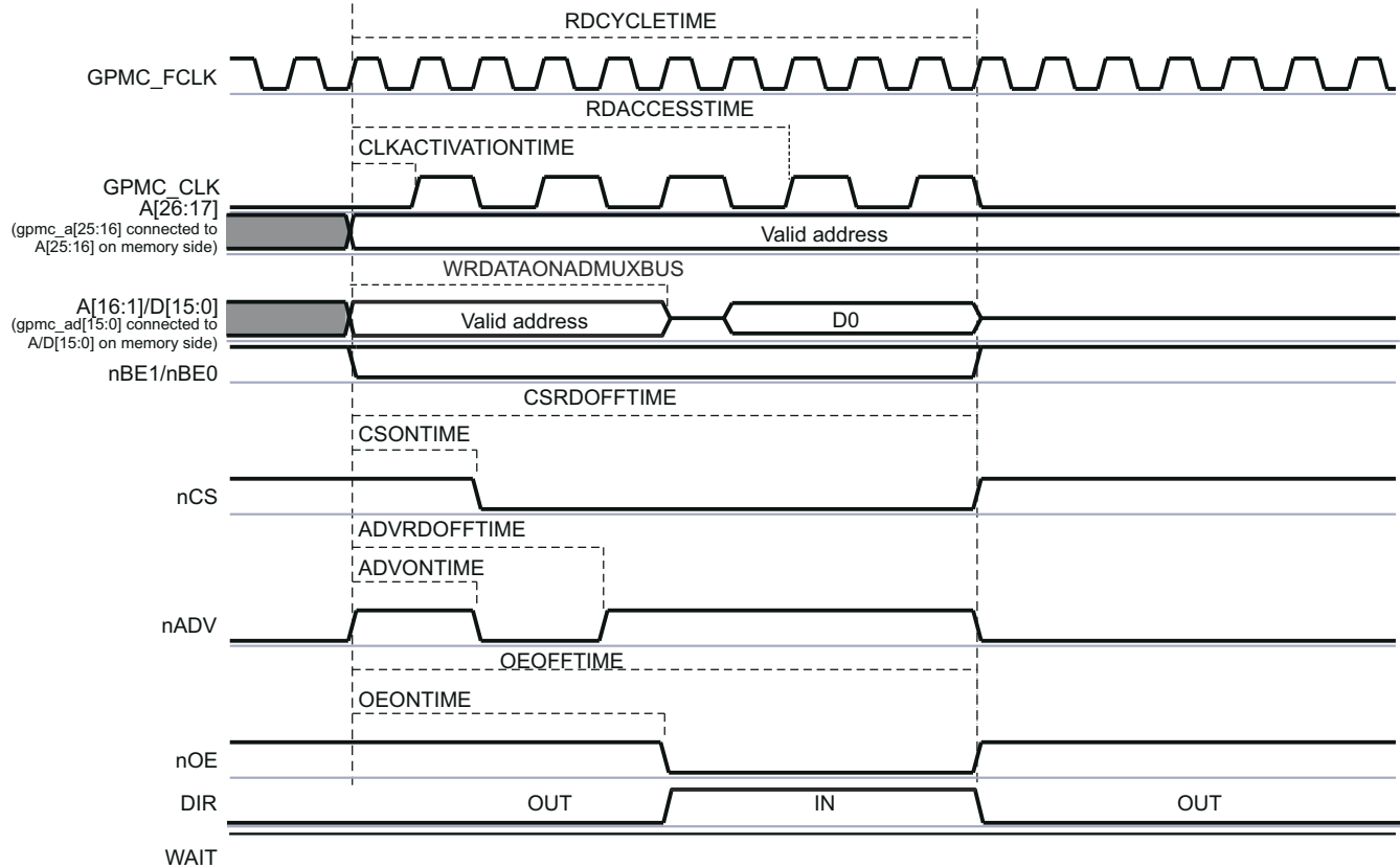
Figure 17-71. Synchronous Single Read (GPMCCLKDIVIDER = 1)
