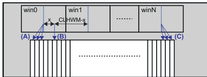
Figure 9-148. ISS ISP ISIF Clamp Value for Horizontal Direction
