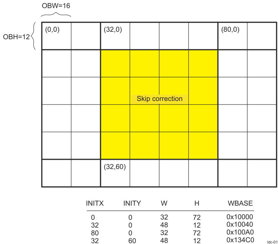
Figure 9-216. ISS SIMCOP LDC Multiple-Pass Correction Example
