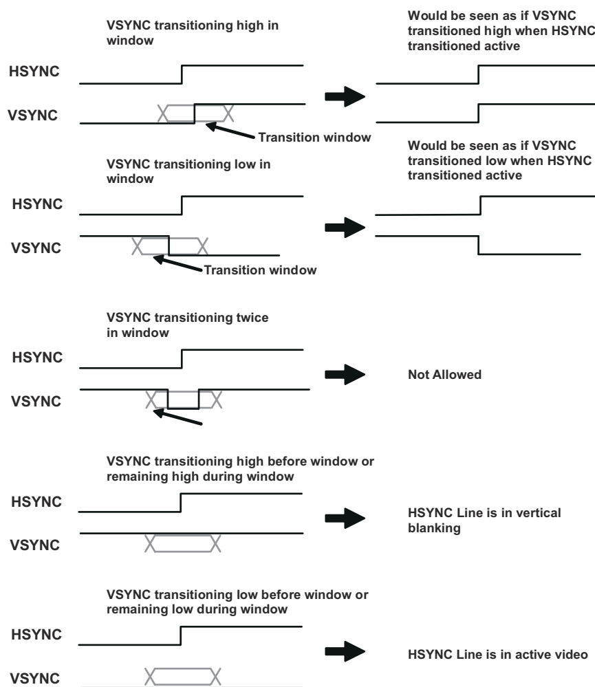
Figure 11-35. VSYNC Equivalence When Using Transition Window
