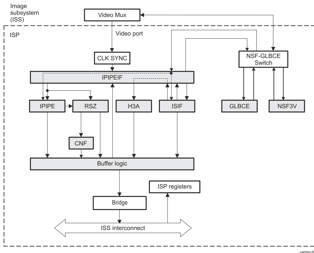
Figure 9-27. ISS ISP Block Diagram
