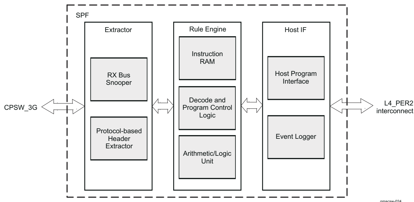
Figure 26-219. SPF Block Diagram
