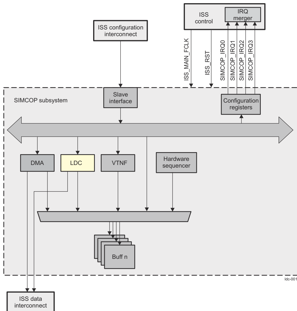
Figure 9-201. ISS SIMCOP LDC Subsystem
