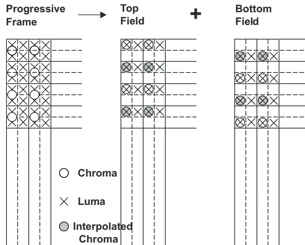
Figure 12-48. Ideal 4:2:2 Chroma Upsampling for Interlaced Scan
