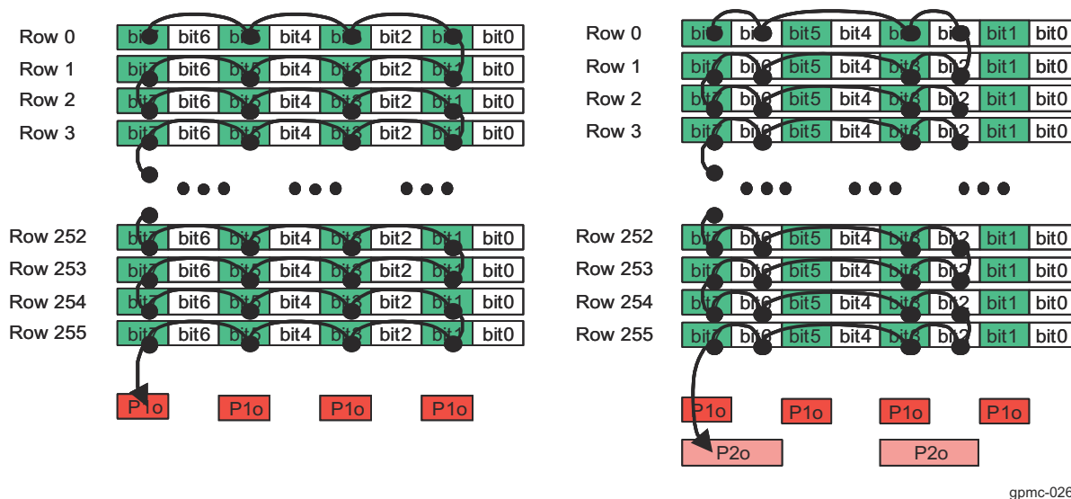
Figure 17-84. Hamming Code Accumulation Algorithm (1/2)
