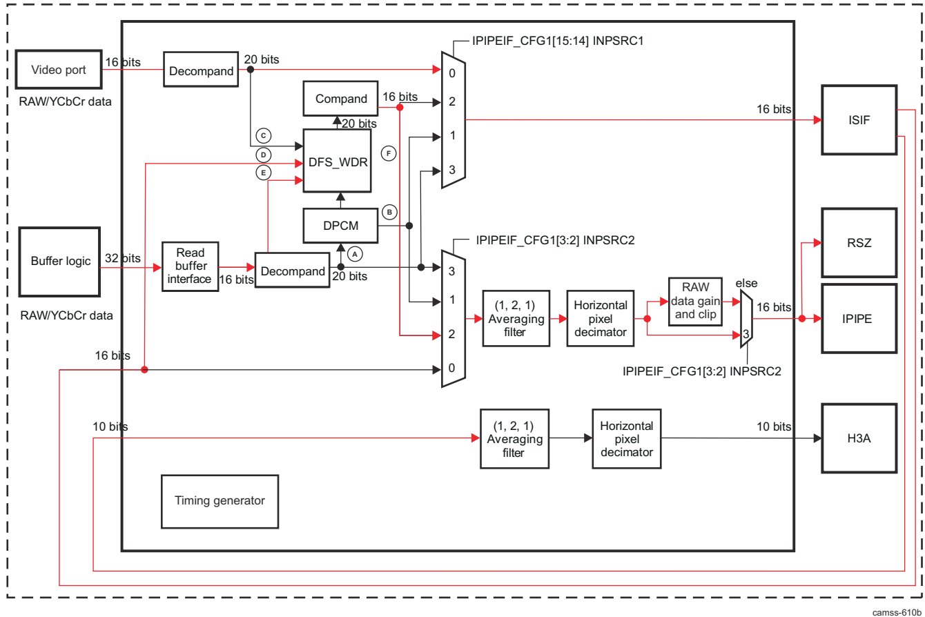
Figure 9-43. ISS ISP IPIPEIF INPSRC1 = 0 and INPSRC2 = 2 Data Paths
