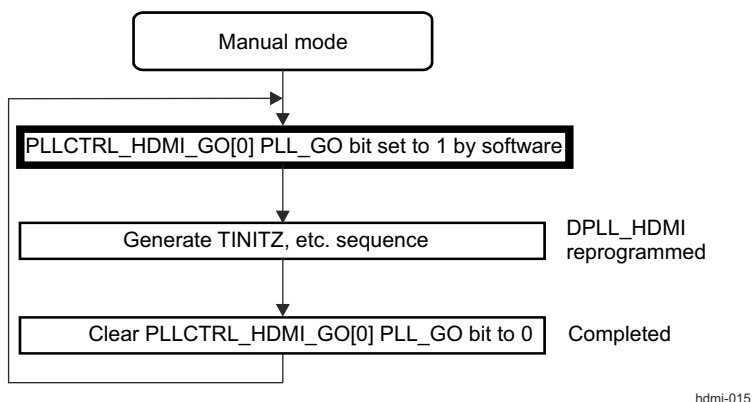
Figure 13-21. DPLL_HDMI GO Sequence (Manual Mode)
