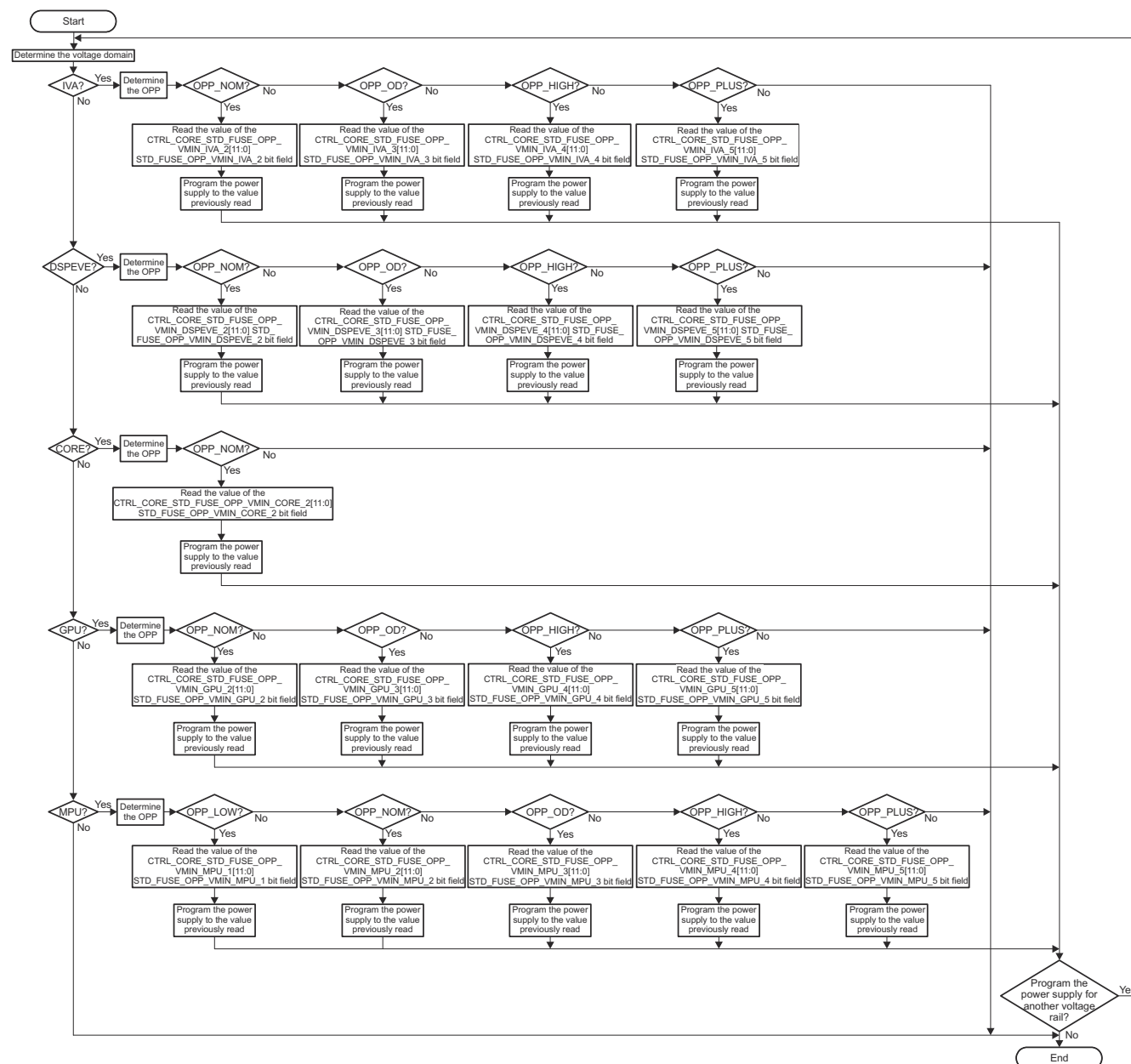
Figure 20-13. AVS Class 0 Procedure
