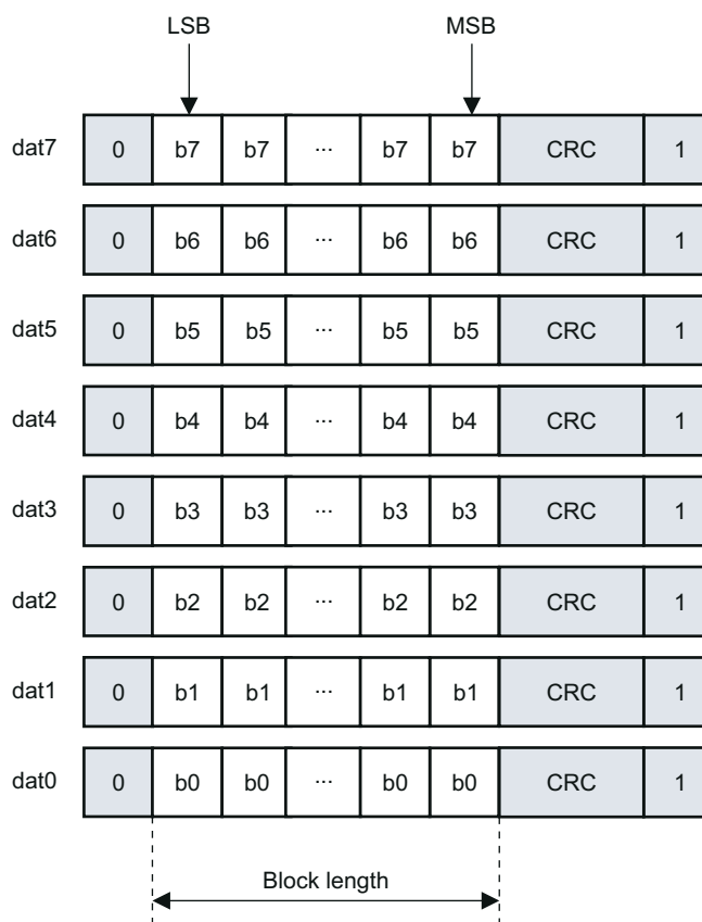
Figure 27-12. Data Token Format for 8-Bit Transfers
