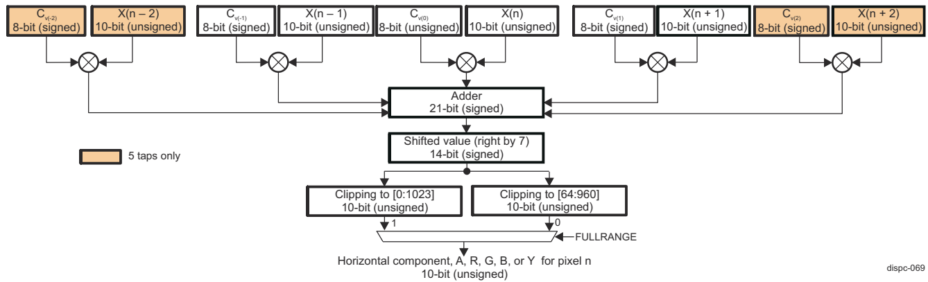
Figure 13-60. DISPC Macro-Architecture of the Horizontal Scaling for A, R, G, B, and Y Components (5-tap Restriction)
