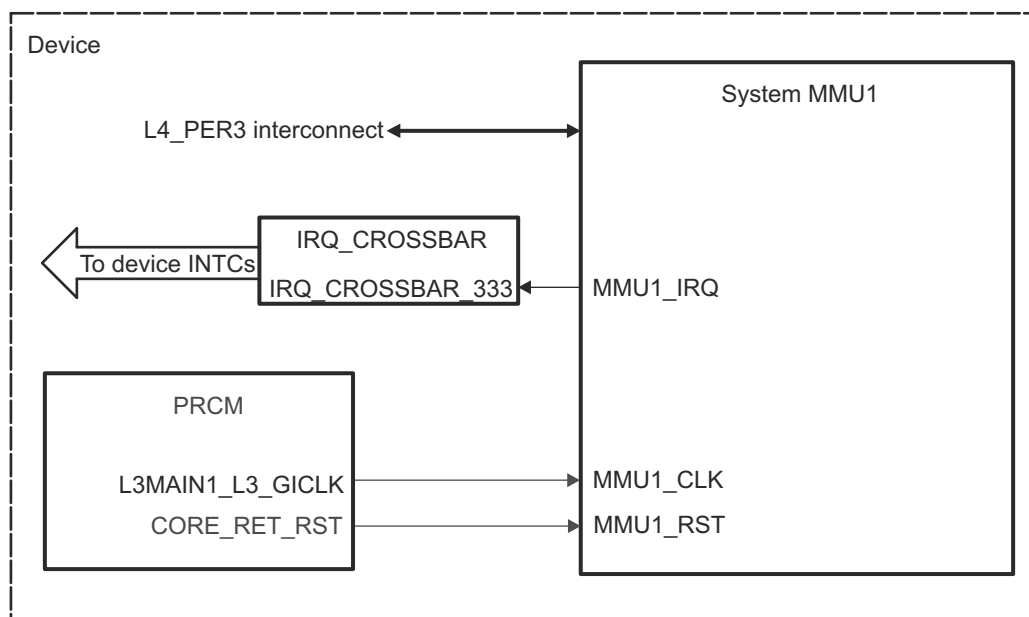
Figure 22-3. System MMU1 Integration
