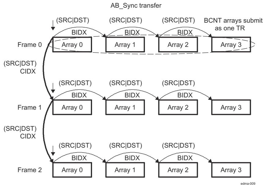
Figure 18-20. AB-Synchronized Transfers (ACNT = n , BCNT = 4, CCNT = 3)
