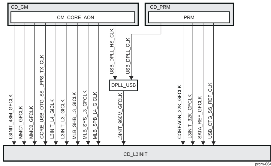
Figure 3-74. CD_L3INIT Overview
