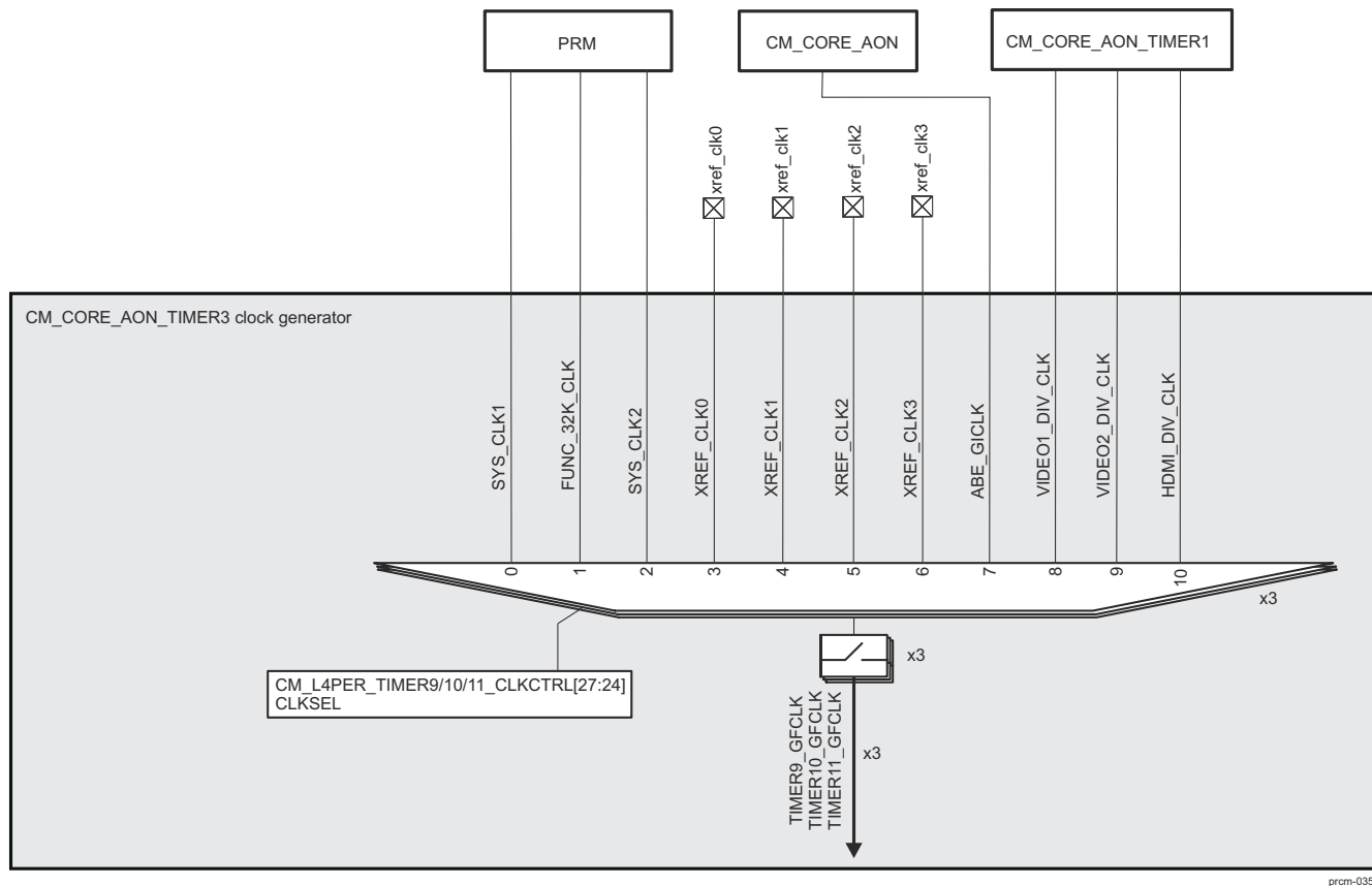
Figure 3-46. CM_CORE_AON_TIMER3 Clock Manager Overview
