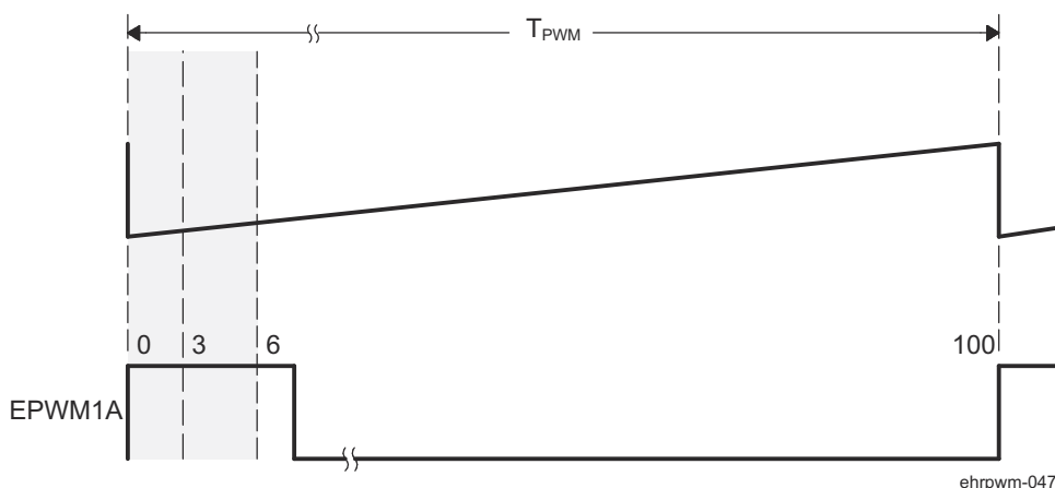
Figure 31-51. Low % Duty Cycle Range Limitation Example When PWM Frequency = 1 MHz
