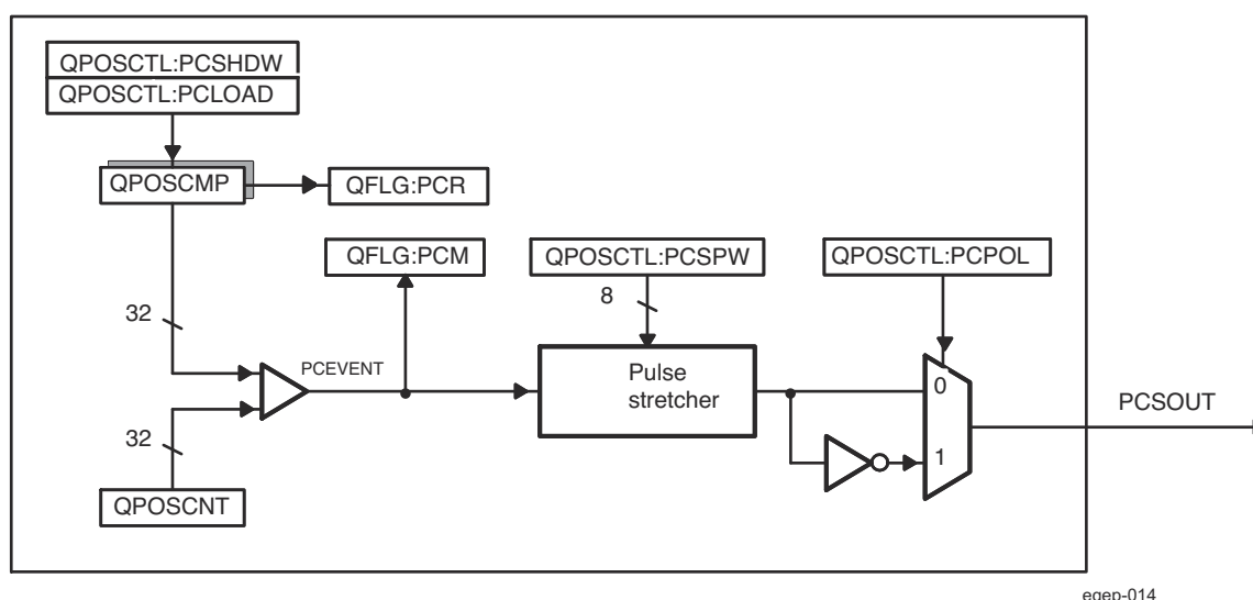
Figure 31-73. eQEP Position-compare Unit
