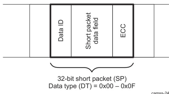
Figure 10-16. CSI2 Short Packet Structure
