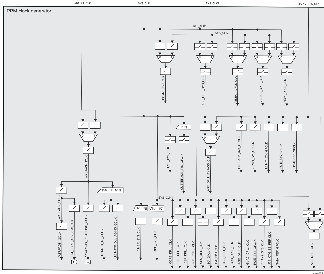
Figure 3-39. PRM Clock Manager Overview
