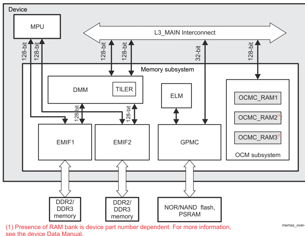
Figure 17-1. Memory Subsystem Functional Diagram
