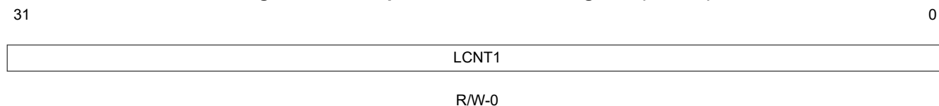
Figure 8-46. Loop 1 Iteration Count Register (LCNT1)
