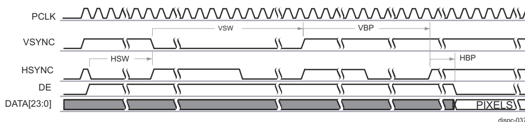
Figure 13-32. DISPC Active Matrix Timing Diagram of Configuration 2 (Start of Frame)
