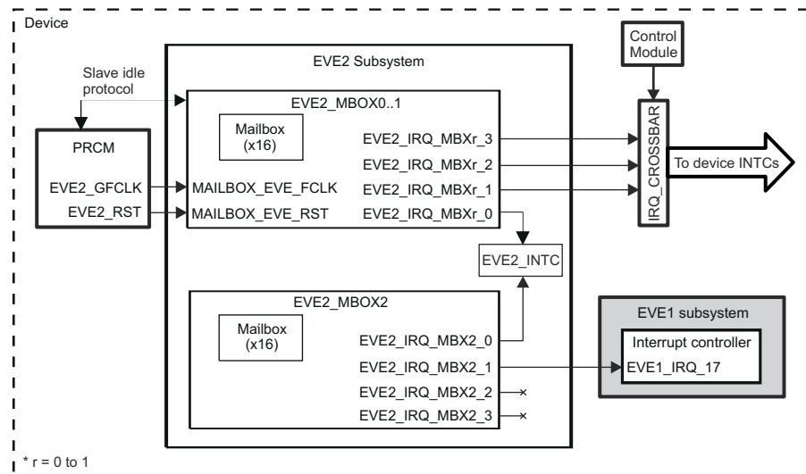
Figure 21-5. EVE2_MBOX Integration
