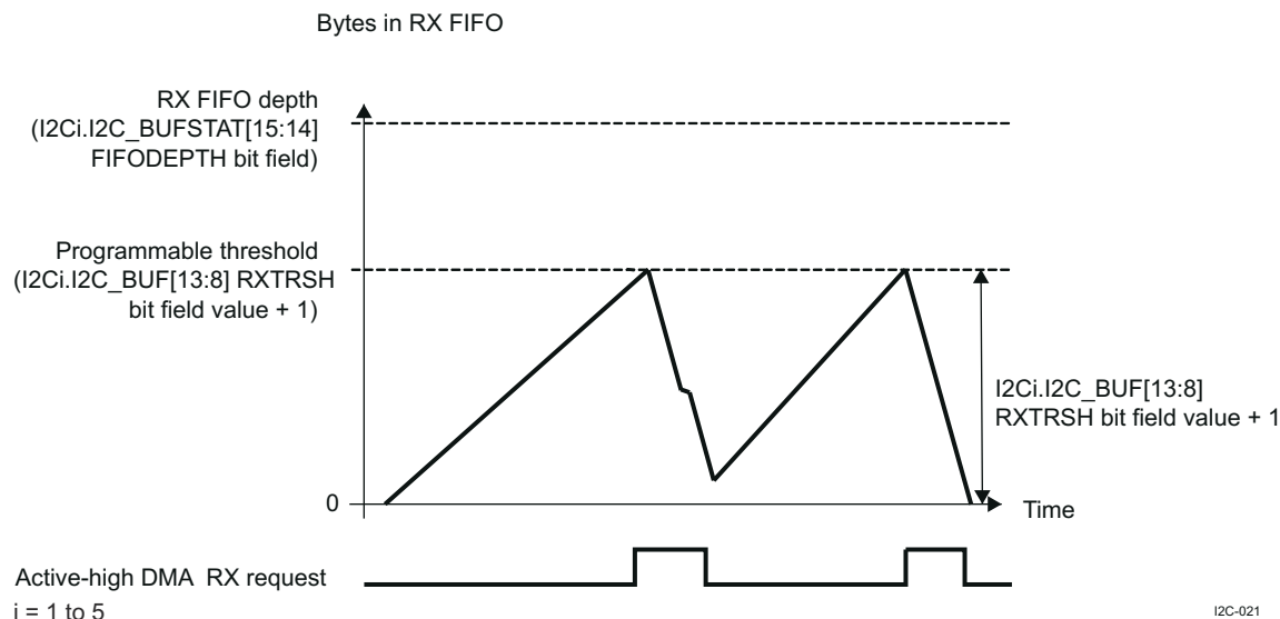
Figure 26-16. HS I 2 C Receive FIFO DMA Request Generation
