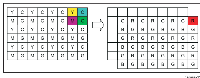
Figure 9-142. ISS ISP ISIF Last Pixel/First Line Generation
