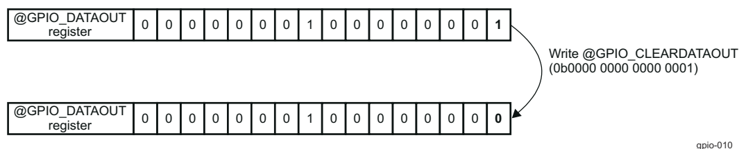
Figure 29-12. GPIO_CLEARDATAOUT Register Example
