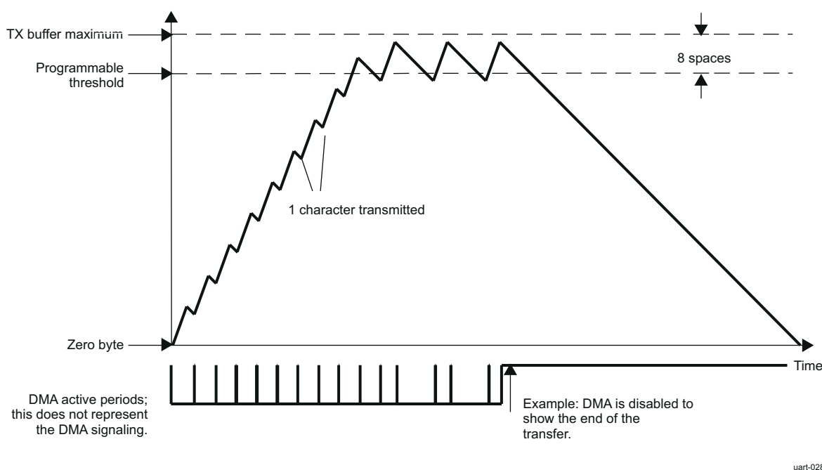
Figure 26-64. Transmit FIFO DMA Request Generation (8 Spaces)
