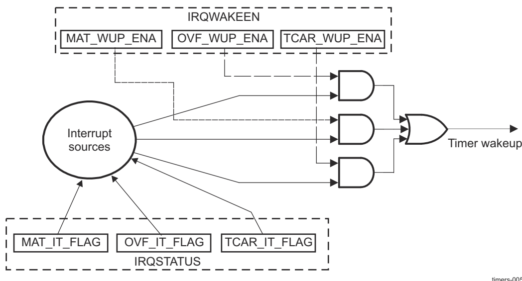
Figure 24-7. Wake-Up Request Generation
