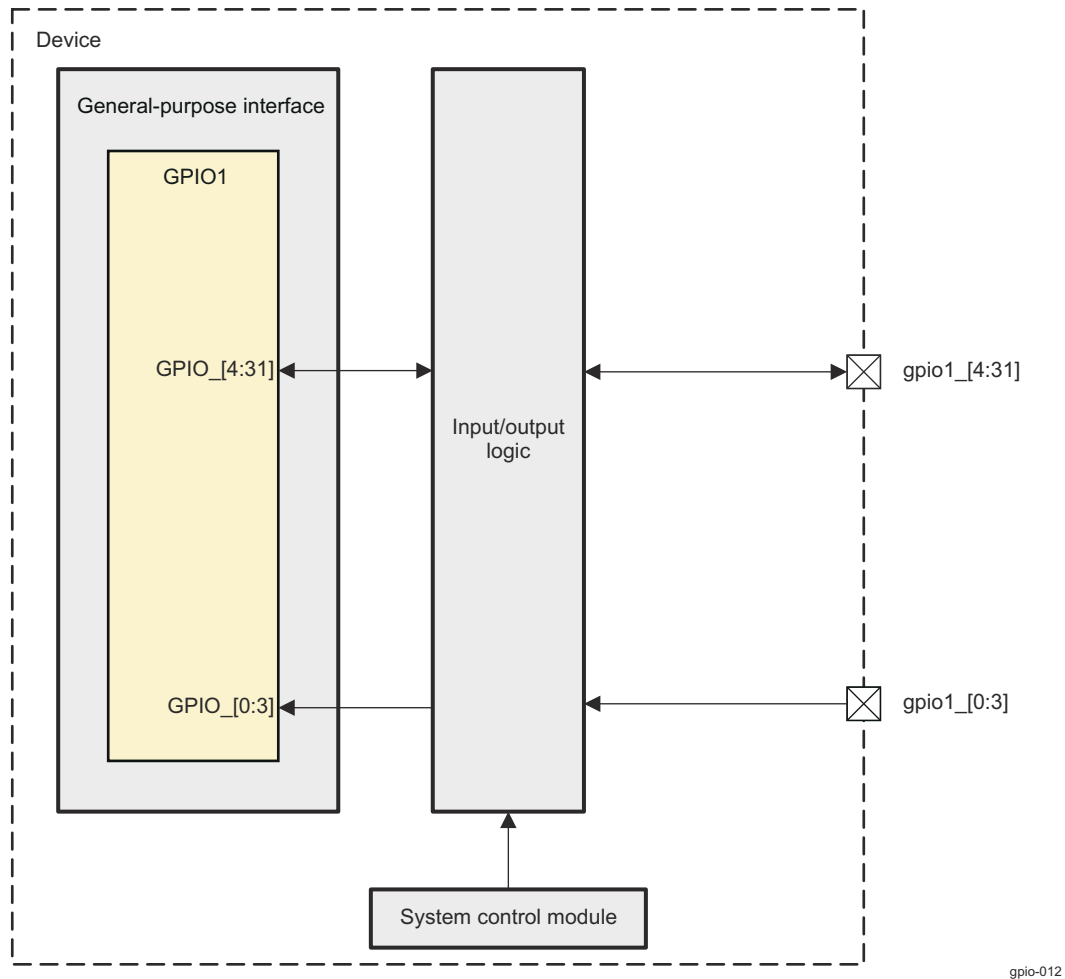
Figure 29-3. GPIO1 Signal Connections
