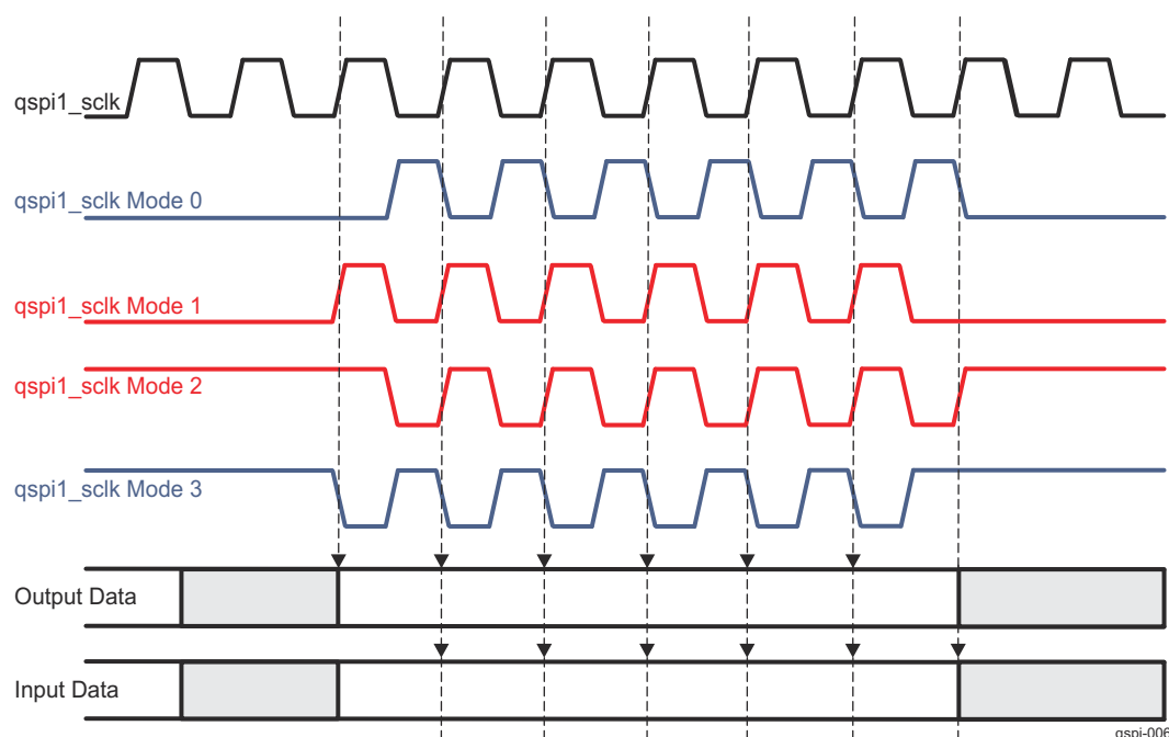
Figure 26-106. SPI Clock Modes
