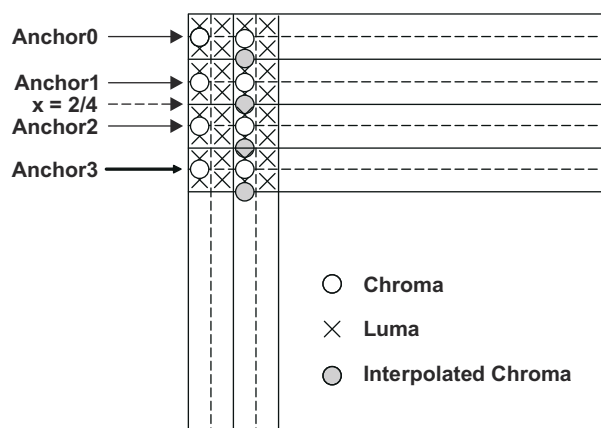
Figure 12-46. Anchor Pixels
