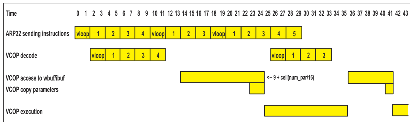
Figure 8-68. Example of Operation Delay Slots
