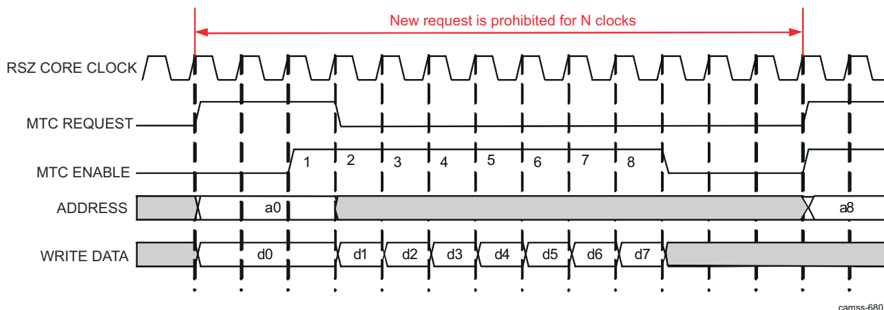
Figure 9-93. ISS ISP RSZ MTC DMA Bandwidth Control
