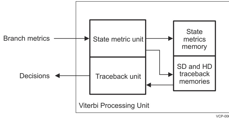
Figure 32-6. Viterbi Processing Unit
