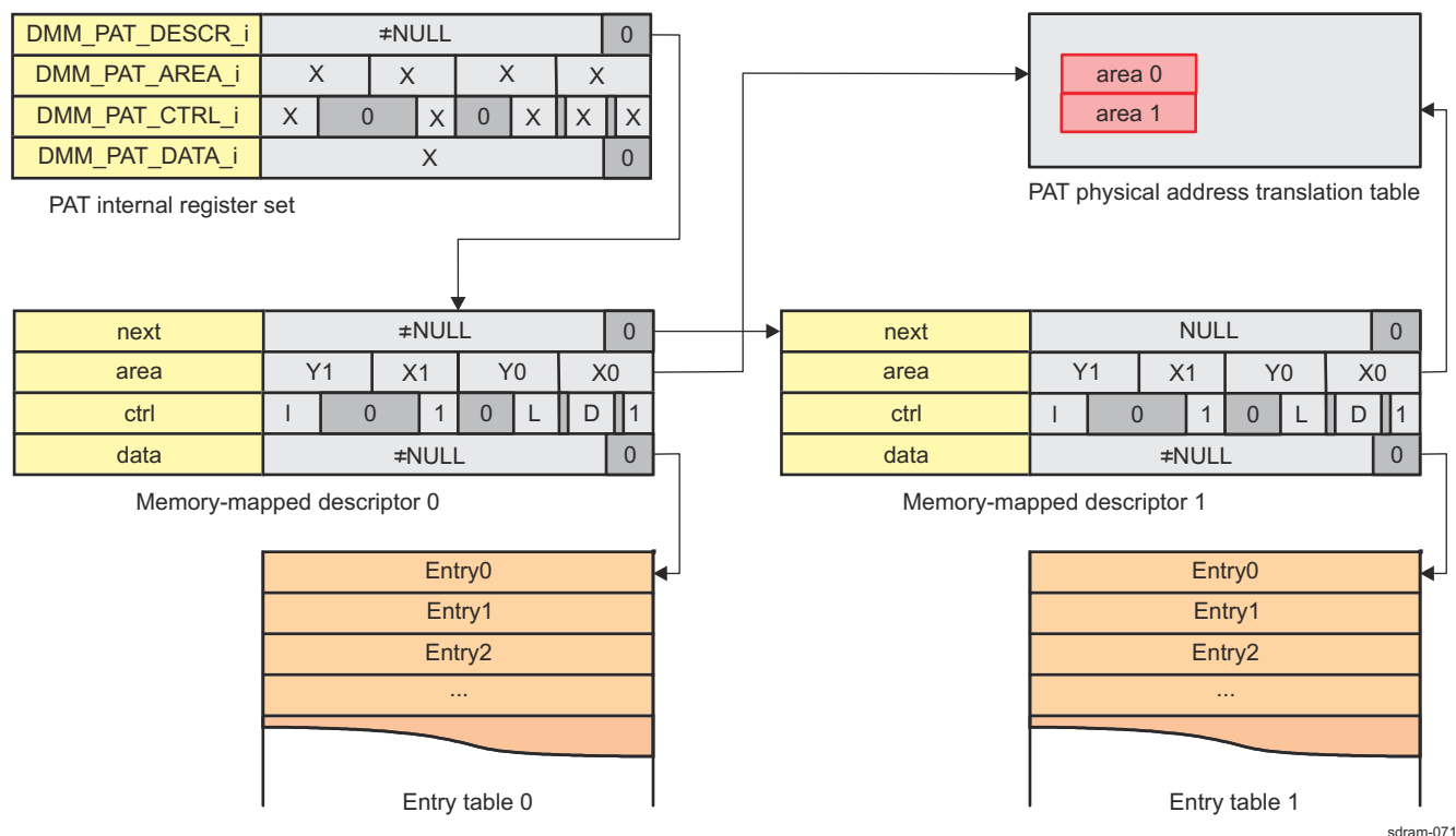
Figure 17-42. Synchronized Auto-Configured Area Refill Scheme
