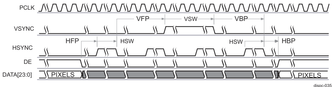
Figure 13-30. DISPC Active Matrix Timing Diagram of Configuration 1 (Between Frames)
