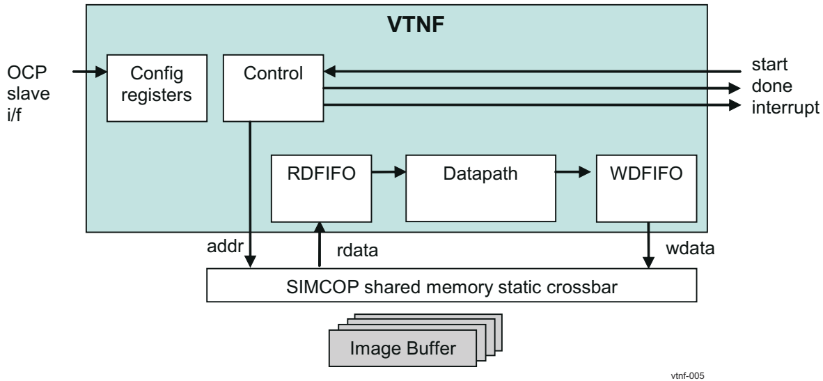
Figure 9-198. ISS SIMCOP VTNF Block Diagram
