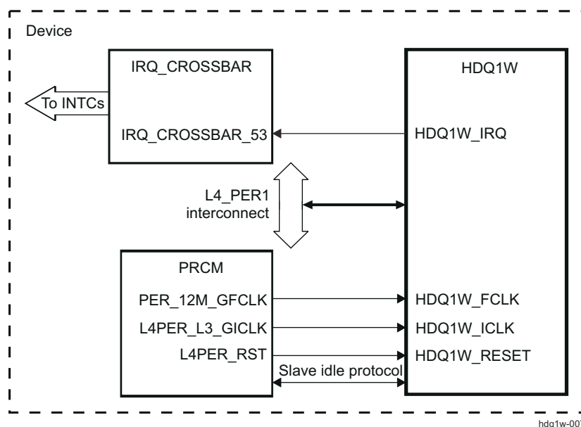
Figure 26-34. HDQ1W Integration
