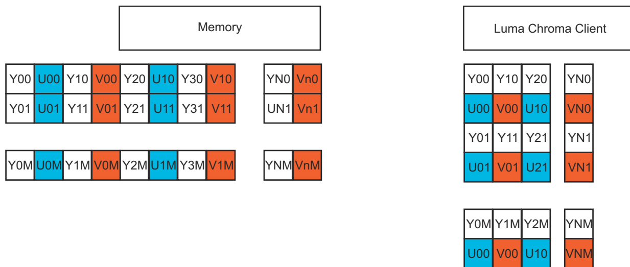
Figure 12-57. YC 4:2:2 (Data Type 7)
