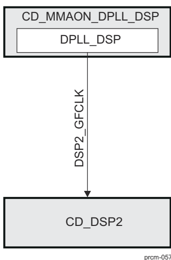
Figure 3-67. CD_DSP2 Overview
