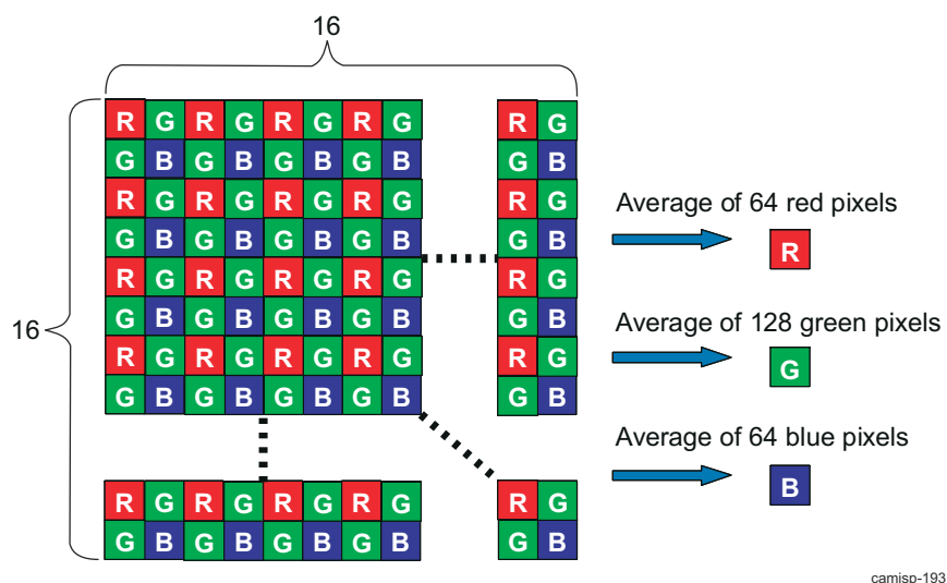
Figure 9-89. ISS ISP IPIPE Boxcar Operation (16 × 16 Block)
