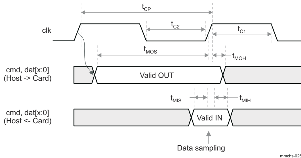
Figure 27-31. Output Driven on Rising Edge
