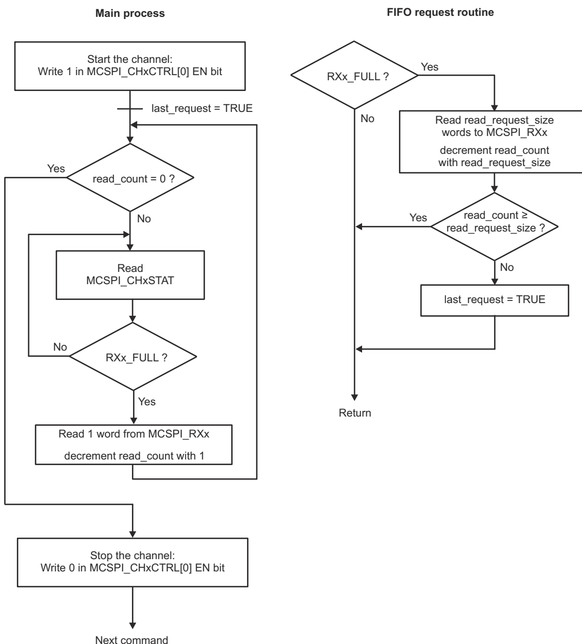
Figure 26-100. FIFO Mode Receive-Only Without Word Count (Master)
