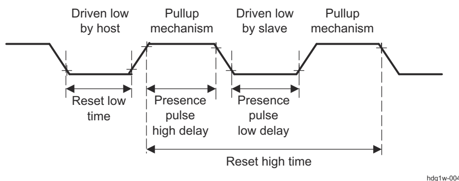
Figure 26-31. 1-Wire (SDQ) Reset Timing Diagram
