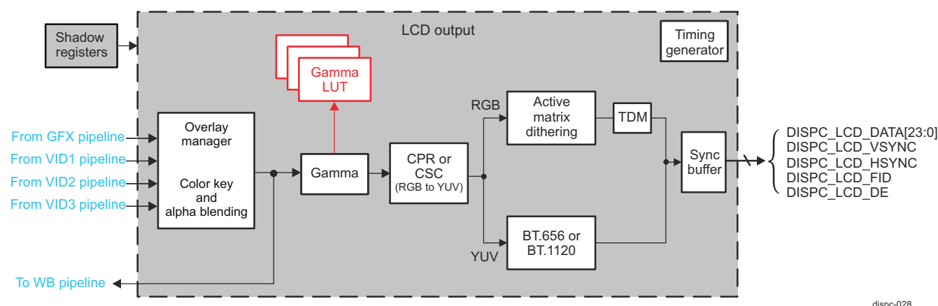
Figure 13-73. DISPC LCD Output Architecture
