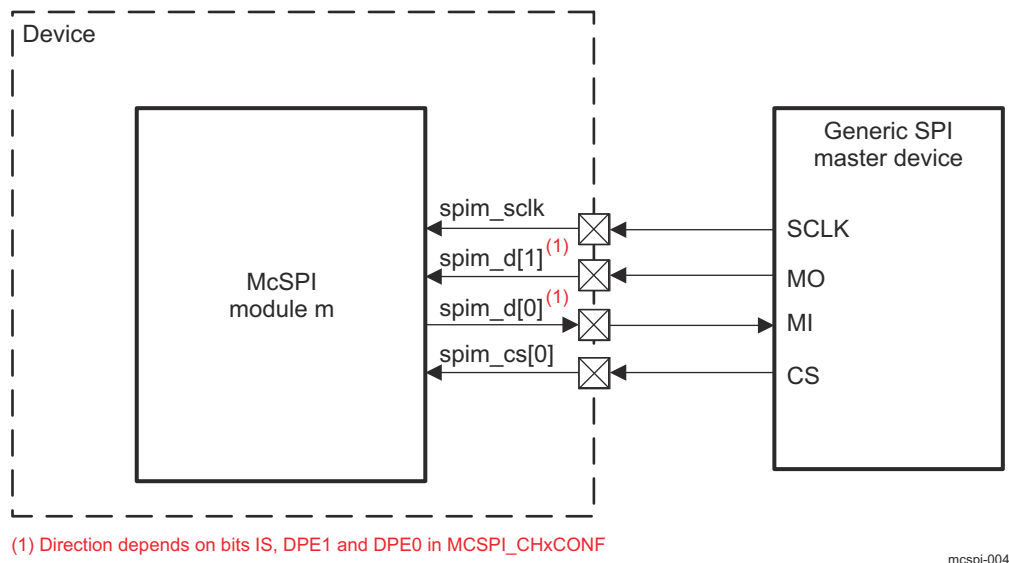
Figure 26-80. McSPI Slave Mode (Full Duplex)
