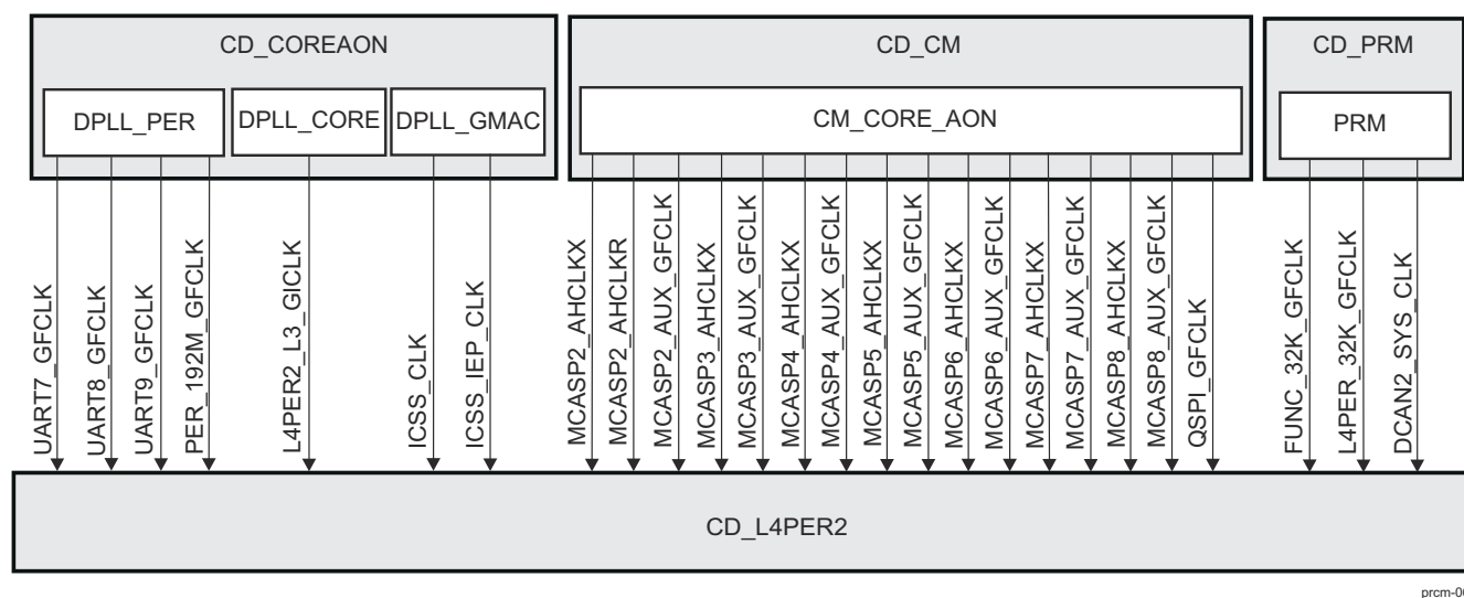
Figure 3-71. CD_L4PER2 Overview
