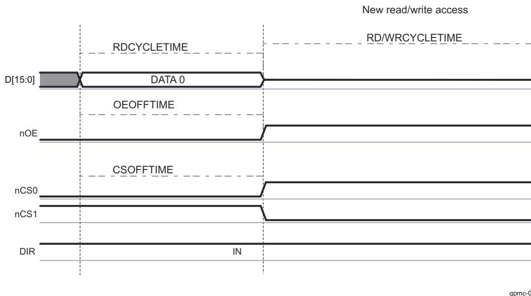
Figure 17-62. Read-to-Read for an Address-Data Multiplexed Device, on Different Chip-Select, Without Bus Turnaround (nCS Attached to a Fast Device)
