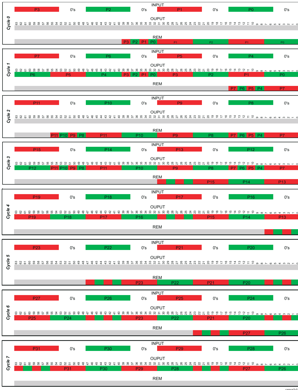
Figure 10-31. CAL MIPI RAW10 Data Packing
