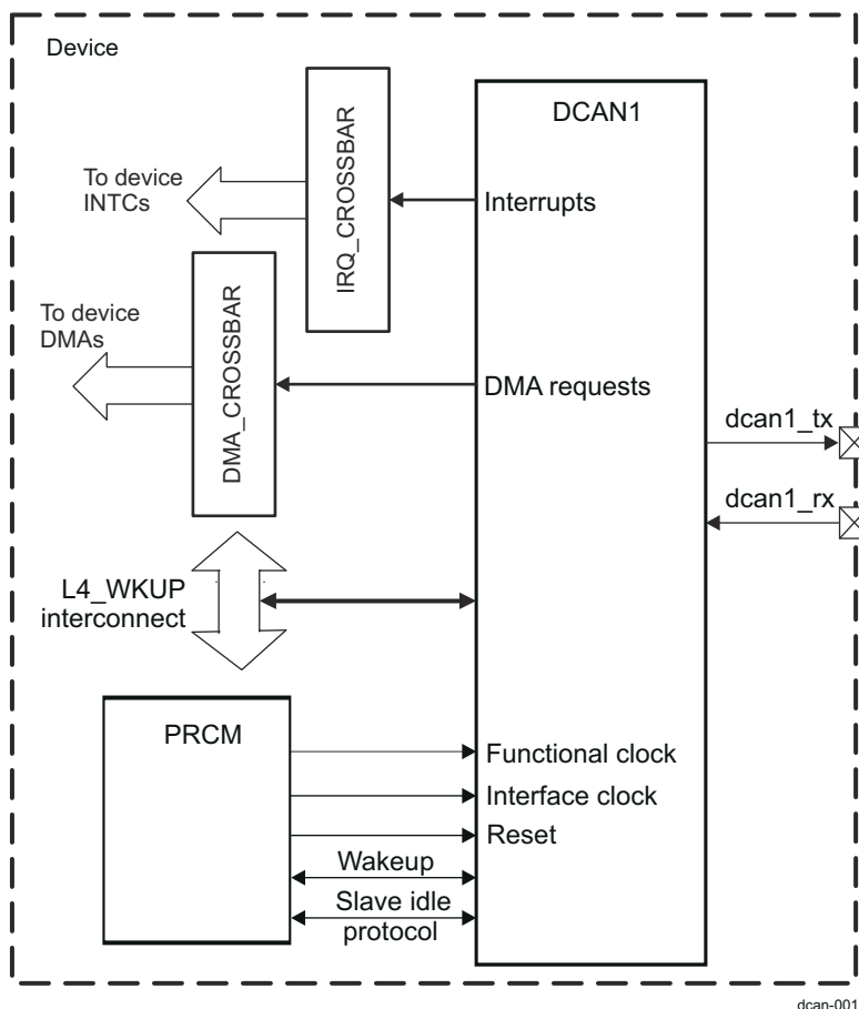
Figure 26-164. DCAN1 Overview
