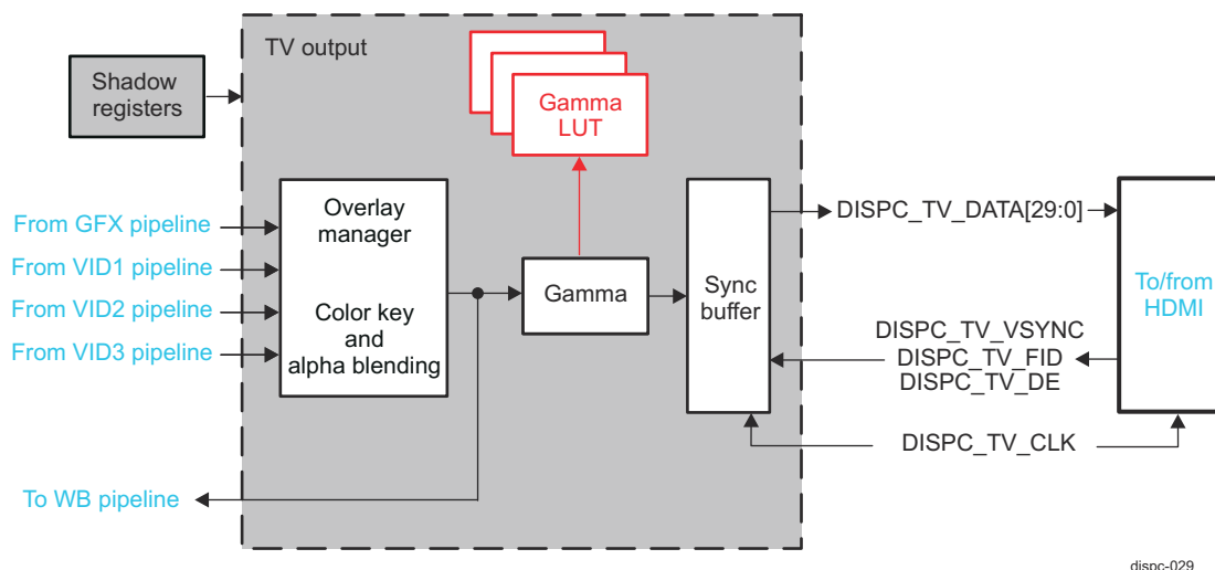
Figure 13-93. DISPC TV Output Architecture
