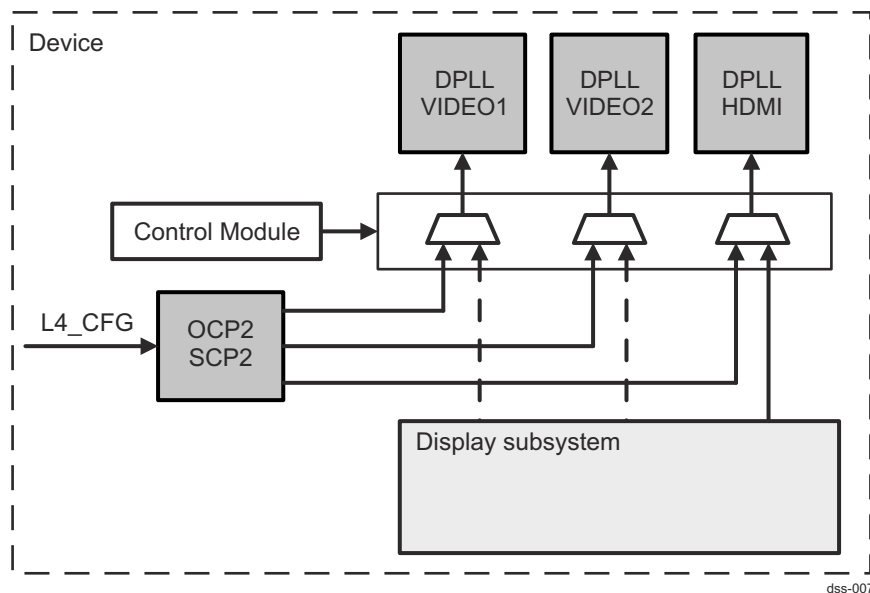
Figure 13-9. OCP2SCP2 Overview
