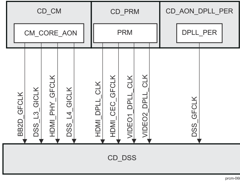
Figure 3-78. CD_DSS Overview
