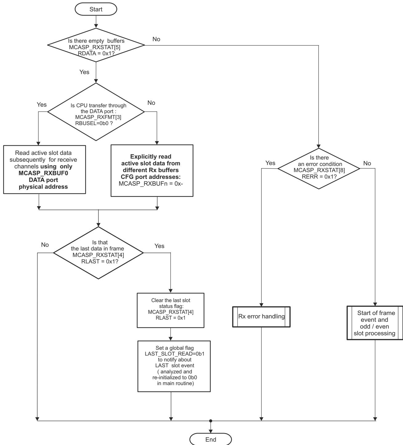
Figure 26-140. McASP Receive Interrupt Events Servicing
