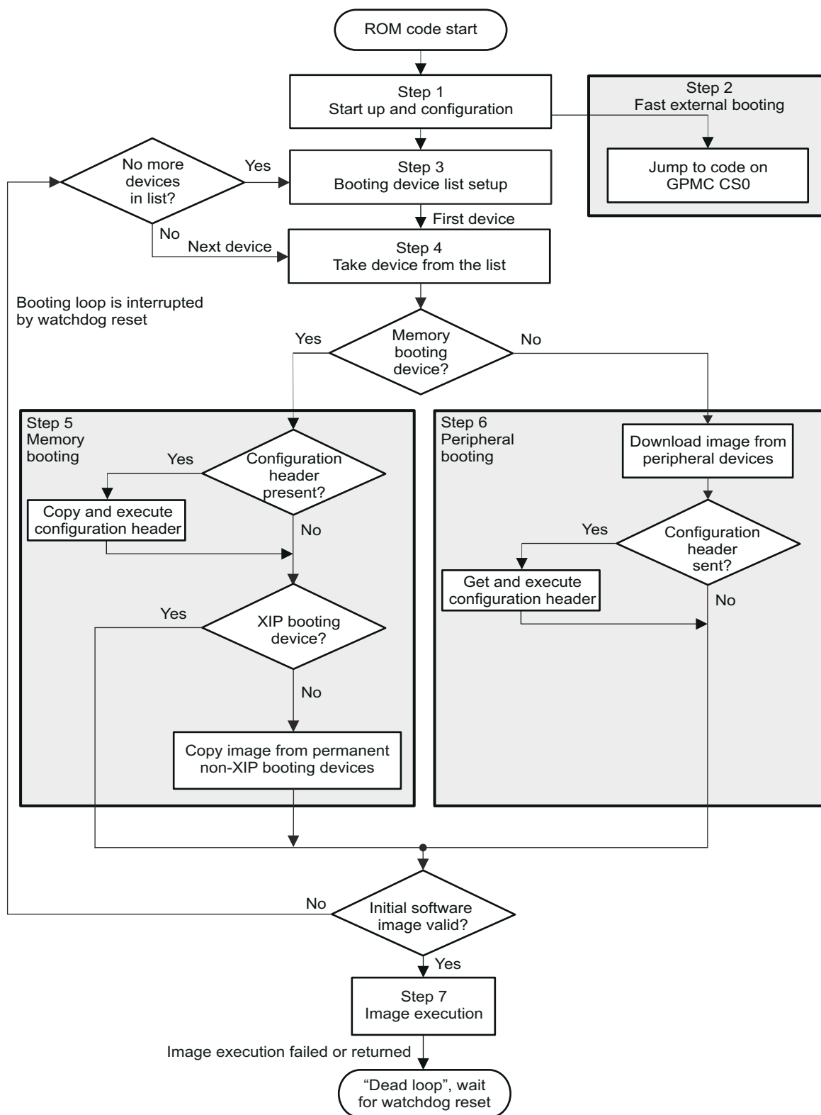
Figure 34-7. Overall Booting Sequence
