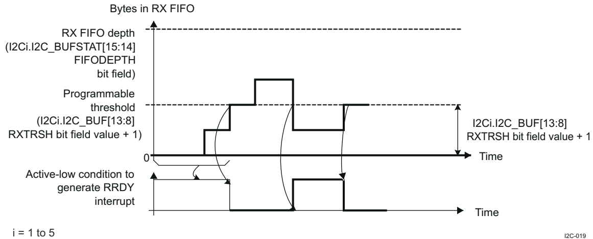
Figure 26-14. HS I 2 C Receive FIFO Interrupt Request Generation
