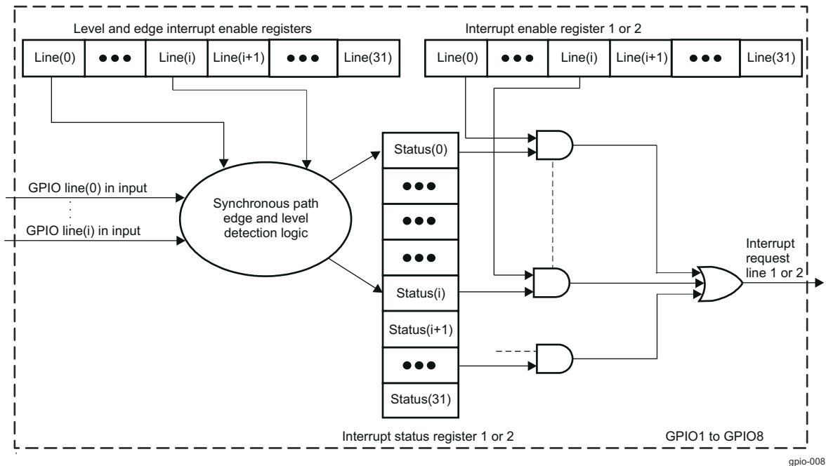
Figure 29-9. Interrupt Request Generation
