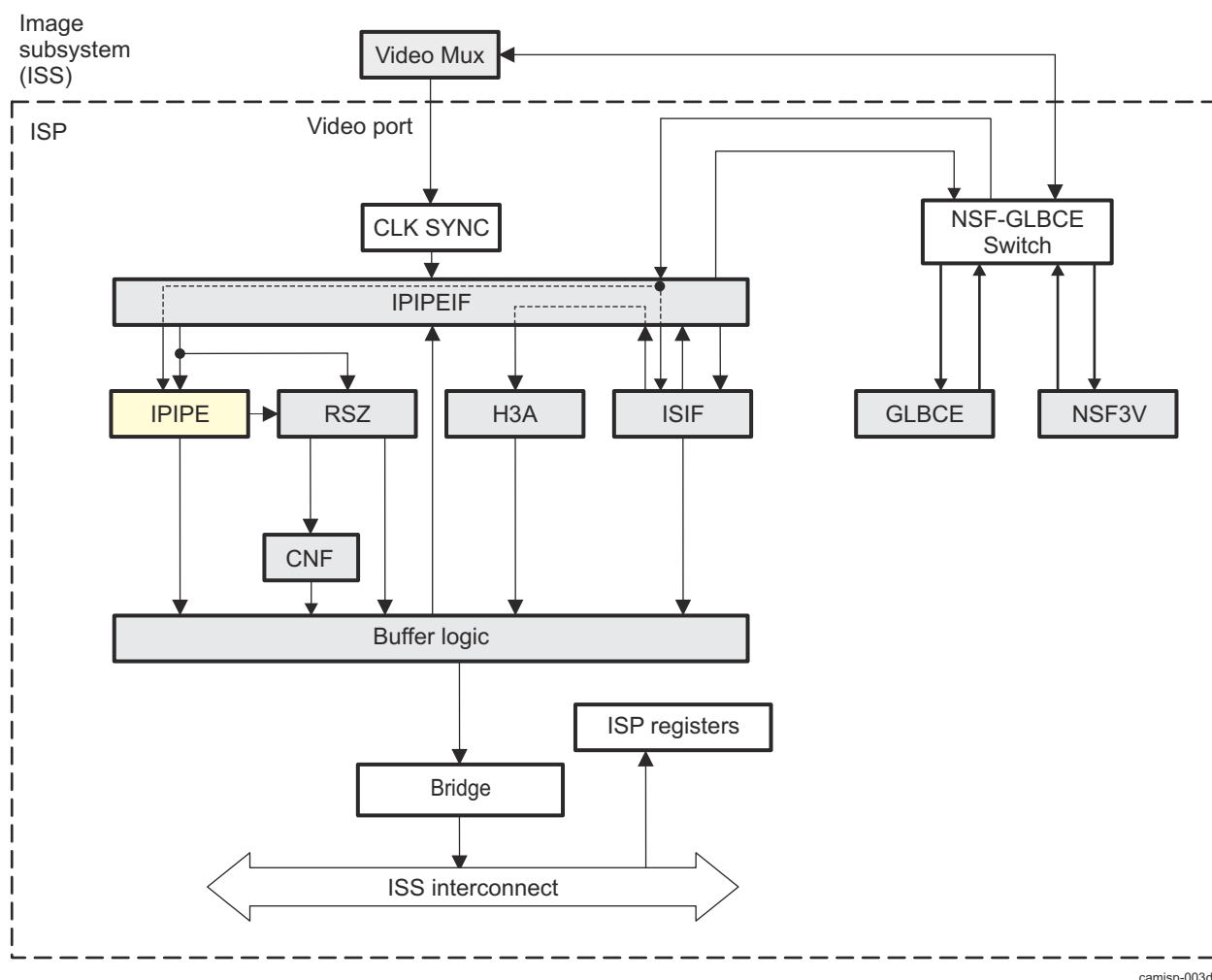
Figure 9-55. ISS ISP IPIPE High-Level Diagram
