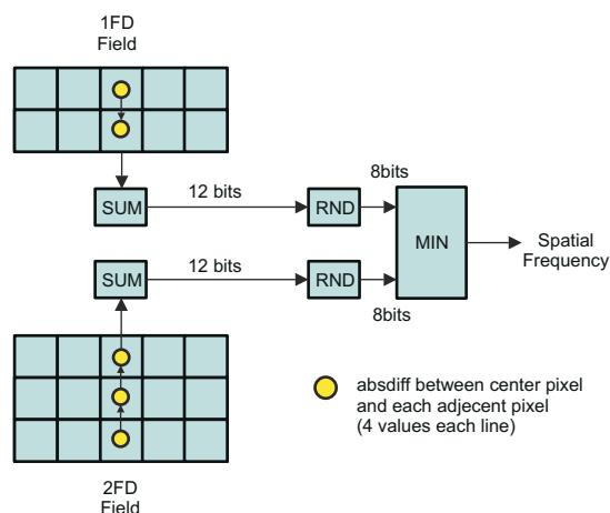
Figure 12-7. Motion Detection (MDT) Uniform Area Data Path
