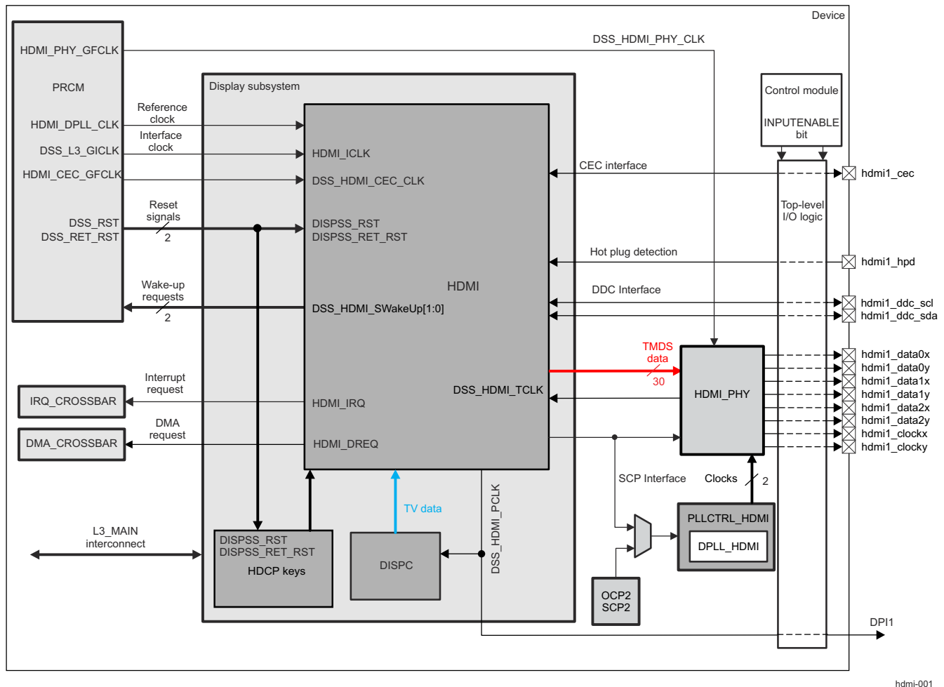
Figure 13-103. HDMI Overview
