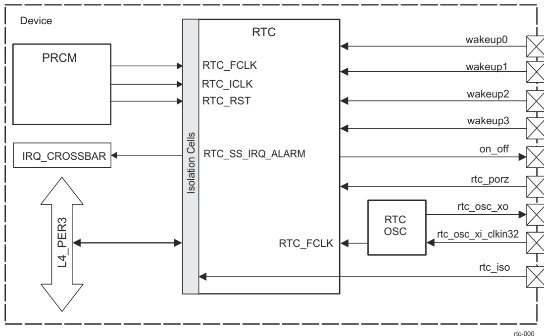
Figure 25-1. RTC Block Diagram
