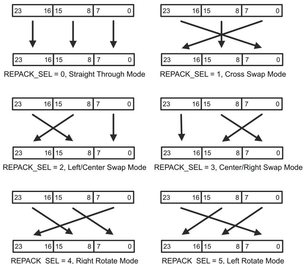
Figure 11-15. Bytelane Swapping Modes
