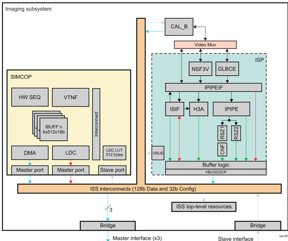
Figure 9-1. ISS Overview
