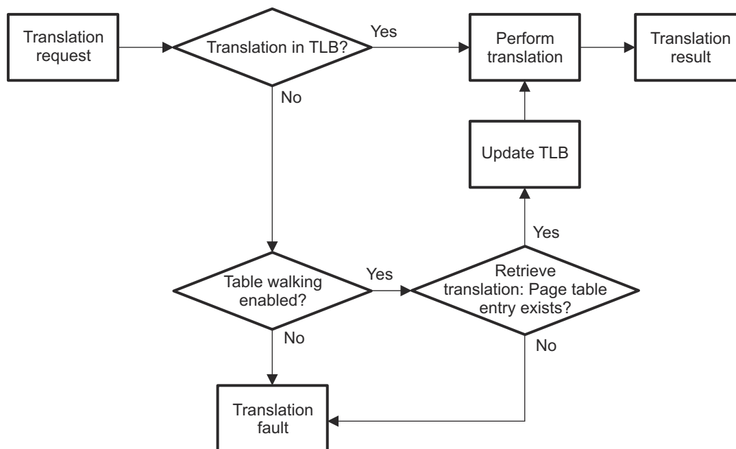
Figure 22-6. Translation Process
