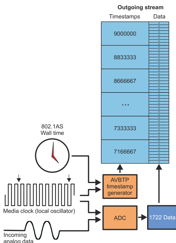
Figure 26-217. Cross Time Stamping and Presentation Timestamps
