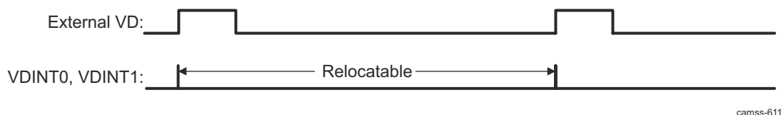
Figure 9-169. ISS ISP ISIF VDINT0/VDINT1/VDINT2 Interrupt Behavior When VDPOL = 0
