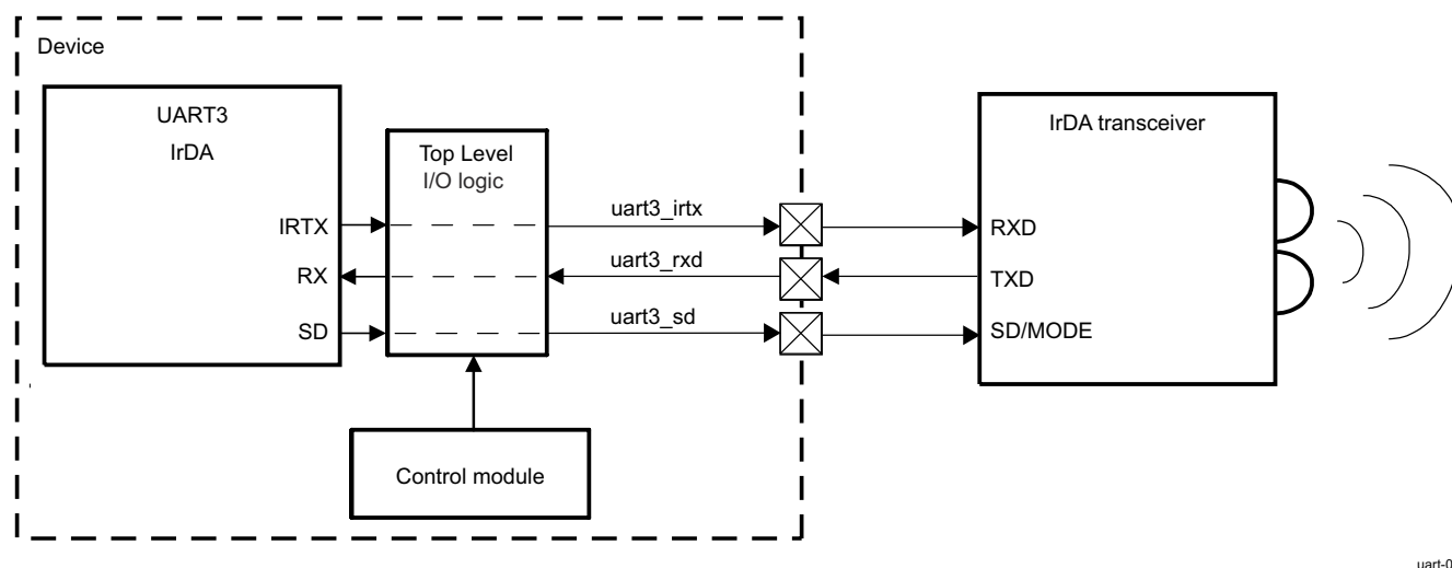
Figure 26-40. IrDA System Overview
