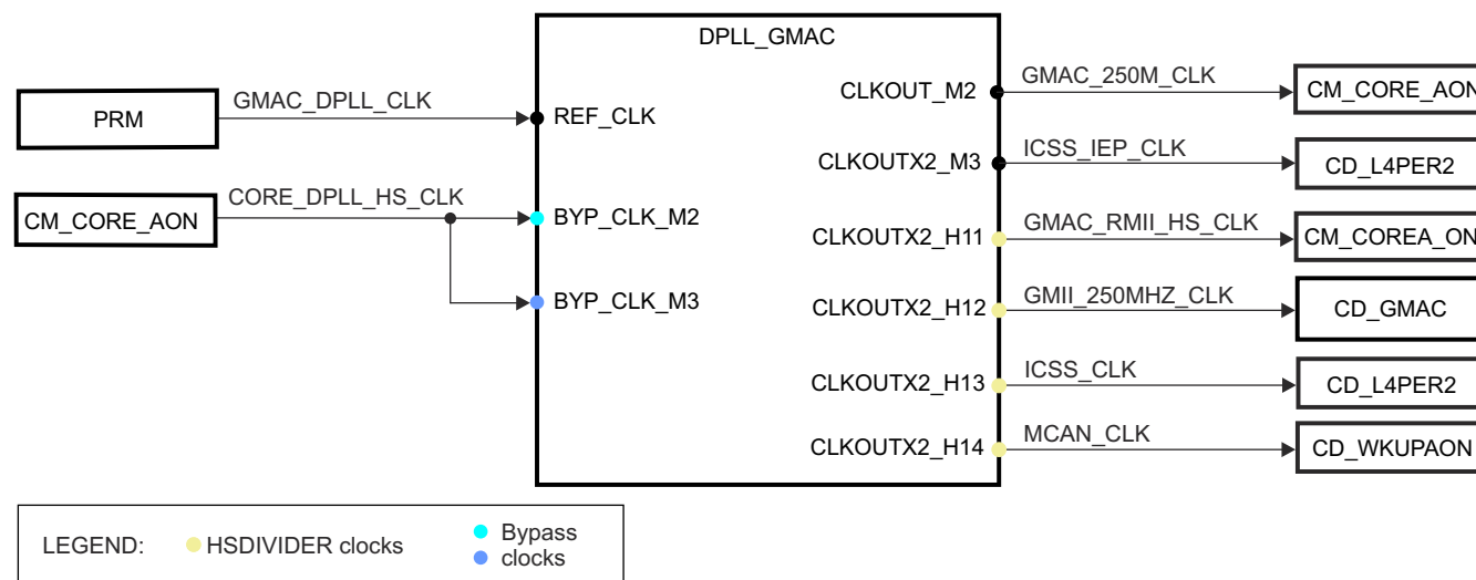
Figure 3-60. DPLL_GMAC Overview
