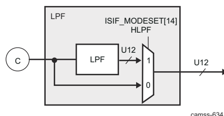
Figure 9-159. ISS ISP ISIF Low-Pass Filter Block Diagram
