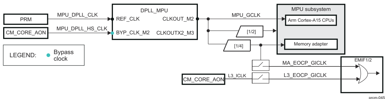
Figure 3-55. DPLL_MPU Overview
