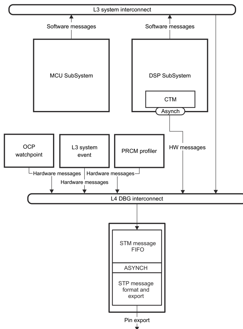
Figure 8-23. Typical STM System Integration
