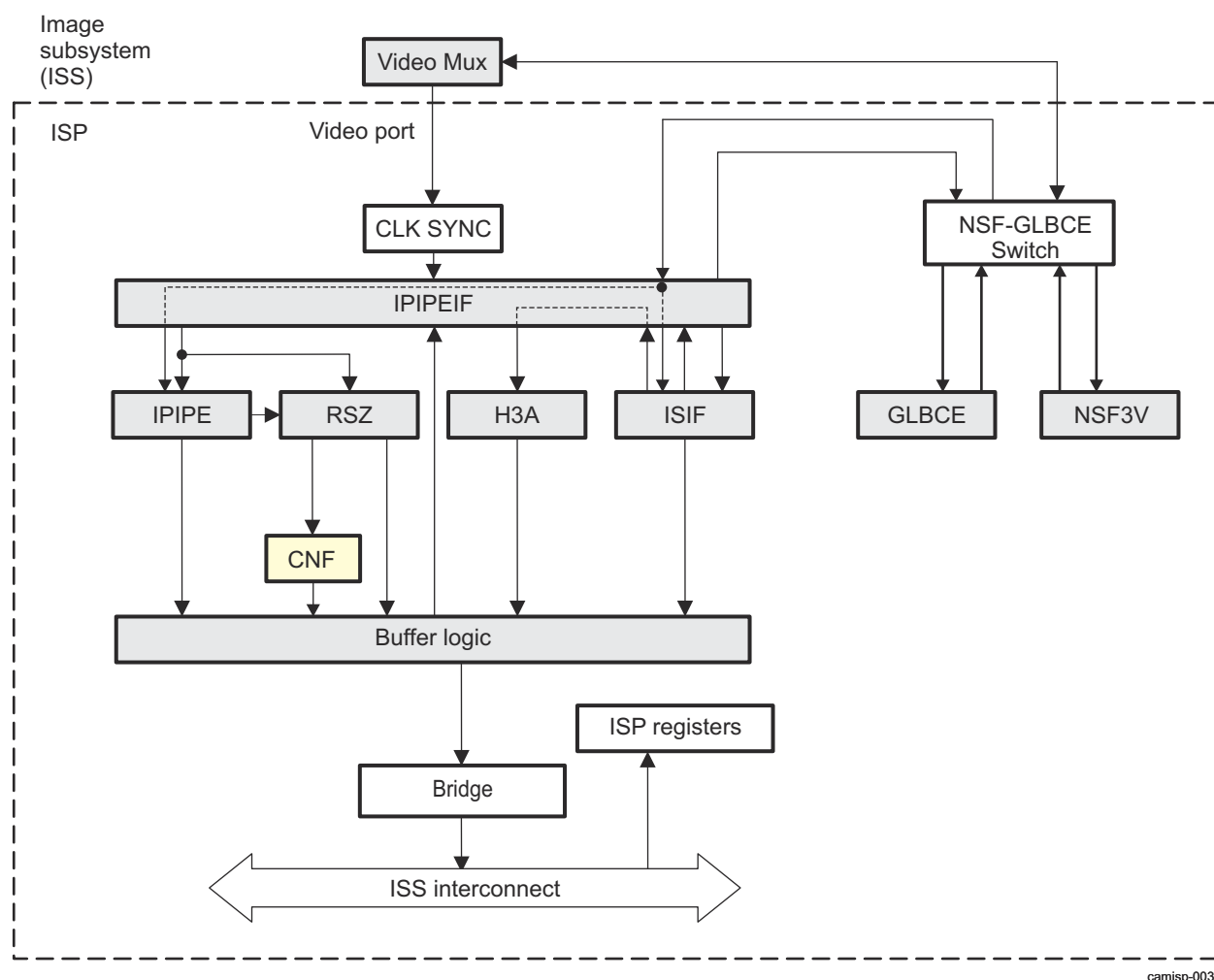
Figure 9-108. ISS ISP CNF High-Level Diagram
