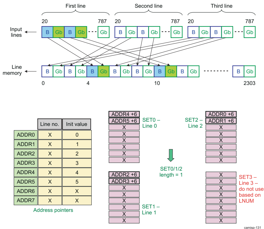
Figure 9-134. ISS ISP ISIF Example of Combining Three Input Lines Into a Single Line
