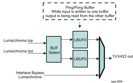
Figure 12-17. Output Data Path
