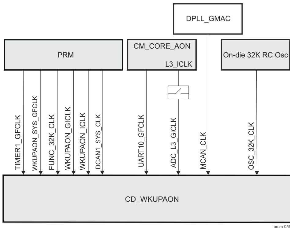
Figure 3-65. CD_WKUPAON Overview
