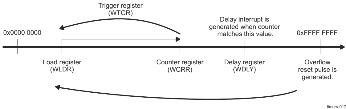
Figure 24-21. Watchdog Timers General Functional View
