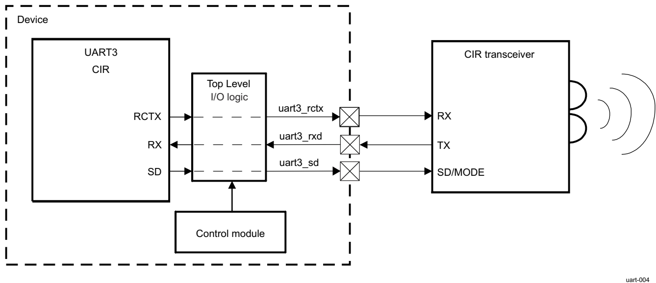
Figure 26-49. CIR System Overview
