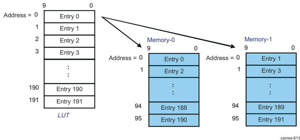
Figure 9-125. ISS ISP ISIF Linearization LUT Memories
