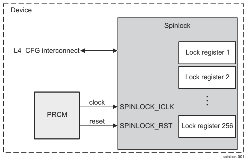
Figure 23-1. Spinlock Overview
