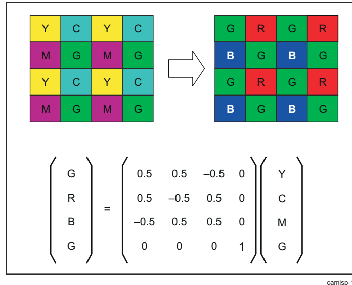
Figure 9-137. ISS ISP ISIF Color Space Converter Operation: CMYG to RGBG
