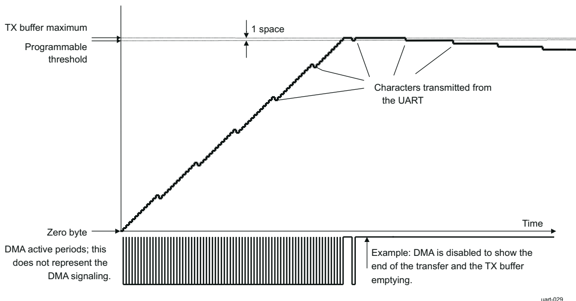
Figure 26-65. Transmit FIFO DMA Request Generation (1 Space)
