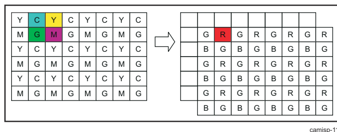
Figure 9-140. ISS ISP ISIF Second Pixel/First Line Generation
