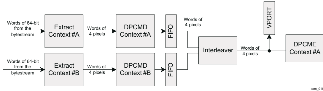
Figure 10-28. CAL Stream Interleaving - Logical View
