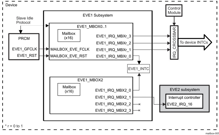
Figure 21-4. EVE1_MBOX Integration
