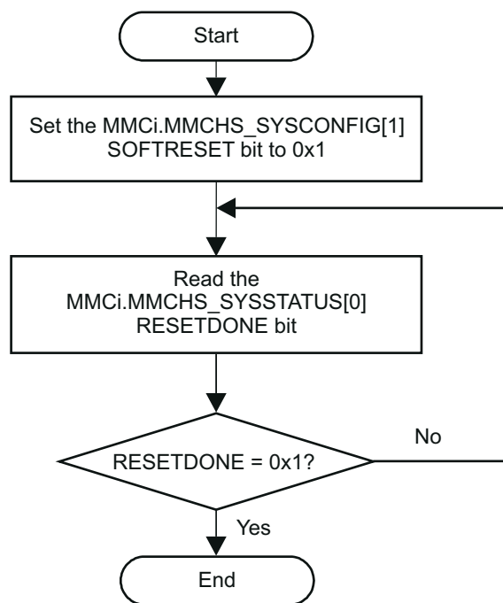
Figure 27-34. eMMC/SD/SDIO Controller Software Reset Flow
