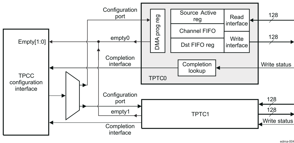
Figure 18-17. TPTC Block Diagram
