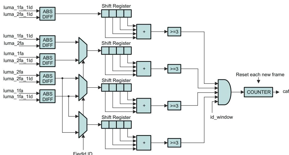
Figure 12-15. Film Mode Detection (FMD) Combing Artifacts Calculation
