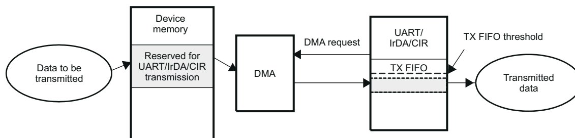
Figure 26-67. DMA Transmission
