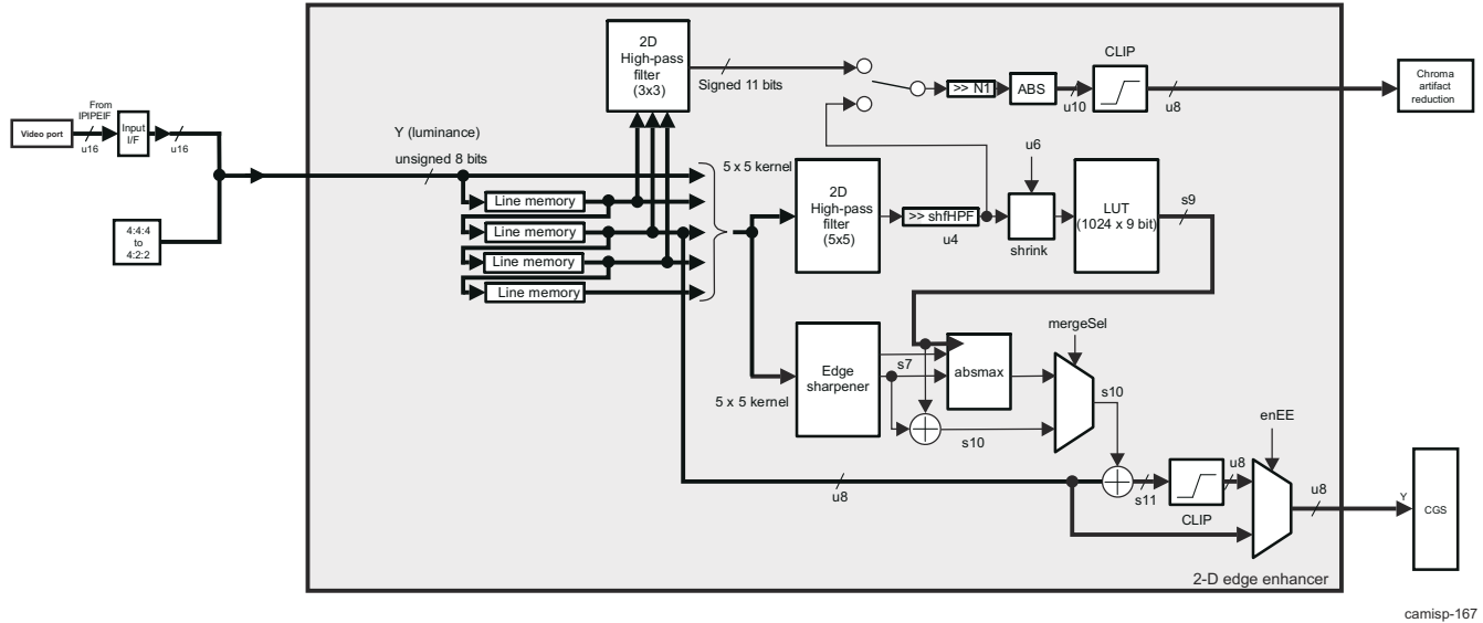
Figure 9-82. ISS ISP IPIPE 2D Edge-Enhancer Block Diagram
