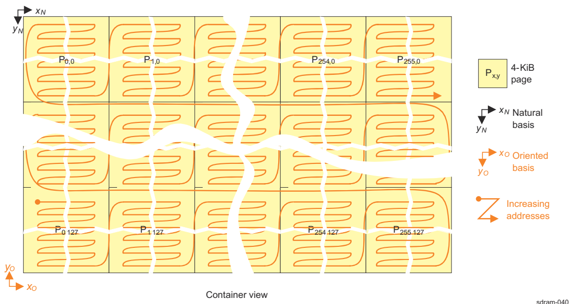
Figure 17-26. Page Mode Ordering of Elements in 0-Degree View With Horizontal Mirror
