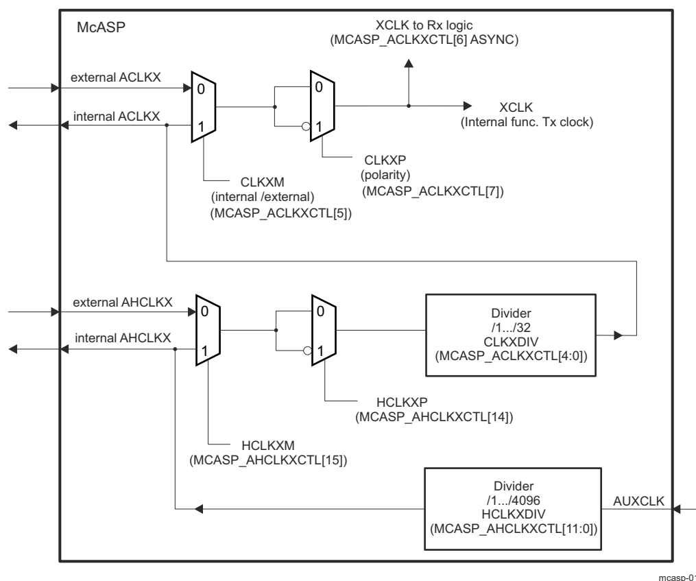
Figure 26-120. Transmit Clock Generator Block Diagram
