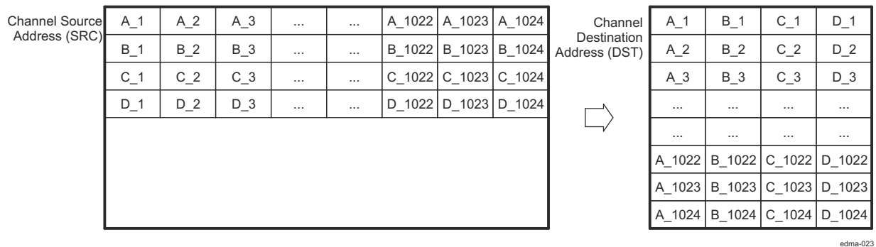
Figure 18-37. Data Sorting Example
