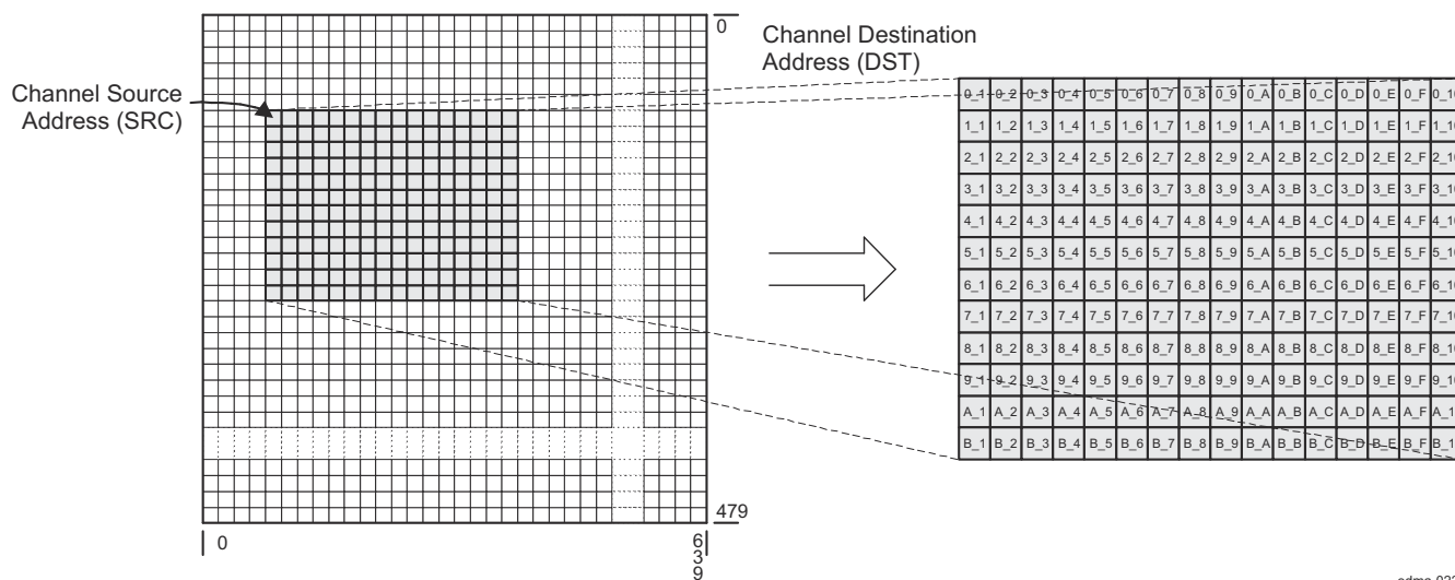
Figure 18-35. Subframe Extraction Transfer
