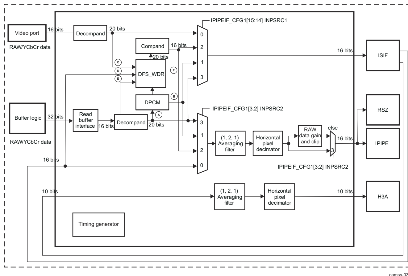
Figure 9-37. ISS ISP IPIPEIF Top-Level Block Diagram
