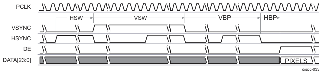
Figure 13-28. DISPC Active Matrix Timing Diagram of Configuration 1 (Start of Frame)
