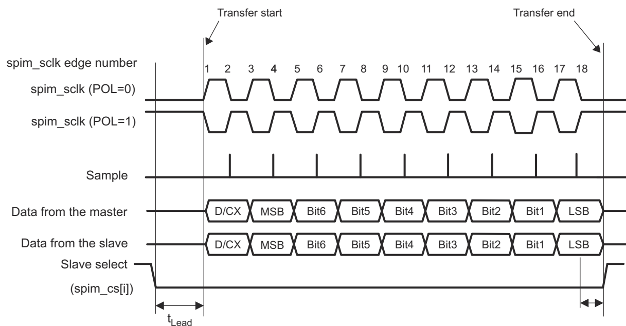
Figure 26-77. Extended SPI Transfer With a Start-Bit (SBE = 1)
