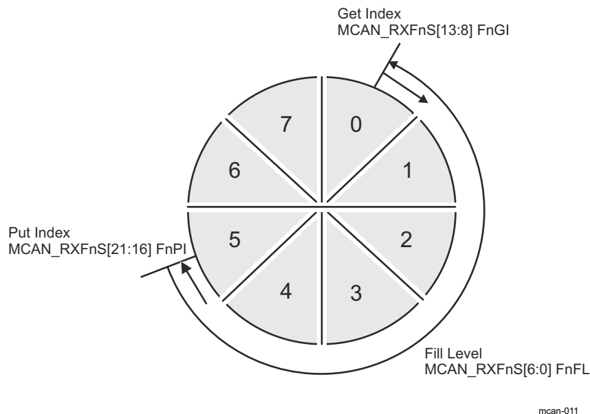
Figure 26-197. Rx FIFO Status
