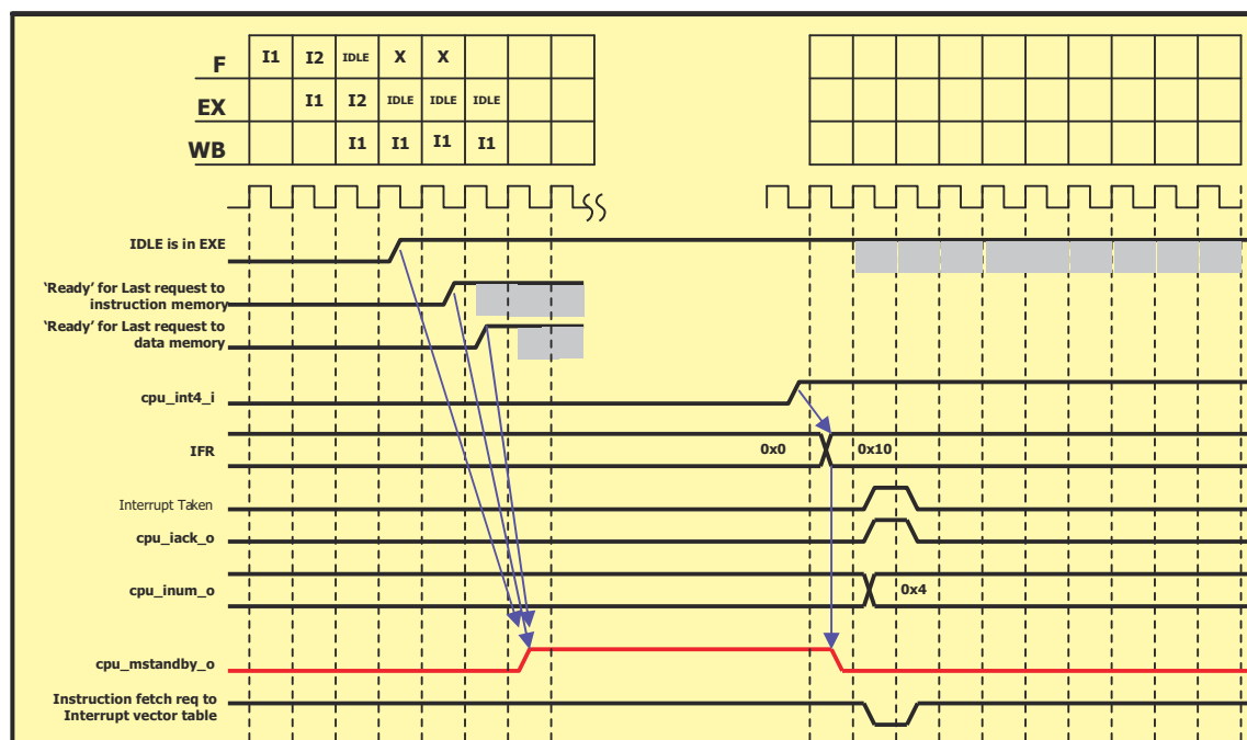
Figure A-57. CPU Standby and Wakeup Procedure
