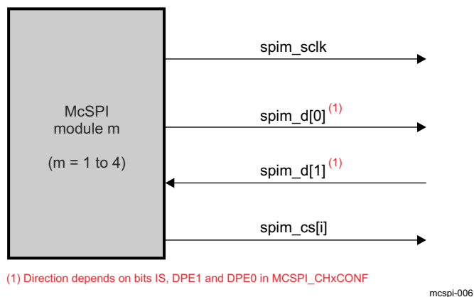
Figure 26-73. McSPI Interface Signals in Master Mode
