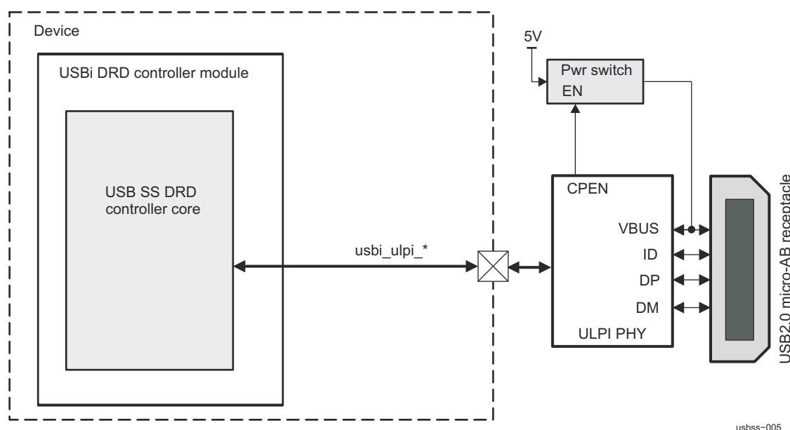
Figure 26-149. SuperSpeed USB Controller Application: USB2.0 DRD (ULPI PHY)
