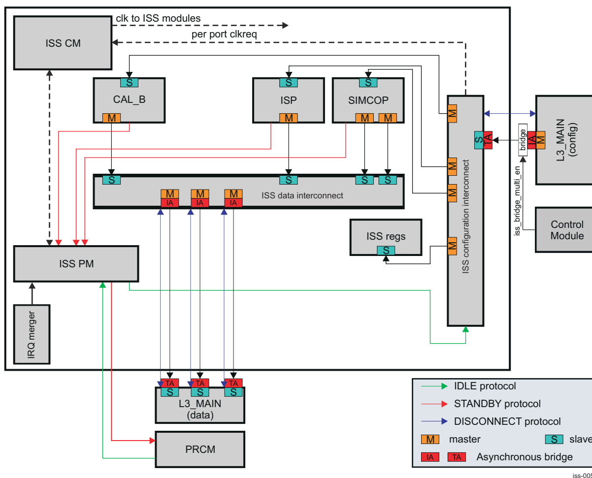
Figure 9-6. ISS Power Management
