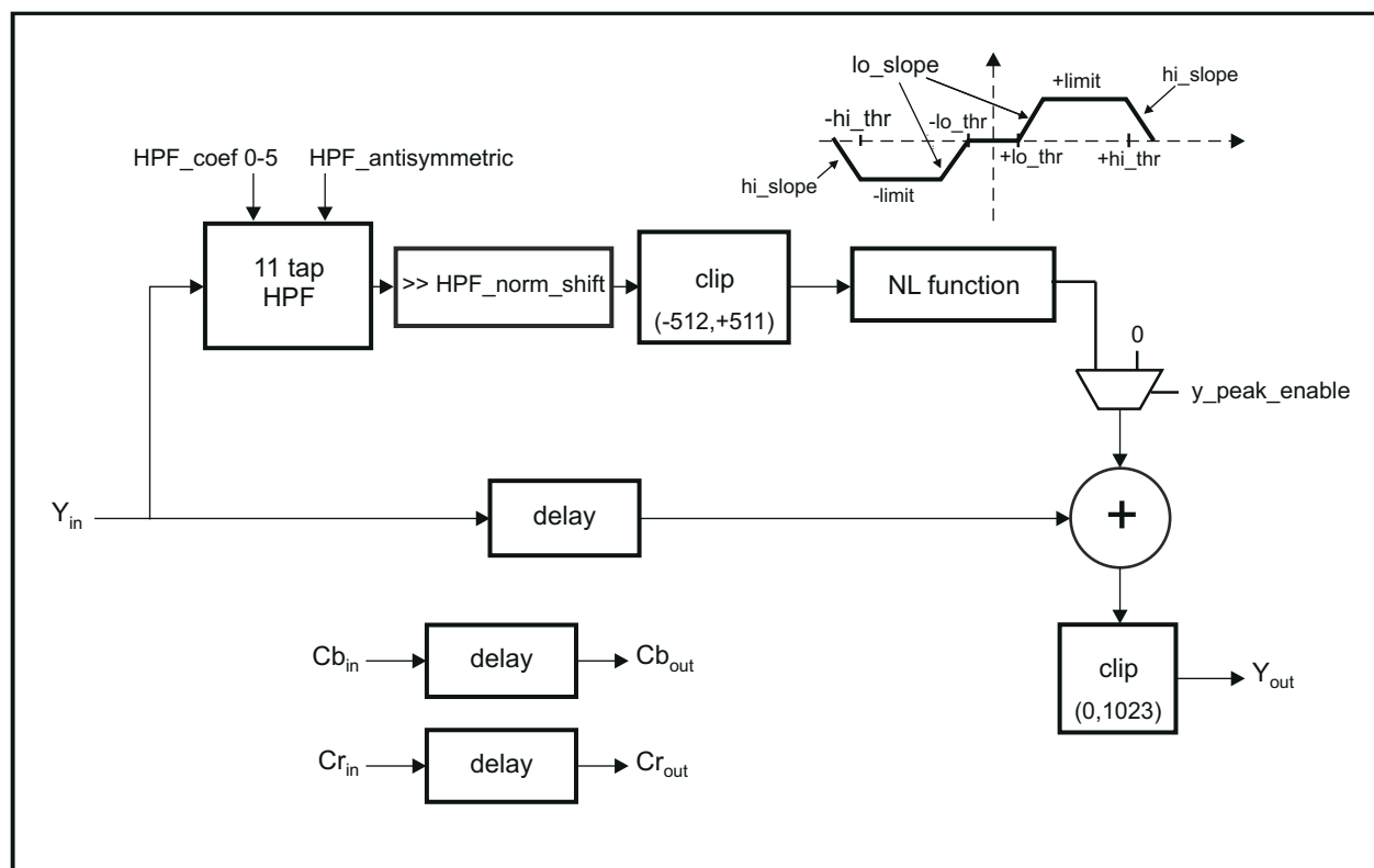
Figure 12-21. Filter Implementation and Parameter Description
