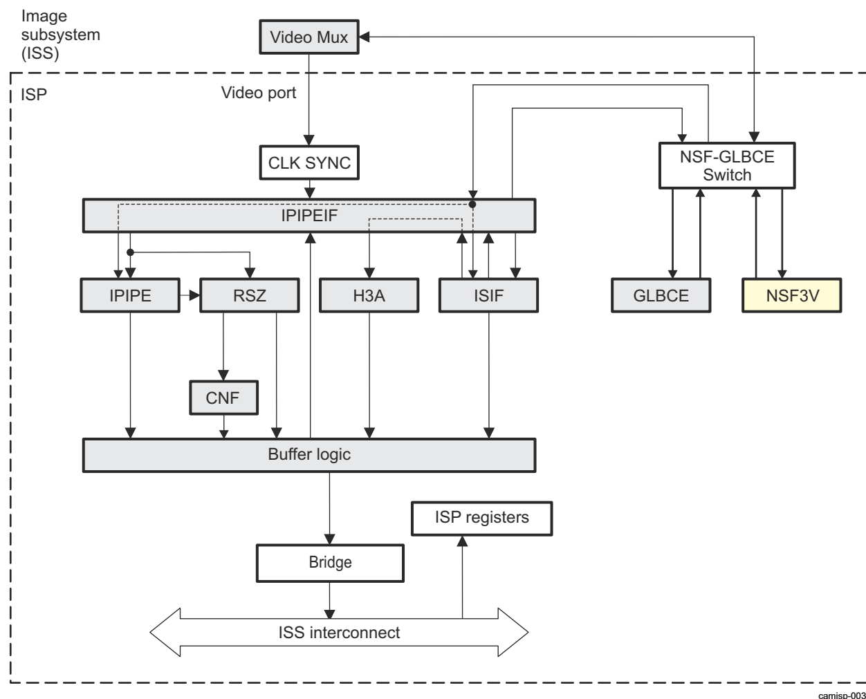
Figure 9-34. ISS ISP NSF3V High-Level Diagram
