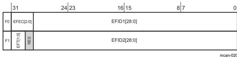
Figure 26-206. Extended Message ID Filter Element Structure
