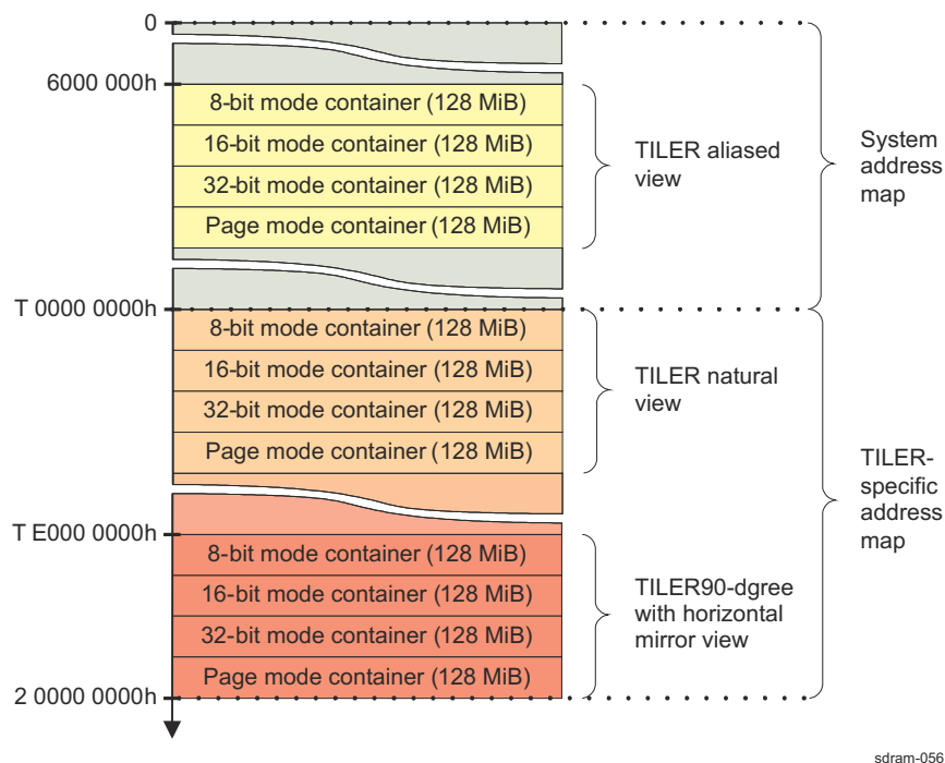
Figure 17-37. TILER Port Address Map
