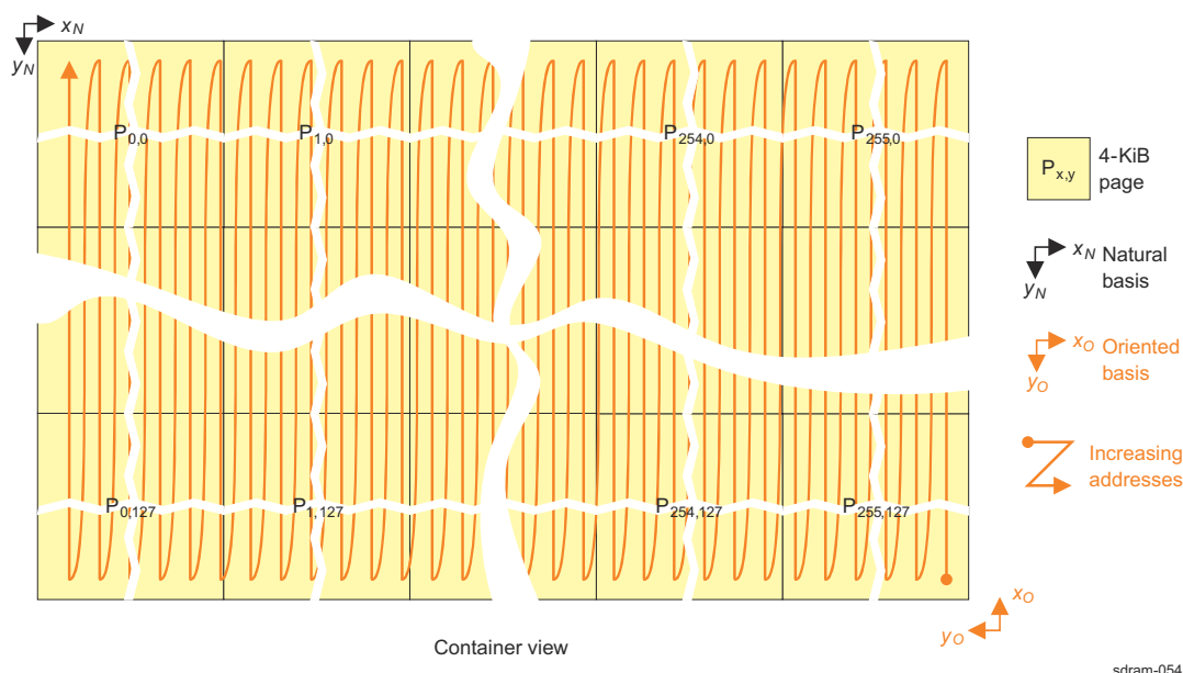
Figure 17-35. Tiled Mode Ordering of Elements in 90-Degree View With Horizontal Mirror
