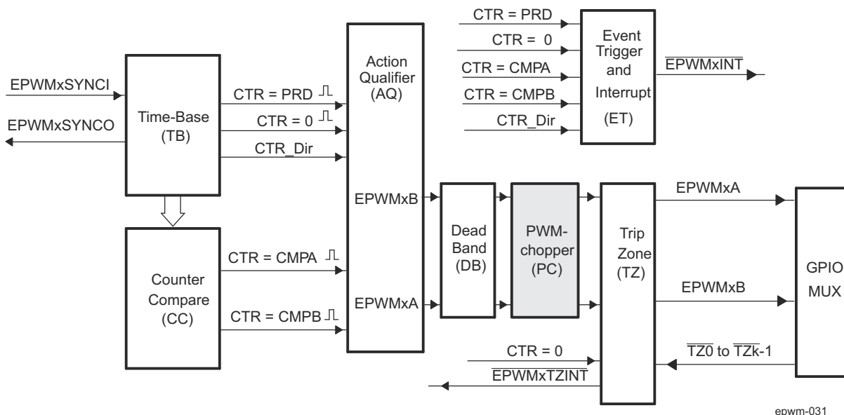
Figure 31-35. PWM-Chopper Submodule
