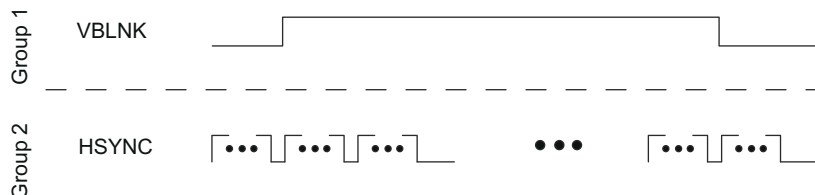
Figure 11-62. VBLNK and HSYNC
