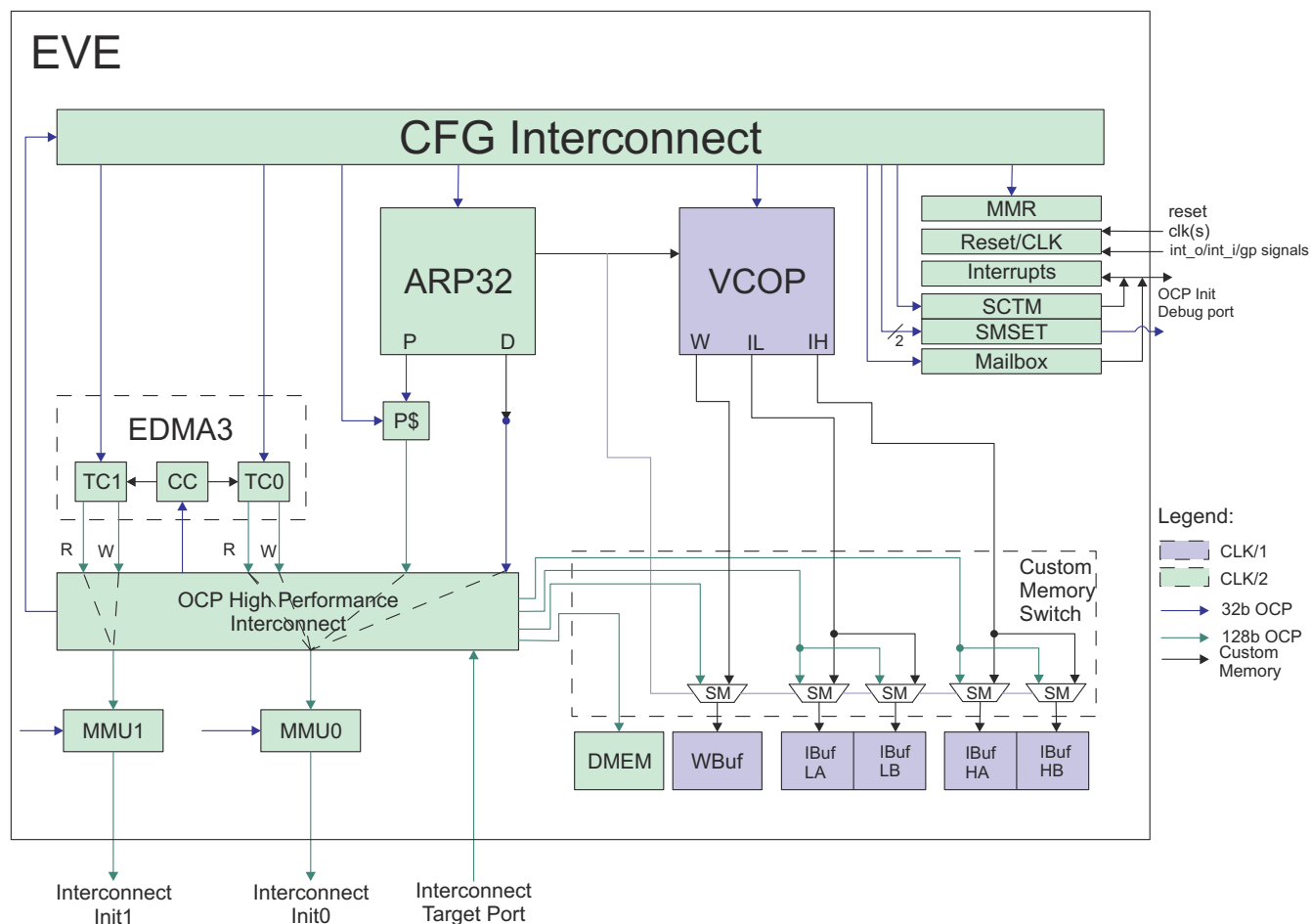
Figure 8-58. EVE Block Diagram
