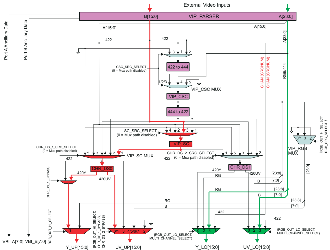
Figure 11-8. Input: A=RGB, B=YUV422; Output: A=RGB, B=Scaled YUV420
