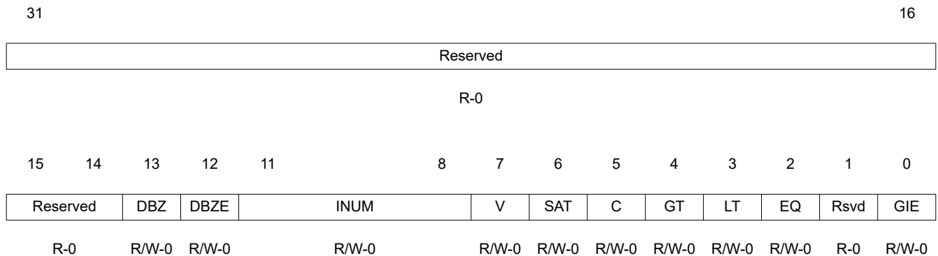
Figure 8-48. Shadow Control Status Register (SCSR)
