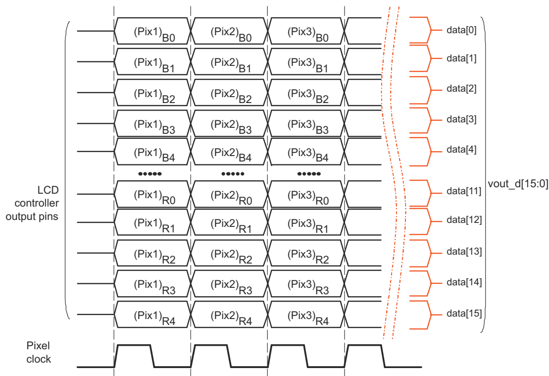
Figure 13-25. DISPC LCD Pixel Data Color16 Active Matrix
