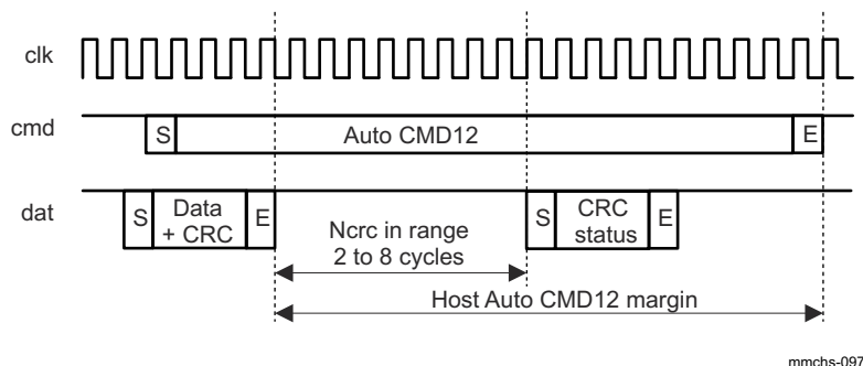
Figure 27-28. Auto CMD12 Timings During Write Transfer
