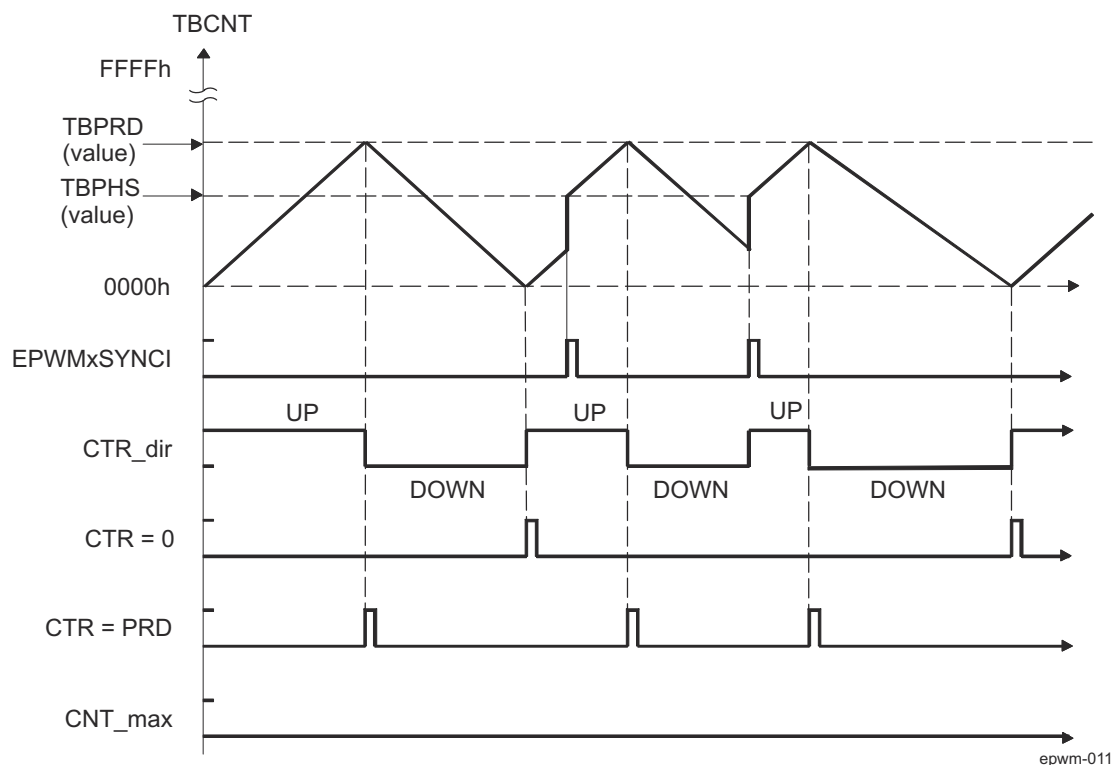
Figure 31-15. ePWM Time-Base Up-Down Count Waveforms, EPWM_TBCTL[13] PHSDIR = 1 Count Up on Synchronization Event
