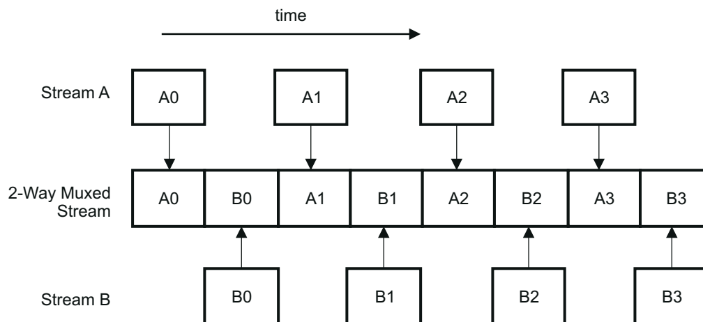
Figure 11-47. 2-Way Multiplexing
