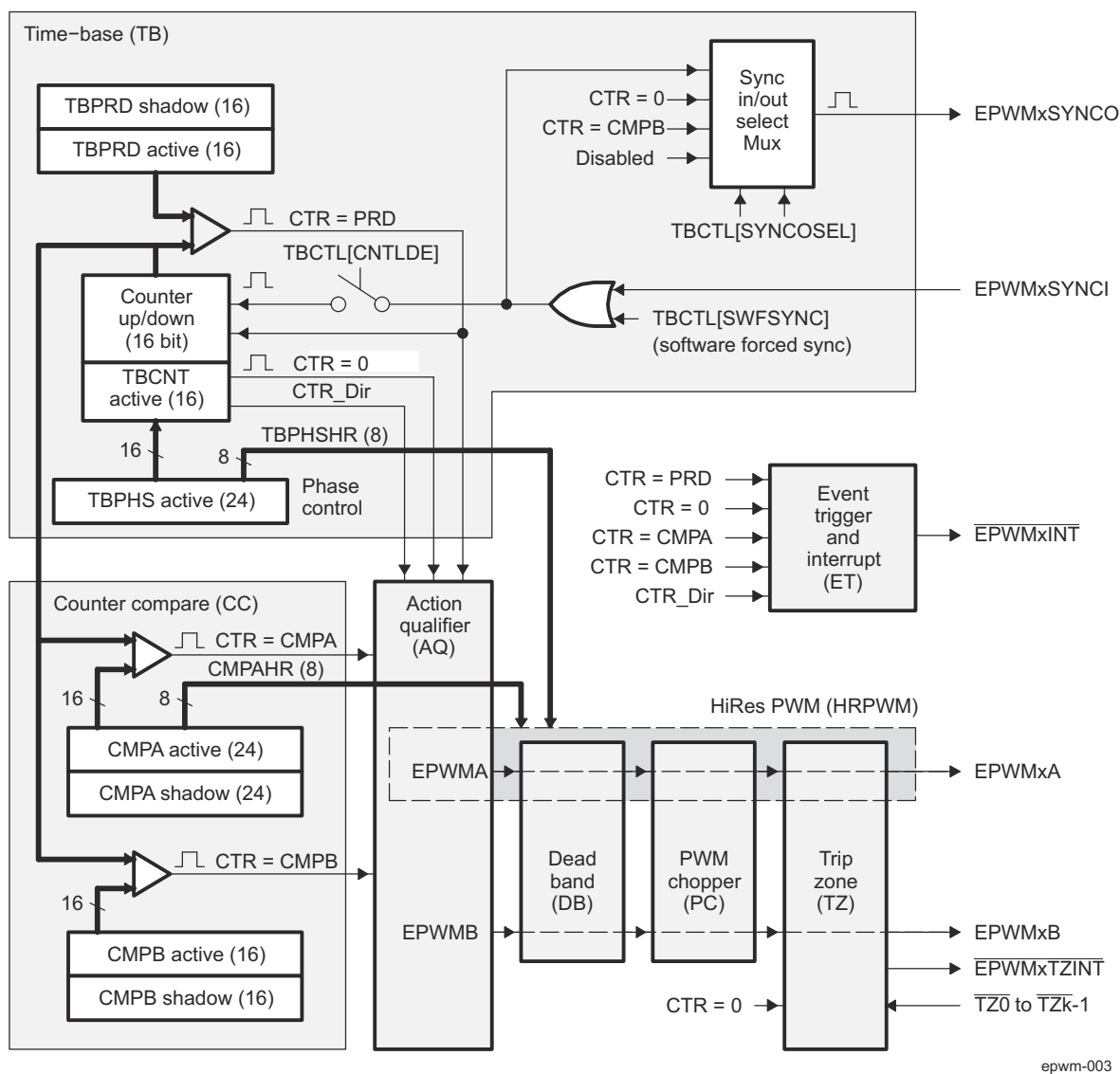
Figure 31-7. ePWM Submodules and Critical Internal Signal Interconnects
