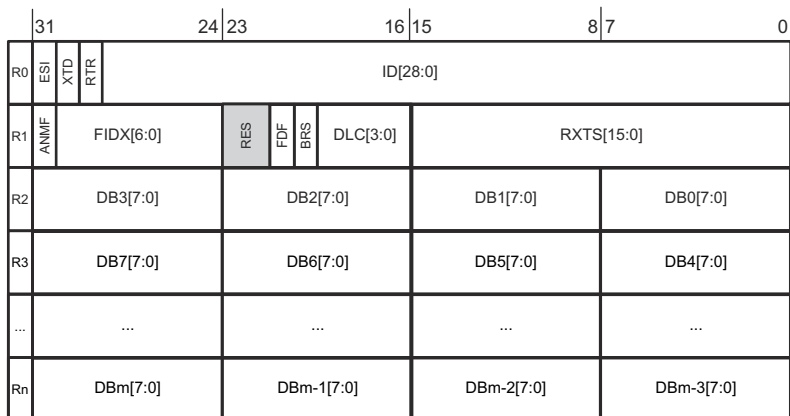
Figure 26-202. Rx Buffer/Rx FIFO Element Structure
