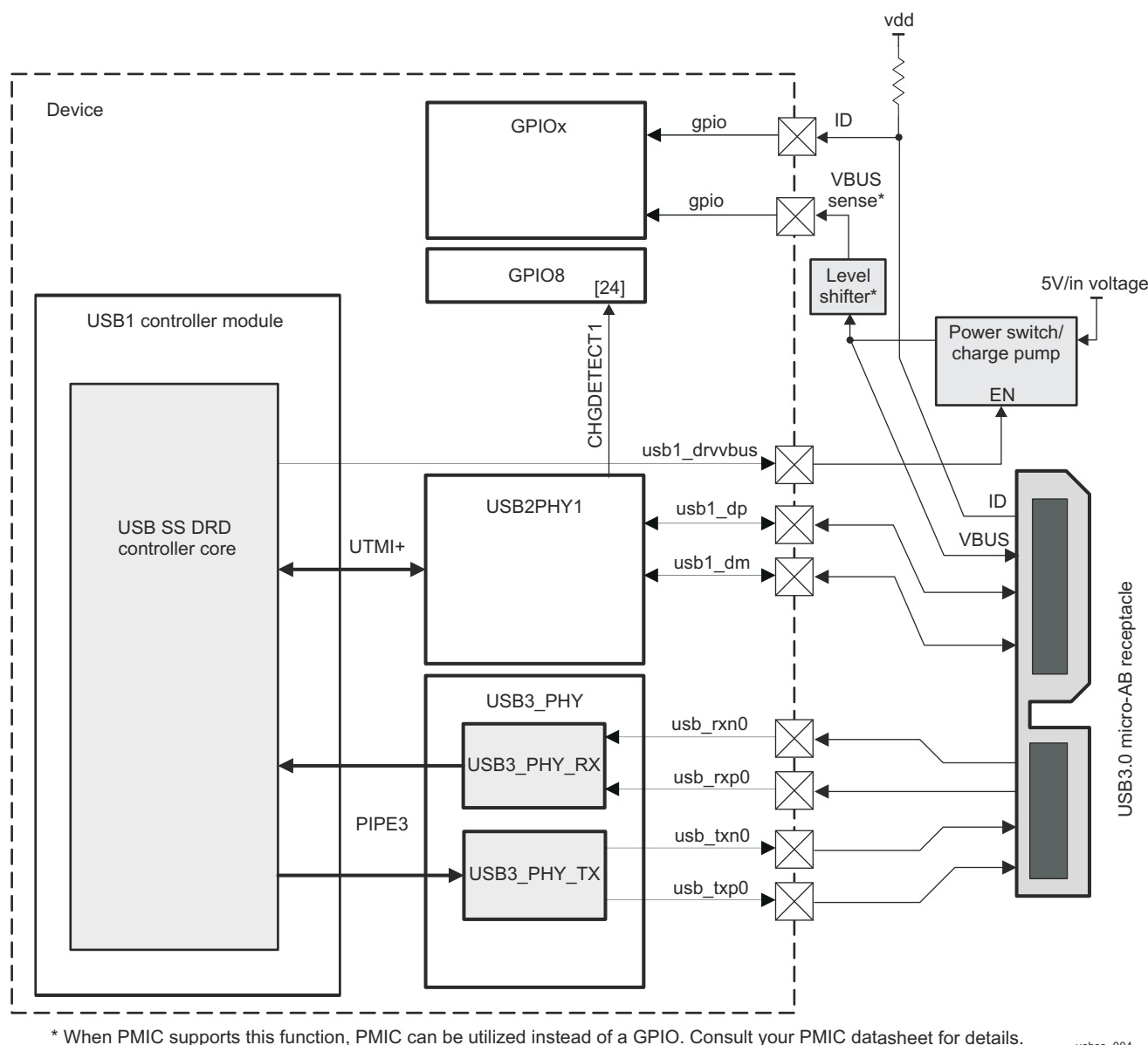
Figure 26-147. SuperSpeed USB Controller Application: USB3.0 DRD
