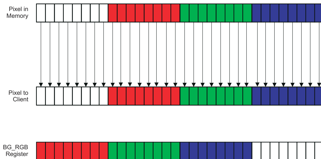
Figure 12-77. ARGB32-8888 (Data Type 7)
