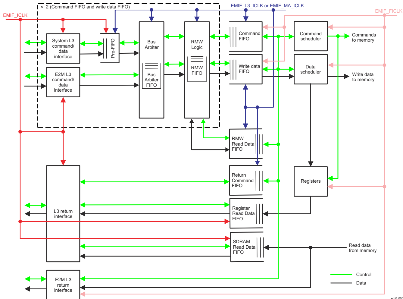
Figure 17-50. FIFO Block Diagram
