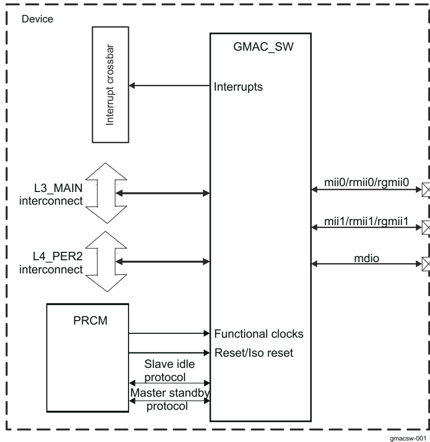
Figure 26-207. GMAC_SW Overview
