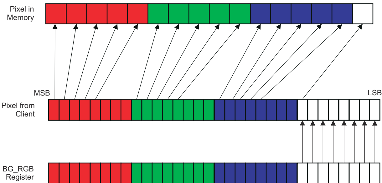
Figure 12-63. RGBA-5551 (Data Type 3)
