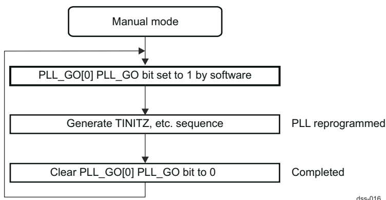
Figure 13-14. VIDEO PLL Go Sequence (Manual Mode)
