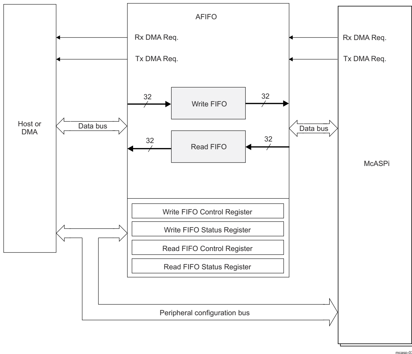
Figure 26-131. McASP Audio FIFO (AFIFO) Block Diagram
