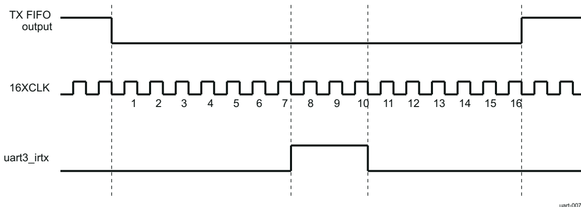
Figure 26-42. IrDA SIR Encoding Mechanism
