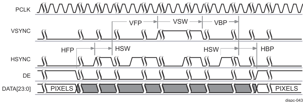
Figure 13-38. DISPC Active Matrix Timing Diagram of Configuration 3 (Between Frames)
