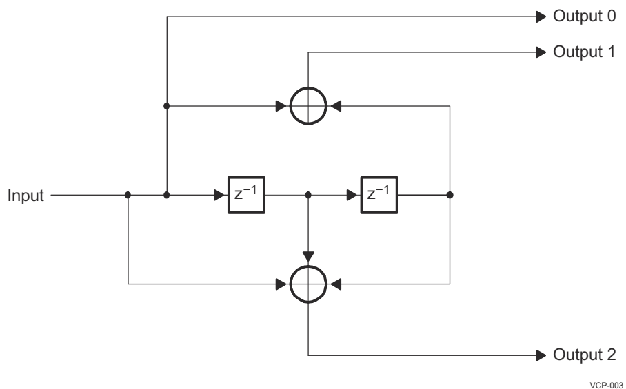
Figure 32-4. Convolutional Encoder Example Block Diagram
