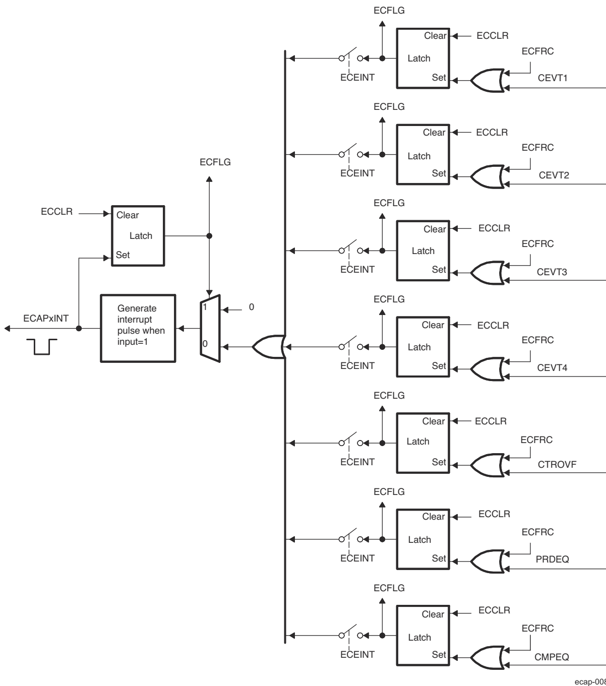
Figure 31-60. Interrupts in eCAP Module
