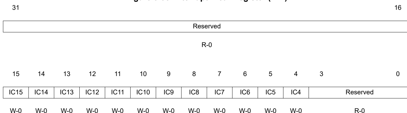
Figure 8-35. Interrupt Clear Register (ICR)
