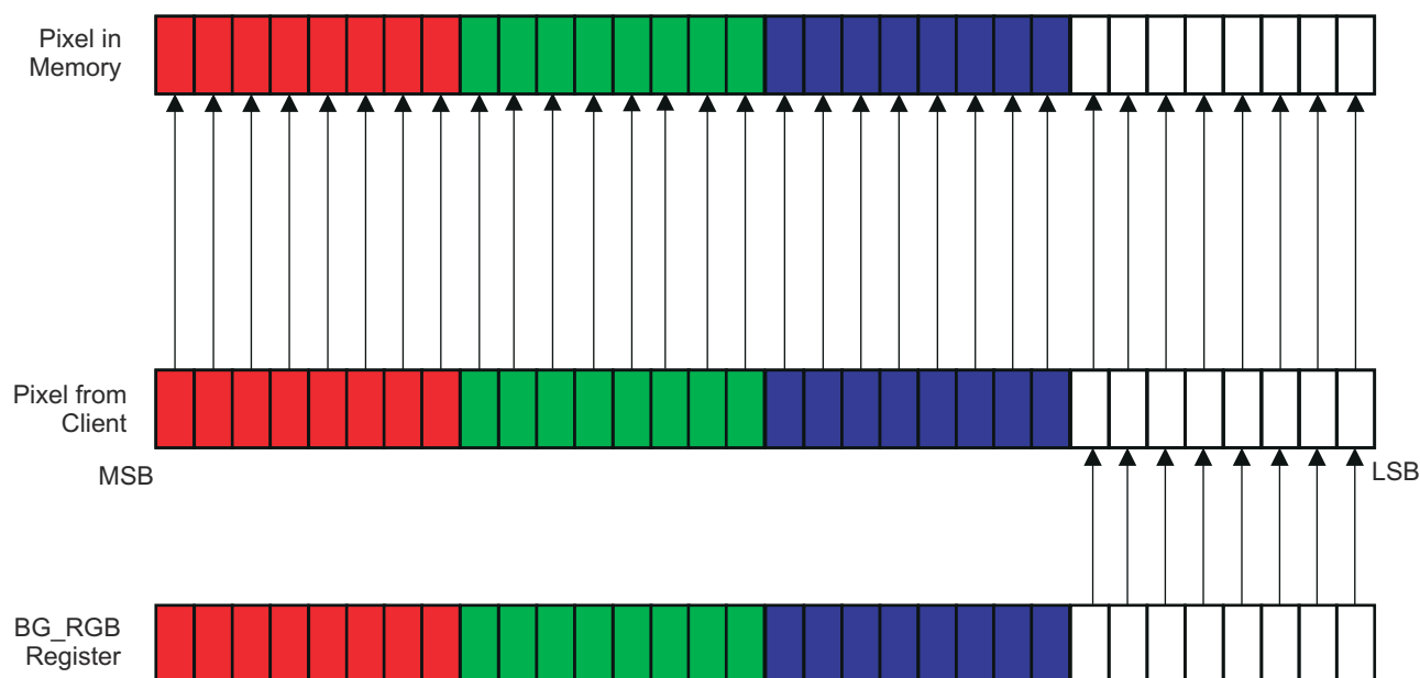
Figure 12-69. RGBA32-8888 (Data Type 9)
