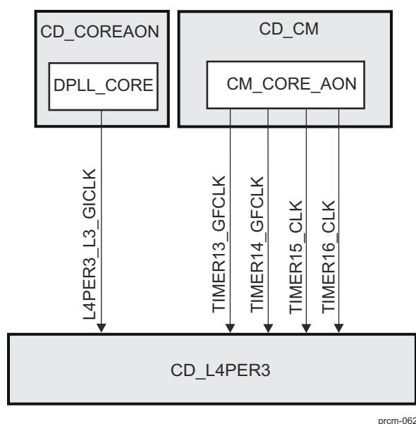
Figure 3-72. CD_L4PER3 Overview
