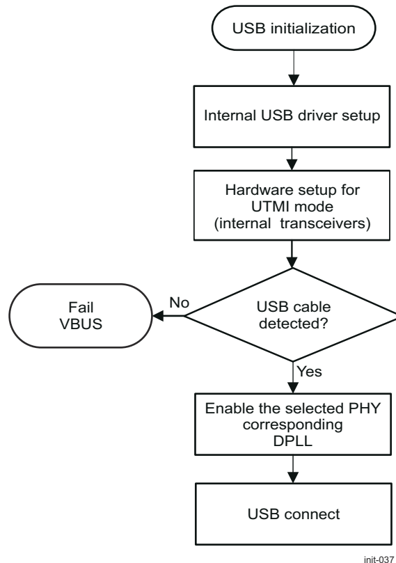
Figure 34-12. USB Initialization Procedure
