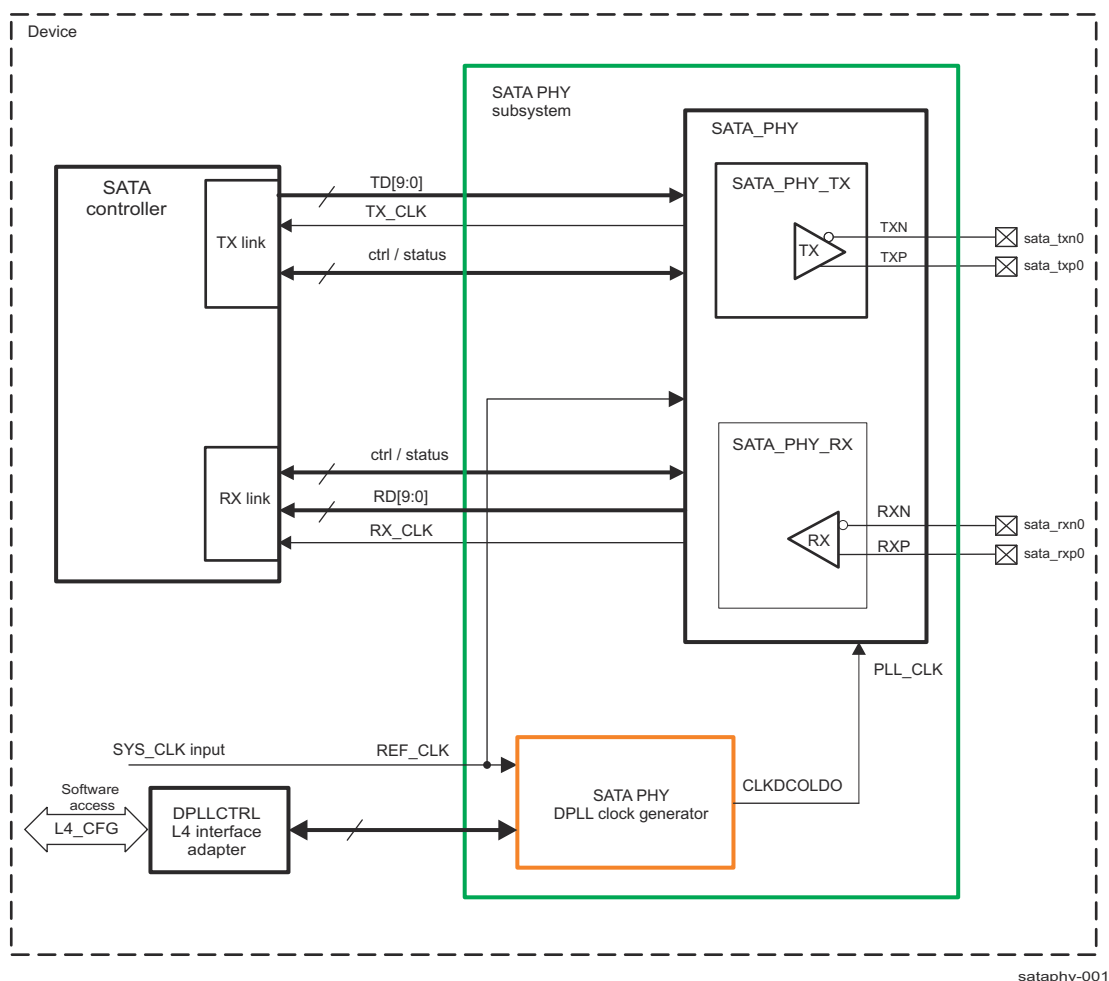
Figure 28-1. SATA PHY Subsystem Overview
