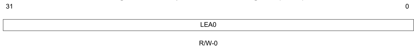
Figure 8-42. Loop 0 End Address Register (LEA0)
