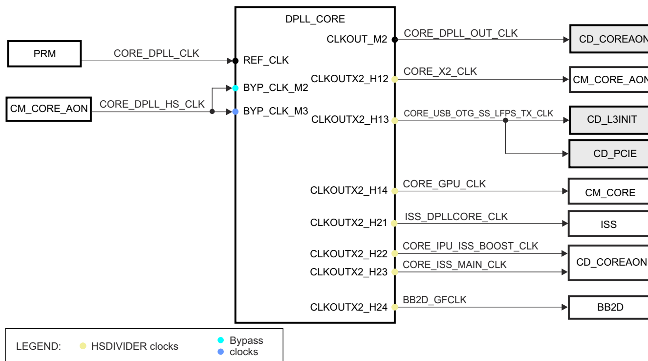
Figure 3-53. DPLL_CORE Overview
