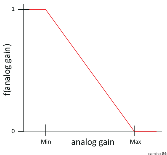
Figure 9-33. ISS ISP GLBCE Iridix f(\text{analog gain}) function
