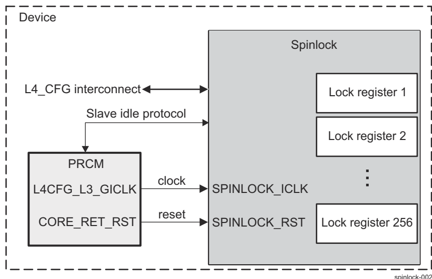
Figure 23-2. Spinlock Integration
