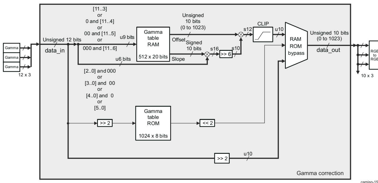
Figure 9-70. ISS ISP IPIPE Gamma Correction Module Block Diagram
