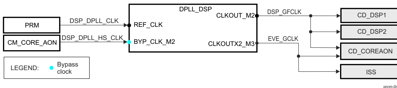
Figure 3-59. DPLL_DSP Overview
