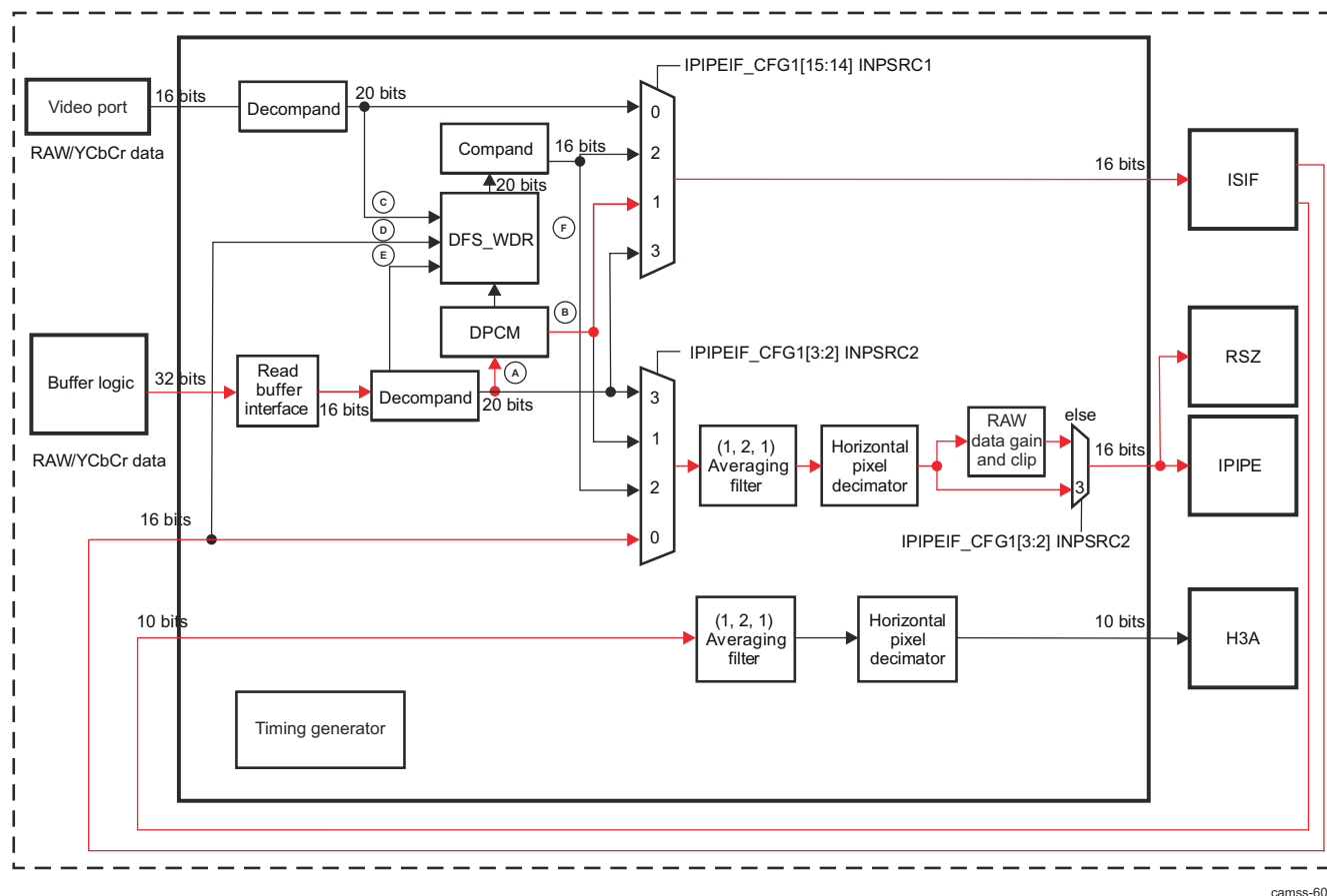
Figure 9-46. ISS ISP IPIPEIF INPSRC1 = 1 and INPSRC2 = 0 Data Path
