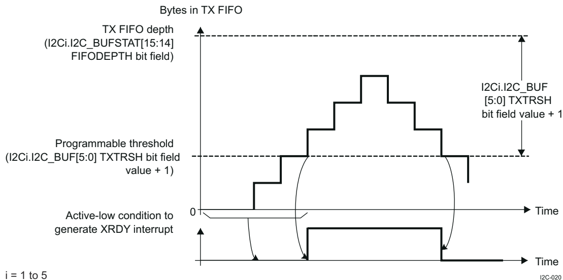
Figure 26-15. HS I 2 C Transmit FIFO Interrupt Request Generation
