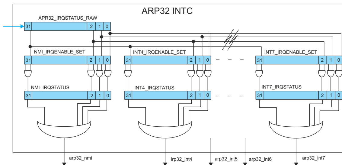
Figure 8-19. EVE INTC for ARP32
