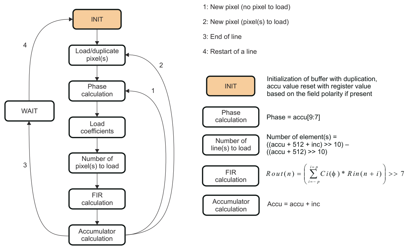
Figure 13-65. DISPC Horizontal Up/Downsampling Algorithm
