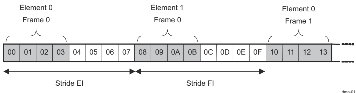
Figure 18-6. Example Showing Double-Index Addressing, Elements, Frames, and Strides
