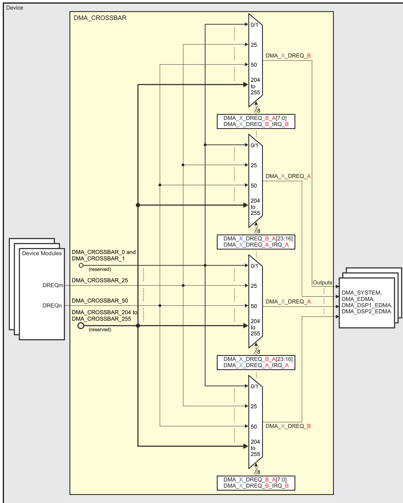
Figure 20-11. DMA_CROSSBAR Module Functional Diagram
