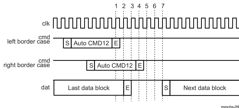
Figure 27-29. Auto CMD12 Timings During Read Transfer
