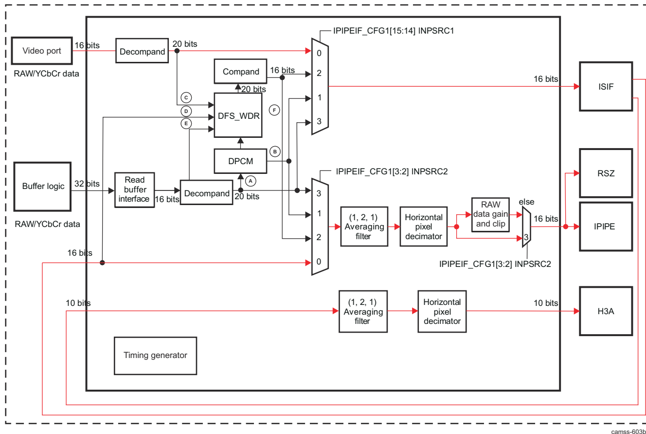
Figure 9-41. ISS ISP IPIPEIF INPSRC1 = 0 and INPSRC2 = 0 Data Path
