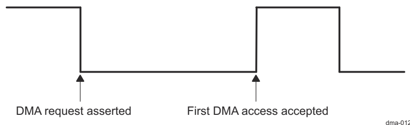
Figure 18-3. Transition-Sensitive DMA Request Scheme
