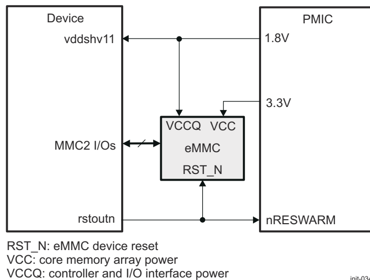
Figure 34-21. eMMC Connection
