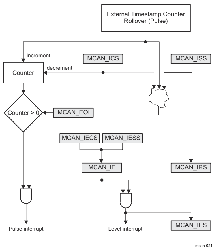
Figure 26-194. External Timestamp Counter Interrupt
