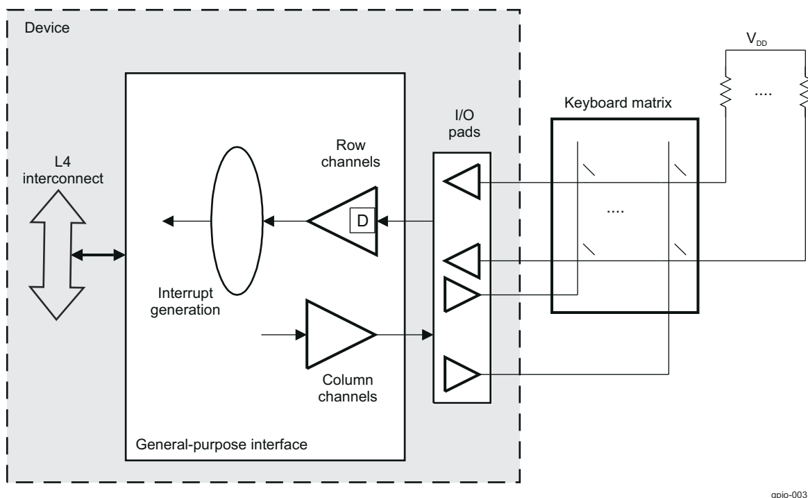
Figure 29-2. General-Purpose Interface Used as a Keyboard Interface
