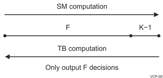
Figure 32-7. Tailed Traceback Mode
