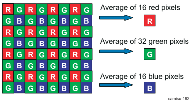
Figure 9-88. ISS ISP IPIPE Boxcar Operation (8 × 8 Block)
