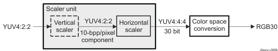
Figure 13-58. DISPC YUV4:2:2 to RGB30 Using Scaler Unit for Resampling Chrominance
