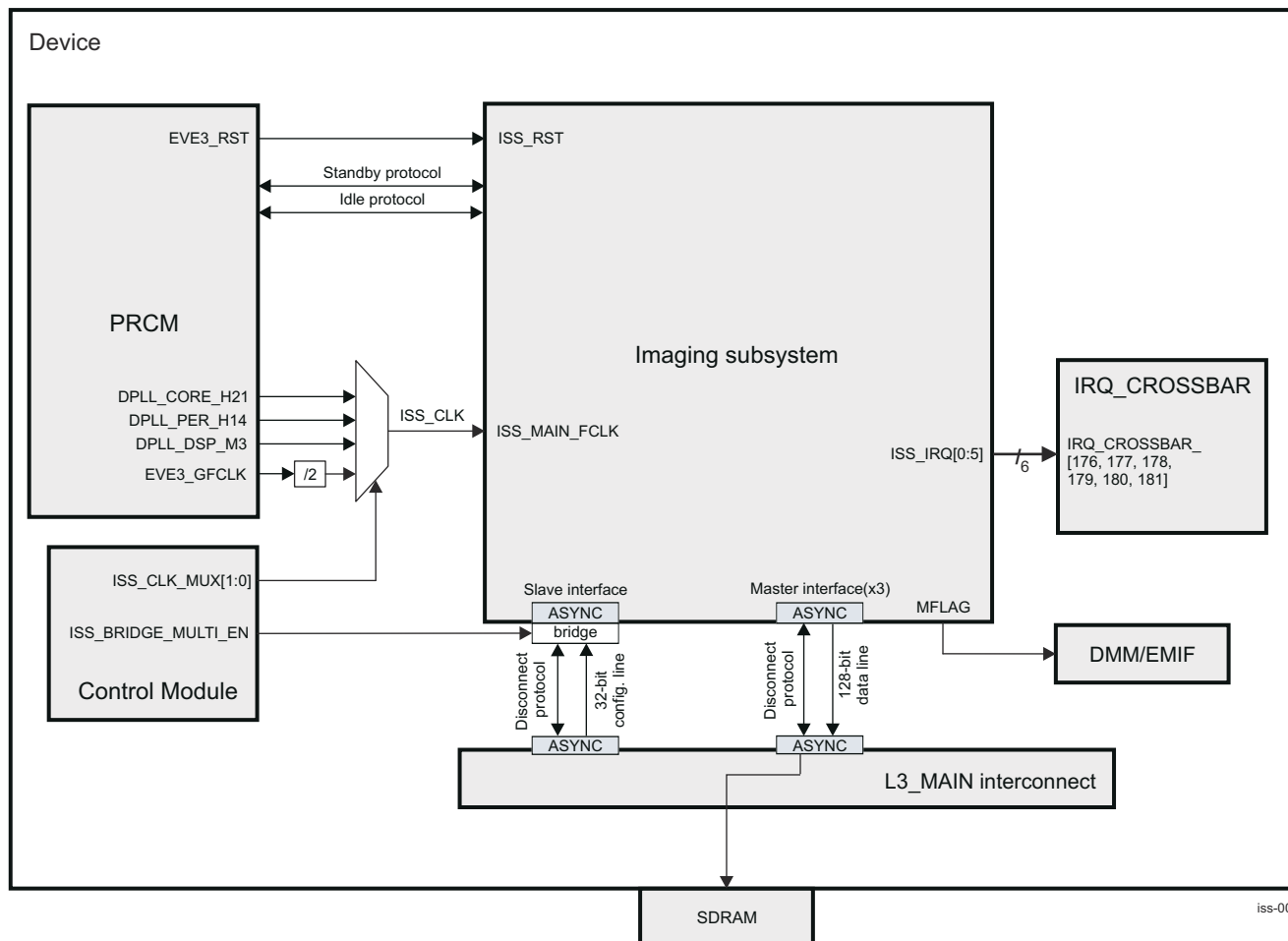
Figure 9-2. ISS Integration
