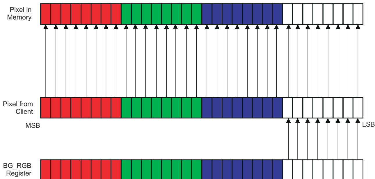
Figure 11-115. RGB32-8888 (Data Type 9)
