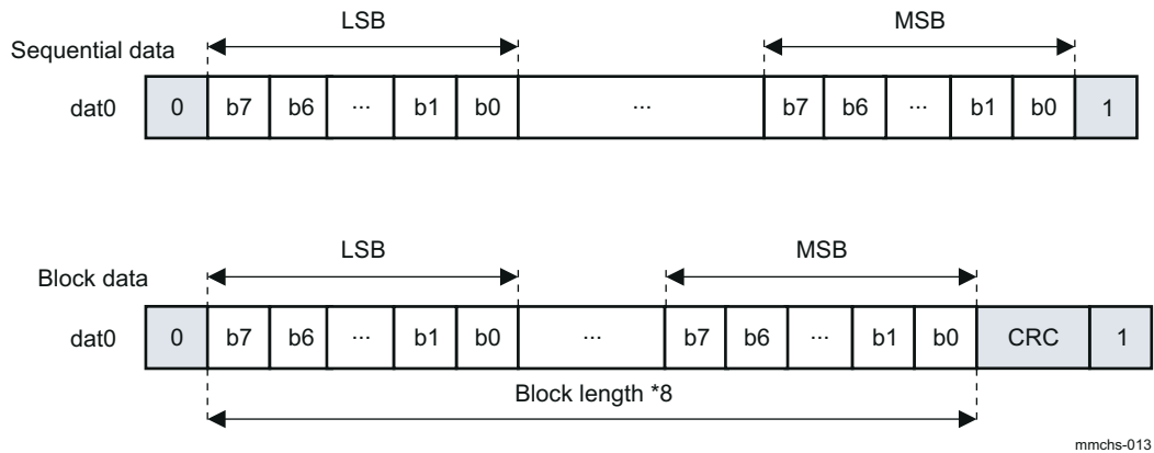
Figure 27-10. Data Token Format for 1-Bit Transfers
