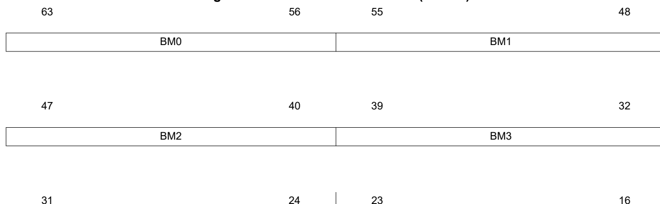
Figure 32-12. Data Source - EDMA (BM = 1)
