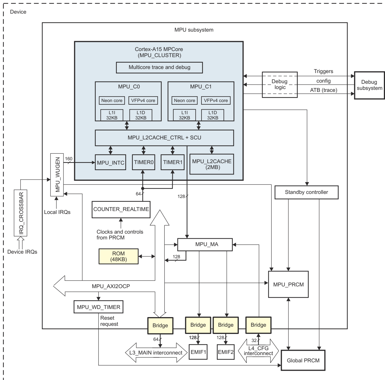
Figure 4-5. MPU Subsystem Block Diagram
