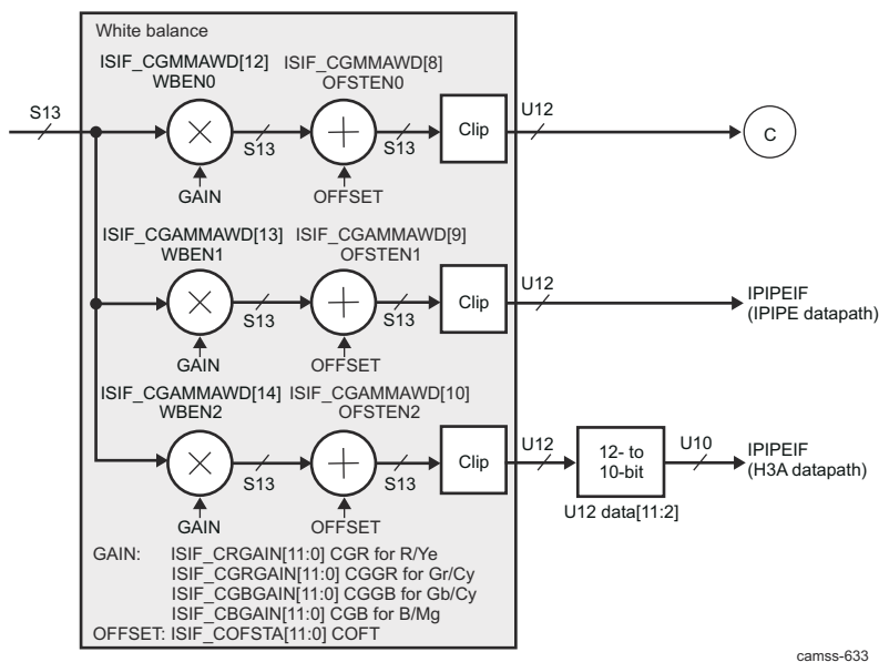
Figure 9-158. ISS ISP ISIF White Balance Block Diagram
