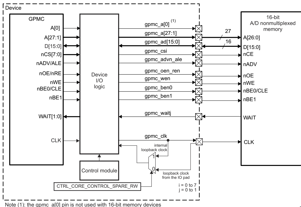
Figure 17-54. GPMC to 16-Bit Nonmultiplexed Memory
