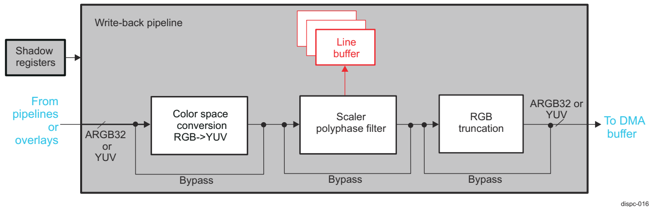
Figure 13-66. DISPC Write-Back Pipeline
