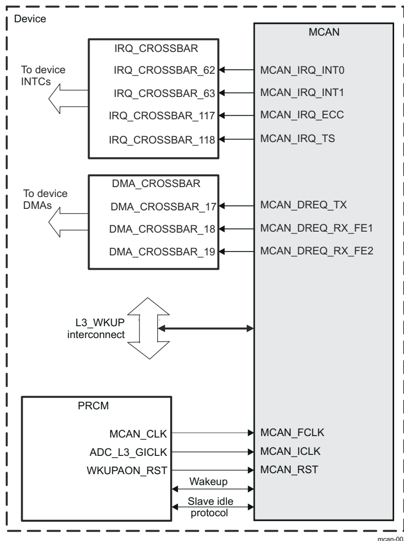
Figure 26-188. MCAN Integration
