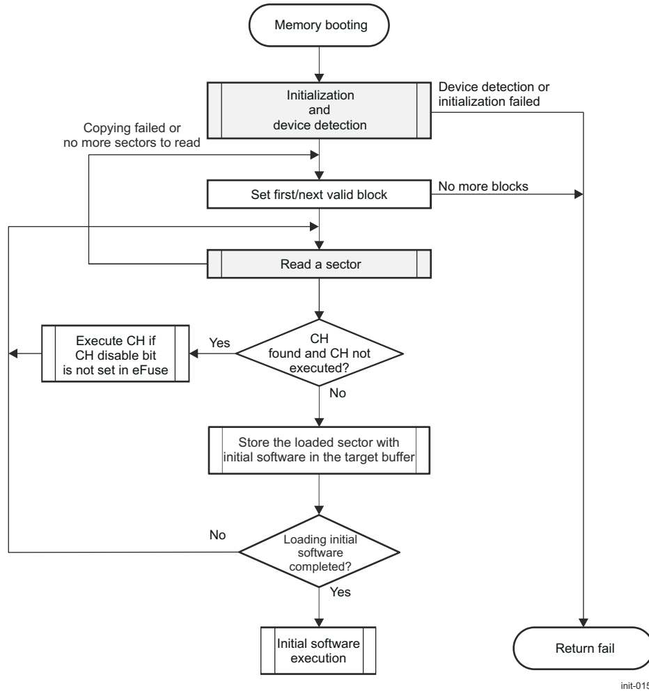
Figure 34-16. Image Shadowing
