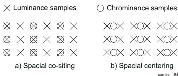
Figure 9-76. ISS ISP IPIPE Chroma Subsampling Position
