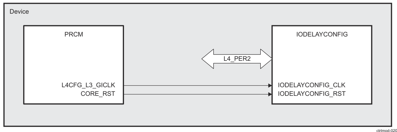
Figure 20-15. IODELAYCONFIG Integration
