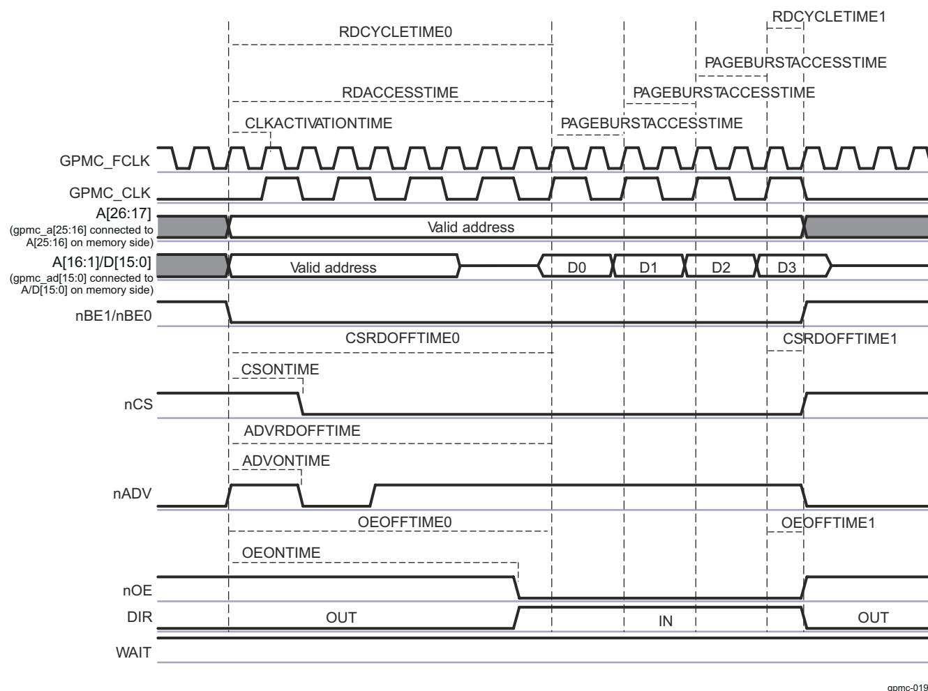
Figure 17-73. Synchronous Multiple (Burst) Read (GPMCFCLKDIVIDER = 1)
