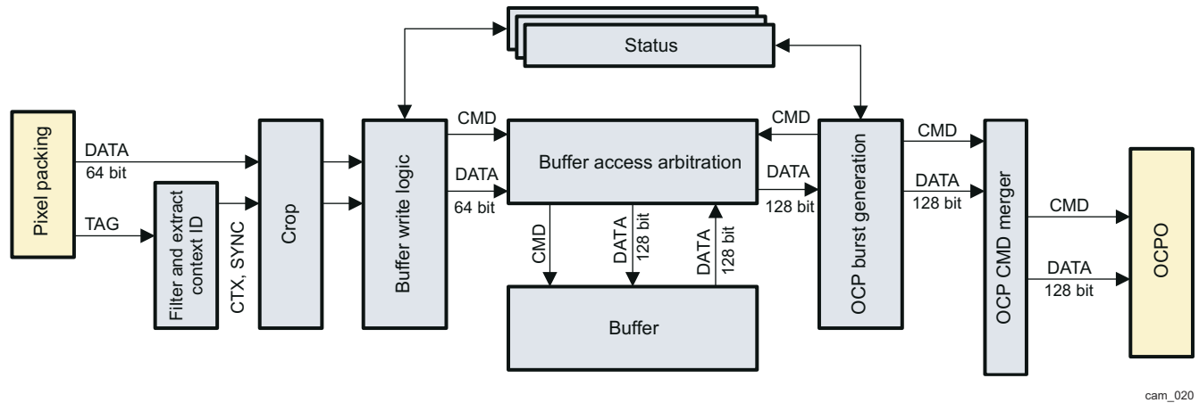
Figure 9-16. CAL Write DMA Block Diagram
