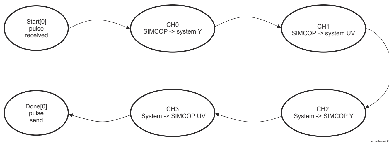
Figure 9-192. YUV4:2:0-NV12 Read/Write Chain
