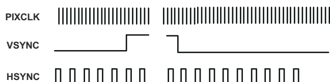
Figure 11-26. Discrete Sync Signals
