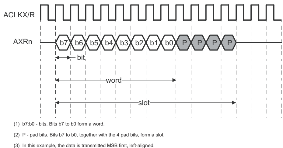
Figure 26-110. Definition of Bit, Word, and Slot
