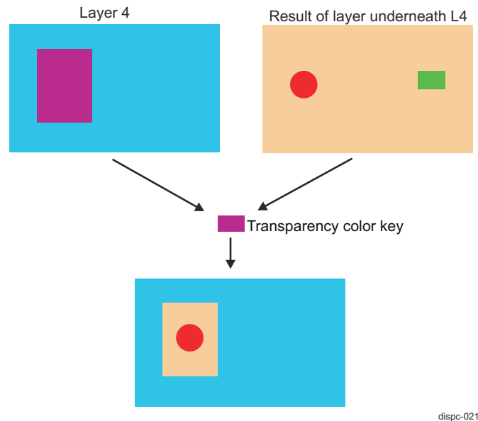
Figure 13-77. DISPC Source Transparency Color Key Example
