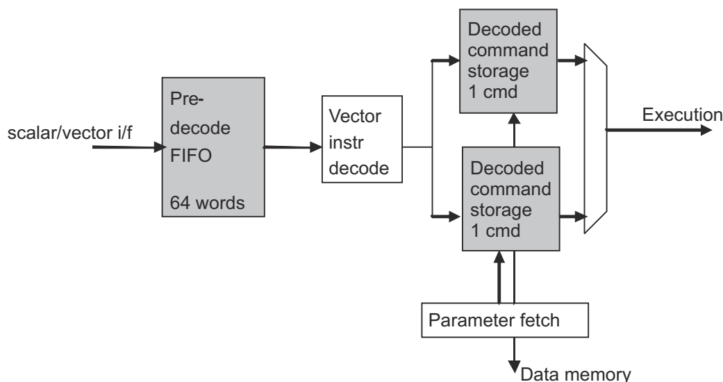
Figure 8-61. VCOP Instruction Buffering
