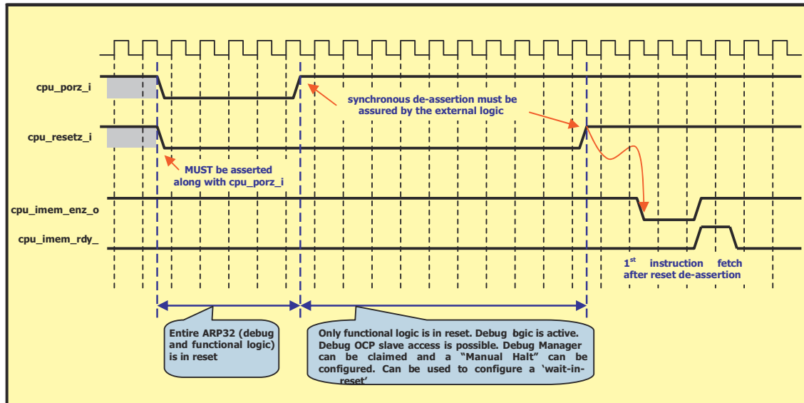
Figure A-56. Power-On-Reset
