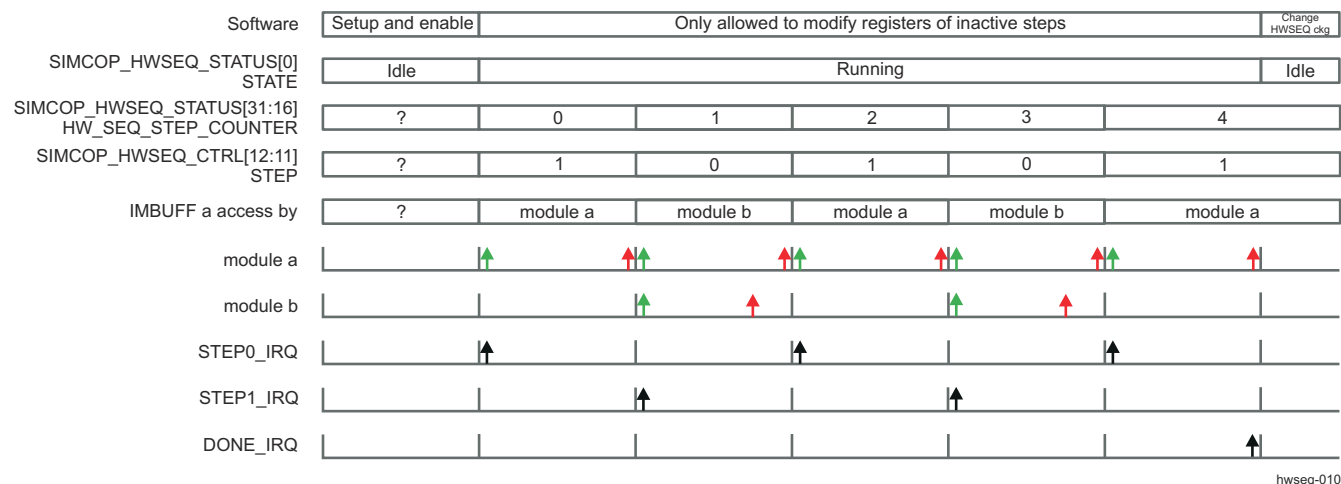
Figure 9-183. Hardware Sequencer Operation Example
