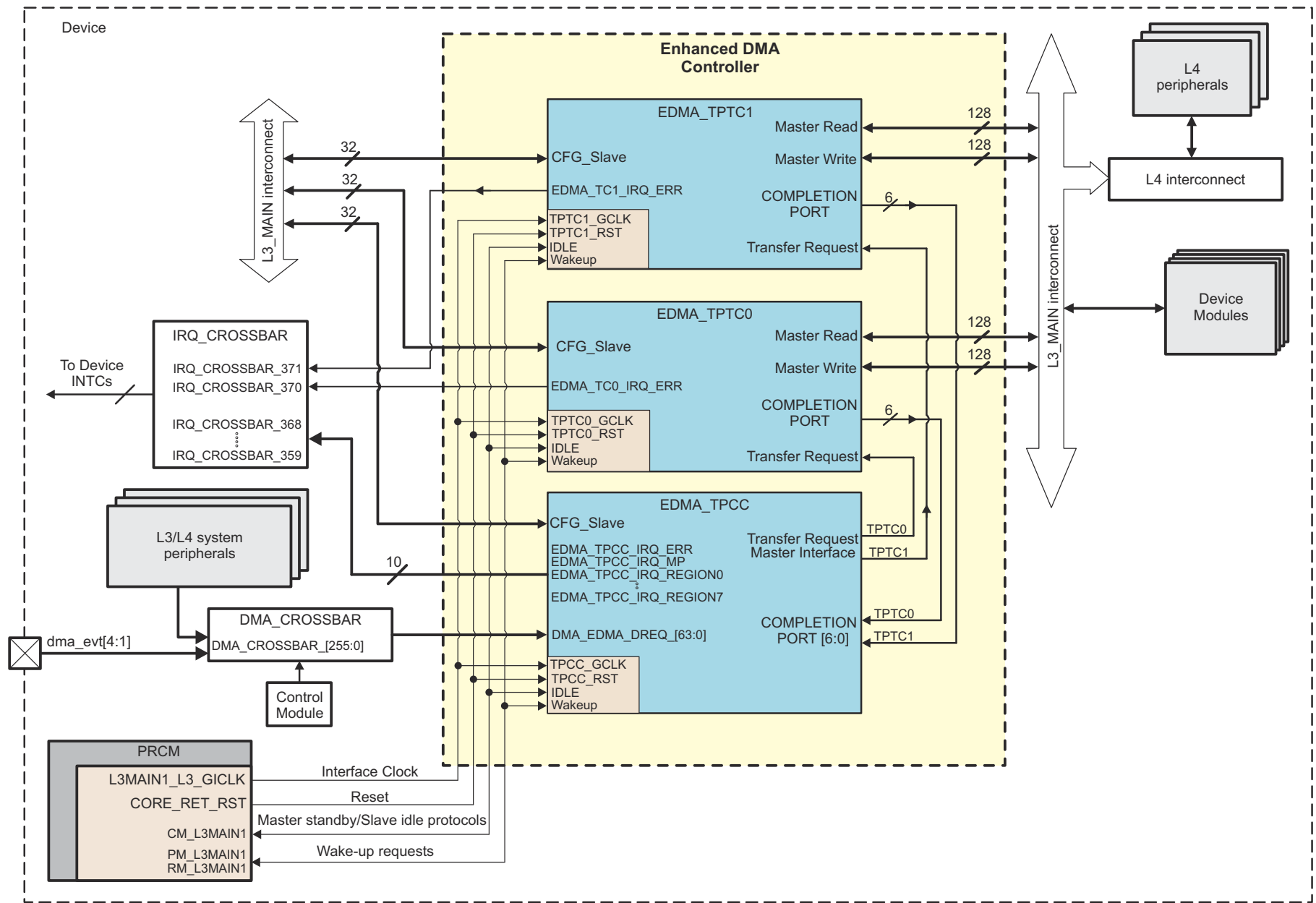
Figure 18-14. EDMA Controller Integration
