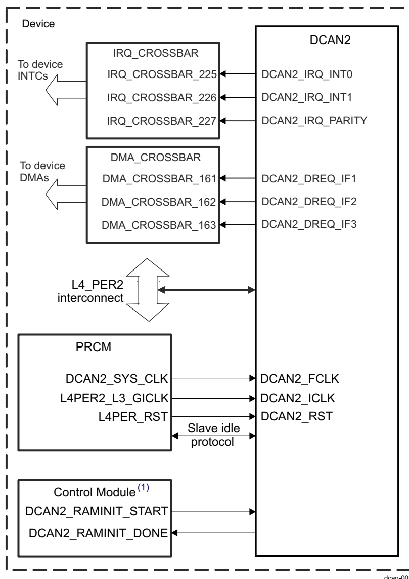
Figure 26-168. DCAN2 Integration
