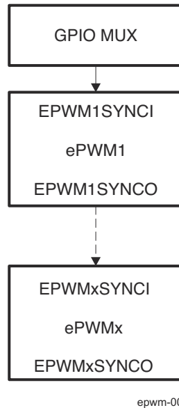
Figure 31-11. ePWM Time-Base Counter Synchronization Scheme 1
