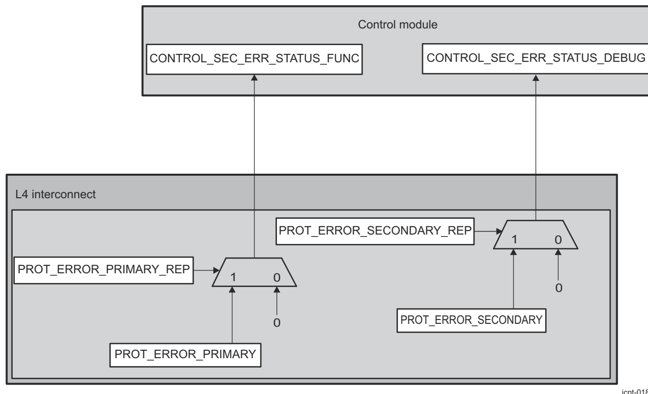
Figure 16-14. Protection Violation Out-of-Band Error Reporting
