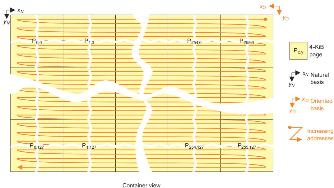
Figure 17-23. Tiled Mode Ordering of Elements in 0-Degree View With Vertical Mirror
