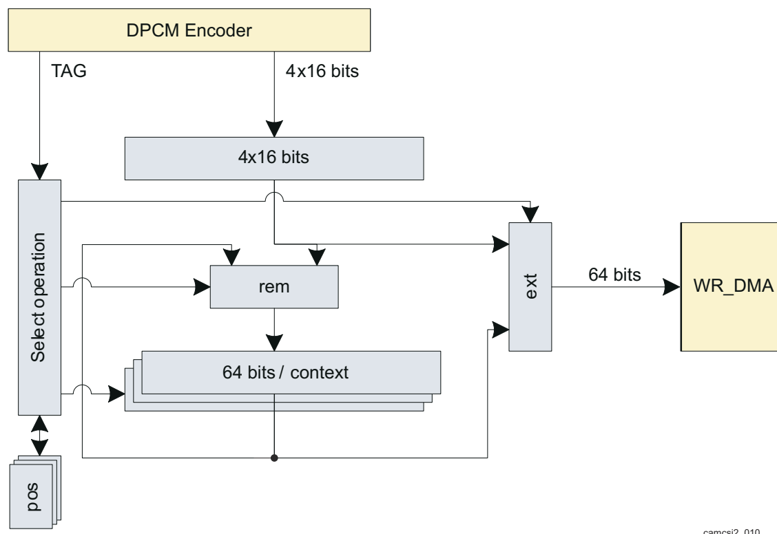
Figure 9-13. CAL Pixel Packing
