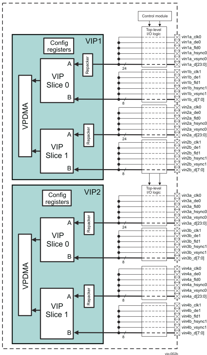
Figure 11-2. VIP Environment
