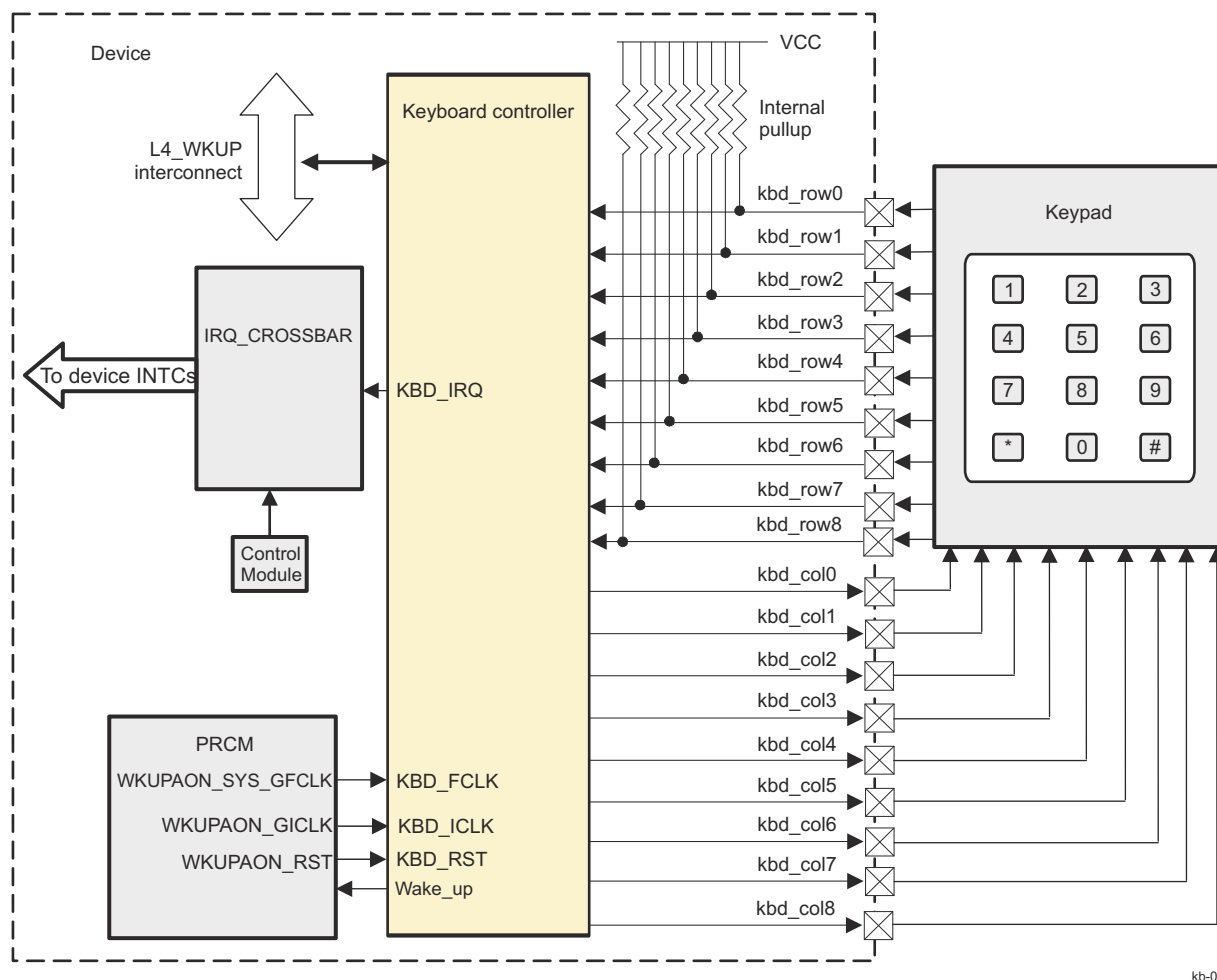
Figure 30-1. Keyboard Controller Overview
