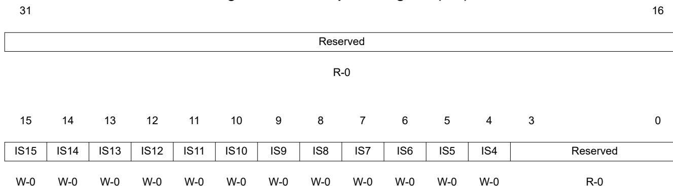
Figure 8-34. Interrupt Set Register (ISR)
