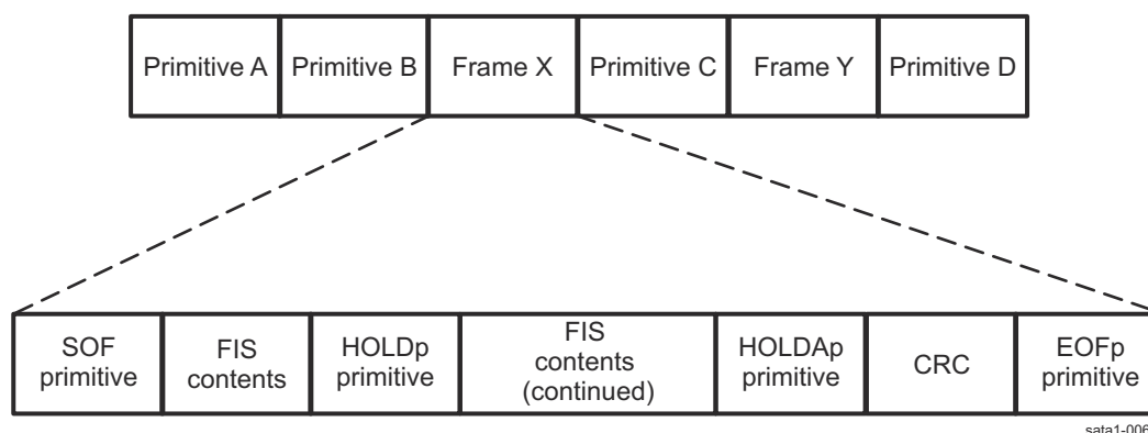
Figure 26-156. SATA Data Stream Components
