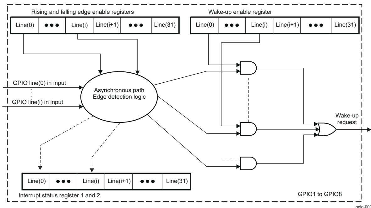
Figure 29-10. Wake-Up Request Generation
