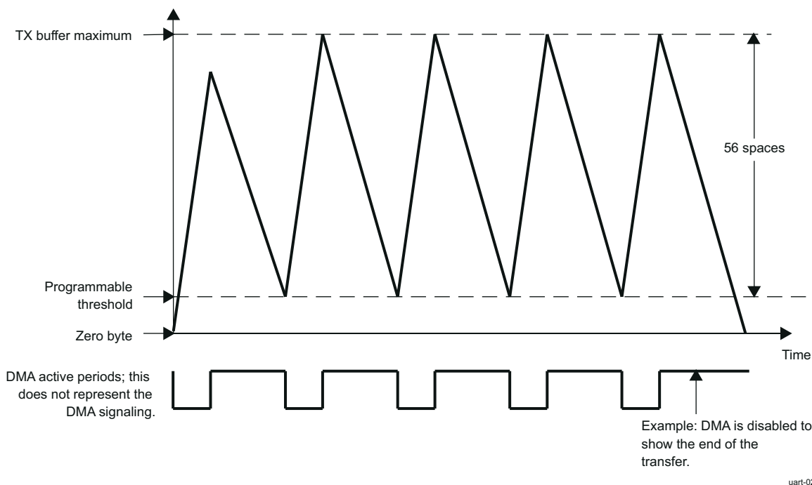
Figure 26-63. Transmit FIFO DMA Request Generation (56 Spaces)
