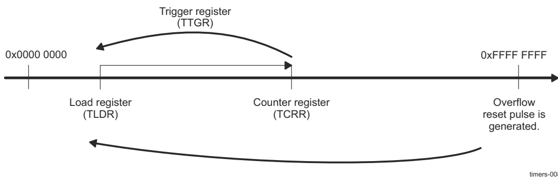
Figure 24-9. TCRR Timing Value
