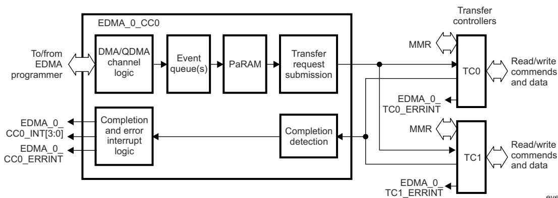
Figure 8-10. EDMA Block Diagram
