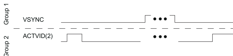
Figure 11-65. VSYNC and ACTIVID(2)
