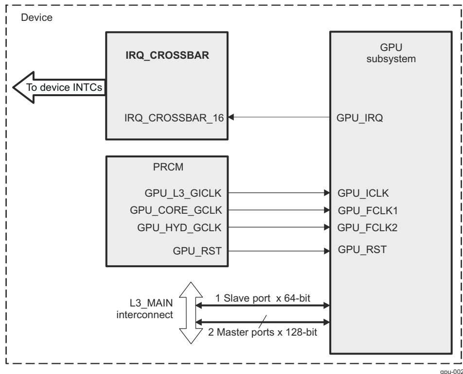
Figure 14-2. GPU Integration
