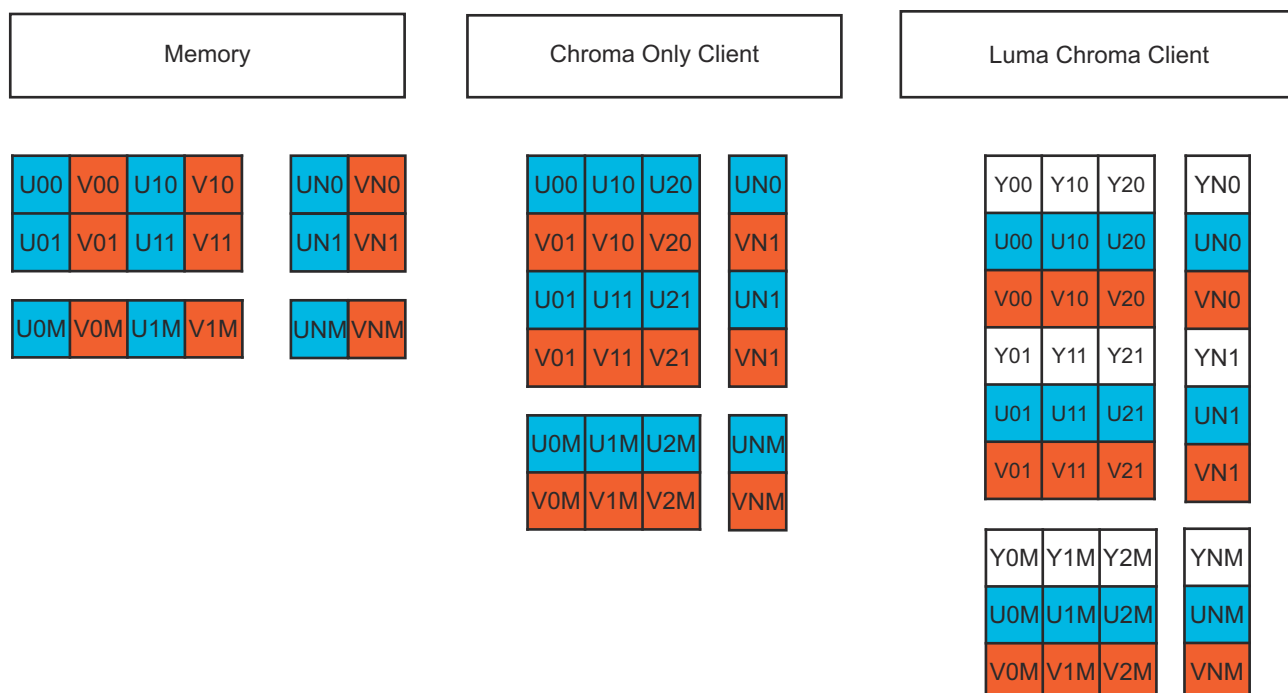
Figure 12-54. C 4:4:4 (Data Type 4)
