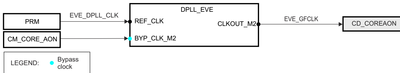
Figure 3-58. DPLL_EVE Overview
