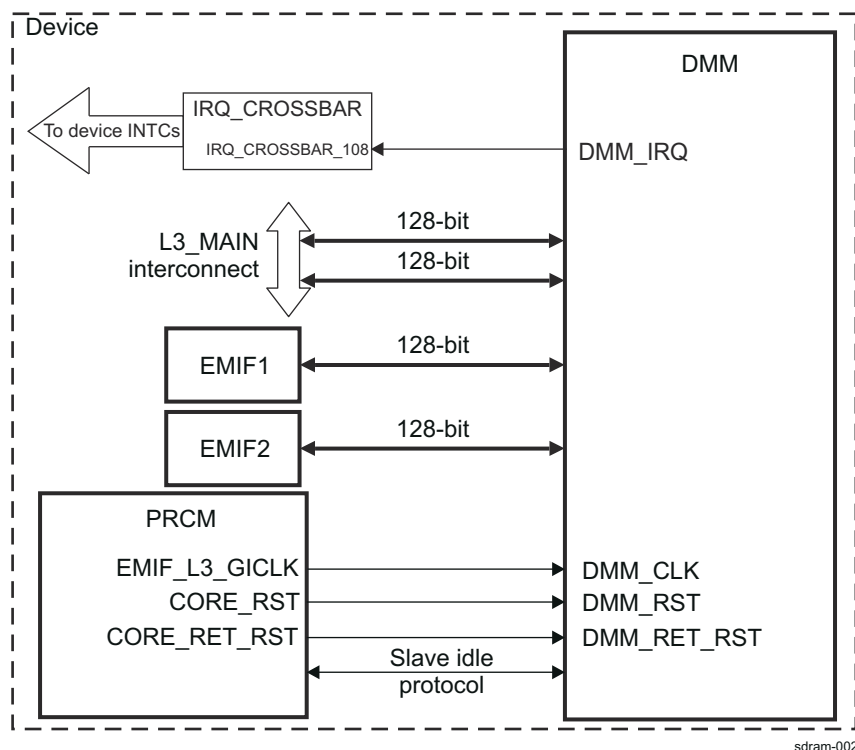
Figure 17-3. DMM Integration
