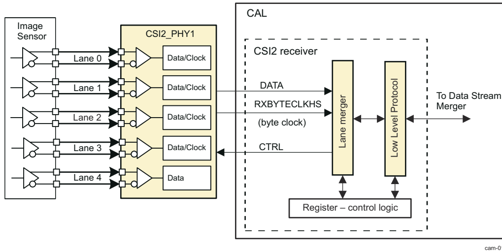
Figure 10-10. CSI2 Low Level Protocol Engine Block Diagram
