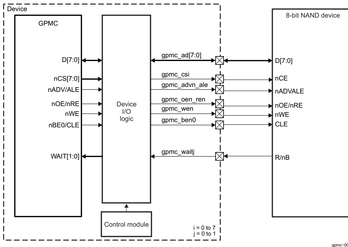
Figure 17-56. GPMC to 8-Bit NAND Device
