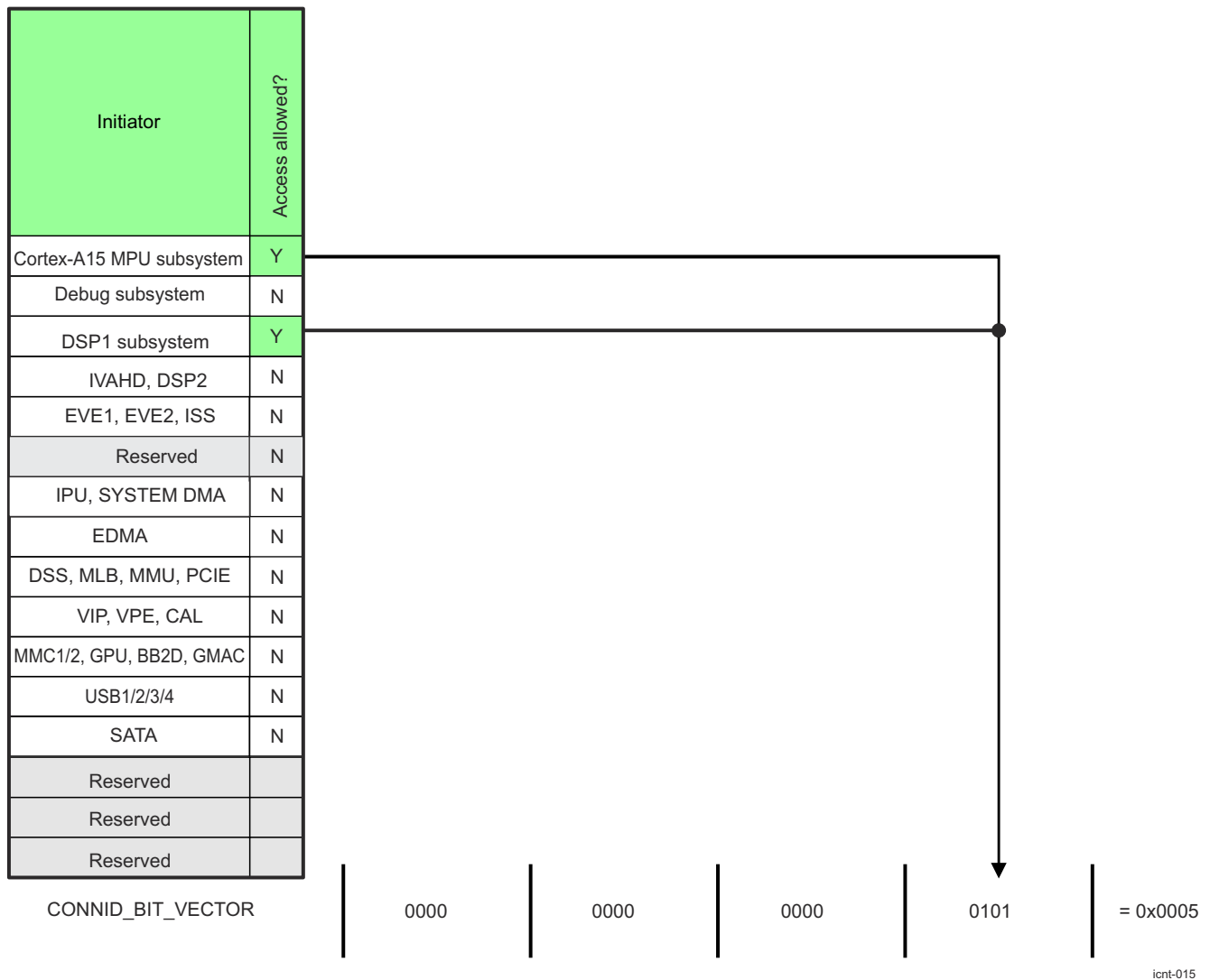
Figure 16-11. Example of CONNID_BIT_VECTOR L4_AP_PROT_GROUP_MEMBERS_k
