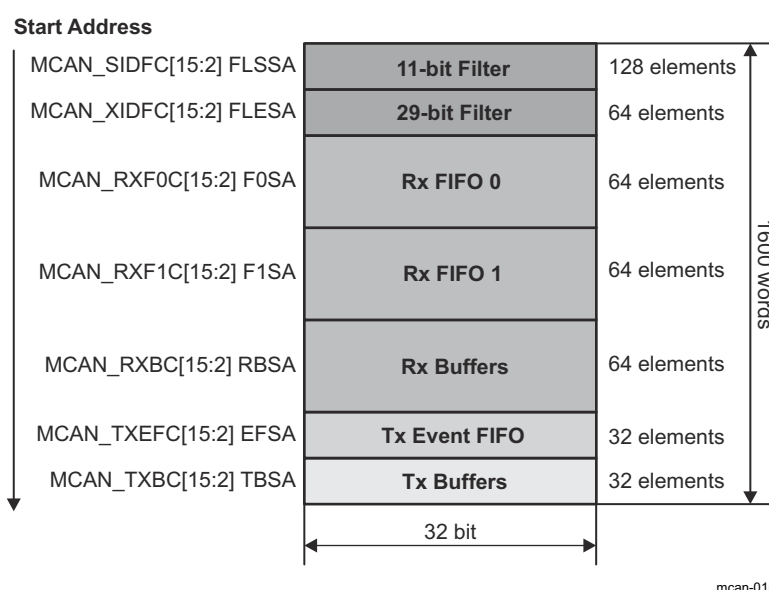
Figure 26-201. Message RAM Configuration
