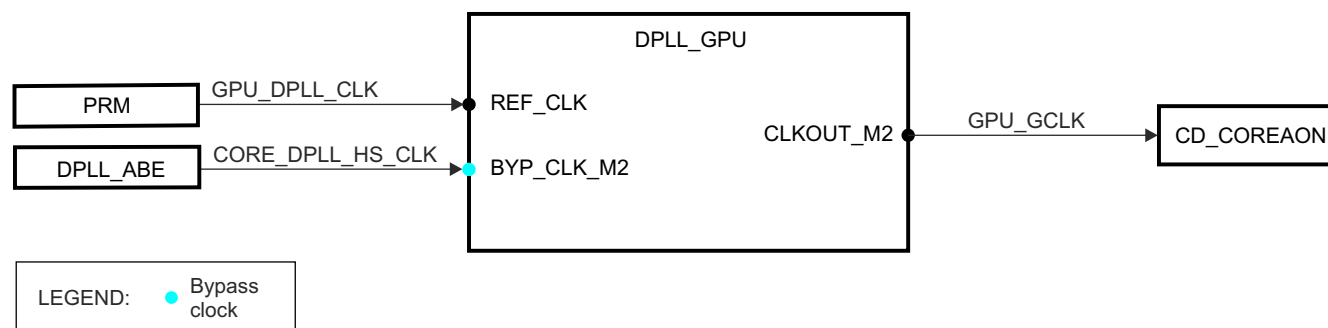
Figure 3-61. DPLL_GPU Overview
