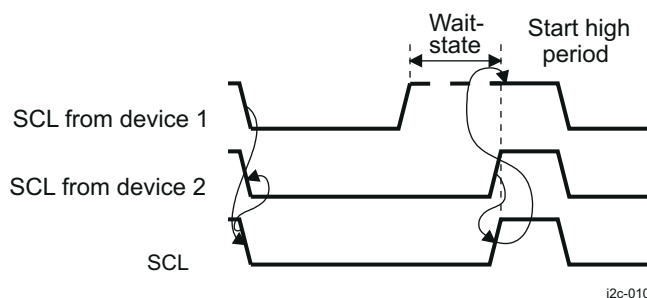
Figure 26-10. HS I 2 C Clock Generators Synchronization
