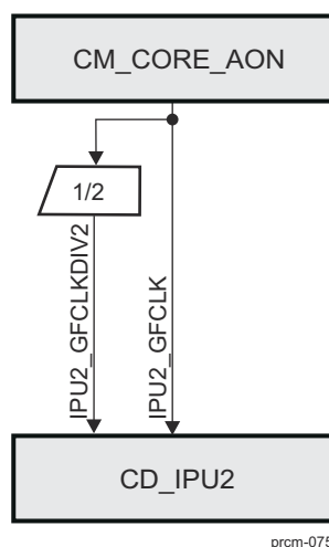
Figure 3-85. CD_IPU2 Overview
