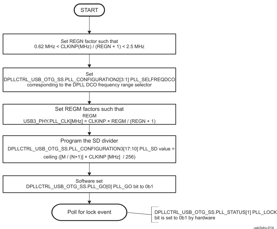
Figure 28-14. USB3_PHY PLL Programming Sequence
