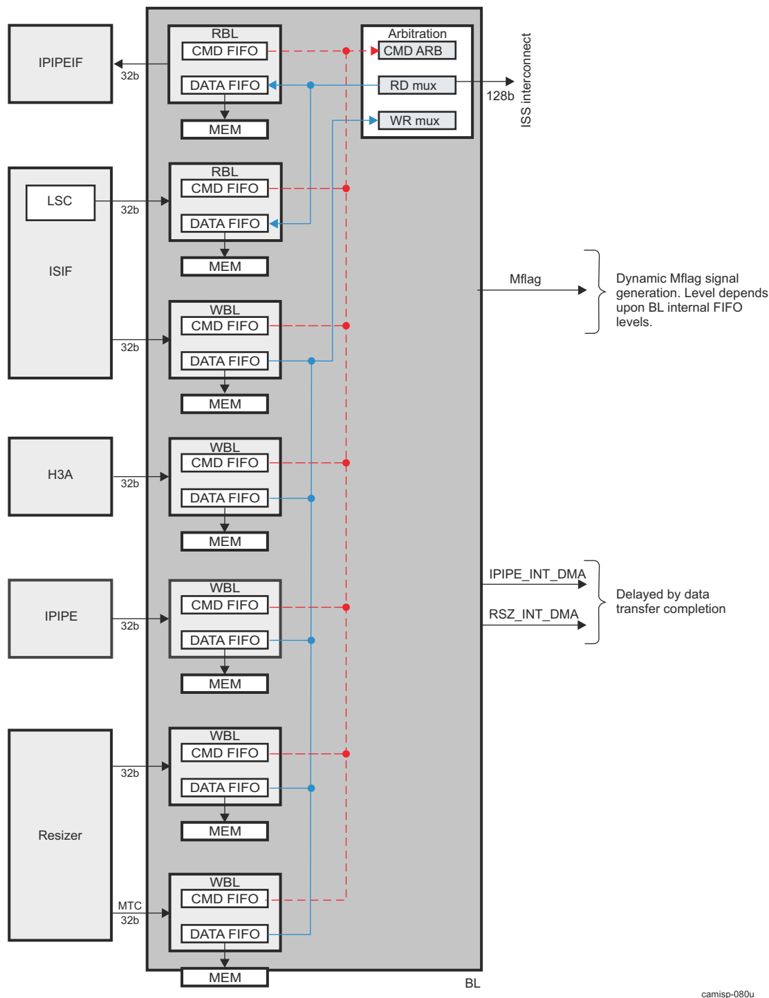
Figure 9-172. ISS ISP BL Block Diagram
