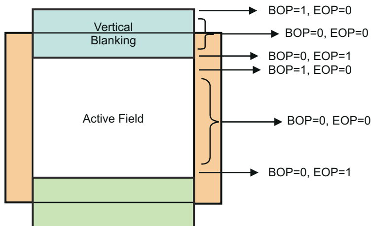
Figure 11-52. BOP/EOP Definition of a Period
