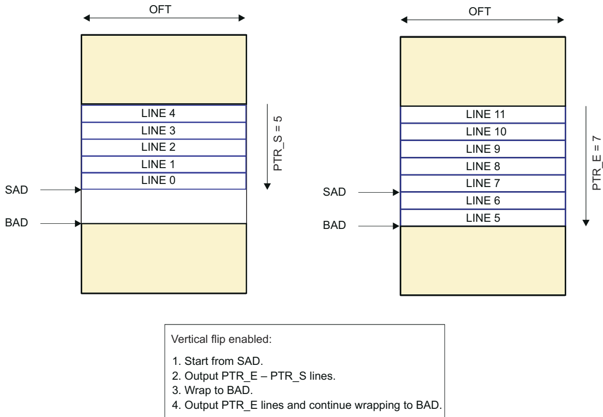
Figure 9-107. ISS ISP RSZ and Circular Buffer Settings – Example 2
