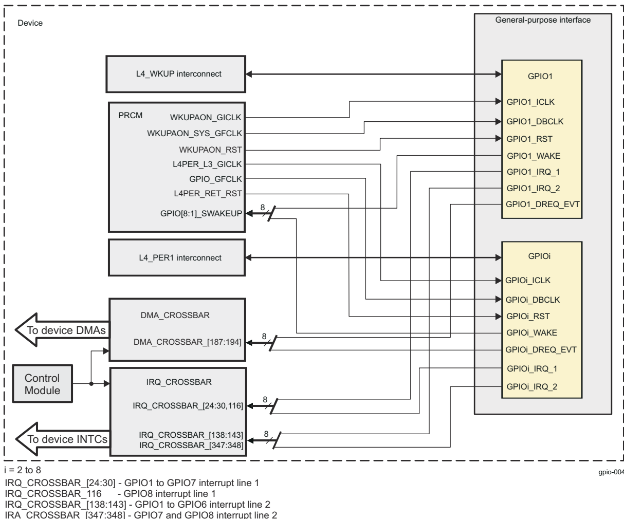
Figure 29-5. GPIO Integration
