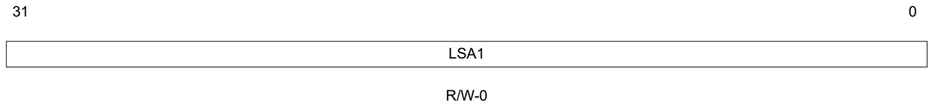
Figure 8-44. Loop 1 Start Address Register (LSA1)
