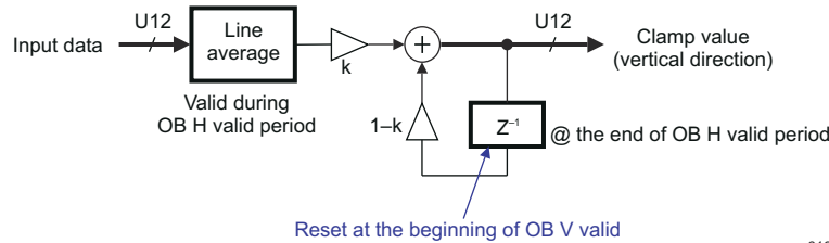
Figure 9-149. ISS ISP ISIF Clamp Value for Vertical Direction Calculation
