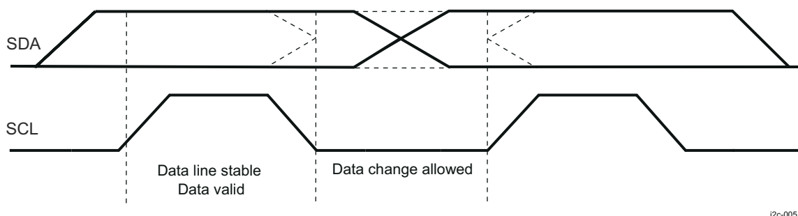
Figure 26-5. HS I 2 C Bit Transfer on the I 2 C Bus
