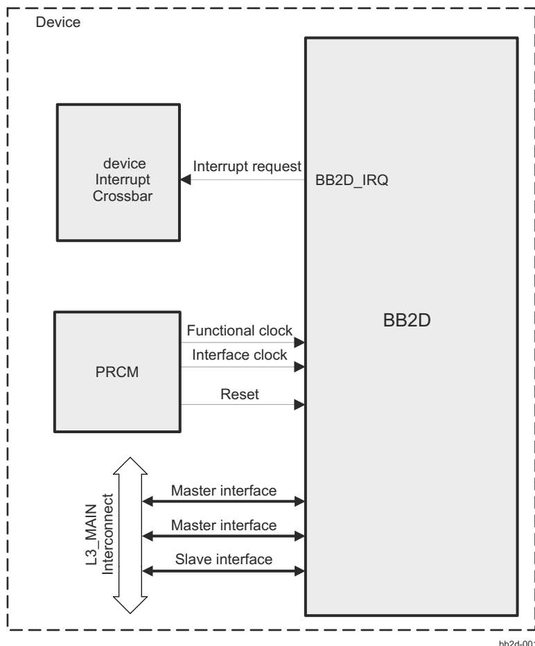
Figure 15-1. BB2D Overview
