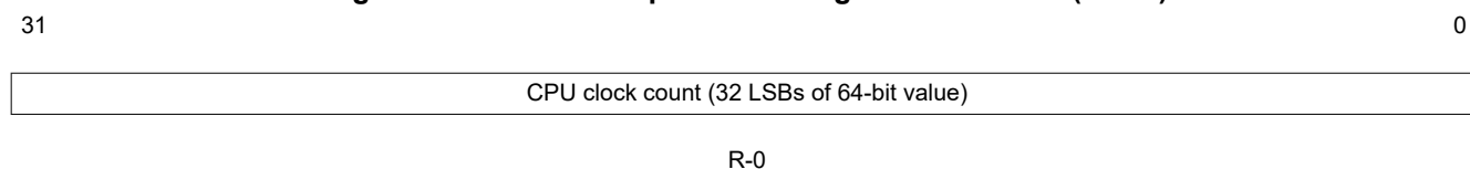
Figure 8-52. Time Stamp Counter Register - Low Half (TSCL)
