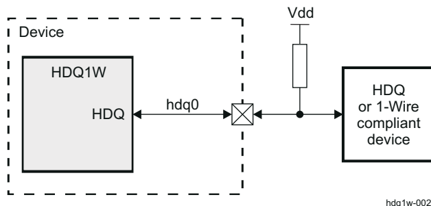
Figure 26-29. HDQ1W Typical Application System Overview
