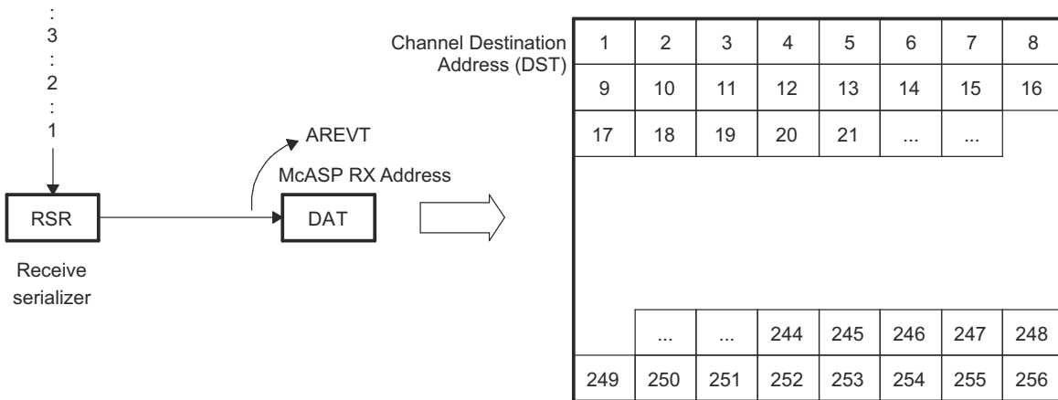
Figure 18-39. Servicing Incoming McASP Data Example
