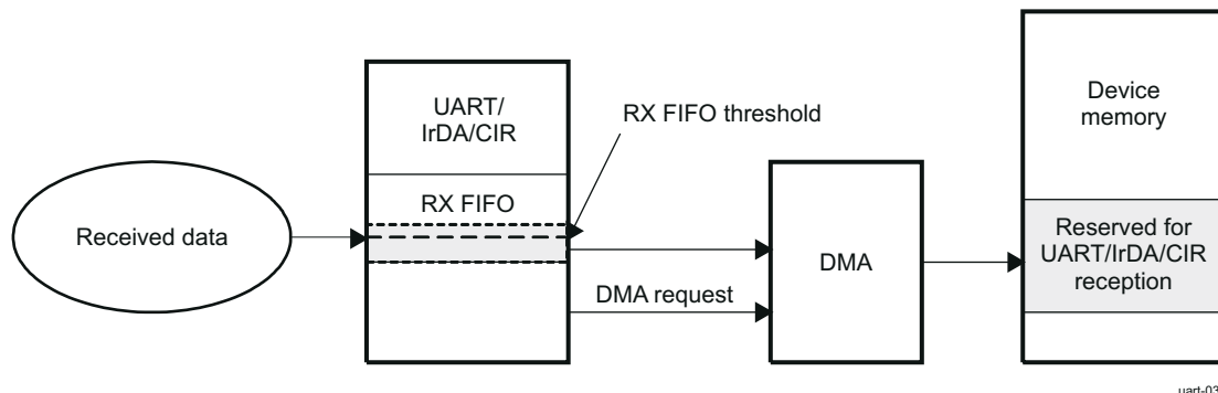
Figure 26-68. DMA Reception
