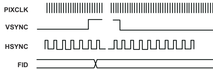
Figure 11-33. 4-Pin Reduced HSYNC Signaling with Vertical Ancillary Data
