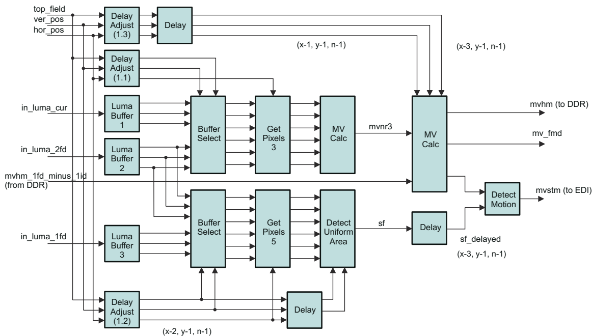
Figure 12-4. Motion Detection (MDT) Block Diagram
