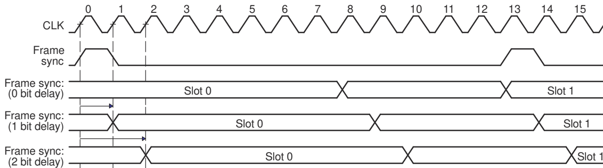
Figure 26-126. Burst Frame Sync Mode
