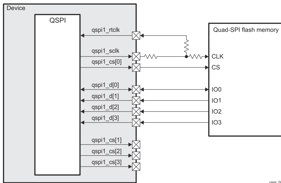
Figure 26-102. QSPI Connected to an External Quad-SPI Flash Memory
