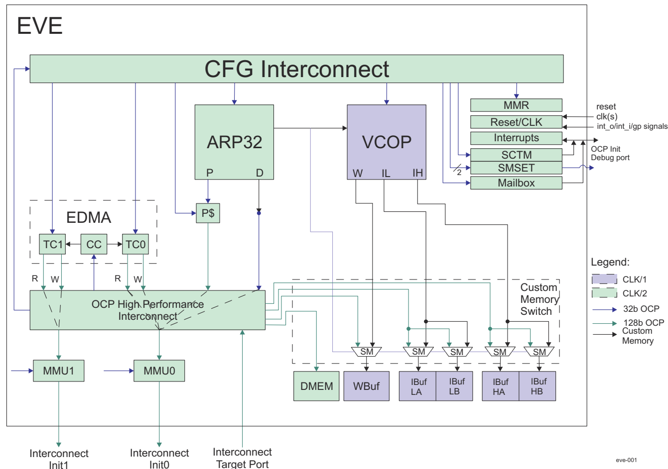
Figure 8-1. EVE Overview
