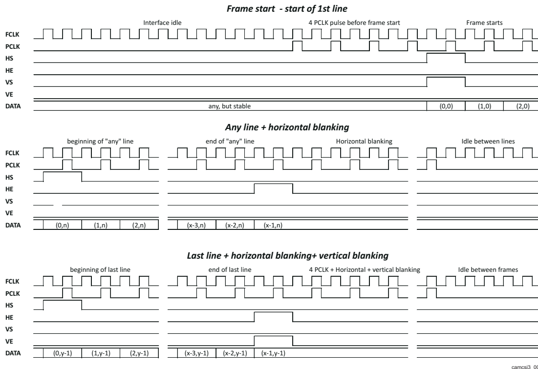
Figure 9-8. CAL BYS Input Port Timing Example
