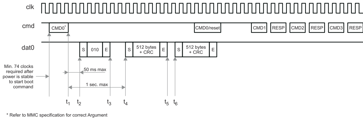
Figure 27-26. Boot Acknowledge Time-Out When Using CMD0
