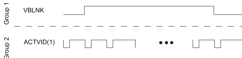
Figure 11-60. VBLNK and ACTID (1)
