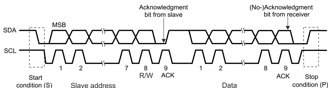
Figure 26-4. HS I 2 C Data Transfer
