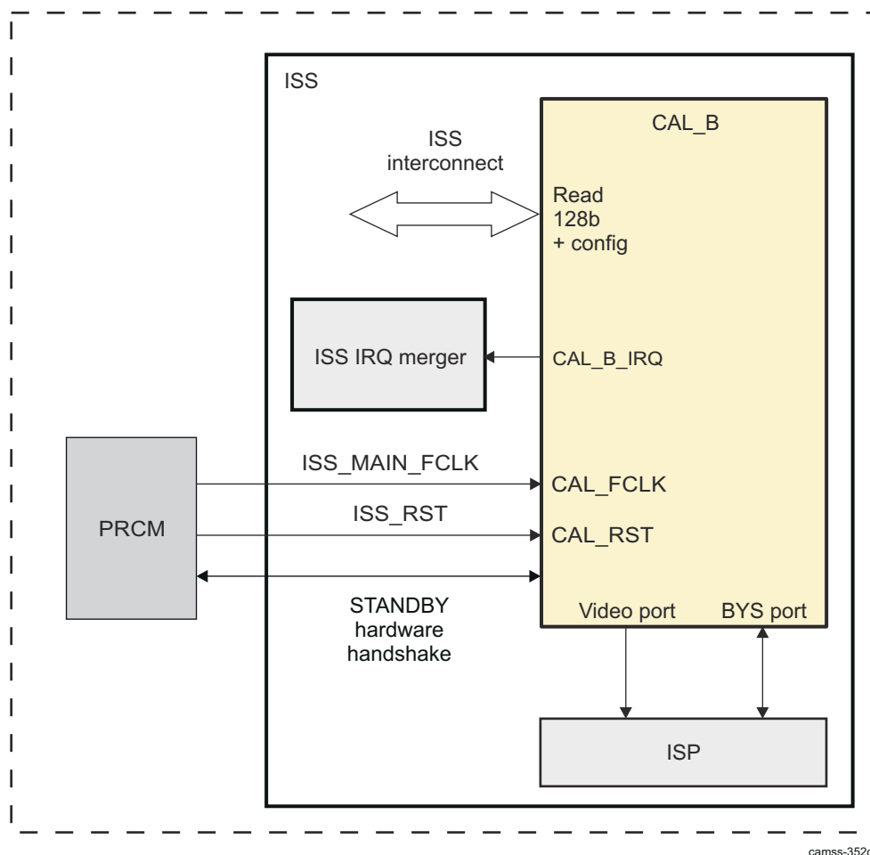
Figure 9-7. CAL Integration
