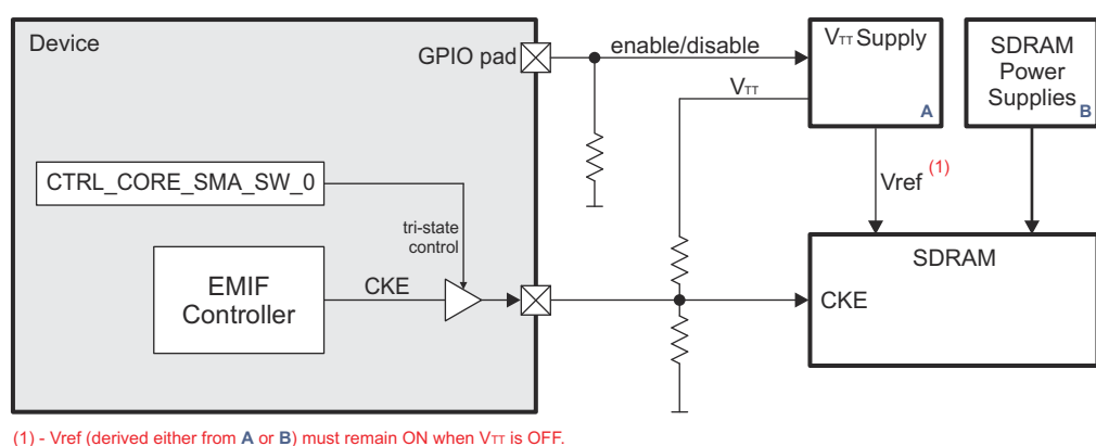
Figure 17-51. Example for Using the CKE Tri-state Functionality
