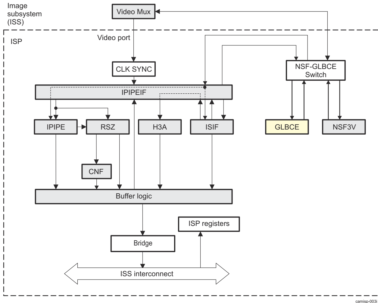
Figure 9-31. ISS ISP GLBCE High-Level Diagram
