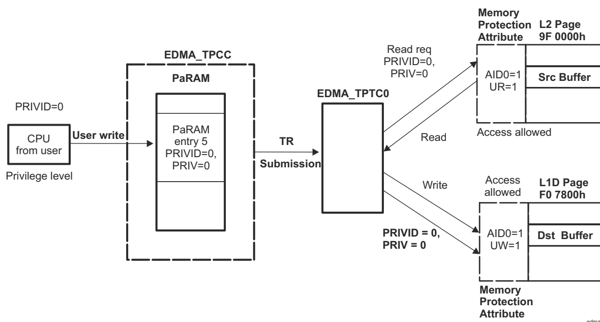
Figure 18-31. Proxy Memory Protection Example
