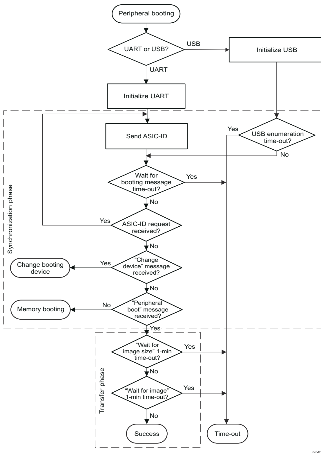
Figure 34-11. Peripheral Booting Procedure
