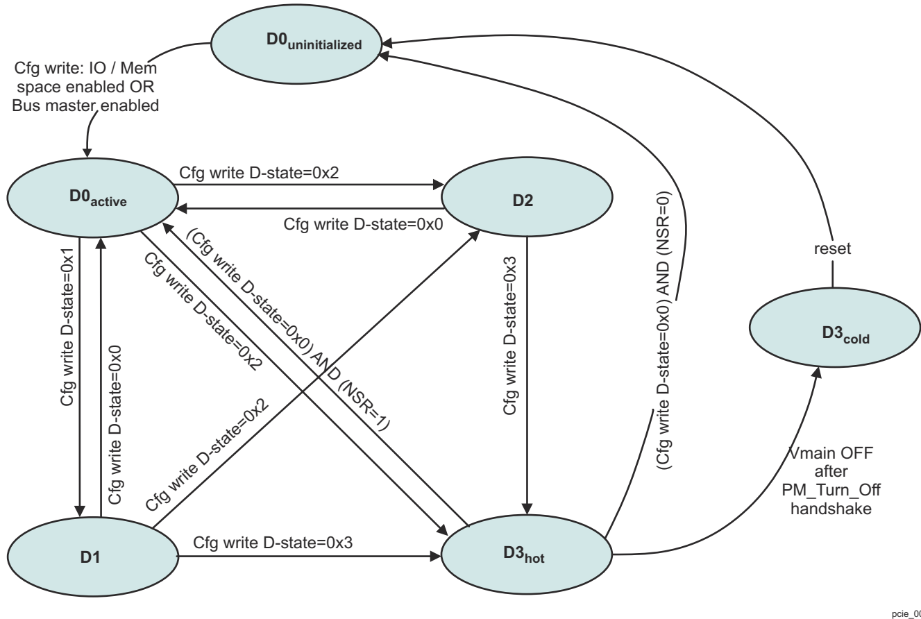
Figure 26-162. PCIe D-state (function power state) FSM diagram
