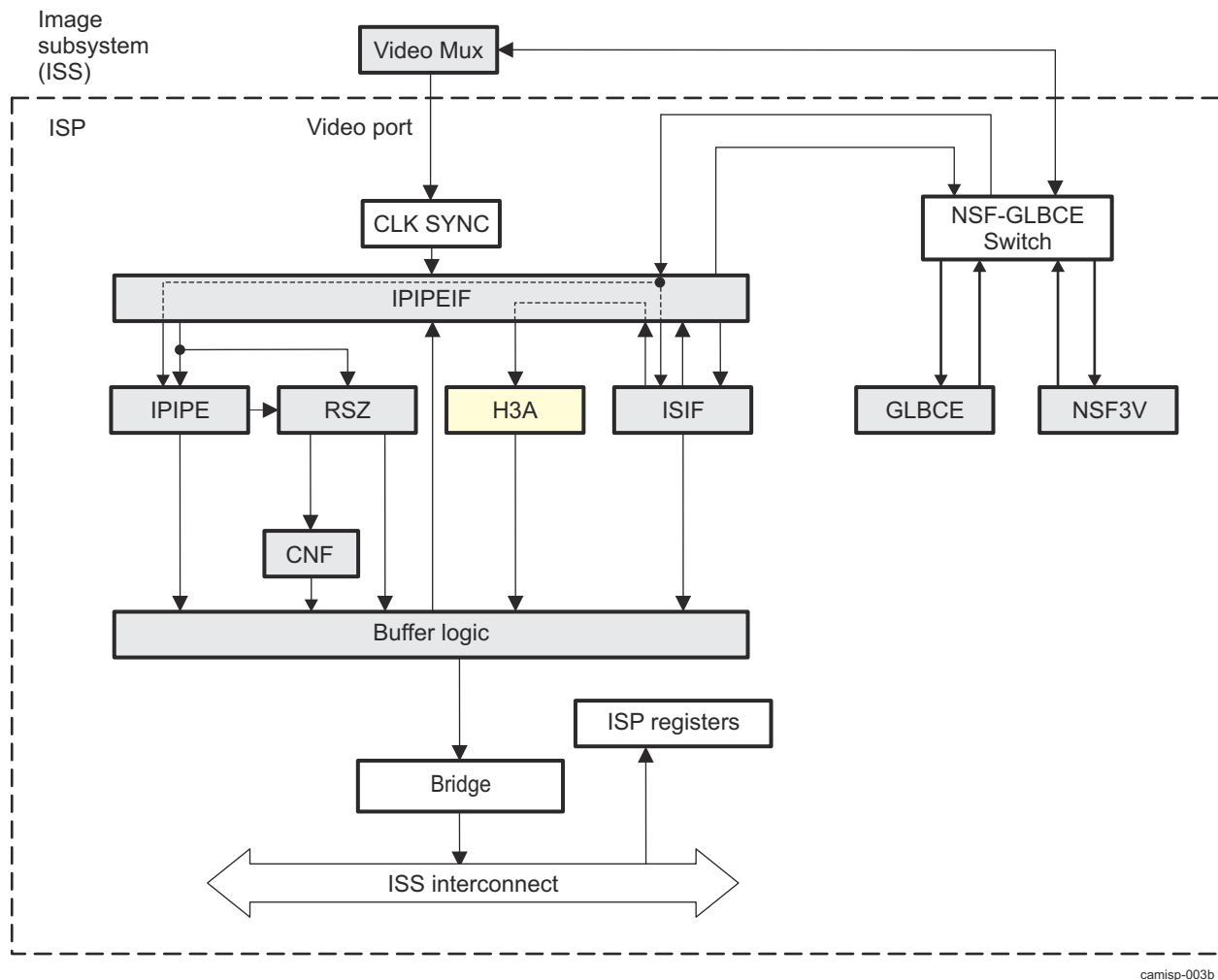
Figure 9-112. ISS ISP H3A High-Level Diagram
