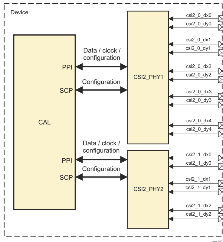
Figure 10-2. CAMSS Environment
