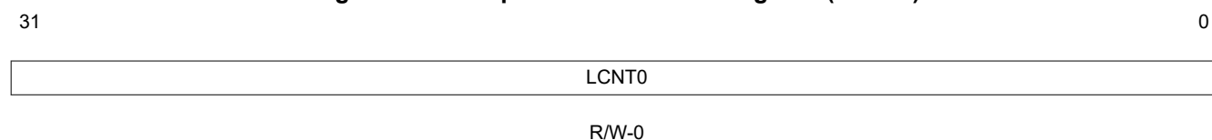
Figure 8-43. Loop 0 Iteration Count Register (LCNT0)
