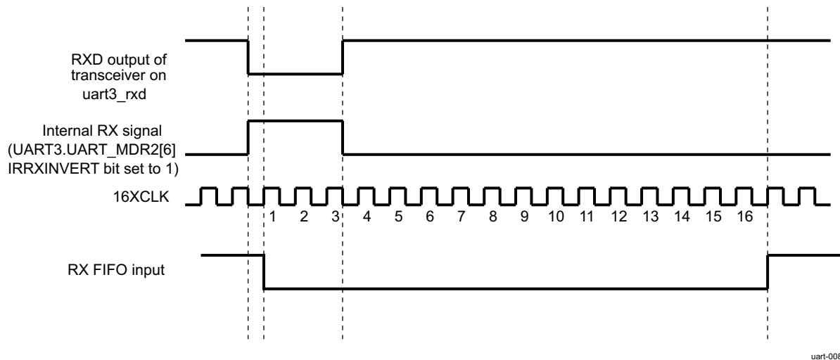
Figure 26-43. IrDA SIR Decoding Mechanism
