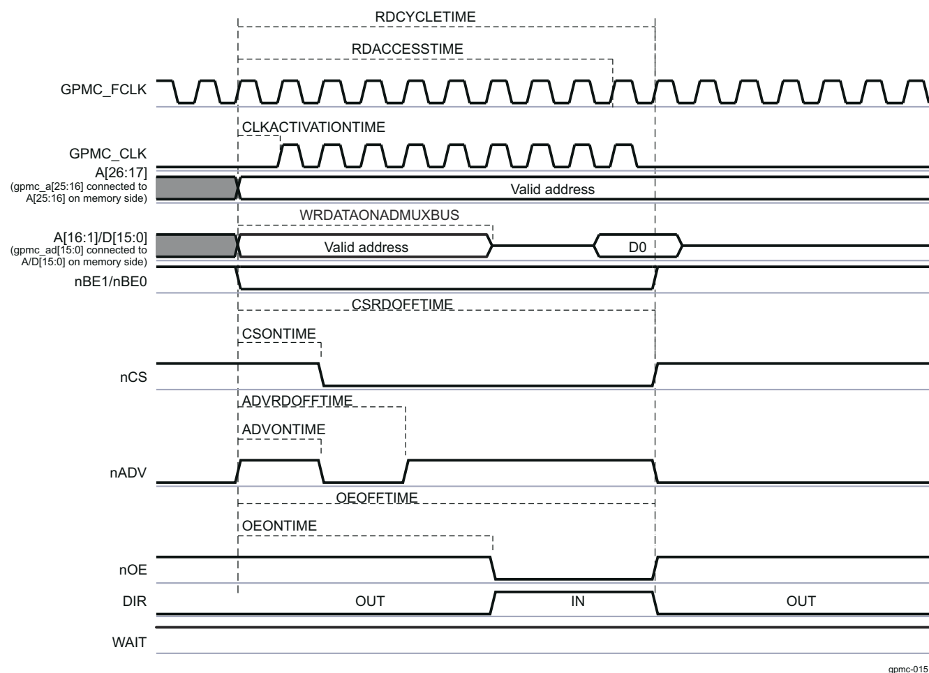
Figure 17-70. Synchronous Single Read (GPMCFCLKDIVIDER = 0)
