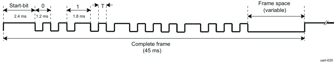
Figure 26-56. SIRC Bit Transmission Example
