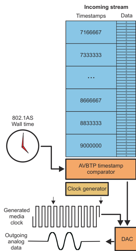
Figure 26-217. Cross Time Stamping and Presentation Timestamps
