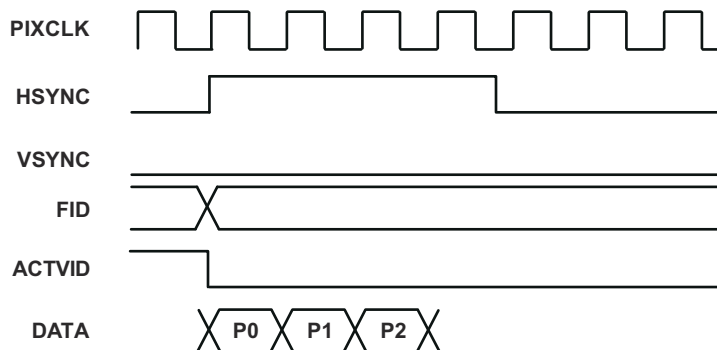
Figure 11-29. Type 1, Horizontal Blanking in Video Region
