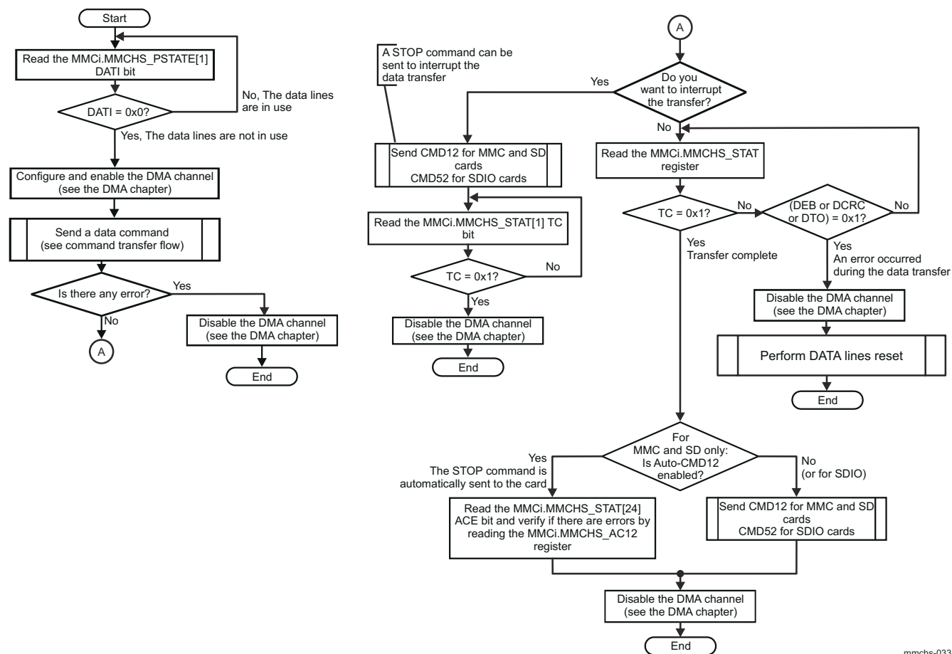
Figure 27-39. eMMC/SD/SDIO Controller Read/Write Transfer Flow in DMA Mode With Polling
