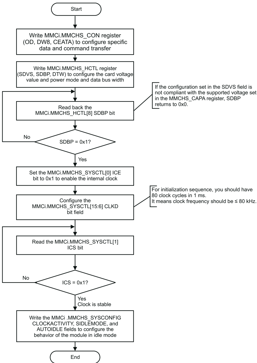
Figure 27-35. eMMC/SD/SDIO Controller Bus Configuration
