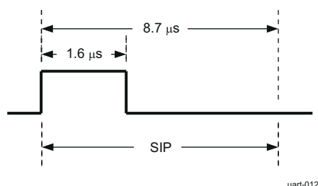
Figure 26-47. SIP
