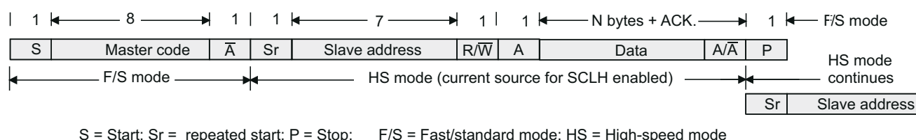
Figure 26-8. HS I 2 C Data Transfer in HS Mode
