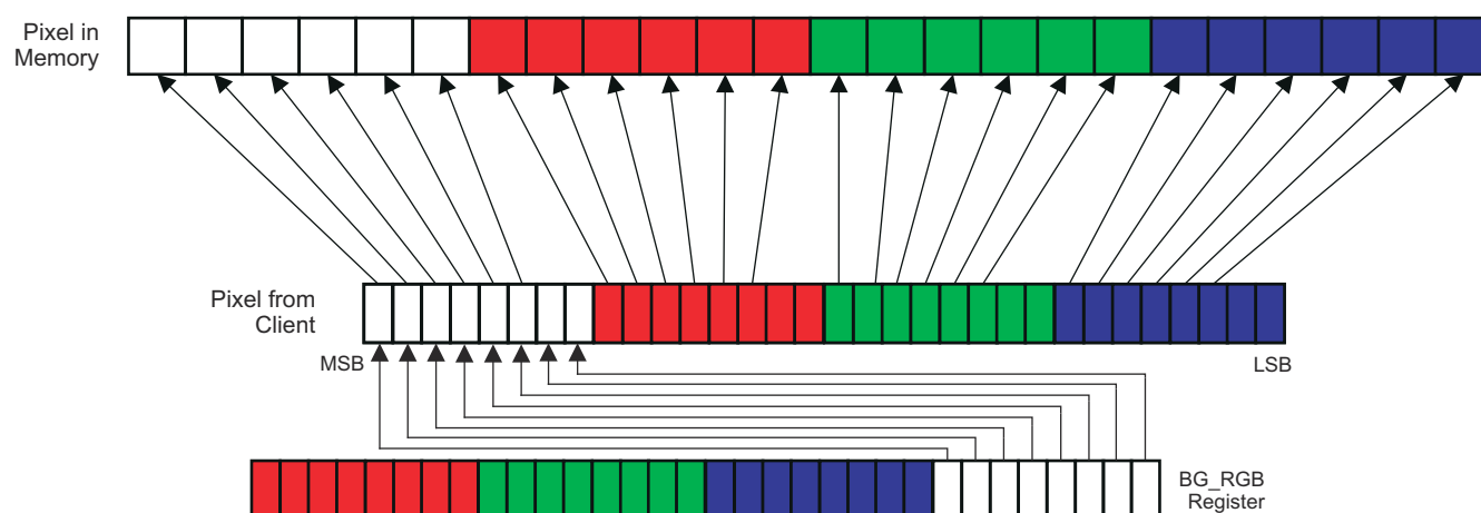
Figure 12-65. ARGB24-6666 (Data Type 5)
