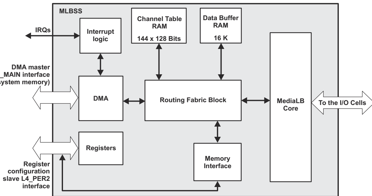
Figure 26-232. MLBSS Structural Overview
