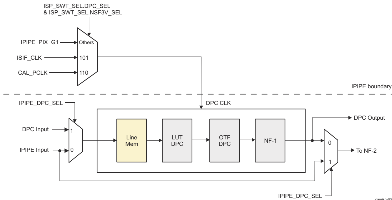
Figure 9-63. ISS ISP IPIPE Data flow of DPC Interface
