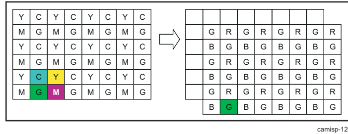
Figure 9-144. ISS ISP ISIF Second Pixel/Last Line Generation
