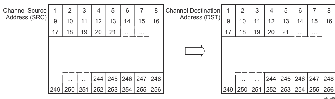
Figure 18-33. Block Move Example
