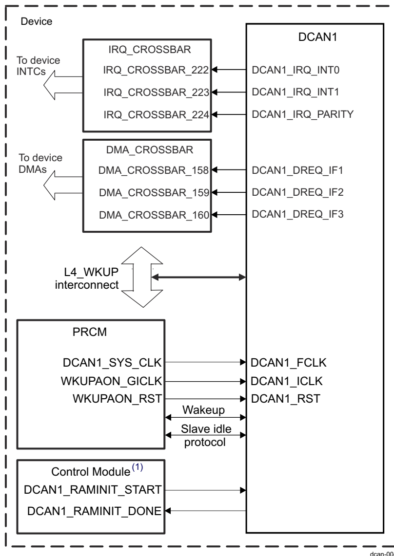
Figure 26-167. DCAN1 Integration
