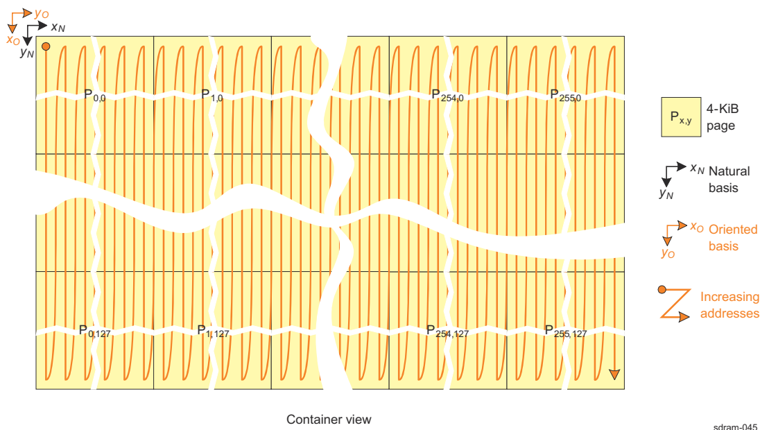
Figure 17-29. Tiled Mode Ordering of Elements in 90-Degree View With Vertical Mirror
