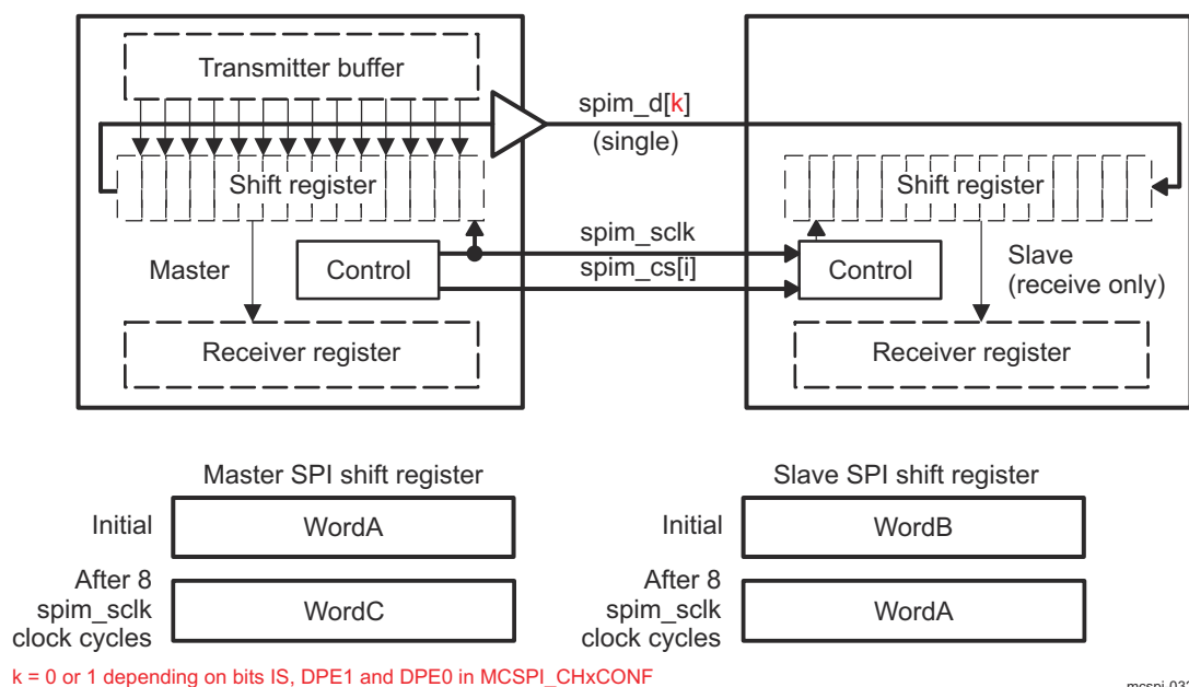
Figure 26-90. SPI Half-Duplex Transmission (Receive-Only Slave)
