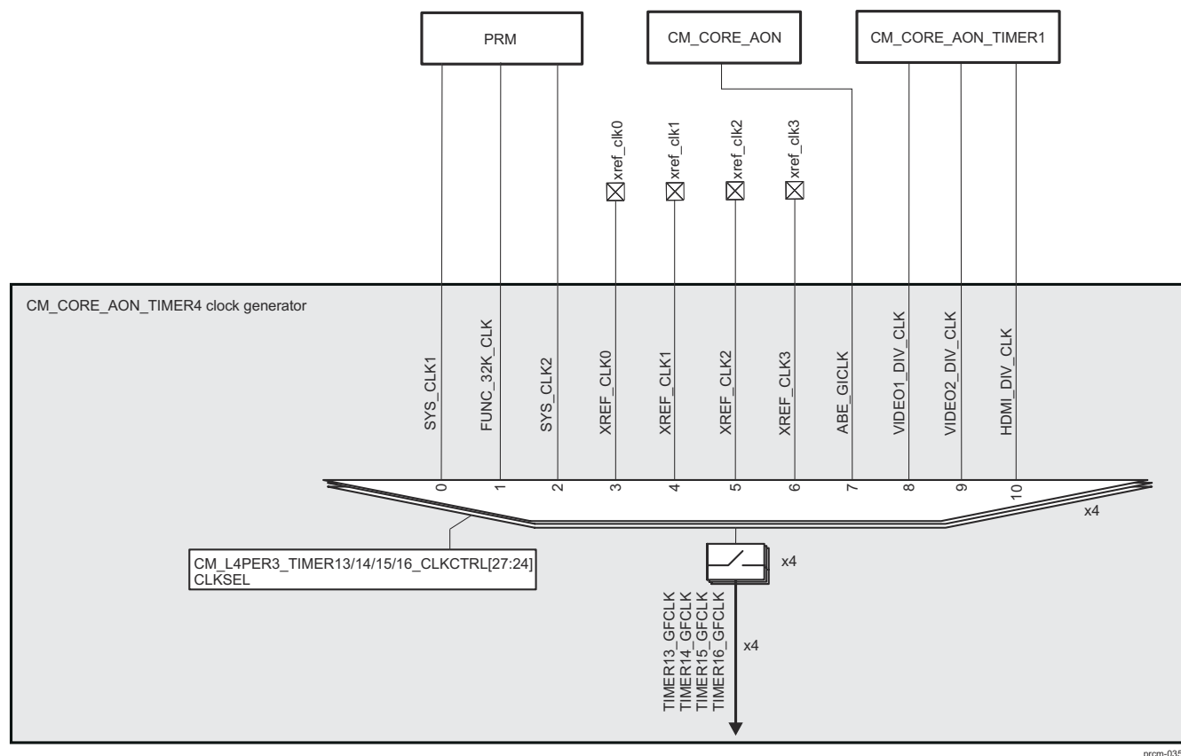
Figure 3-47. CM_CORE_AON_TIMER4 Clock Manager Overview
