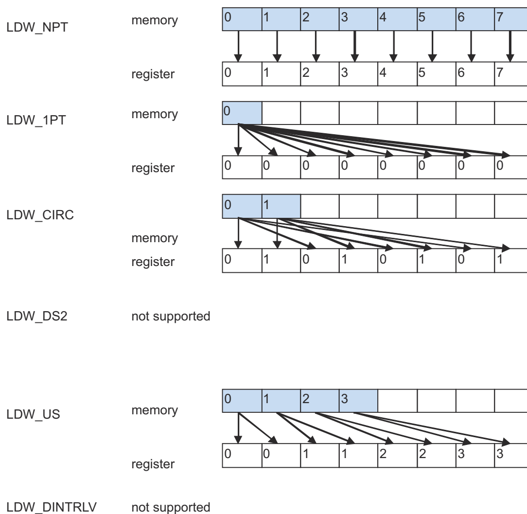
Figure 8-63. Load Word Distribution Options
