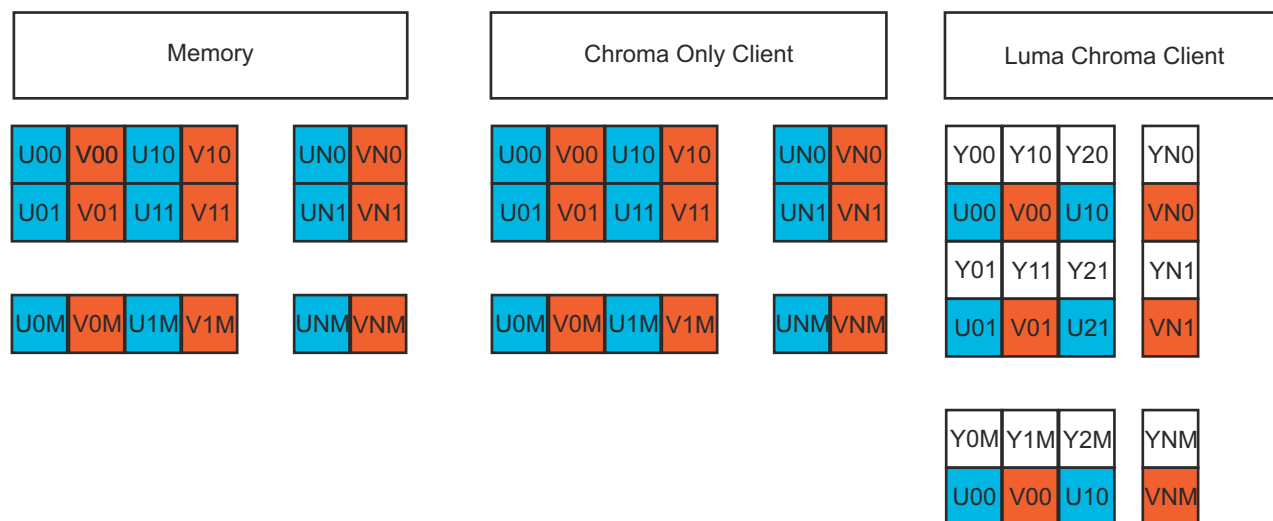
Figure 11-101. C 4:2:2 (Data Type 5)
