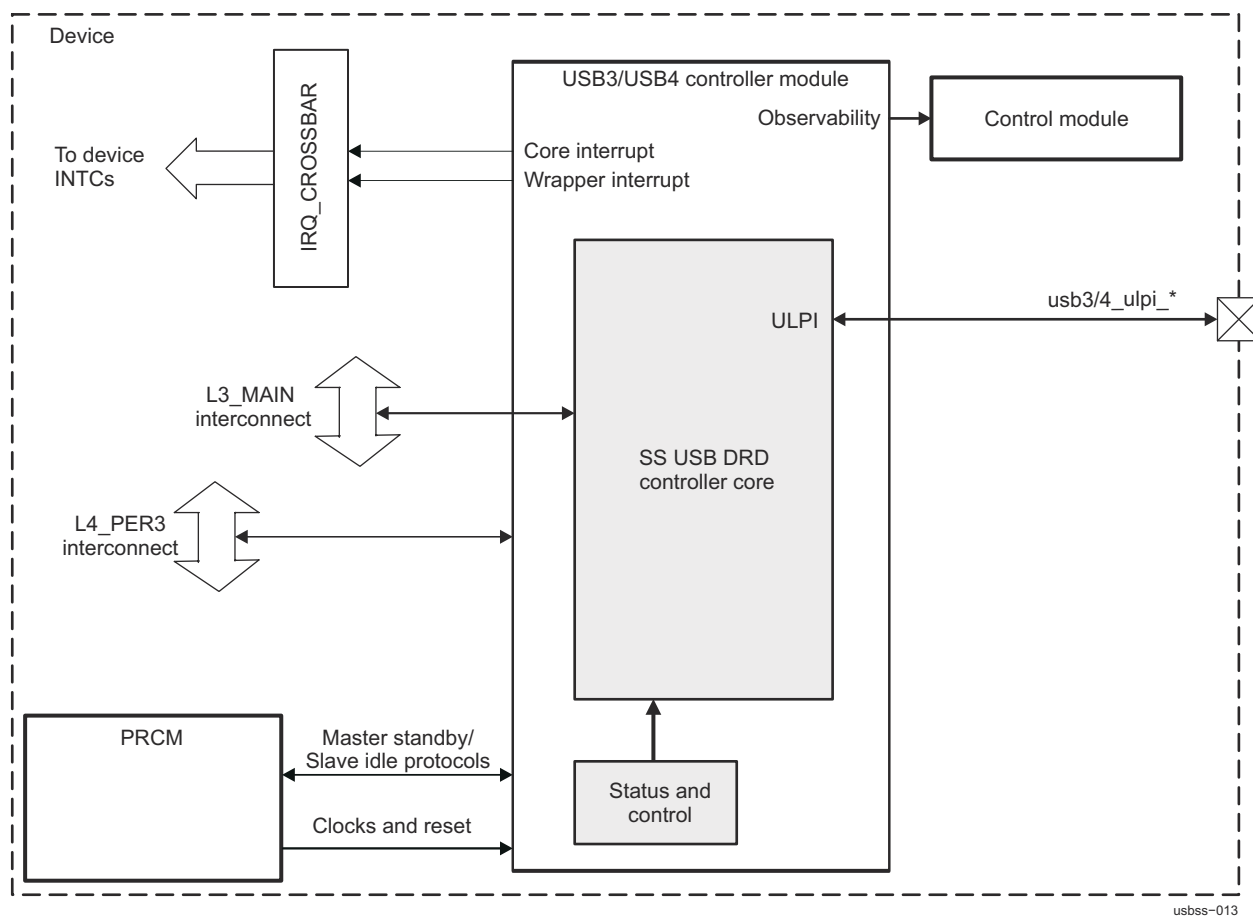
Figure 26-145. USB3 Highlight
