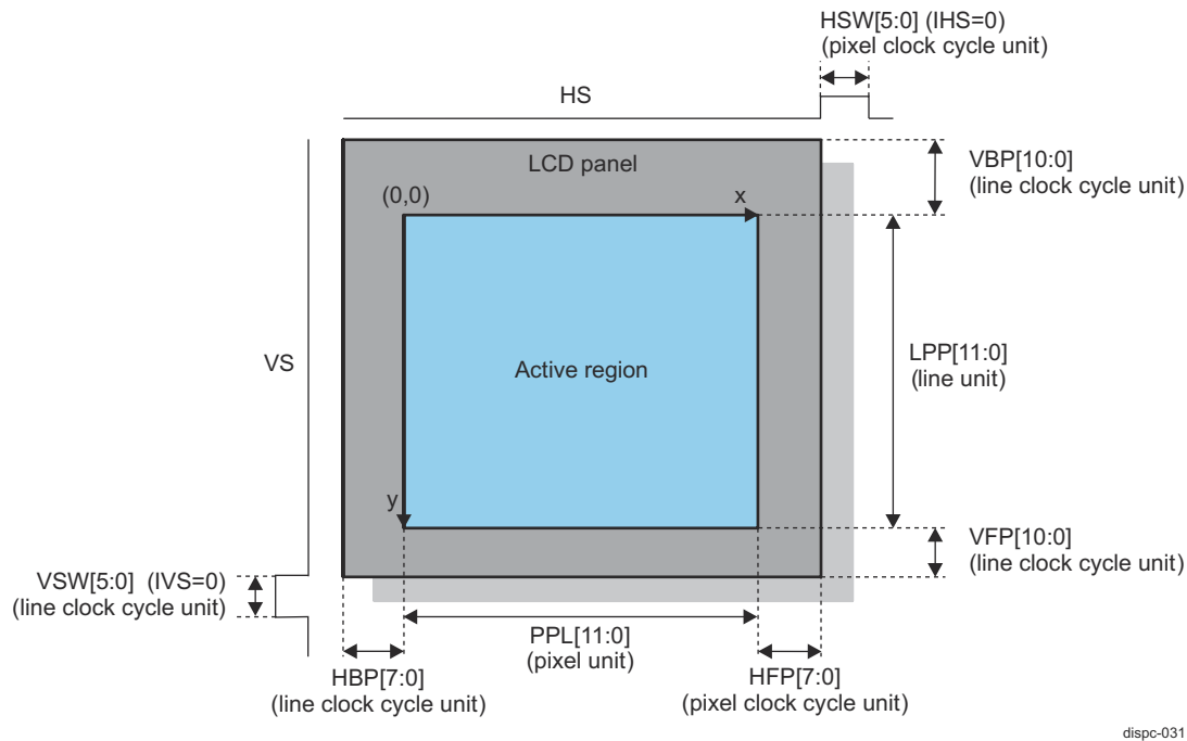
Figure 13-92. DISPC Timing Values (Active Matrix Display)
