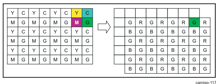
Figure 9-141. ISS ISP ISIF Second Last Pixel/First Line Generation
