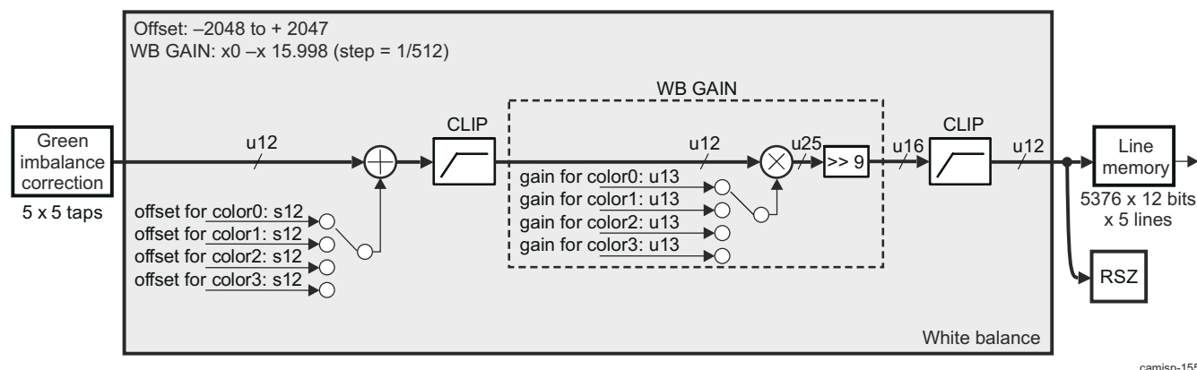
Figure 9-64. ISS ISP IPIPE White Balance
