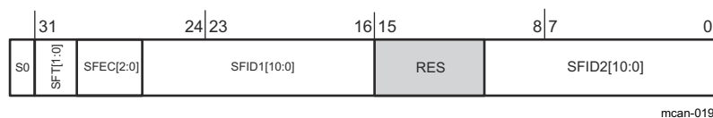
Figure 26-205. Standard Message ID Filter Element Structure
