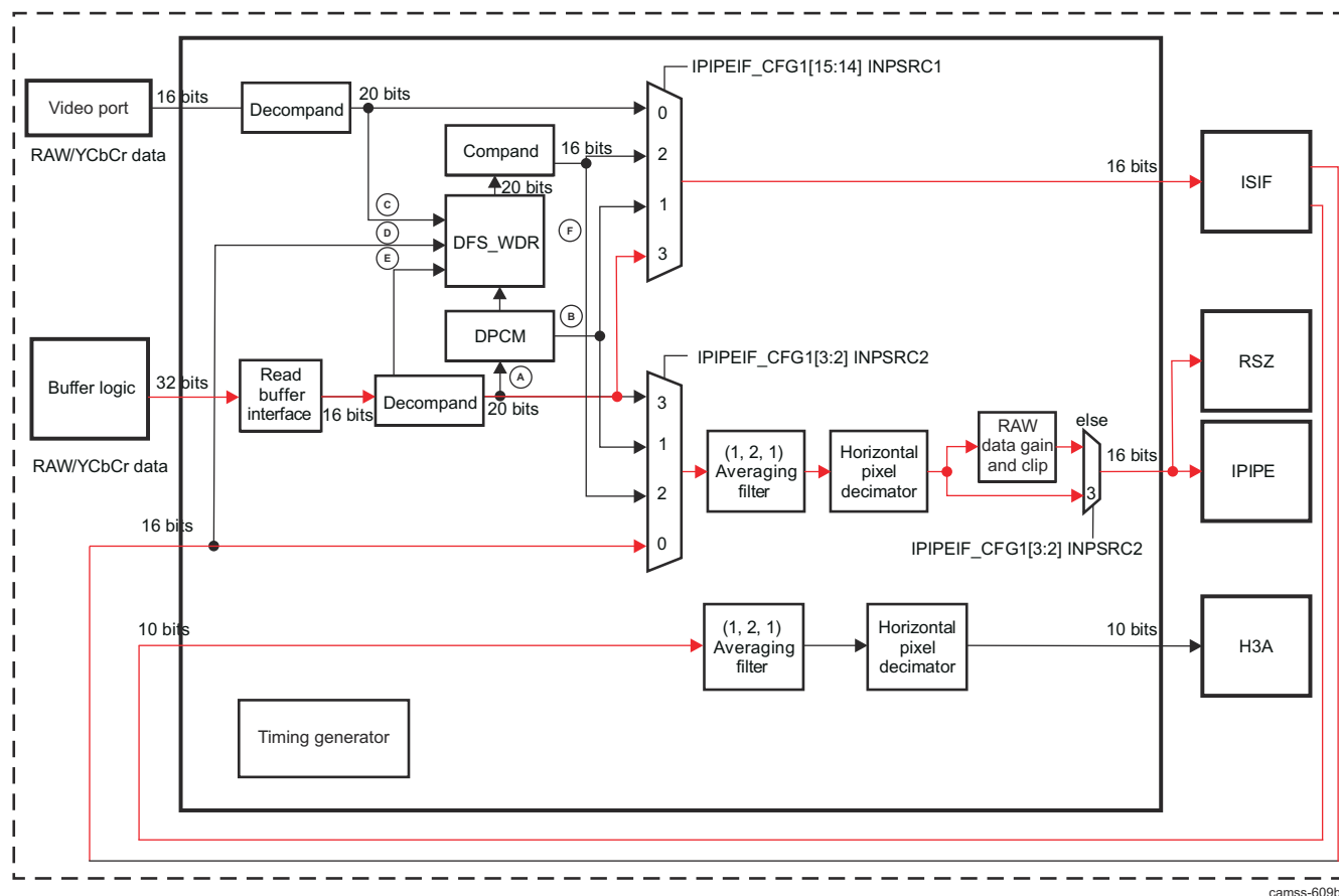
Figure 9-48. ISS ISP IPIPEIF INPSRC1 = 3 and INPSRC2 = 0 Data Path
