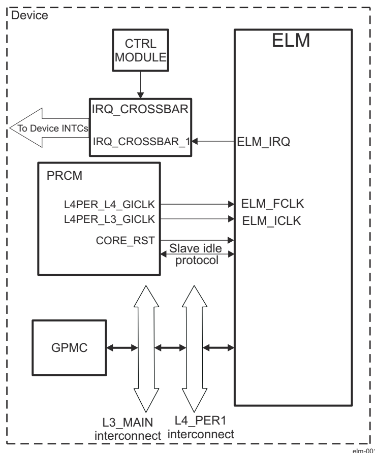
Figure 17-105. ELM Integration
