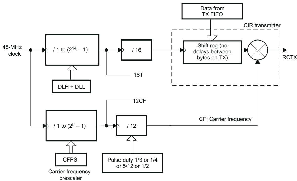
Figure 26-71. CIR Mode Block Components
