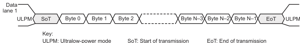
Figure 10-11. CSI2 One Data-Lane Configuration
