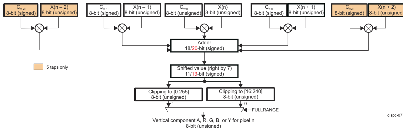
Figure 13-69. DISPC Macro-Architecture of the Vertical Scaling for A, R, G, B, and Y Components
