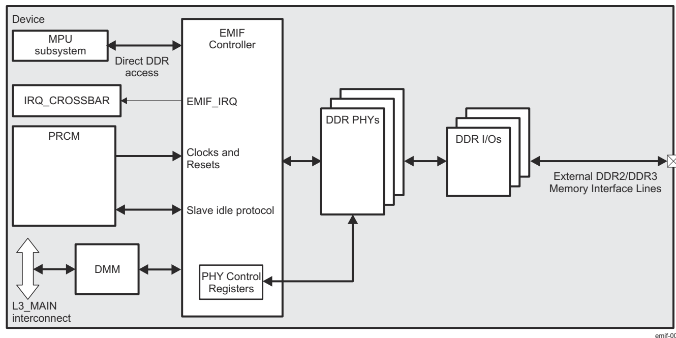
Figure 17-45. EMIF Controller Overview
