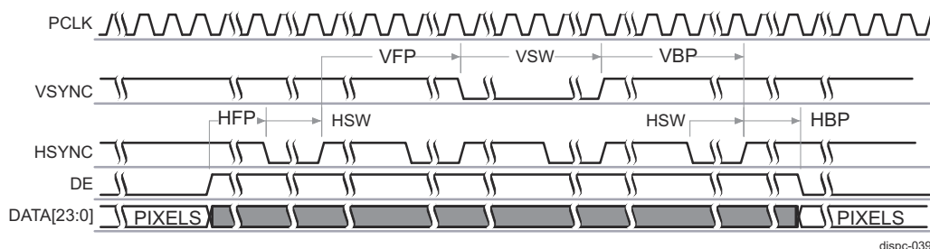
Figure 13-34. DISPC Active Matrix Timing Diagram of Configuration 2 (Between Frames)
