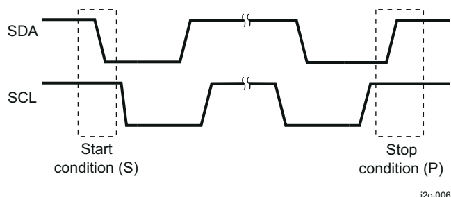
Figure 26-6. HS I 2 C S and P Condition Events
