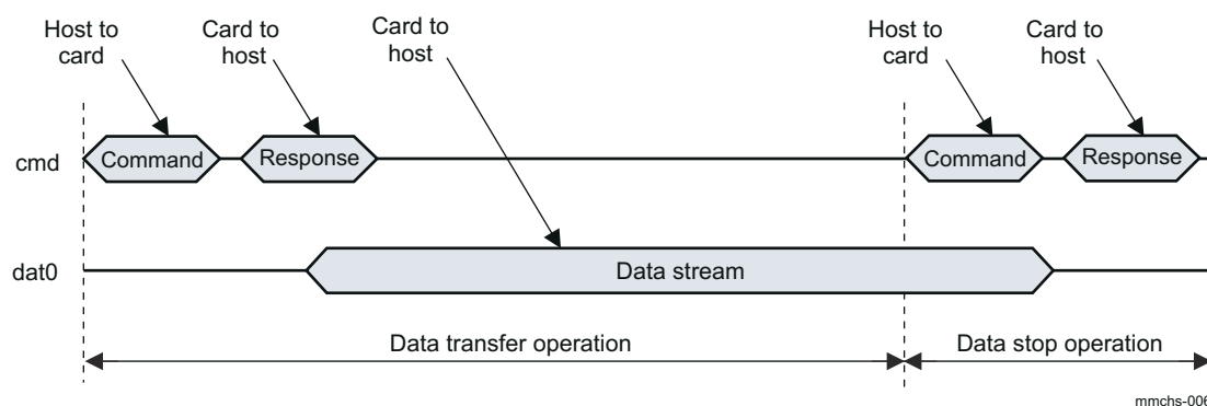
Figure 27-3. Sequential Read Operation (MMC Cards Only)
