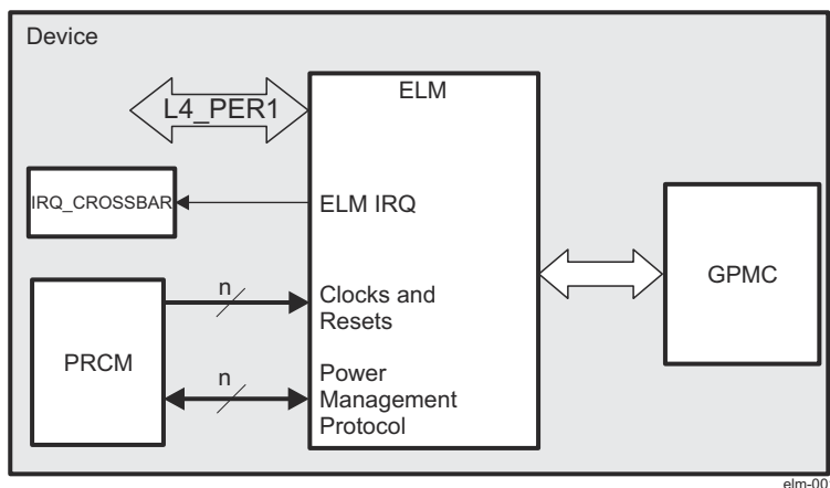
Figure 17-104. ELM Overview
