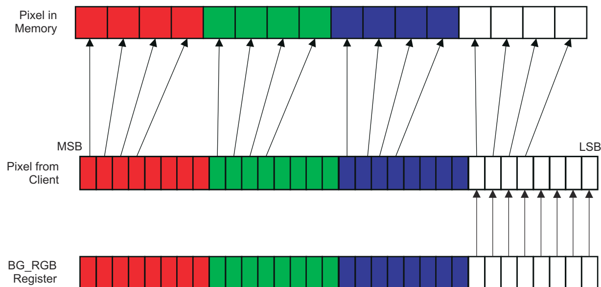
Figure 11-110. RGBA-4444 (Data Type 4)
