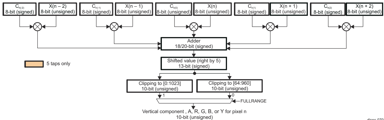
Figure 13-61. DISPC Macro-Architecture of the Vertical Scaling for A, R, G, B, and Y Components (5 and 3 taps)
