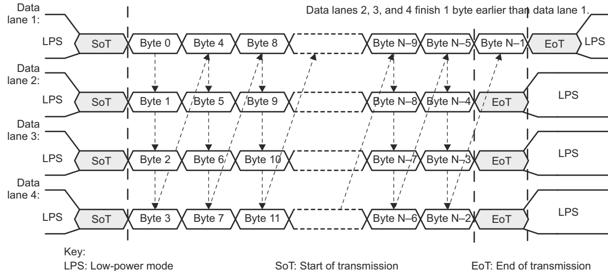
Figure 10-14. CSI2 Four Data-Lane Merger Configuration
