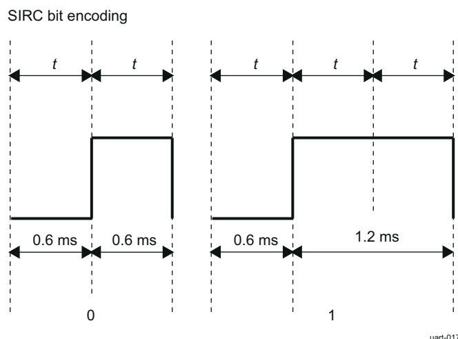
Figure 26-53. SIRC Bit Encoding
