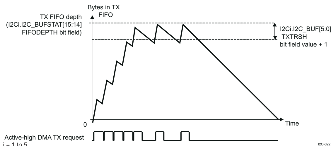
Figure 26-18. HS I²C Transmit FIFO Request Generation (Low Threshold)
