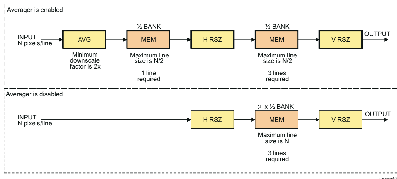
Figure 9-99. ISS ISP RSZ Averager Memory Utilization
