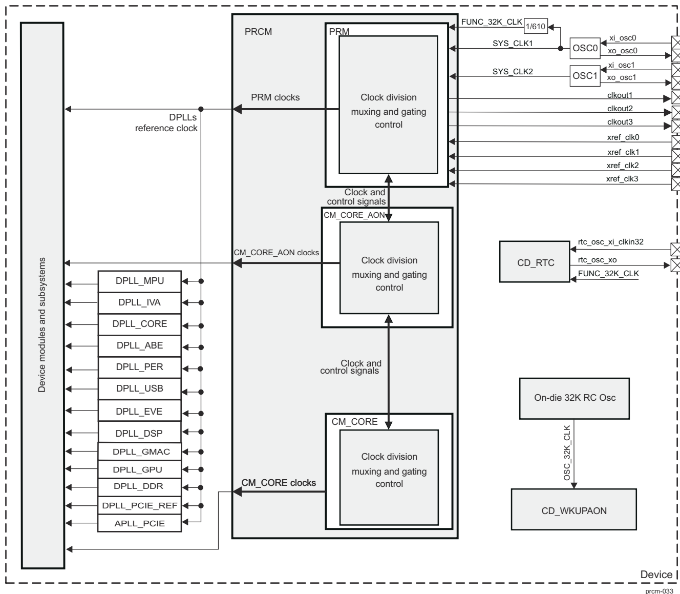
Figure 3-38. PRCM Module Clock Manager Overview
