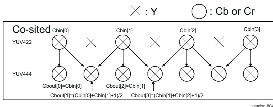
Figure 9-65. ISS ISP IPIPE YUV422 to 444 in co-sited mode
