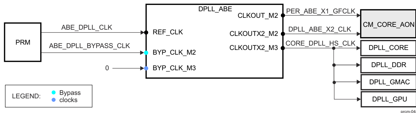
Figure 3-54. DPLL_ABE Overview
