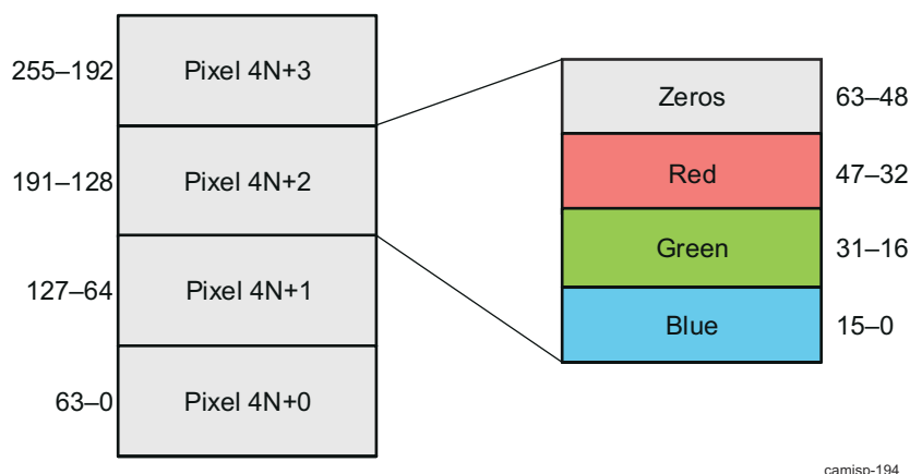
Figure 9-90. ISS ISP IPIPE Boxcar Data Packing in SDRAM
