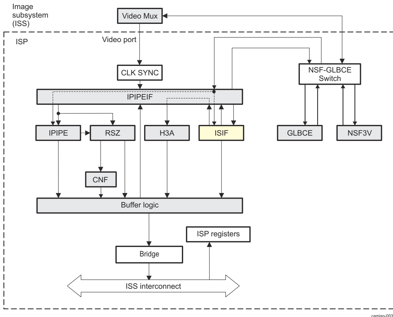
Figure 9-121. ISS ISP ISIF High-Level Diagram
