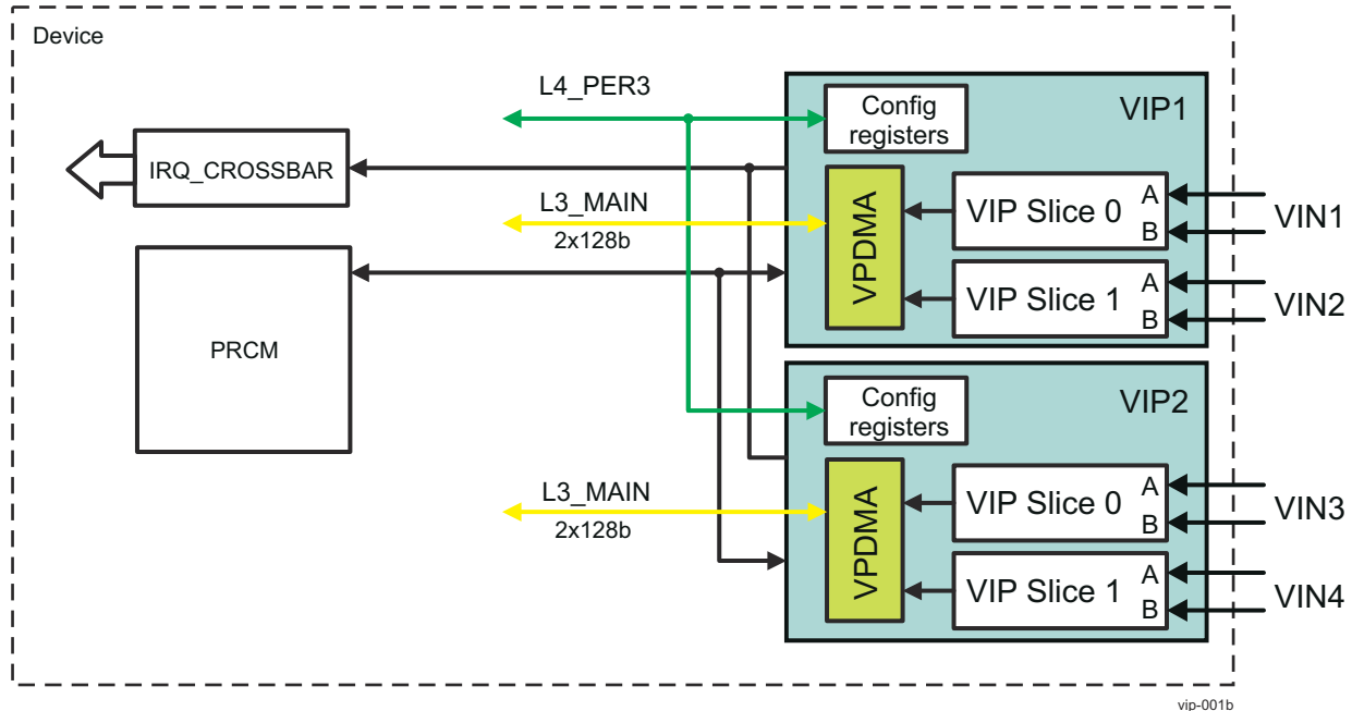
Figure 11-1. VIP Overview
