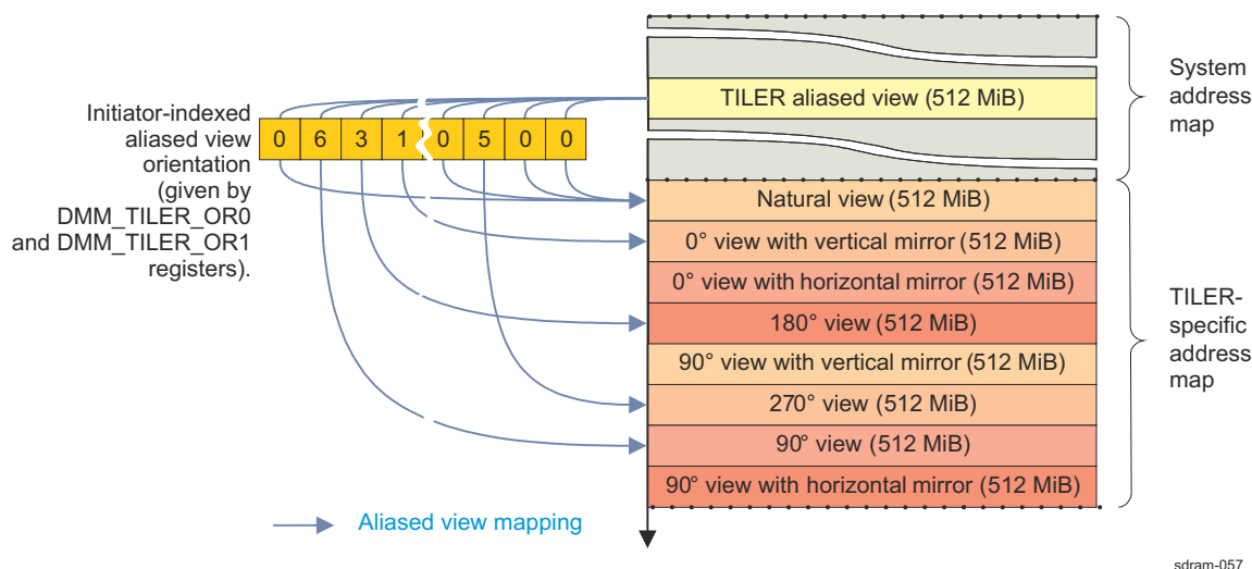
Figure 17-38. TILER Aliased View Orientation
