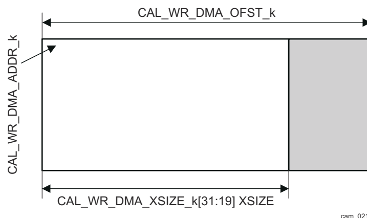
Figure 9-17. Write DMA - Framing
