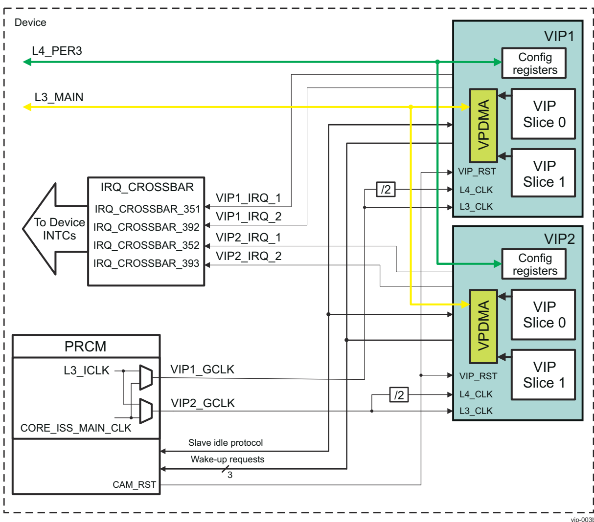
Figure 11-3. VIP Integration
