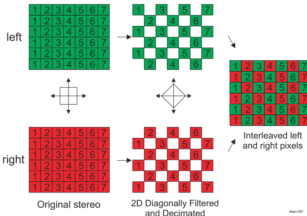
Figure 13-99. DISPC Illustration of DLP 3D Format
