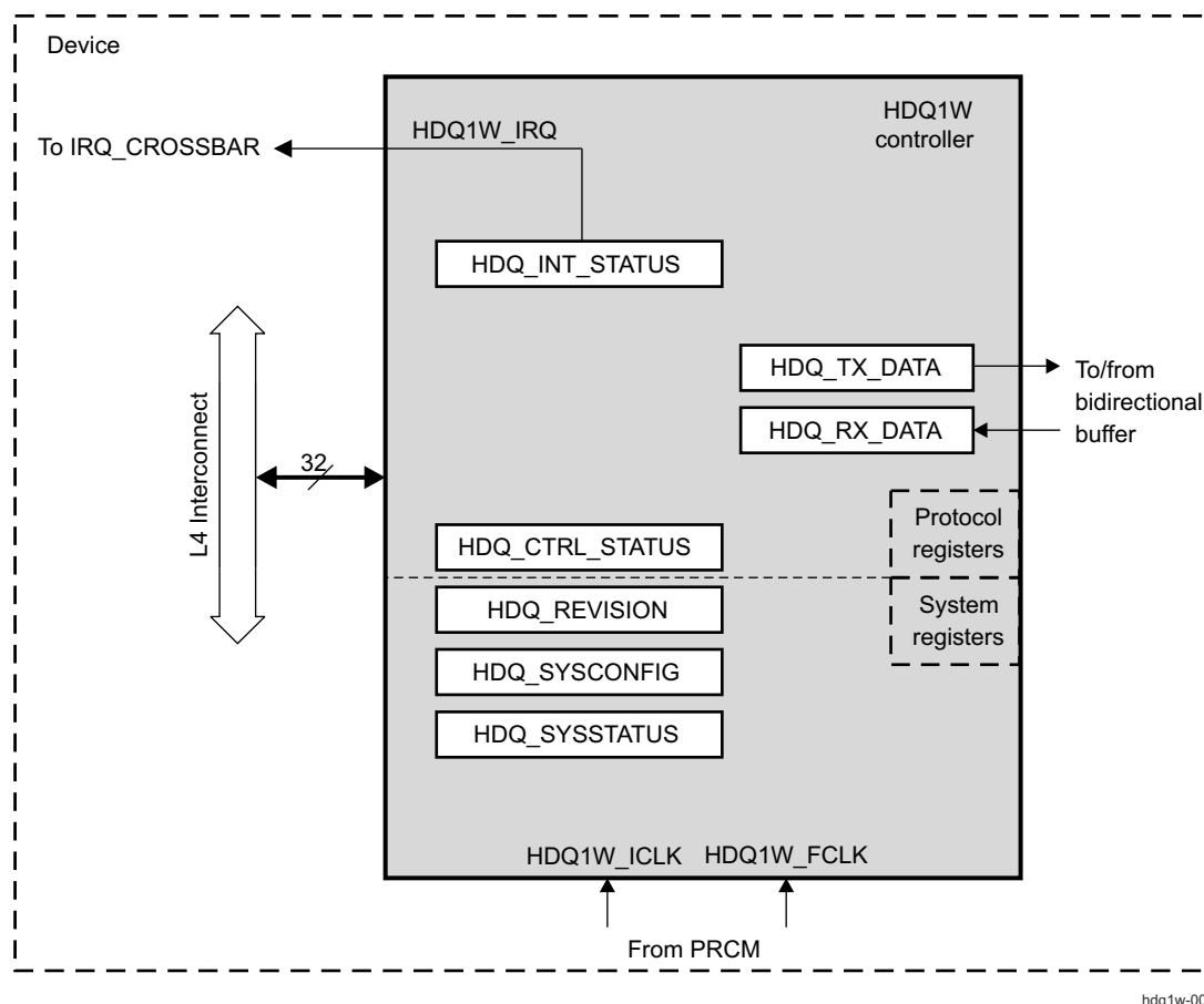
Figure 26-35. HDQ1W Block Diagram
