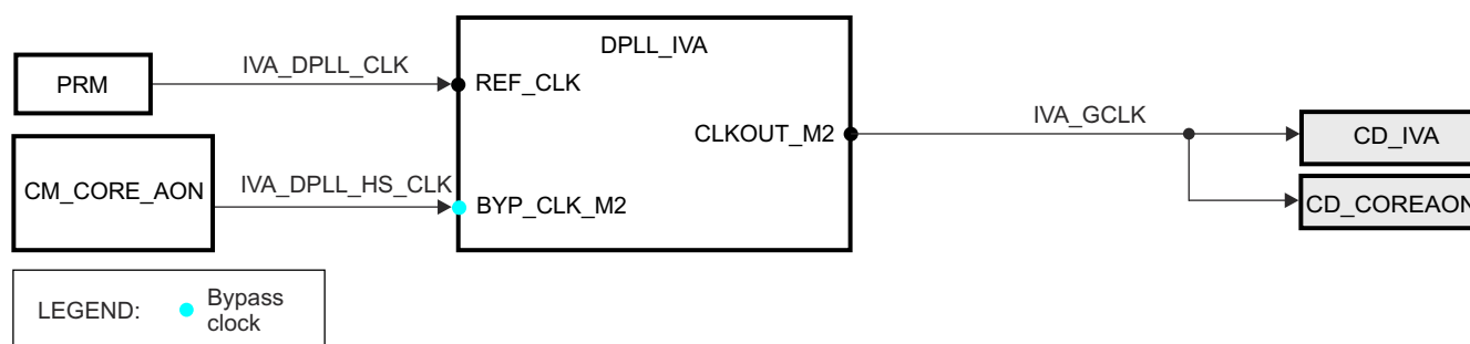
Figure 3-56. DPLL_IVA Overview
