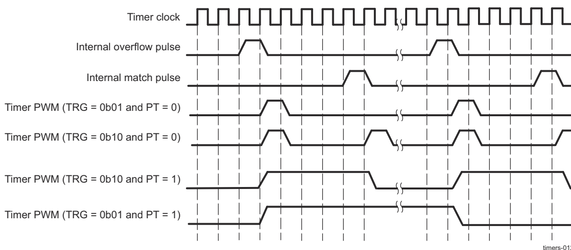
Figure 24-13. Timing Diagram of PWM With TCLR[7] SCPWM Bit = 0
