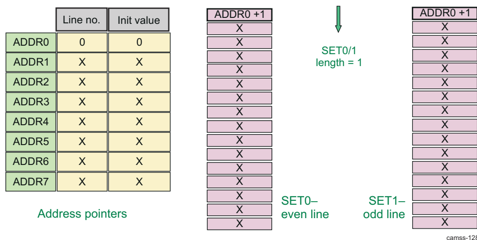
Figure 9-131. ISS ISP ISIF Conventional Read-Out Pattern
