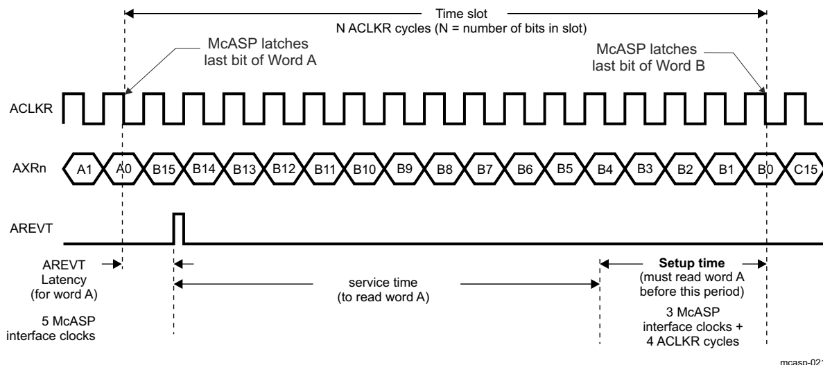
Figure 26-129. CPU Service Time Upon Receive Event (AREVT)
