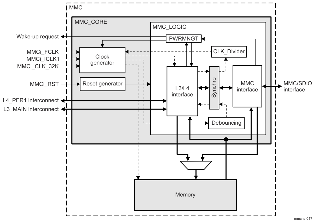
Figure 27-15. eMMC/SD/SDIO Diagram
