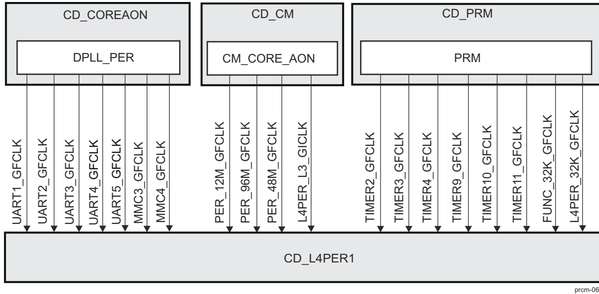
Figure 3-70. CD_L4PER1 Overview
