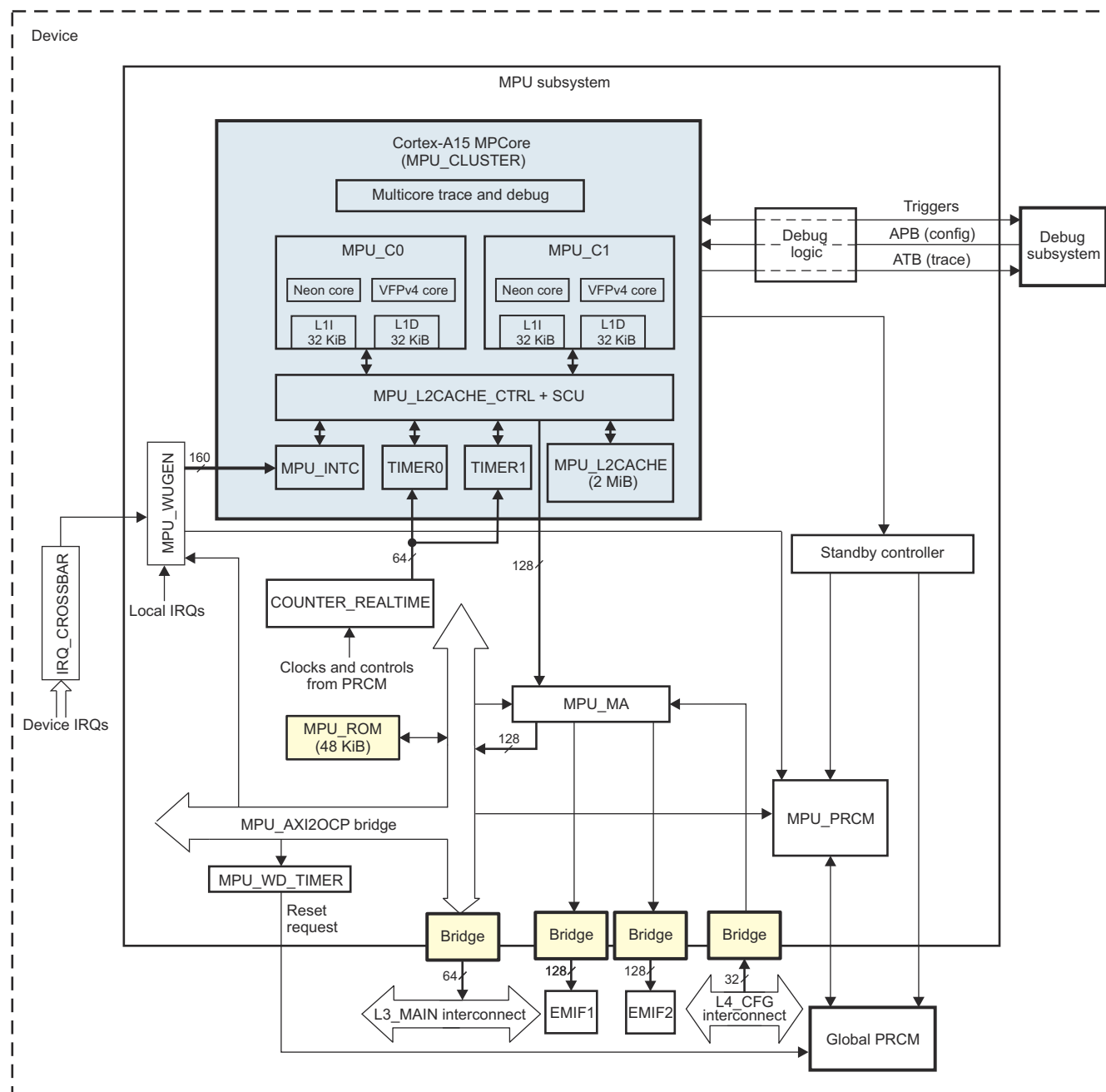
Figure 4-1. MPU Subsystem Overview
