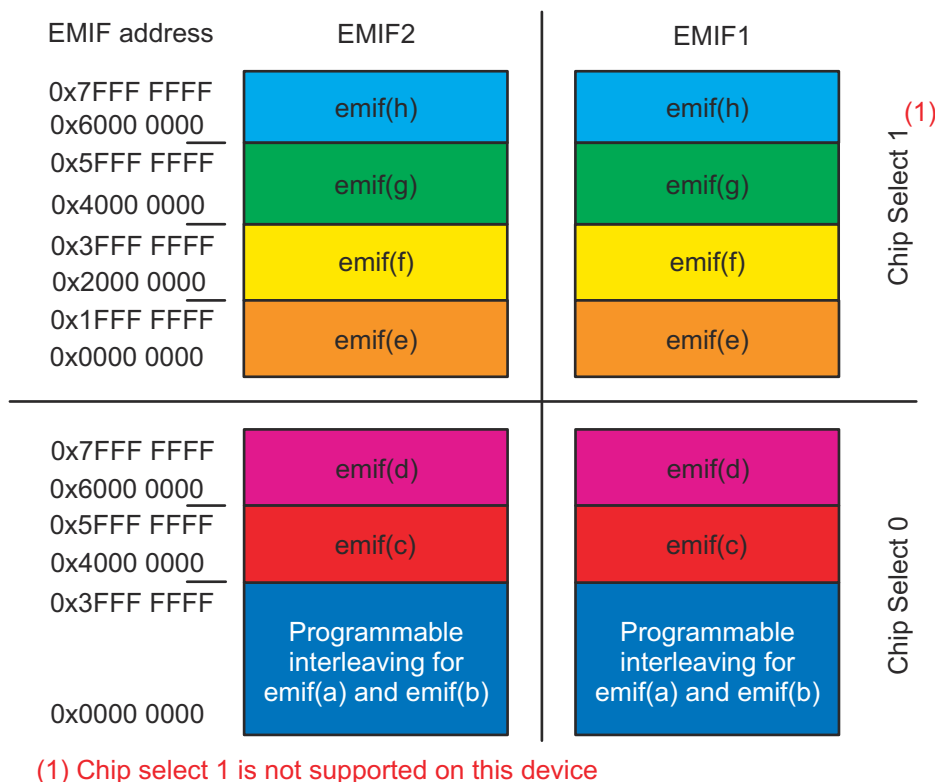
Figure 4-8. Fixed MPU-to-EMIF Address Mapping With High-Order Interleaving
