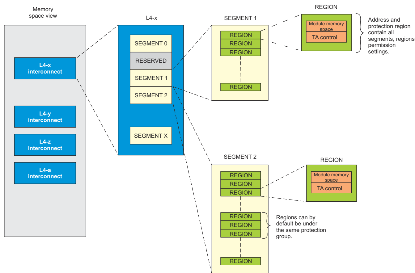
Figure 16-12. L4 Segmentation
