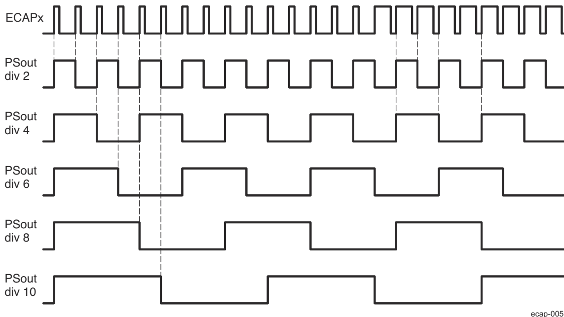
Figure 31-57. Prescale Function Waveforms
