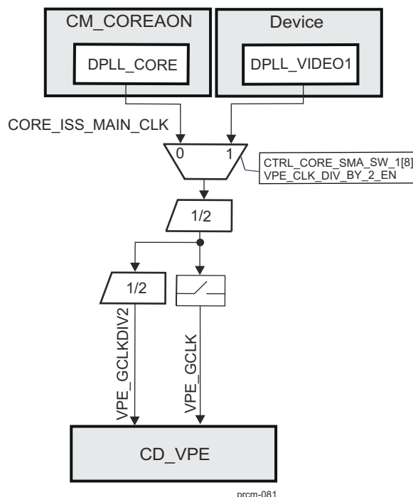
Figure 3-90. CD_VPE Overview
