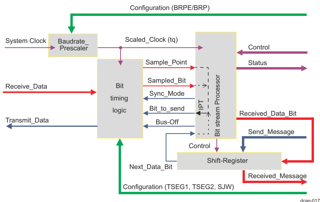
Figure 26-178. Structure of the CAN Core's CAN Protocol Controller
