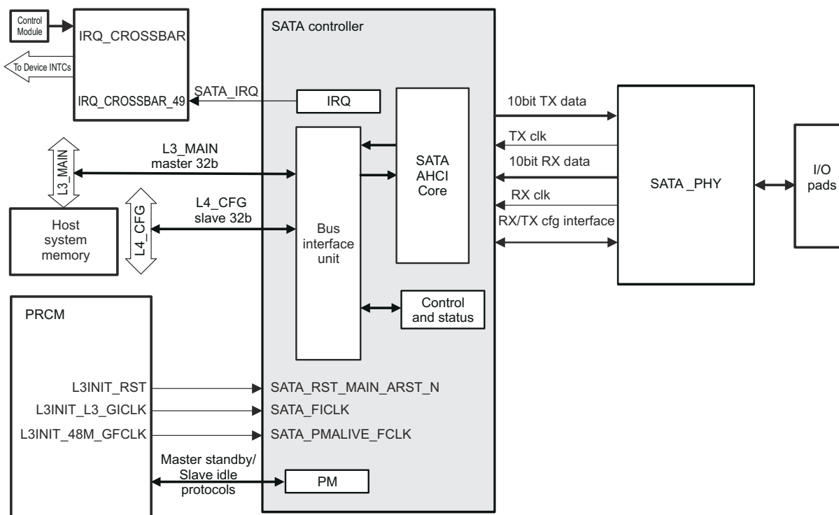
Figure 26-153. SATA Controller Integration
