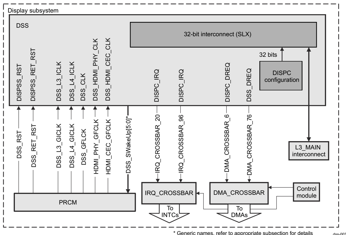
Figure 13-3. Display Subsystem Integration
