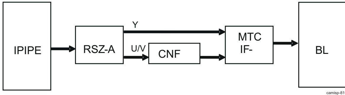
Figure 9-35. ISS ISP NSF3V High-Level Diagram
