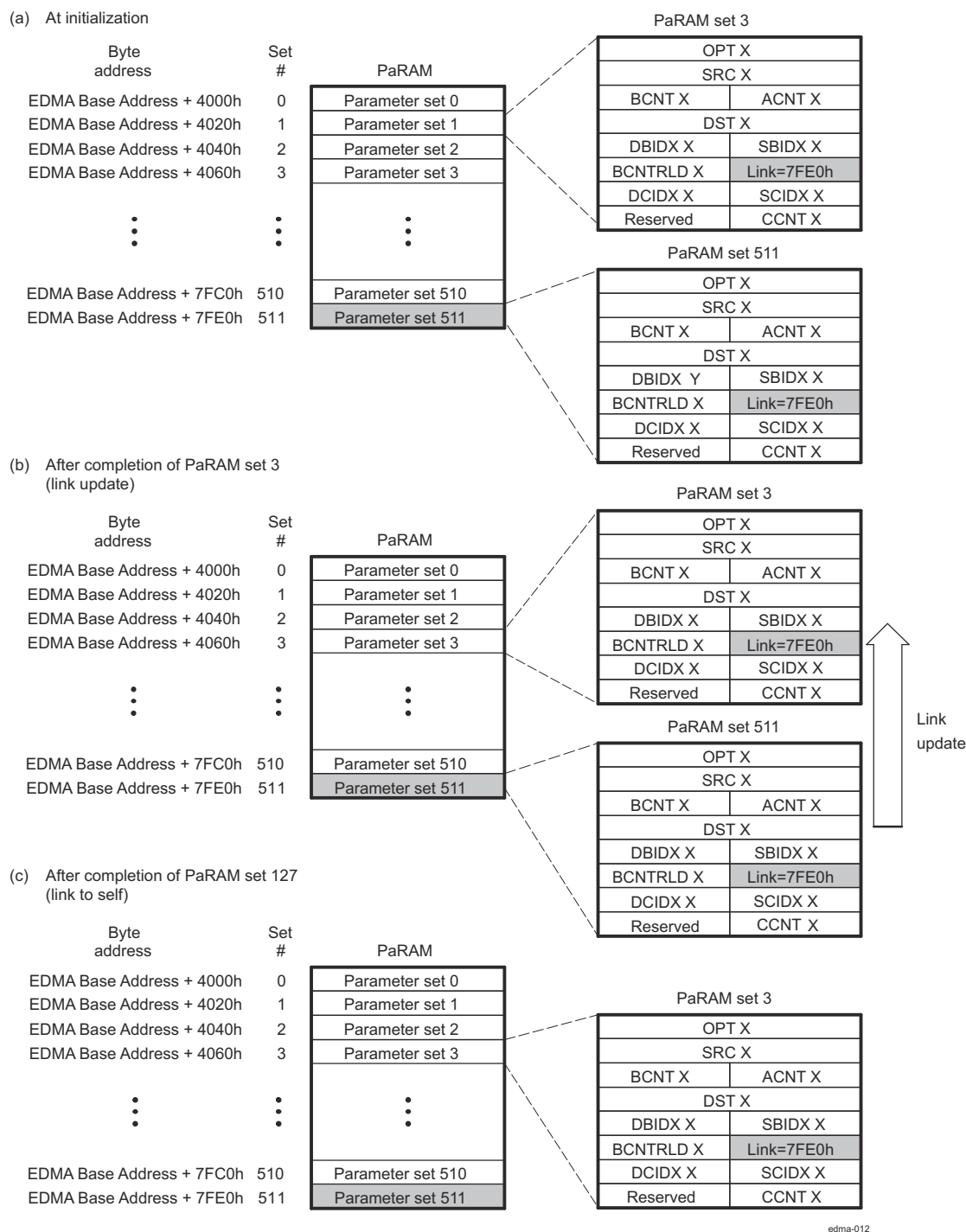
Figure 18-23. Link-to-Self Transfer
