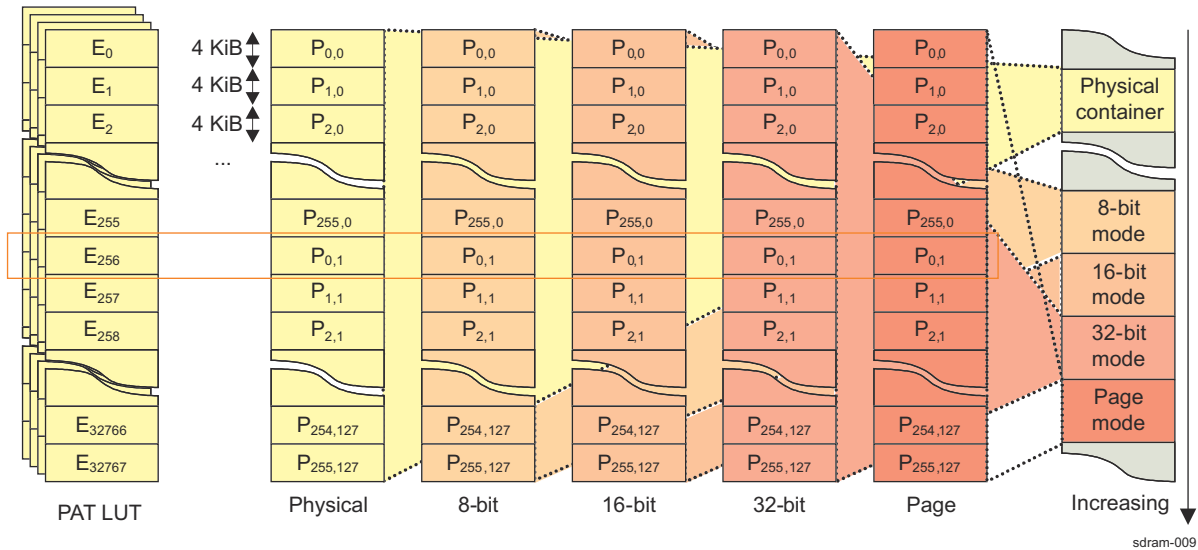
Figure 17-14. TILER Page Mapping When Using 4-kiB Pages
