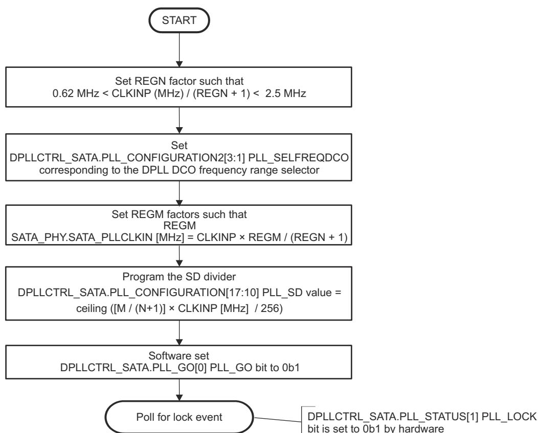
Figure 28-7. SATA PLL Programming Sequence
