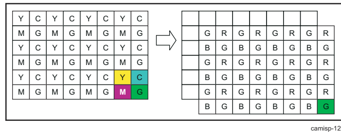
Figure 9-146. ISS ISP ISIF Last Pixel/Last Line Generation
