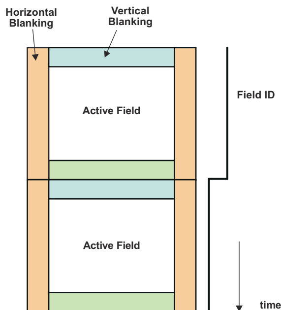
Figure 11-19. Digitized Video
