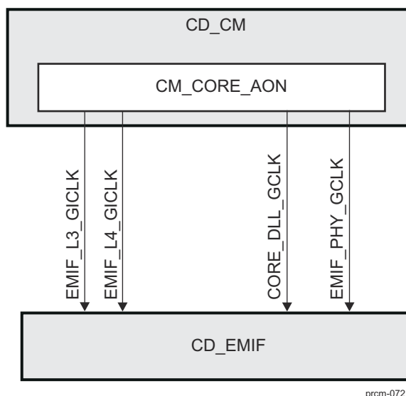
Figure 3-82. CD_EMIF Overview
