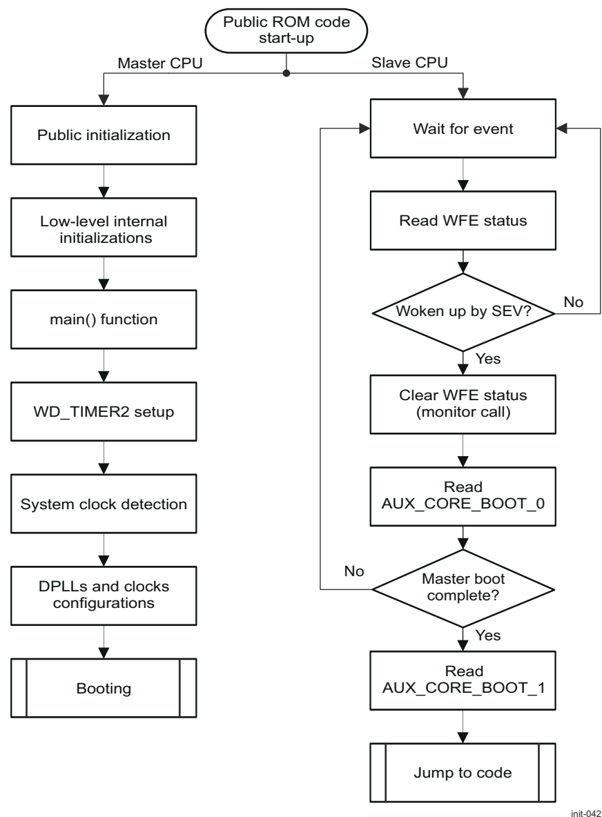
Figure 34-8. ROM Code Multiprocessor Start-Up Sequence
