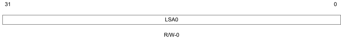
Figure 8-41. Loop 0 Start Address Register (LSA0)
