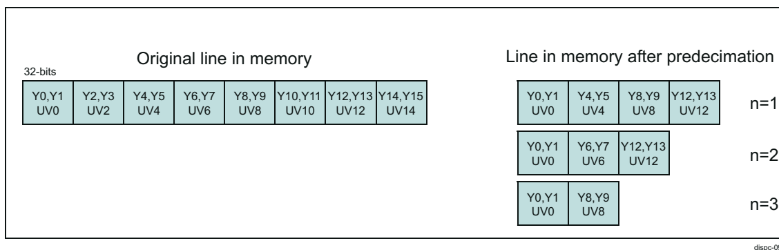
Figure 13-45. YUV4:2:2 Predecimation
