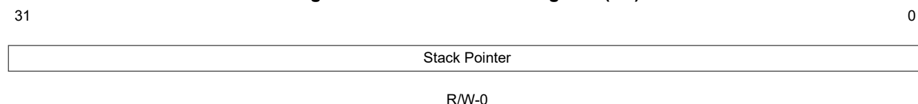
Figure 8-38. Stack Pointer Register (SP)
