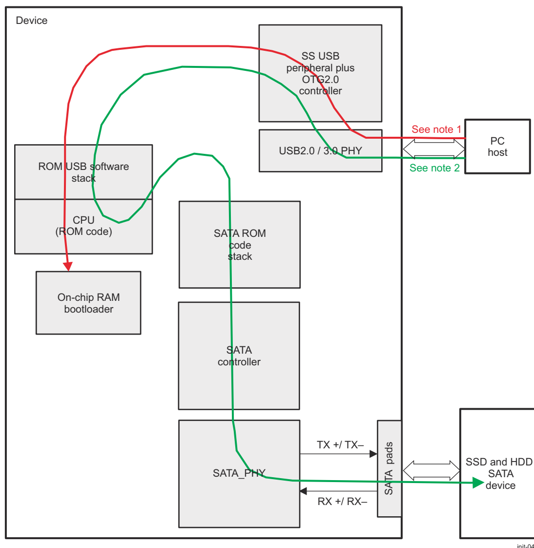
Figure 34-13. SATA Flashing Over USB
