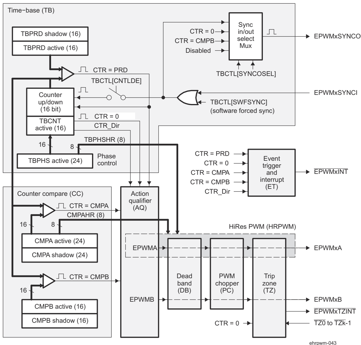
Figure 31-47. HRPWM System Interface
