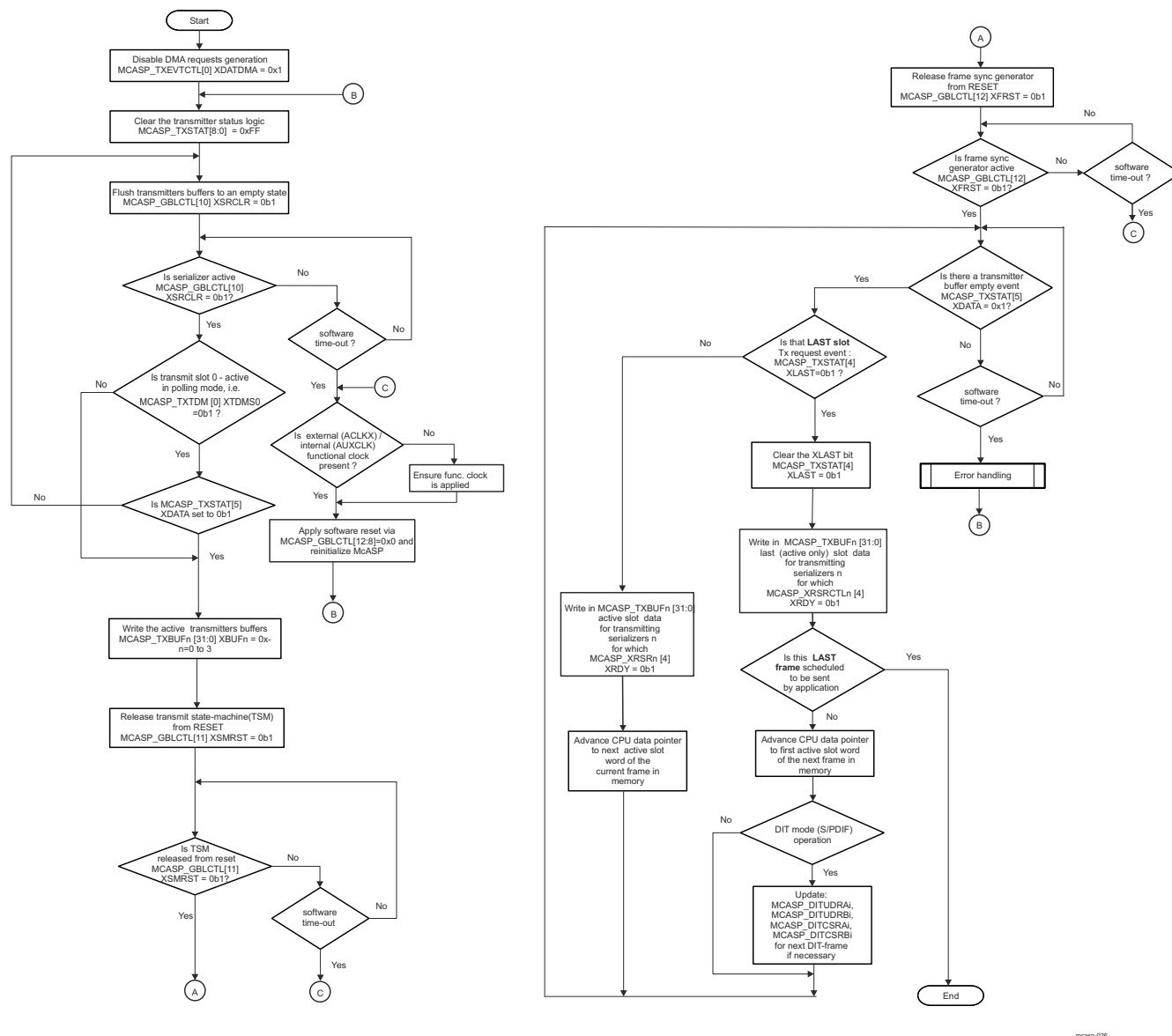
Figure 26-135. McASP DIT- /TDM- Transmission Polling Method
