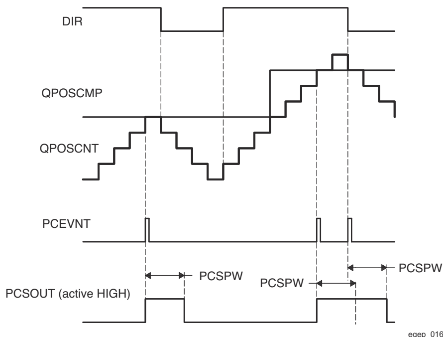
Figure 31-75. eQEP Position-compare Sync Output Pulse Stretcher
