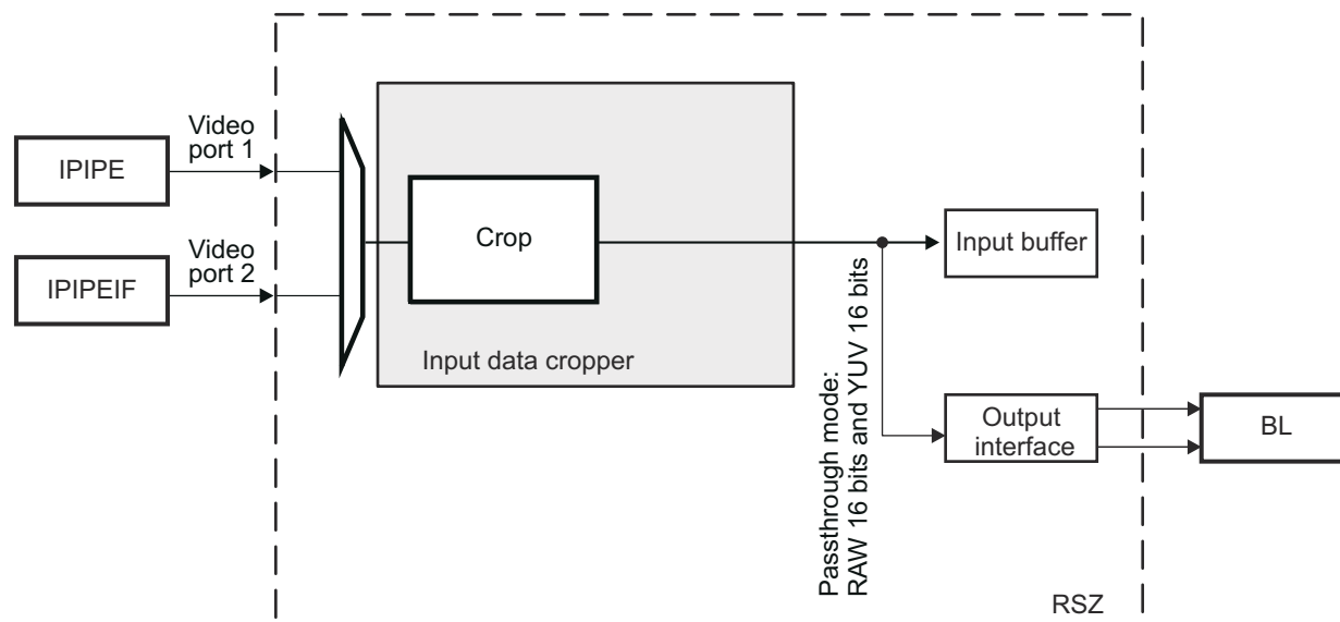
Figure 9-97. ISS ISP RSZ Input Data Cropper Block Diagram
