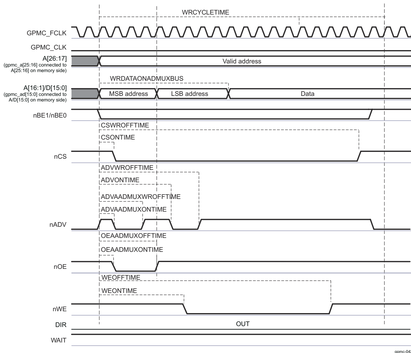
Figure 17-69. Asynchronous Single Write on an AAD-Multiplexed Device
