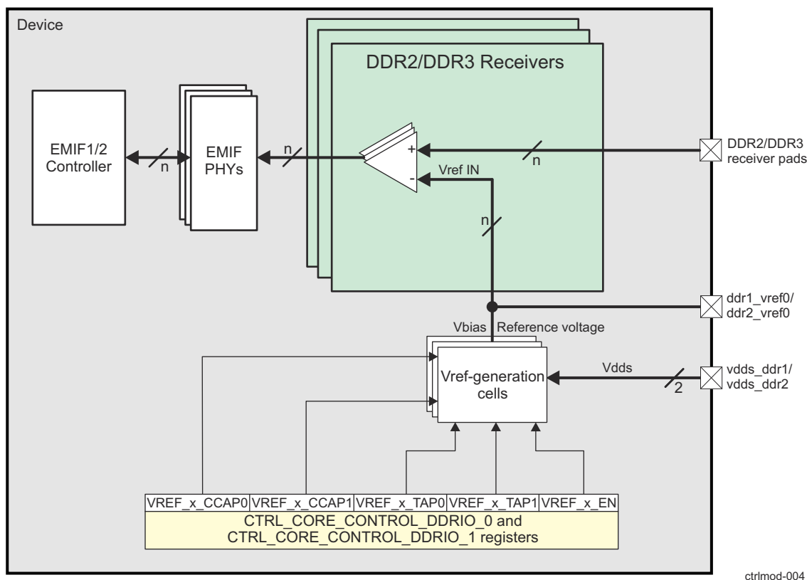
Figure 20-12. Vref-Generation Cells and Their Controls
