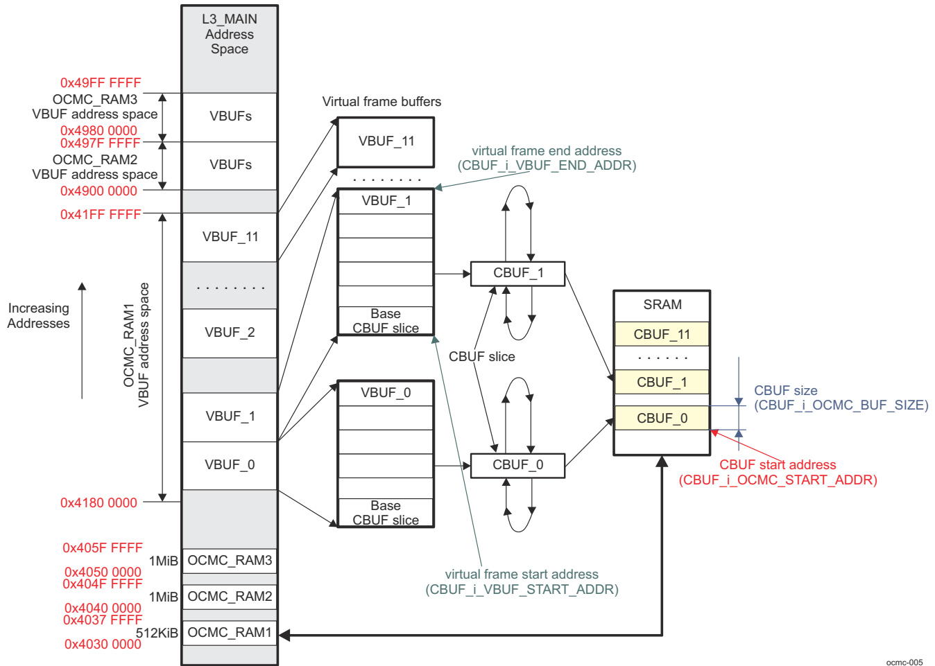
Figure 17-109. VBUF to CBUF Address Mapping
