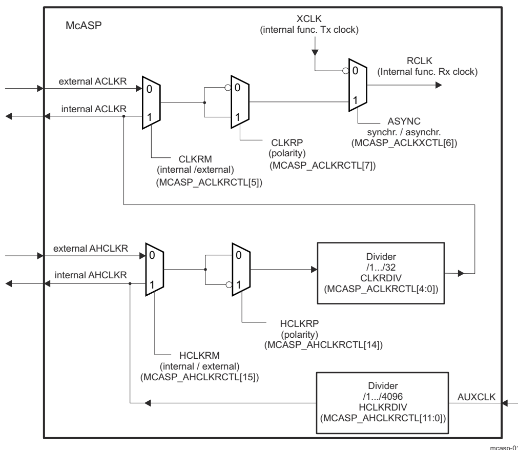
Figure 26-121. Receive Clock Generator Block Diagram
