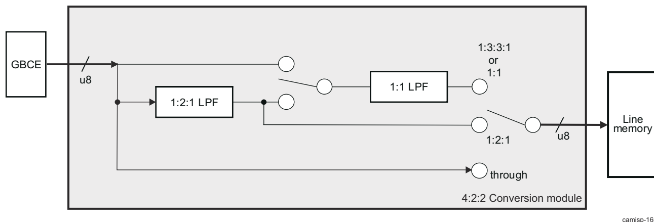
Figure 9-77. ISS ISP IPIPE 4:2:2 Conversion Module Block Diagram
