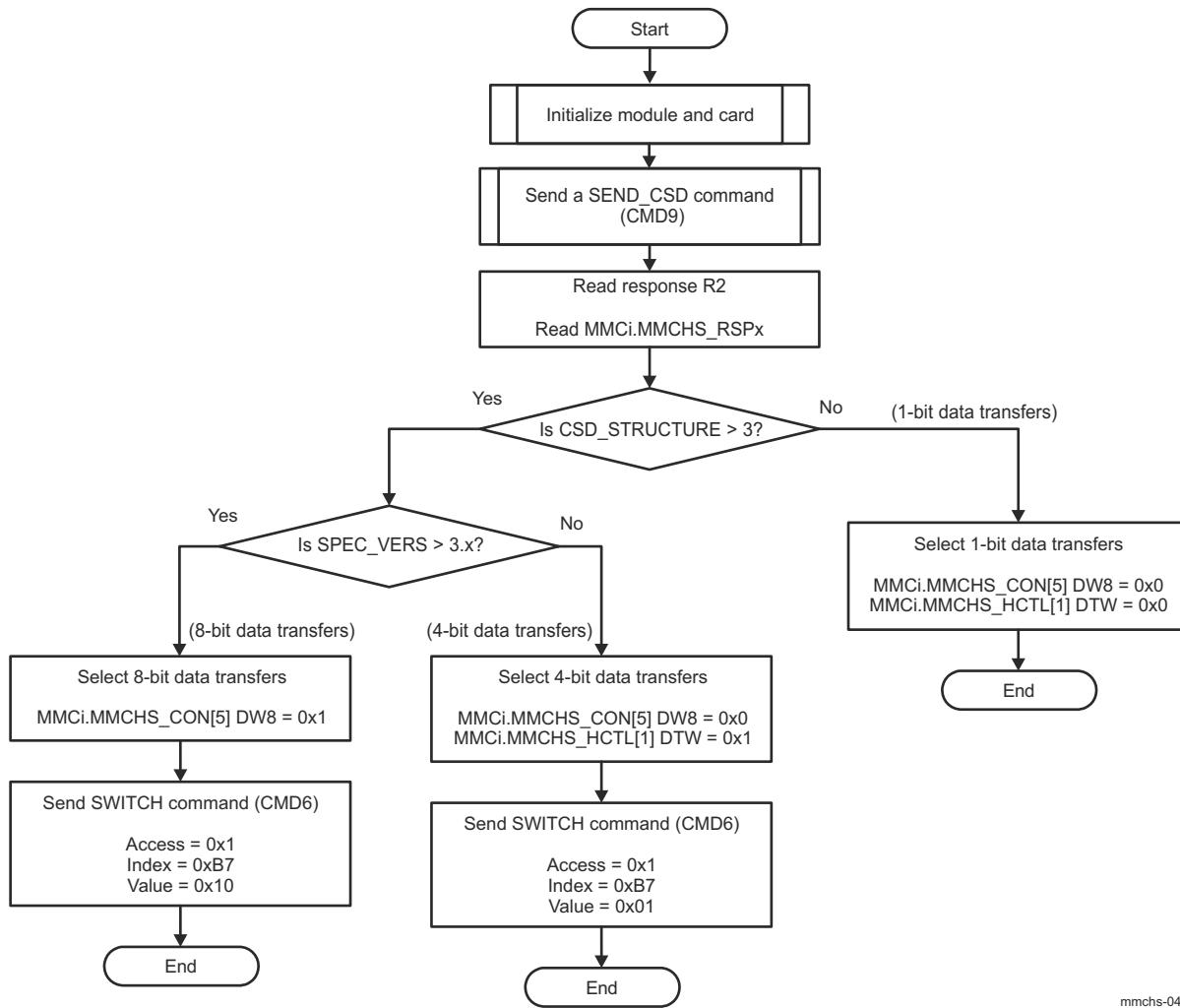
Figure 27-47. eMMC/SD/SDIO Controller Bus Width Configuration Flow
