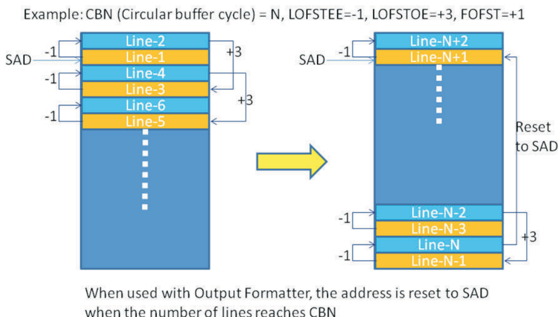
Figure 9-168. ISS ISP ISIF Combination of Circular Buffer and Output Formatter
