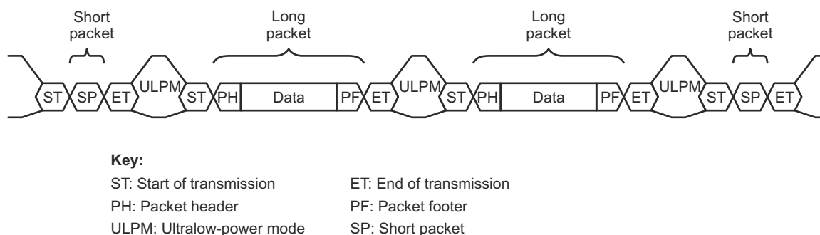
Figure 10-15. CSI2 Protocol Layer With Short and Long Packets
