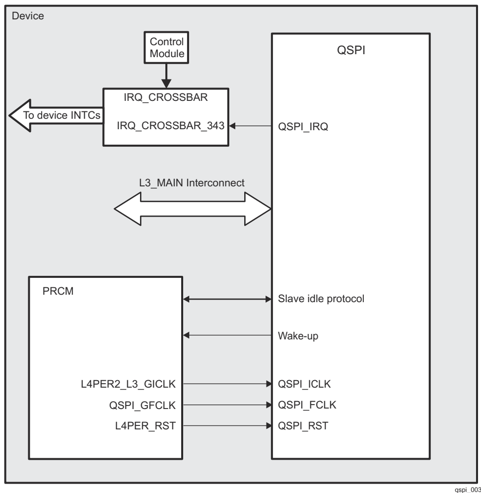
Figure 26-103. QSPI Integration
