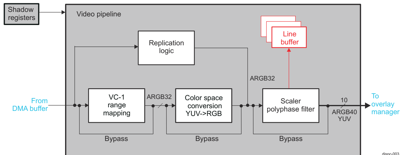
Figure 13-48. DISPC Configuration 1: Video Pipeline
