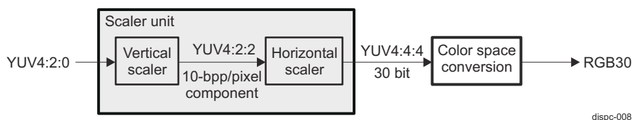
Figure 13-57. DISPC YUV4:2:0 to RGB30 Using Scaler Unit for Resampling Chrominance
