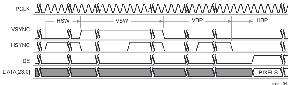
Figure 13-36. DISPC Active Matrix Timing Diagram of Configuration 3 (Start of Frame)
