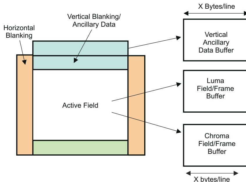
Figure 11-41. Interlaced Field Vertical Blanking Ancillary Data Storage
