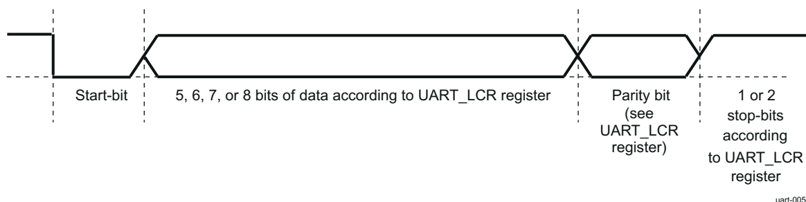
Figure 26-39. UART Frame Data Format
