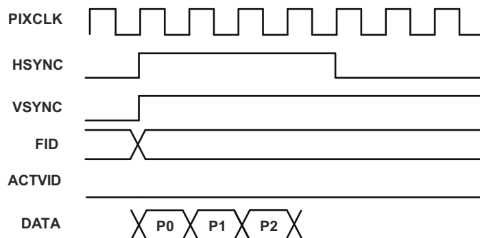
Figure 11-27. Type 1, First Horizontal Blanking Pixel
