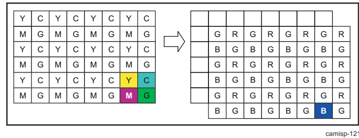
Figure 9-145. ISS ISP ISIF Second Last Pixel/Last Line Generation
