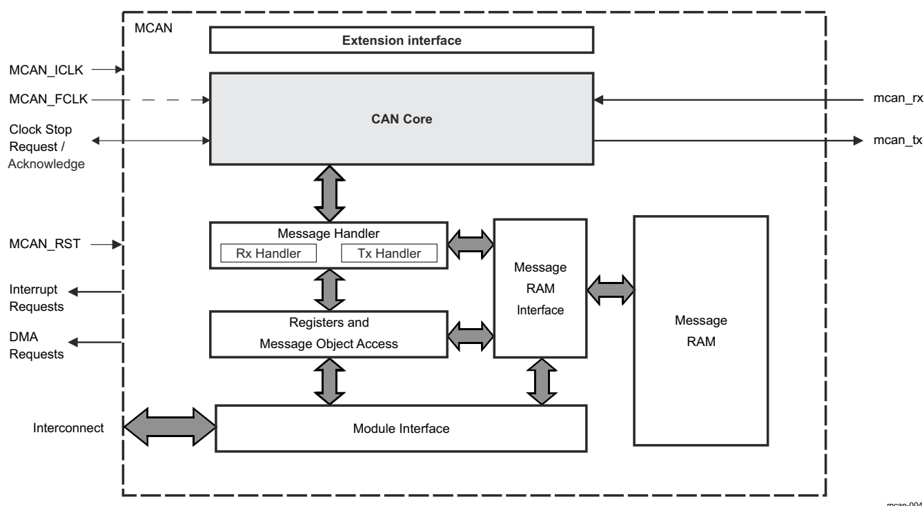
Figure 26-189. MCAN Block Diagram
