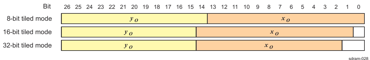
Figure 17-19. Tiled Mode Addressing in 0- or 180-Degree Orientation (S = 0)
