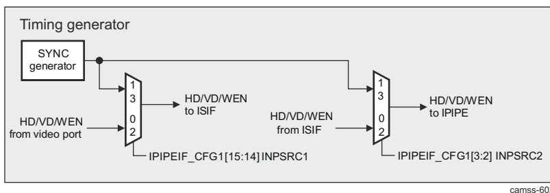
Figure 9-49. ISS ISP IPIPEIF Timing Generator Submodule
