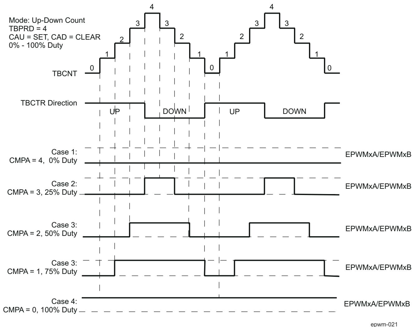
Figure 31-25. ePWM Up-Down-Count Mode Symmetrical Waveform
