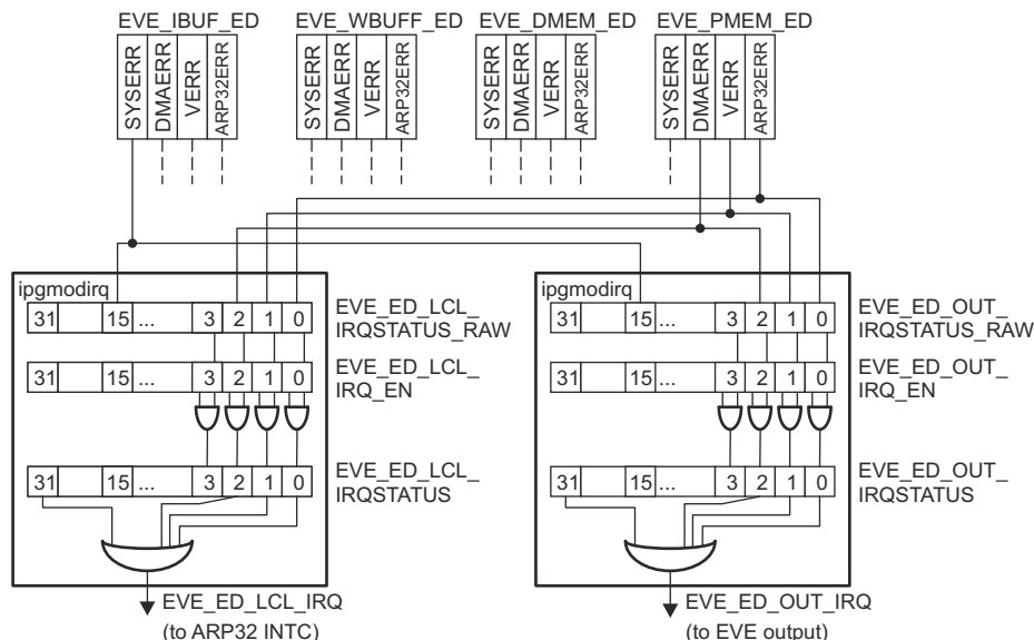
Figure 8-18. EVE Parity/Error Detect Interrupt
