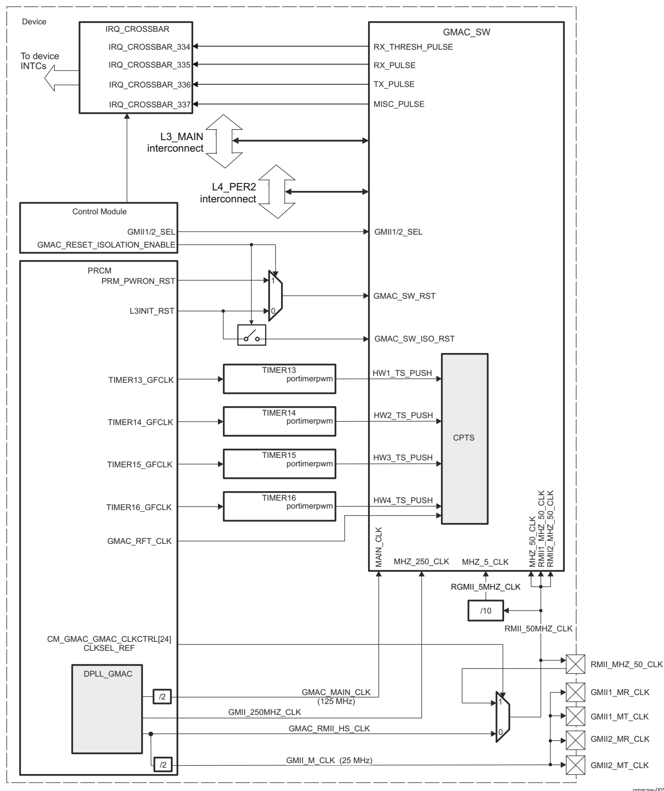
Figure 26-211. GMAC_SW Integration
