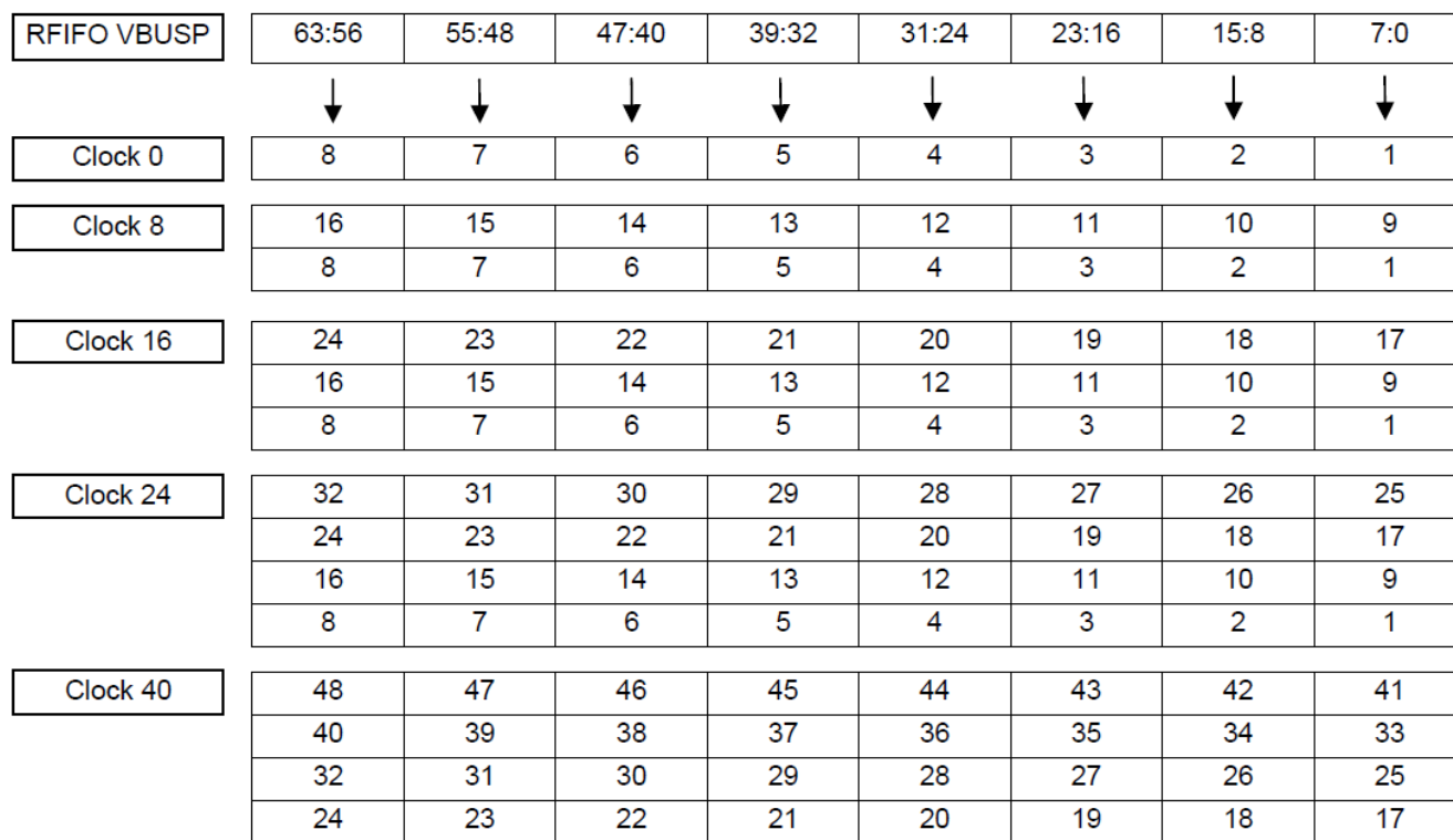
Figure 26-220. Packet Octets as Stored in the Packet Buffer
