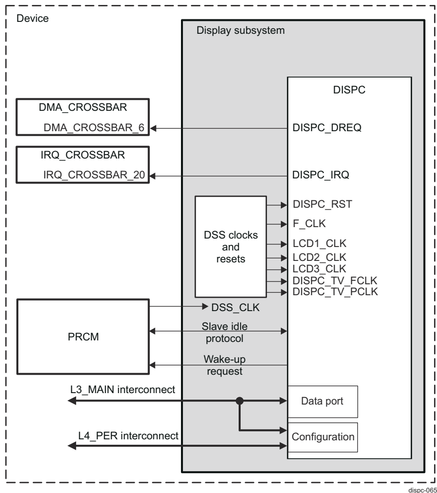
Figure 13-41. DISPC Integration
