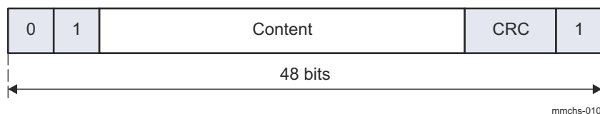
Figure 27-7. Command Token Format
