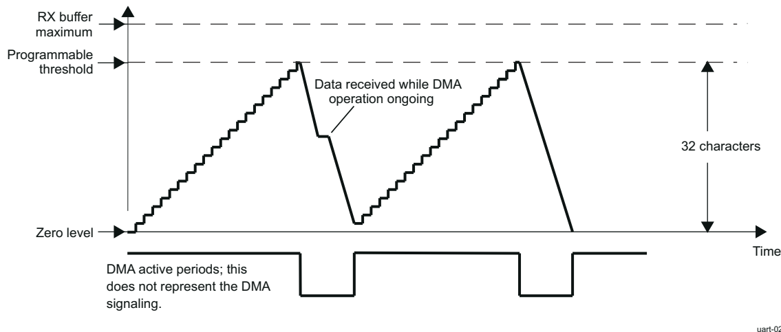
Figure 26-62. Receive FIFO DMA Request Generation (32 Characters)
