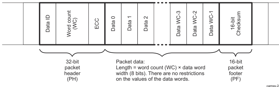
Figure 10-17. CSI2 Long Packet Structure
