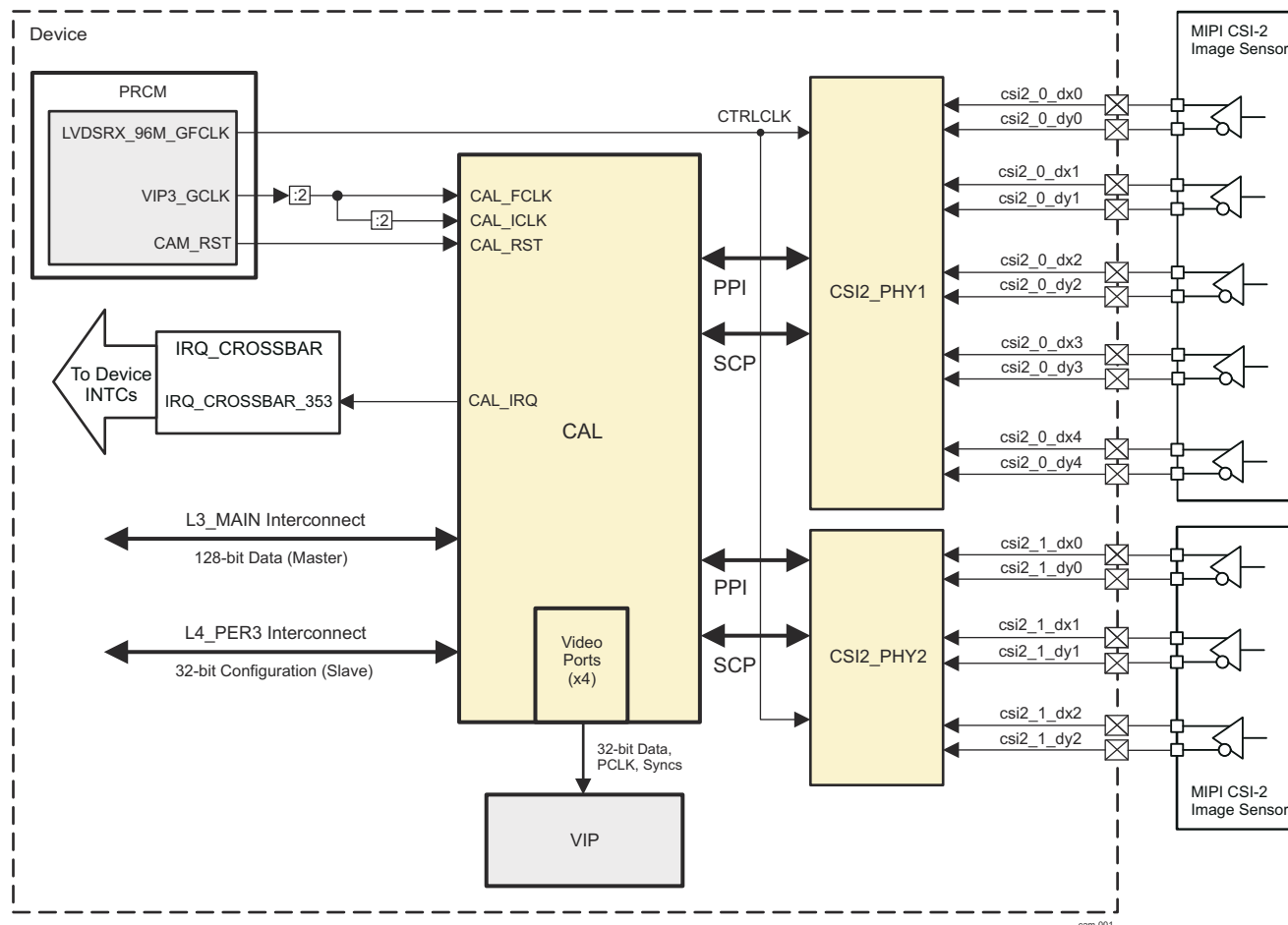
Figure 10-1. CAMSS Overview
