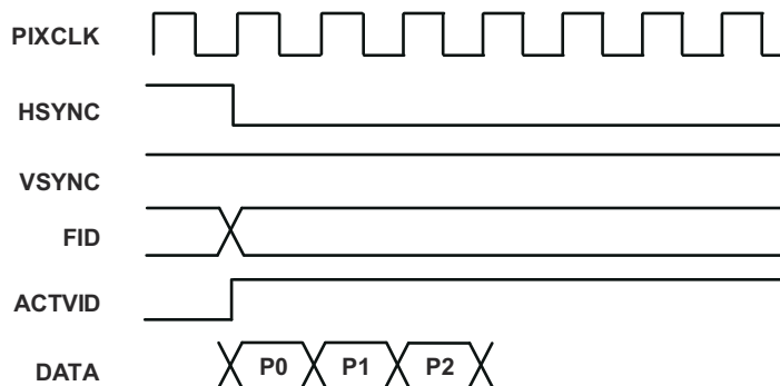
Figure 11-28. Type 1, First Vertical Ancillary Data Pixel
