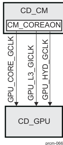
Figure 3-76. CD_GPU Overview
