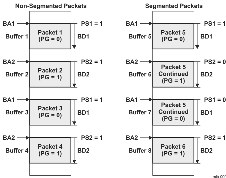
Figure 26-235. Single-Packet Mode Memory Space
