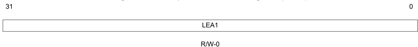
Figure 8-45. Loop 1 End Address Register (LEA1)
