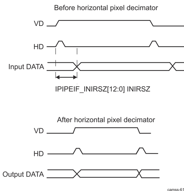
Figure 9-53. ISS ISP IPIPEIF Resizer Offset Definition
