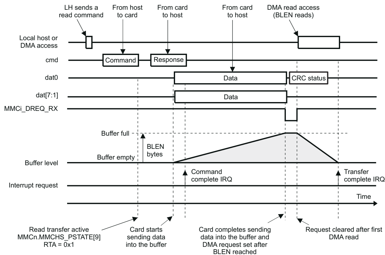
Figure 27-18. DMA Receive Mode
