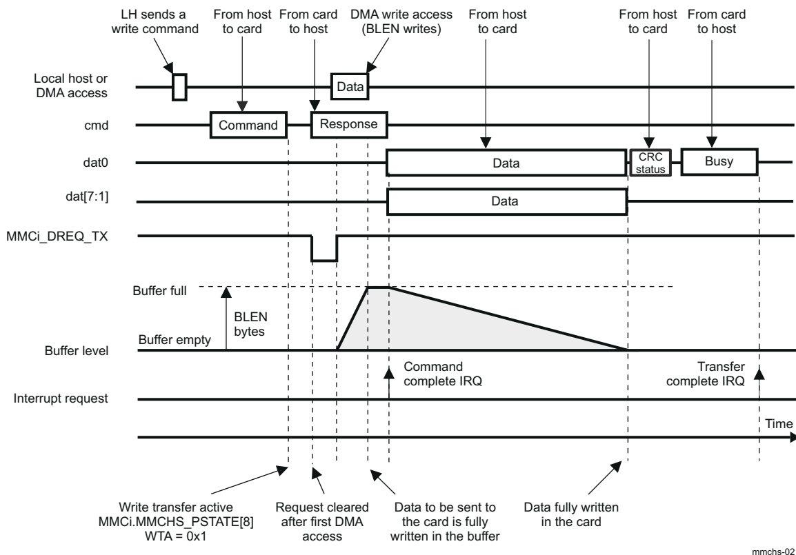
Figure 27-19. DMA Transmit Mode
