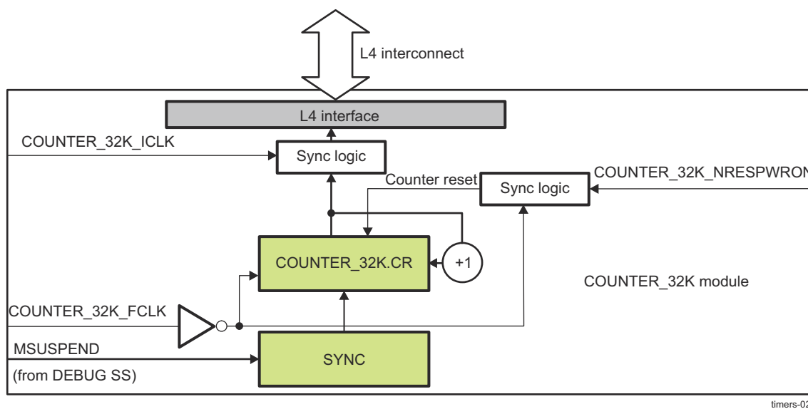
Figure 24-17. COUNTER_32K Block Diagram
