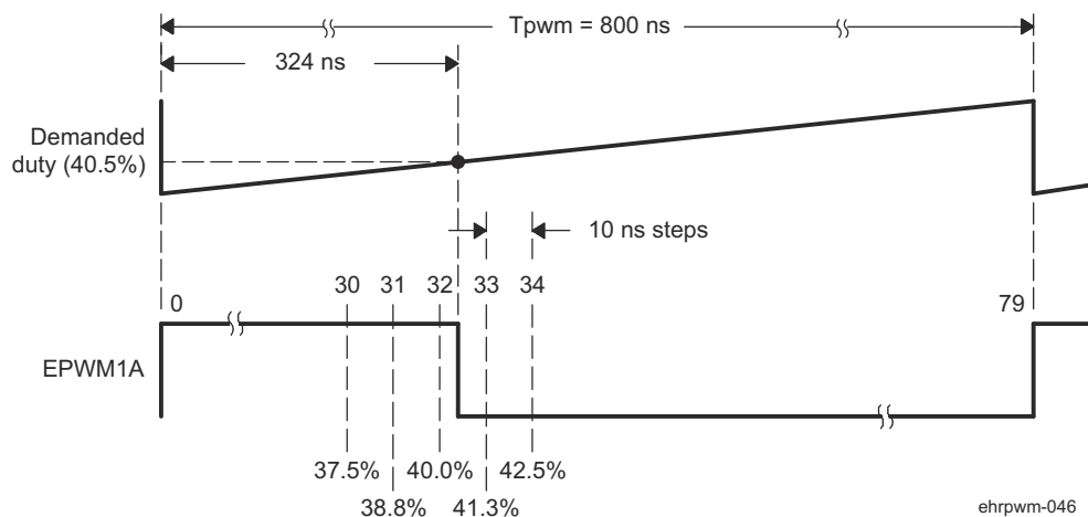
Figure 31-50. Required PWM Waveform for a Requested Duty = 40.5%
