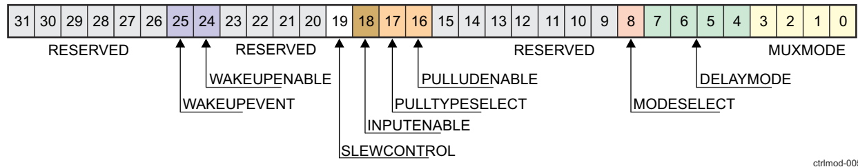
Figure 20-4. Pad Configuration Register Bits
