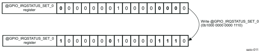
Figure 29-13. Write in GPIO_IRQSTATUS_SET_0 Register Example
