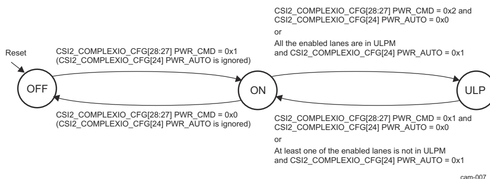
Figure 10-6. CSI2 Complex I/O Power FSM
