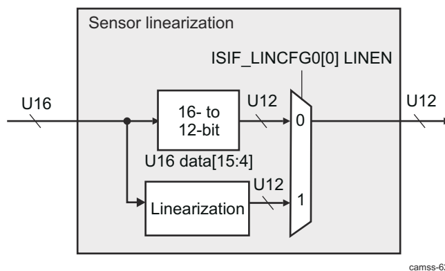
Figure 9-124. ISS ISP ISIF Sensor Linearization Block Diagram
