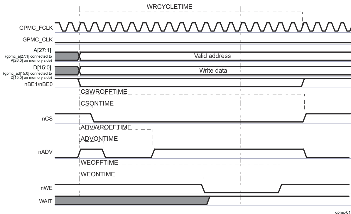
Figure 17-78. Asynchronous Single Write on an Address/Data-Nonmultiplexed Device
