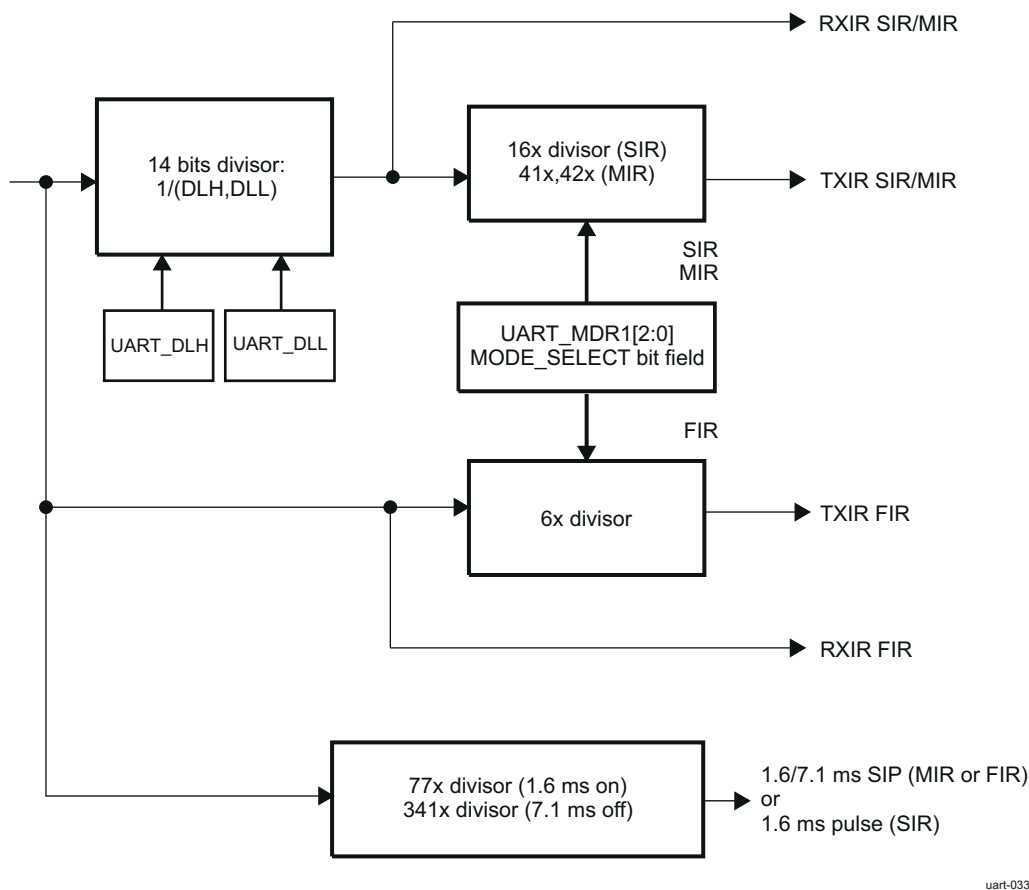
Figure 26-70. Baud Rate Generator
