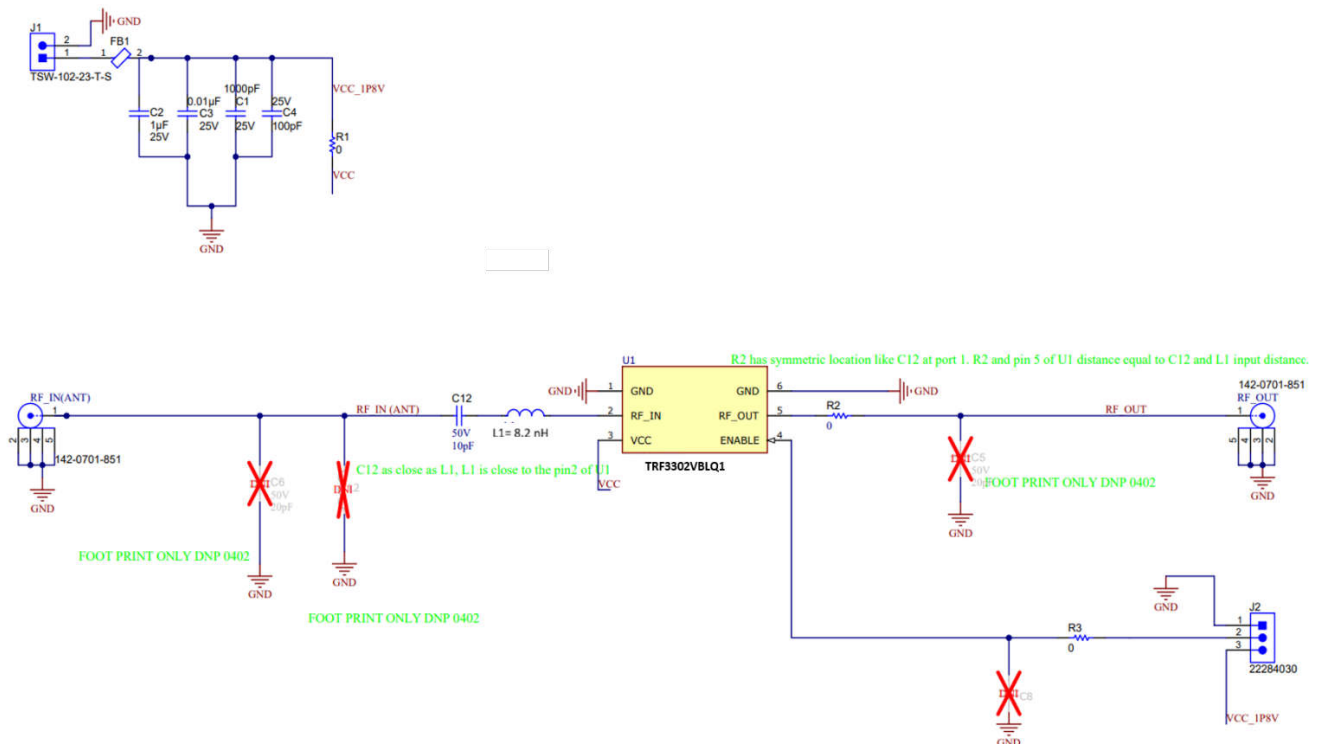
Figure 3-1. TRF3302Q1EVM Schematic for L1 Band
