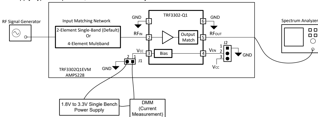
Figure 2-1. Single Tone Setup for TRF3302Q1EVM for Gain and Output P1dB
