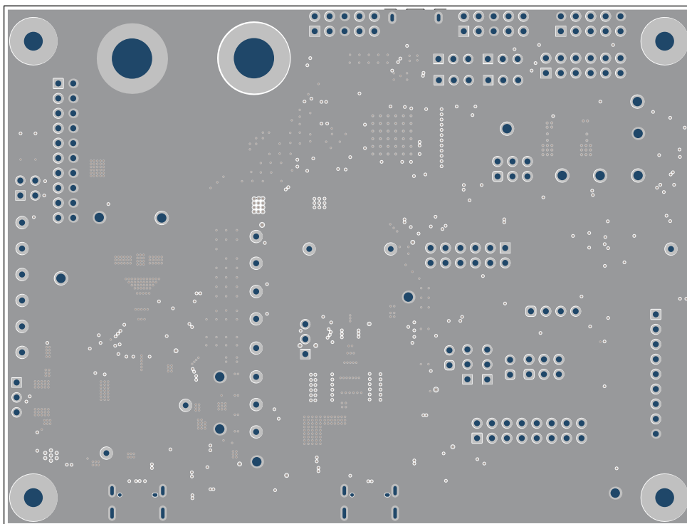
Figure 4-14. Signal Layer (2)
