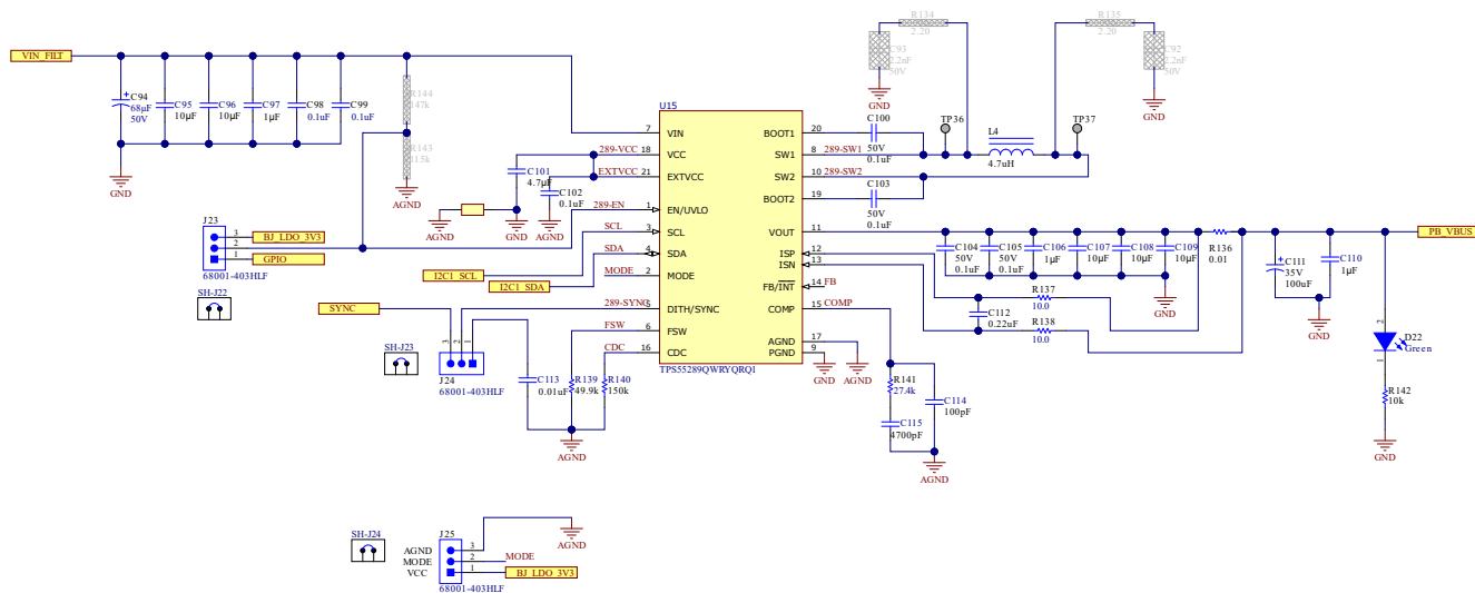
Figure 4-2. TPS55289-Q1 Schematic
