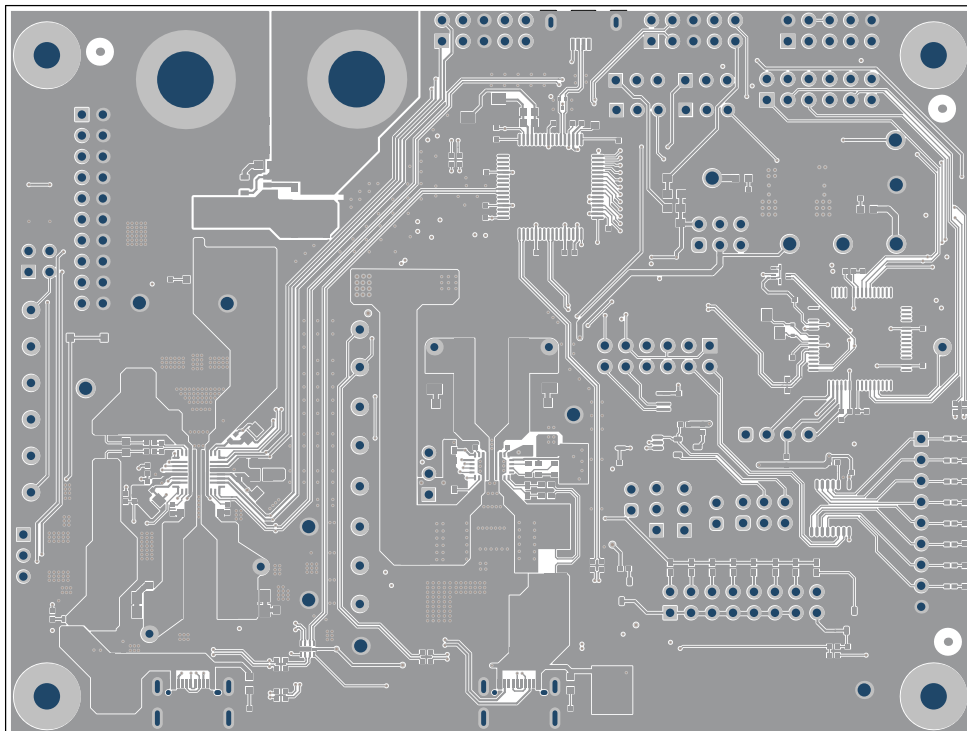
Figure 4-13. Top Layer(1)
