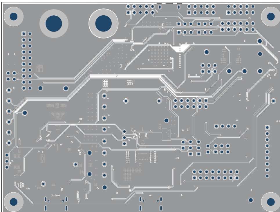
Figure 4-15. Signal Layer(3)
