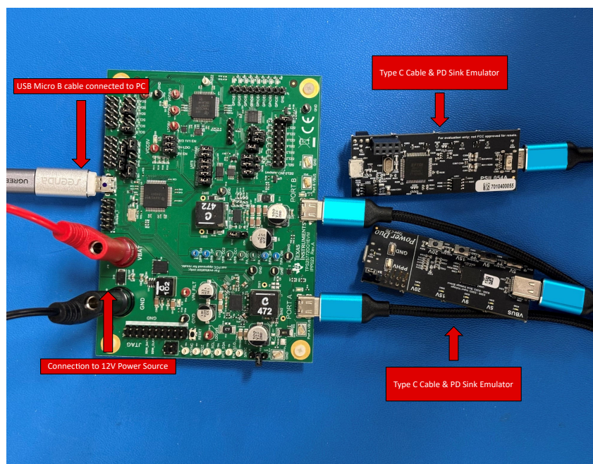
Figure 2-1. EVM Connections
