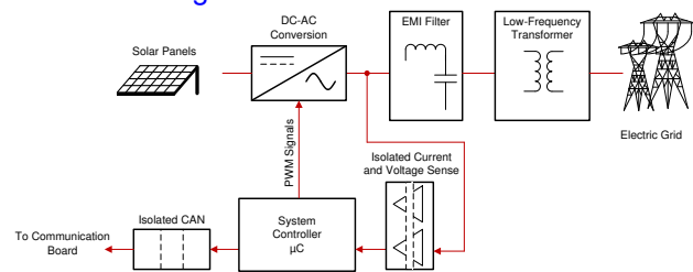
Figure 2. Isolated CAN in Solar Inverters
