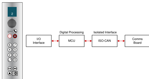
Figure 1. Isolated CAN in Elevators
