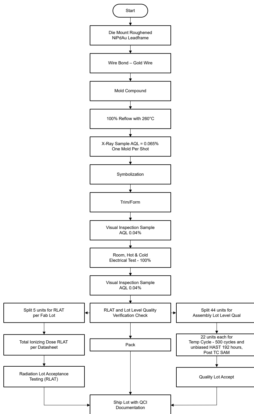
Figure 1-1. TPS7H401X-SEP Space Enhanced Plastic Production Flow Chart
