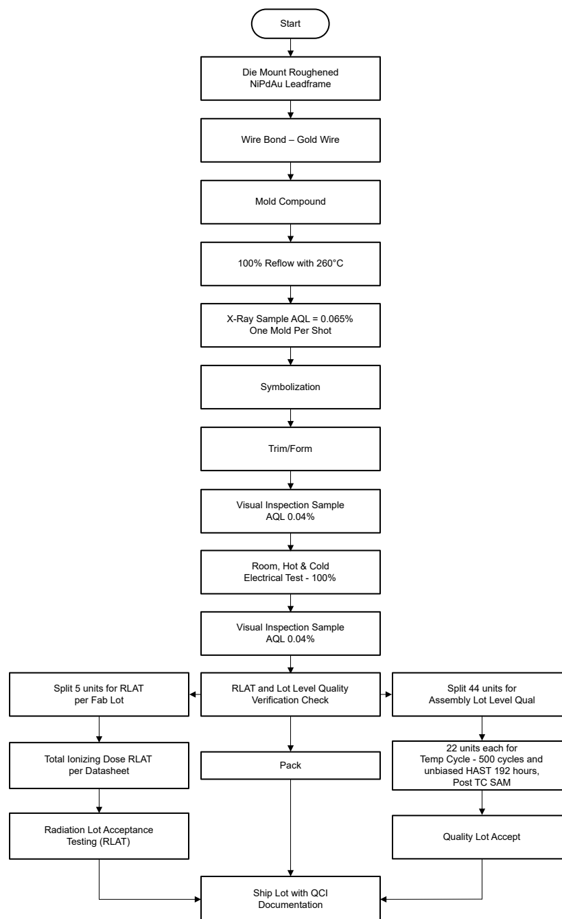
Figure 1-1. TPS7H410x-SEP Space Enhanced Plastic Production Flow Chart
