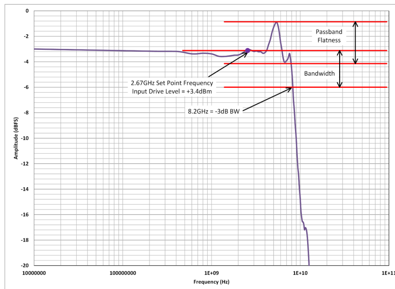
Figure 2-3. ADC Input Pass-Band Flatness Response: Bypass Mode
