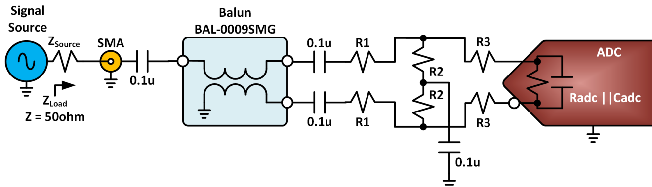
Figure 2-1. Example Input Network Connected to the ADC
