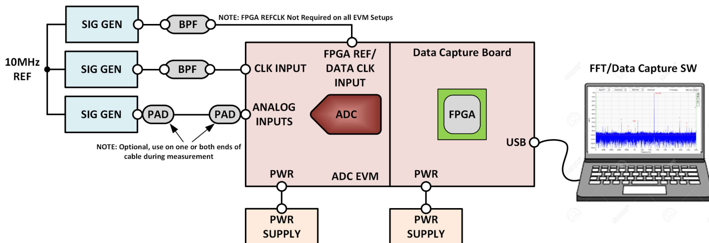
Figure 2-2. Fundamental Frequency Response Measurement Method Setup for an ADC
