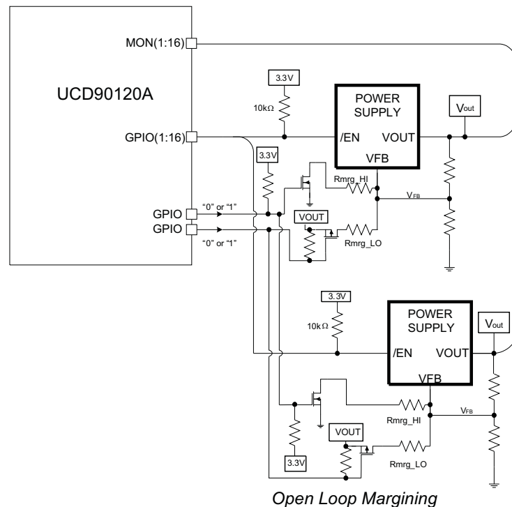
Figure 23. Open-Loop Margining
