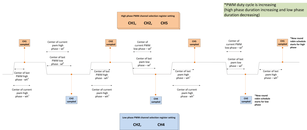
Figure 7-4. ADC center sampling mode
