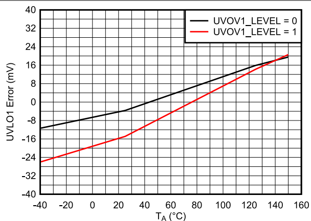
Figure 6-8. UVLO Threshold Error vs. Temperature
