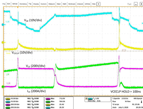
Figure 8-6. VCE Clamp Response with 100ns Hold Time
