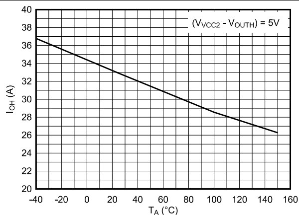
Figure 6-1. I O TH vs. Temperature
