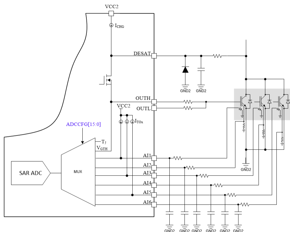
Figure 7-3. Block diagram of implementation of ADC processing for the case where three power transistors are connected in parallel.
