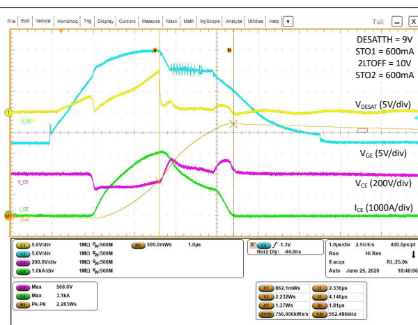
Figure 8-10. Two-Level Turn Off (2LTOFF) Shutdown Response to DESAT Event
