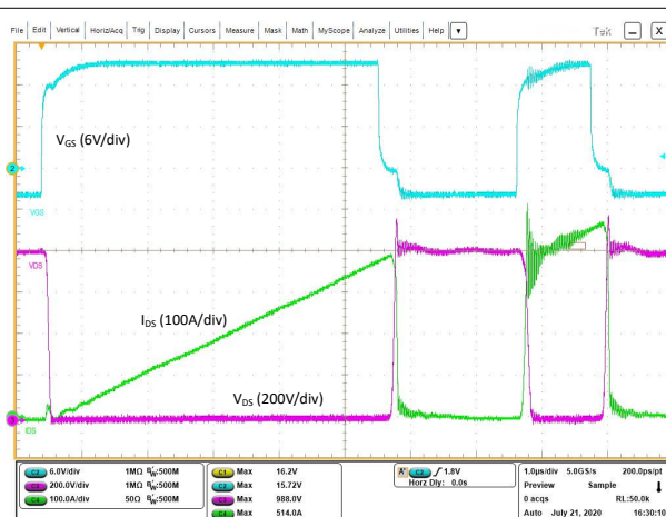
Figure 8-5. SiC Double Pulse Waveform
