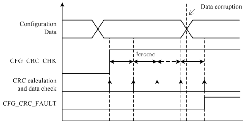
Figure 7-35. Configuration Data CRC Check Timing
