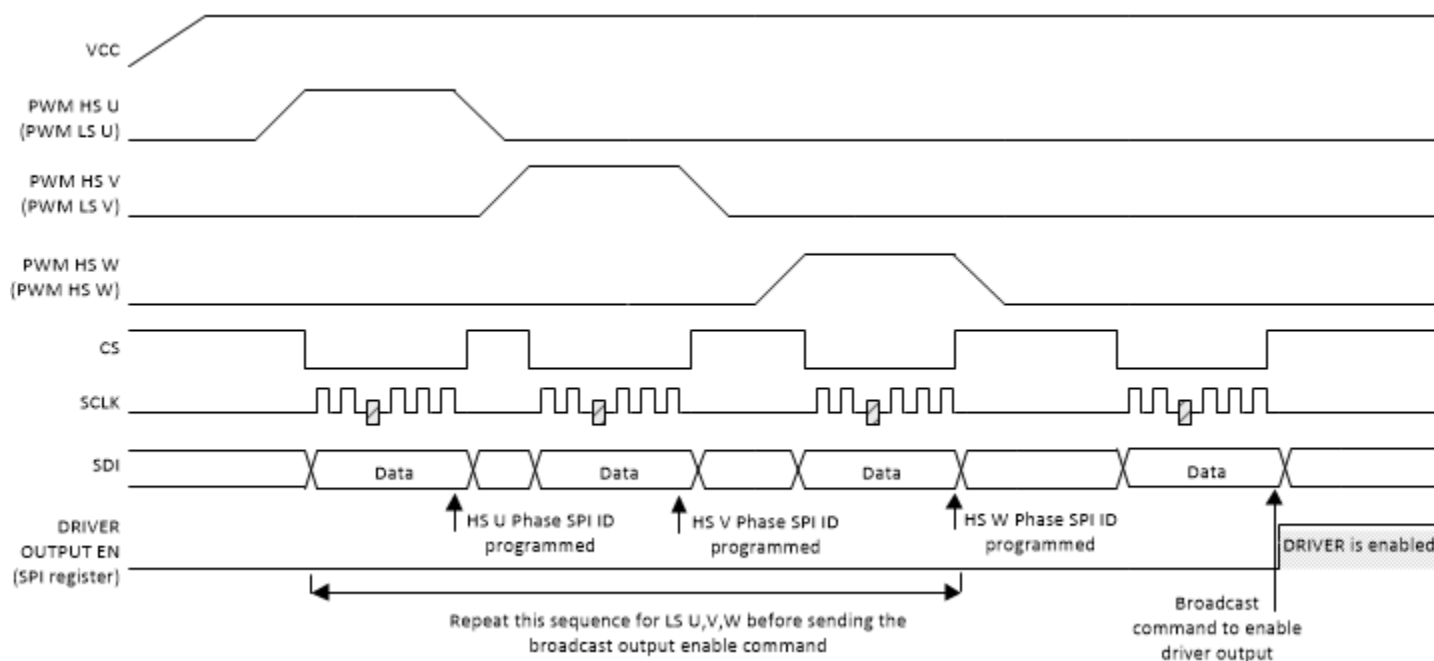
Figure 8-1. Timing diagram for addressing when using the Address-based SPI Communication Scheme.
