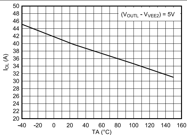
Figure 6-2. I O TL vs. Temperature
