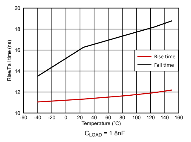
Figure 5-15. Output Rise and Fall Time
