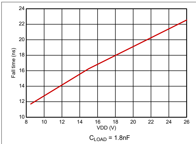
Figure 5-14. Output Fall Time
