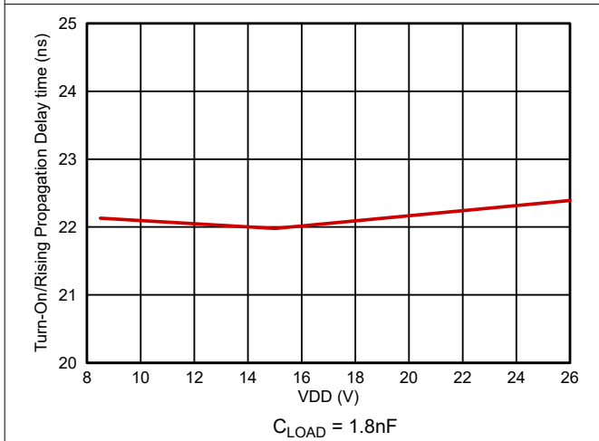
Figure 5-16. Input to Output Rising (Turnon) Propagation Delay
