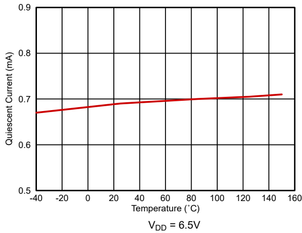
Figure 5-2. Quiescent Current
