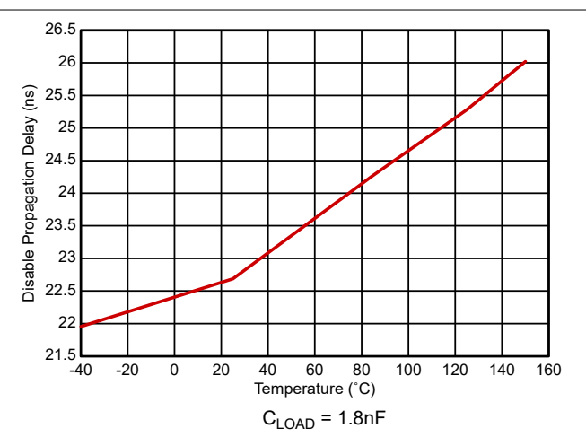
Figure 5-19. Disable Propagation Delay
