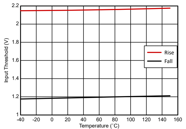
Figure 5-7. Input Threshold
