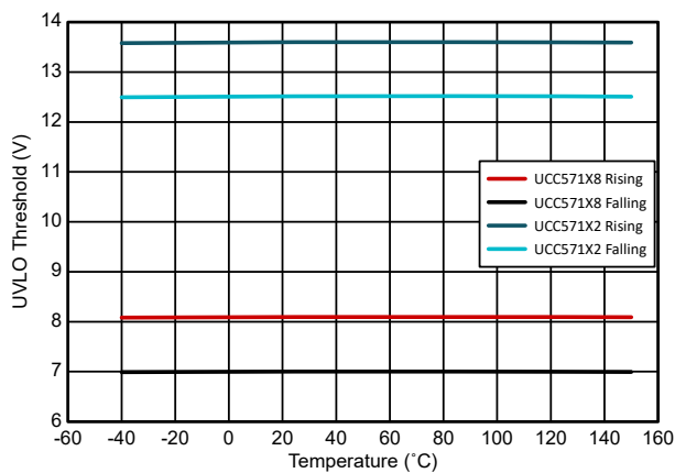
Figure 5-6. UVLO Threshold
