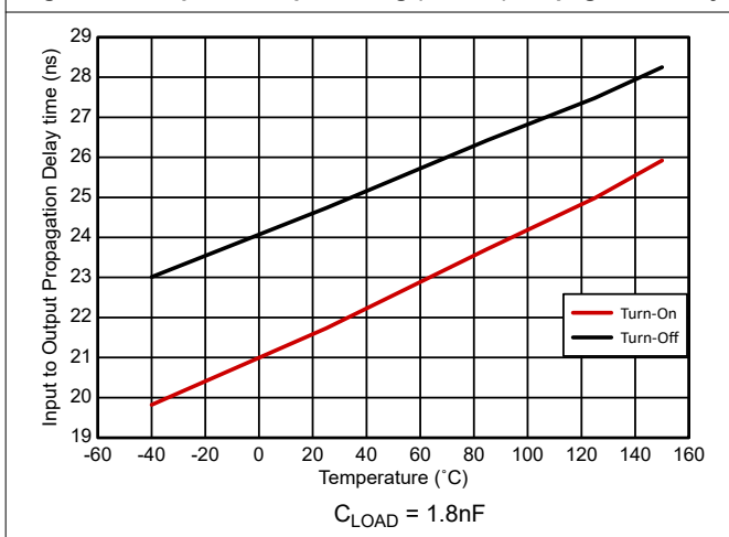
Figure 5-18. Input Propagation Delay
