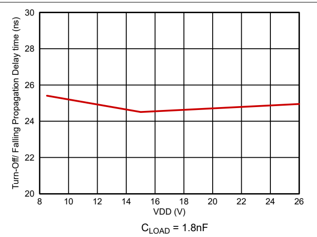
Figure 5-17. Input to Output Falling (Turnoff) Propagation Delay
