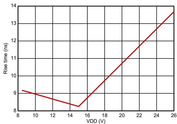
Figure 5-16. Output Rise Time C LOAD = 1.8 nF
