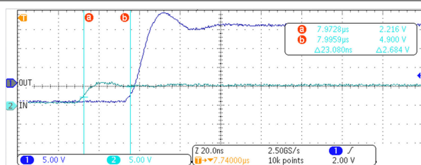
Figure 7-3. UCC57102Z-Q1 Rising (Turn-On) Propagation Delay
