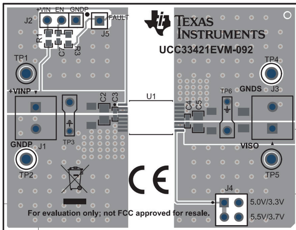
Figure 10-1. Layout Example
