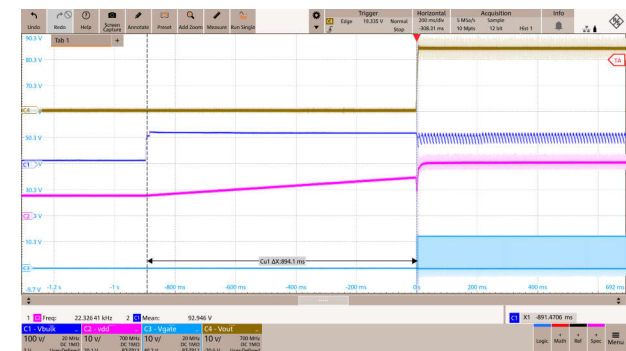
Figure 8-5. Start-Up Waveforms at 85Vac and Full Load
