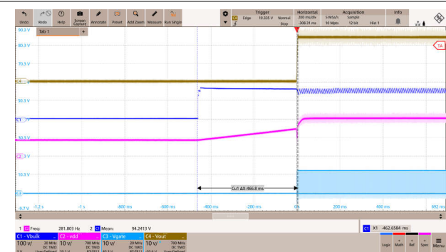
Figure 8-7. Start-Up Waveforms at 115Vac and Full Load
