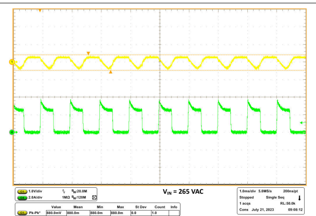
Figure 8-15. Load Transients at 265Vac
