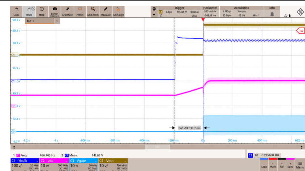
Figure 8-9. Start-Up Waveforms at 230Vac and Full Load
