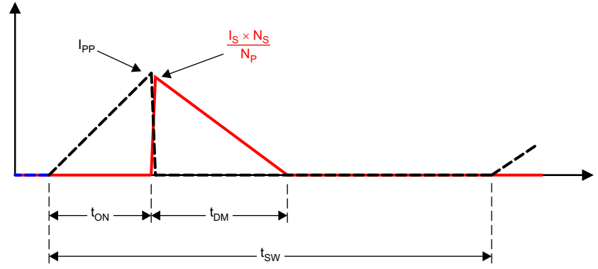
Figure 7-6. Transformer-Current Relationship
