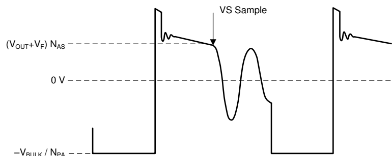
Figure 7-3. Auxiliary-Winding Voltage
