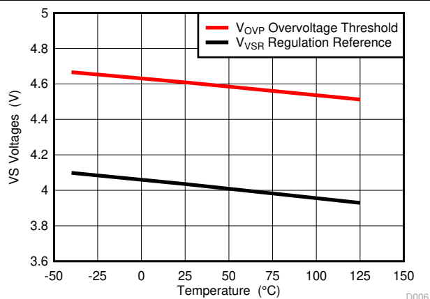
Figure 6-6. VS Voltages vs. Temperature
