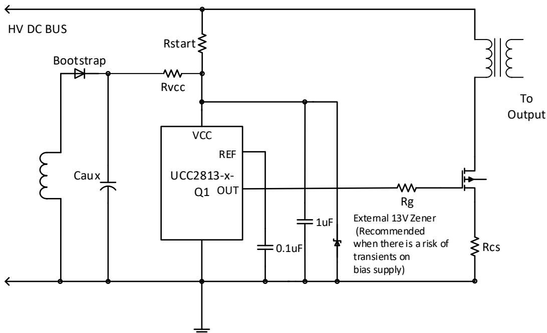
Figure 8-11. Power-Up Recommendation
