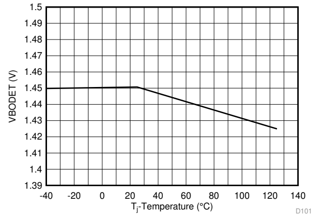
Figure 2. VINAC Brownout Detection Threshold
