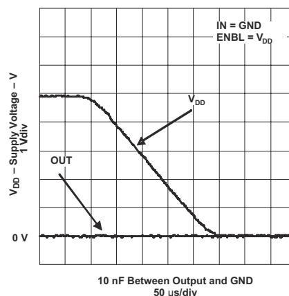
Figure 7-24. Output Behavior vs V_{DD} (Noninverting)
