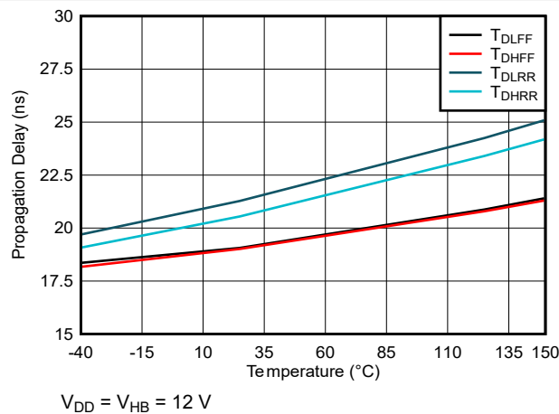
Figure 5-12. Propagation Delays vs Temperature
