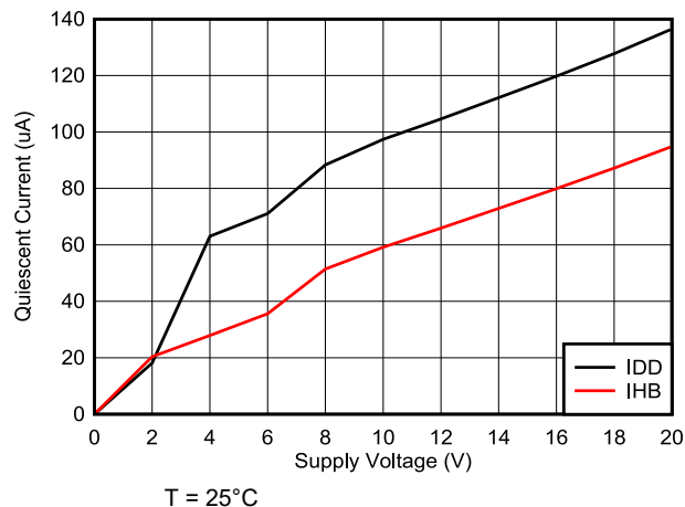
Figure 5-2. Quiescent Current vs Supply Voltage
