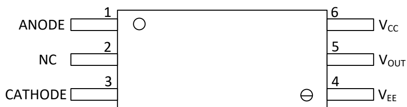
Figure 5-1. UCC23313-Q1 Package SO-6 Top View
