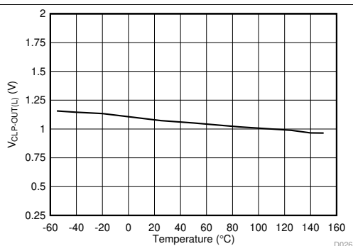
Figure 20. V_{CLP-OUT(L)} Short Circuit Clamping Voltage vs. Temperature
