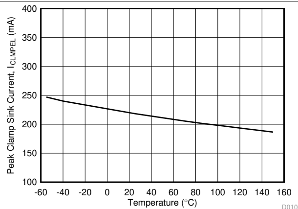
Figure 22. I_{CLMPEL} Miller Clamp Sink Current vs. Temperature
