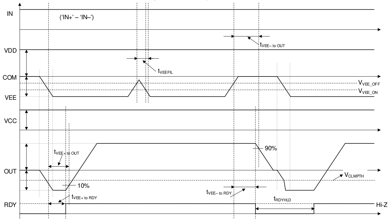
Figure 34. VEE UVLO Protection Timing Diagram
