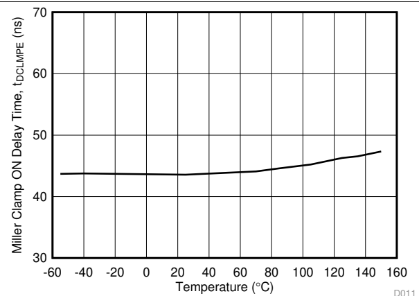
Figure 23. t_{DCLMPE} Miller Clamp ON Delay Time vs. Temperature
