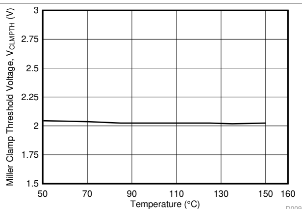
Figure 21. V_{CLMPH} Miller Clamp Threshold Voltage vs. Temperature
