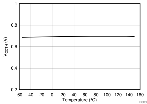
Figure 24. V_{OCTH} OC Detection Threshold vs. Temperature
