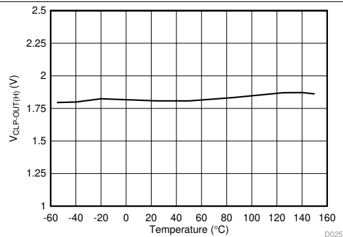
Figure 19. V_{CLP-OUT(H)} Short Circuit Clamping Voltage vs. Temperature
