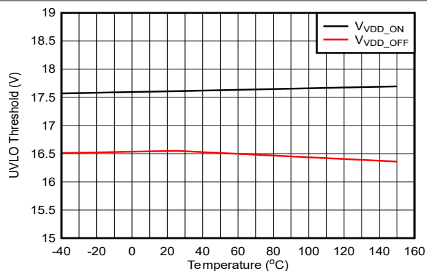
Figure 5-25. VDD 17-V UVLO Threshold vs Temperature
