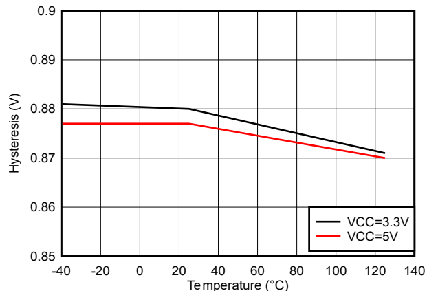
Figure 5-27. IN/EN Hysteresis vs Temperature
