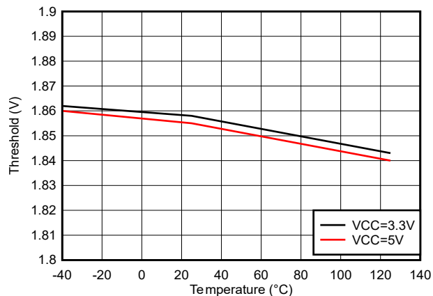
Figure 5-29. IN/EN High Threshold
