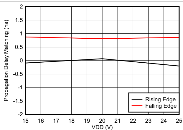
Figure 5-17. Propagation Delay Matching ( t_{\text{DM}} ) vs VDD
