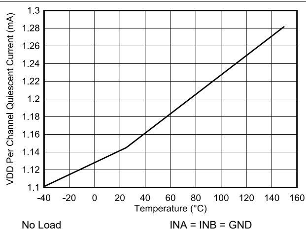
Figure 6-7. VDD Per Channel Quiescent Current ( I_{VDDA} , I_{VDDB} )
