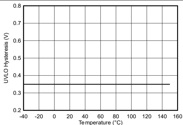
Figure 6-11. 5-V VDD UVLO Hysteresis Voltage
