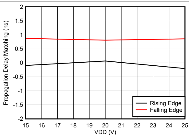
Figure 5-15. Propagation Delay Matching ( t_{\text{DM}} ) vs VDD
