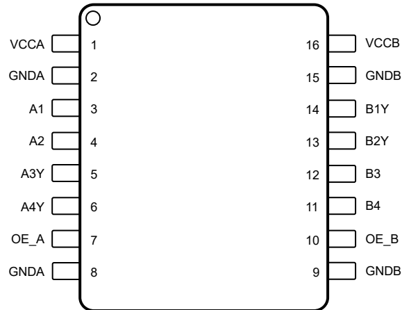
Figure 4-6. TXG4042 DBQ 16-Pin QSOP Top View
