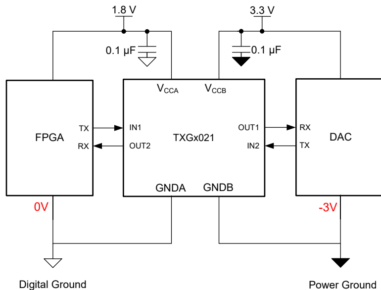
Figure 8-1. TXG4021 in Test and Measurement
