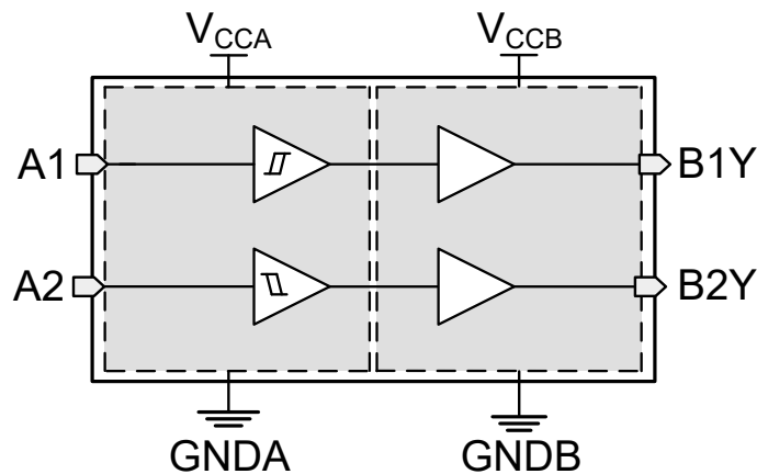
Figure 7-2. TXG4020 Functional Block Diagram
