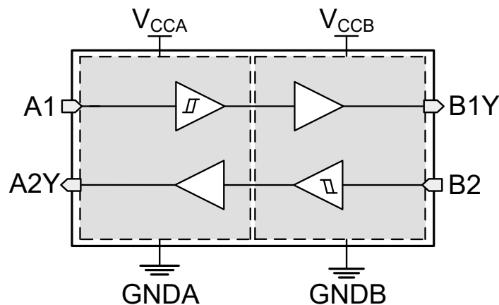
Figure 7-1. TXG4021 Functional Block Diagram
