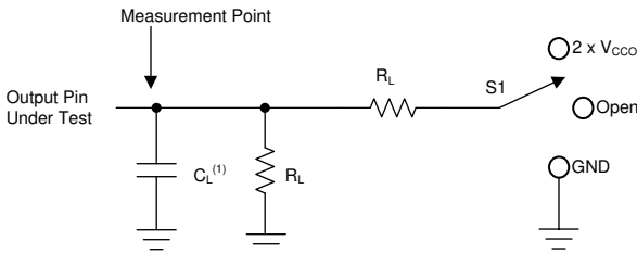
Figure 6-1. Load Circuit
