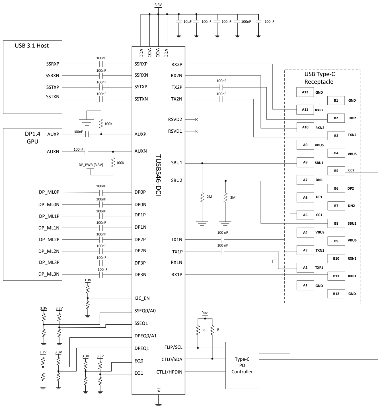
Figure 8-2. Application Circuit
