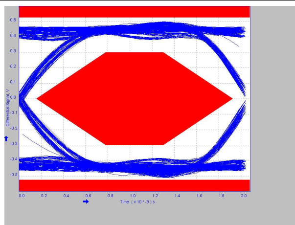
Figure 8-13. 6 Inches Post-Channel With TUSB216-Q1 BOOST=0 RX_SEN=HIGH
