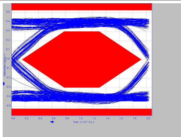
Figure 8-7. 3 Meter Pre-Channel With TUSB216-Q1 BOOST=0 RX_SEN=HIGH
