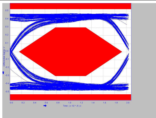
Figure 8-12. 6 Inches Post Channel Without TUSB216-Q1
