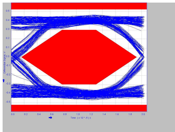
Figure 8-9. 5 Meter Pre-Channel With TUSB216-Q1 BOOST=1 RX_SEN=MED
