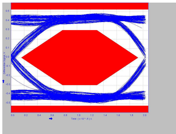
Figure 8-5. 2 Meter Pre-Channel With TUSB216-Q1 BOOST=0 RX_SEN=HIGH
