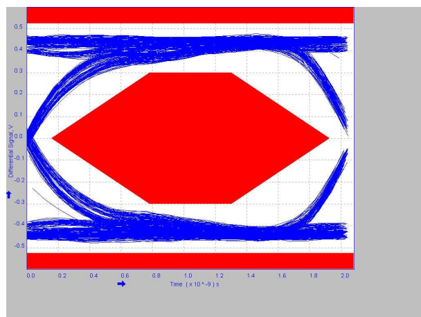
Figure 8-14. 1 Meter Post-Channel Without TUSB216-Q1
