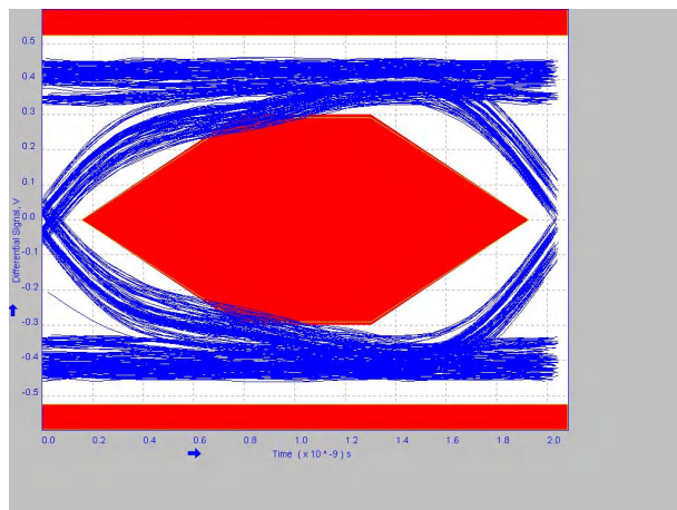
Figure 8-20. 4 Meter Post-Channel Without TUSB216-Q1
