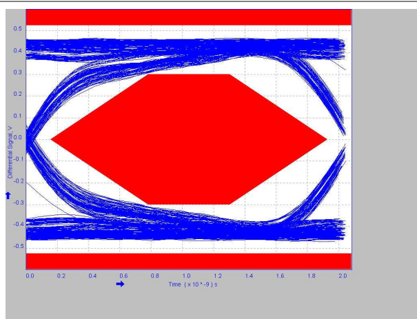
Figure 8-3. 2 Meter Pre-Channel Without TUSB216-Q1
