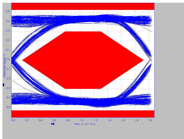
Figure 8-18. 2 Meter Post-Channel With TUSB216-Q1 BOOST=1 RX_SEN=MED
