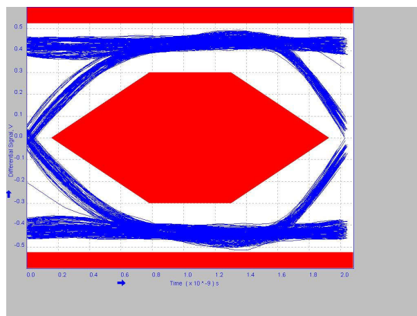
Figure 8-15. 1 Meter Post-Channel With TUSB216-Q1 BOOST=0 RX_SEN=MED
