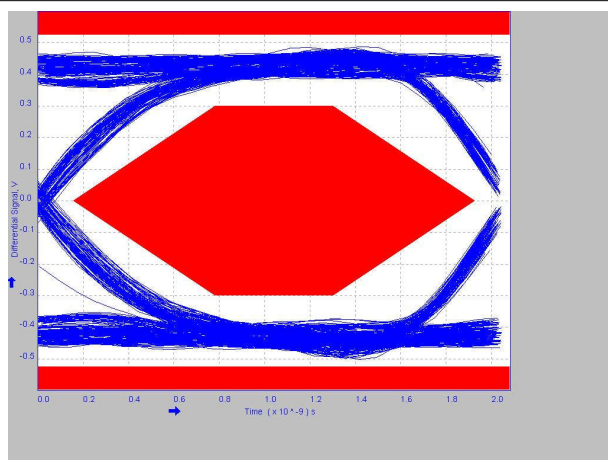
Figure 8-16. 1 Meter Post-Channel With TUSB216-Q1 BOOST=0 RX_SEN=HIGH
