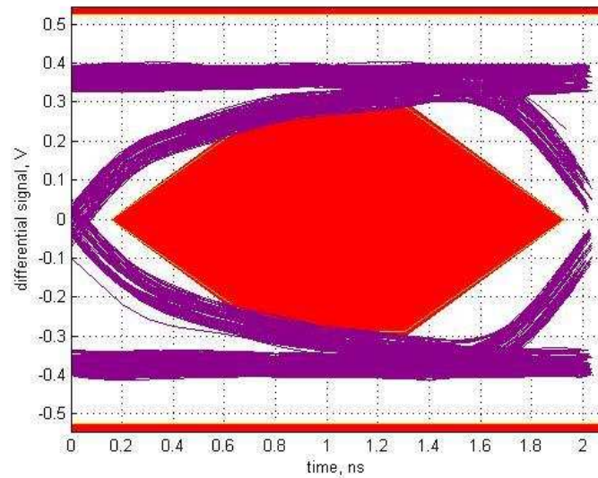
Figure 9. No TUSB213
