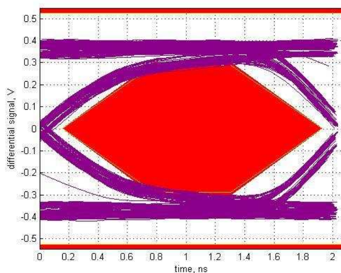
Figure 9. No TUSB212
