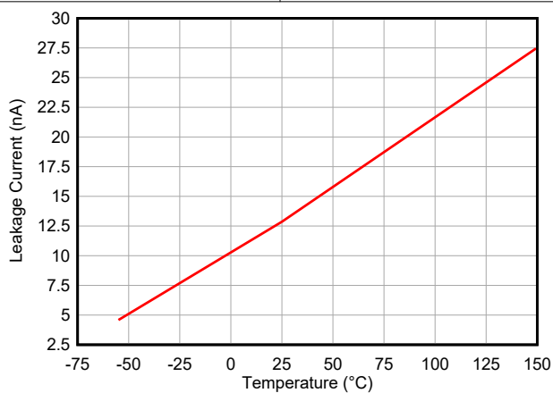
Figure 5-3. Leakage vs Temperature
