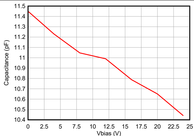
Figure 5-2. Capacitance vs Bias Voltage
