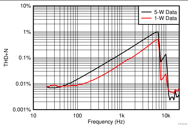
Figure 5-4. THD+N vs Frequency
