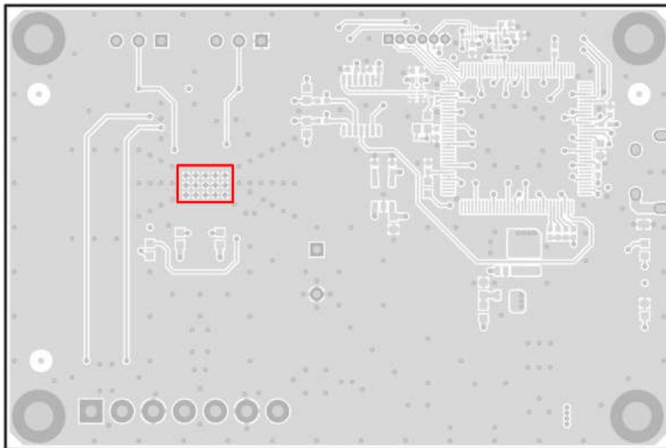
Figure 8-5. Bottom Layer
