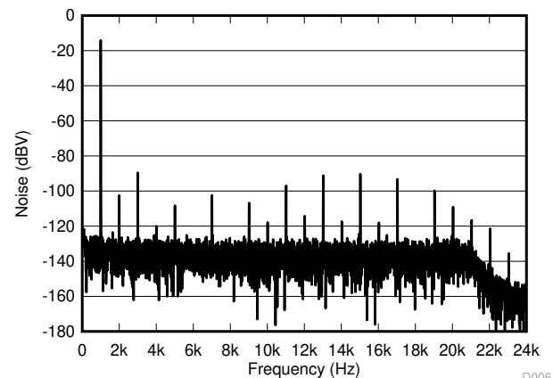
Figure 5-6. Noise FFT With 1-W Output
