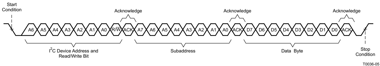
Figure 6-5. Random Write Transfer
