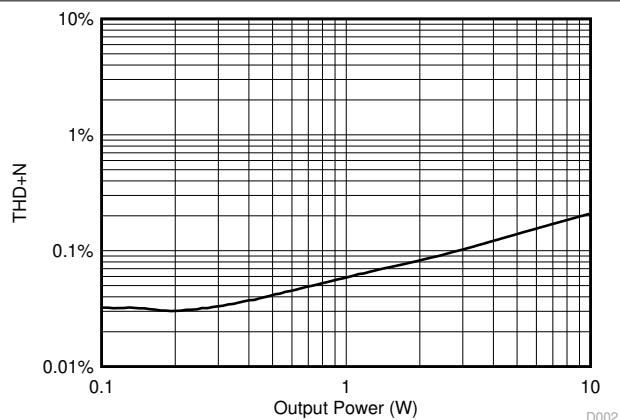
Figure 5-2. THD+N vs Output Power
