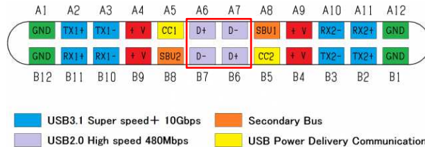
Figure 13. USB Type-C Connector Pinout
