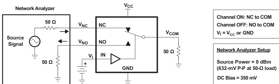
Figure 24. Crosstalk ( X_{TALK} )
