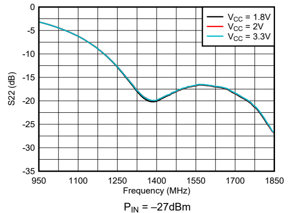
Figure 5-34. Output Return Loss ( S_{22} ) Across V_{CC}
