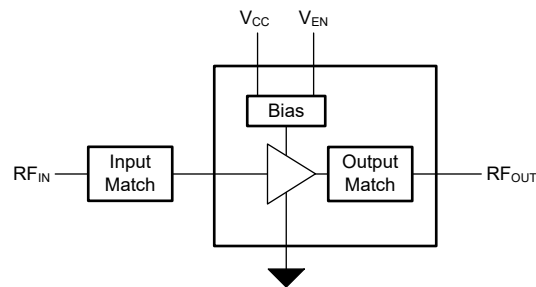
Figure 6-1. TRF3302-Q1 Functional Block Diagram
