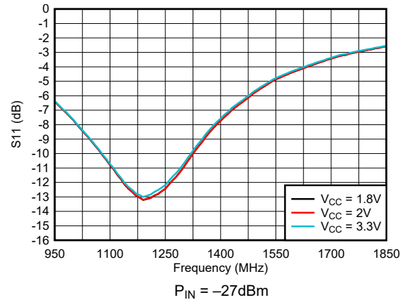
Figure 5-32. Input Return Loss ( S_{11} ) Across V_{CC}
