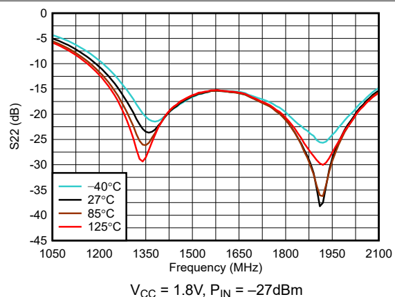
Figure 5-10. Output Return Loss (S22) Across Temperature
