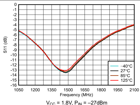
Figure 5-8. Input Return Loss (S11) Across Temperature
