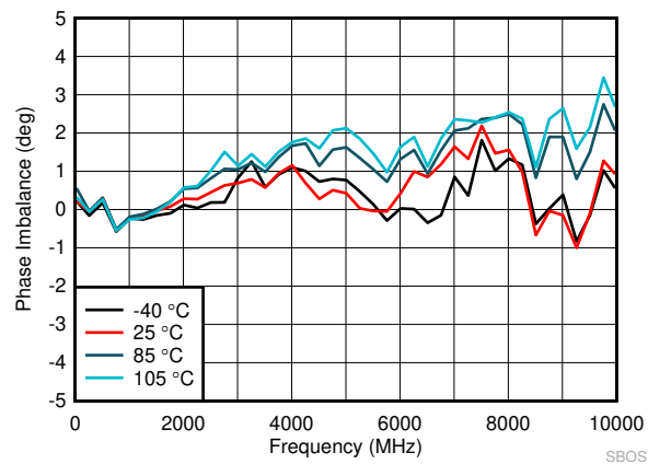
Figure 6-32. Phase Imbalance
