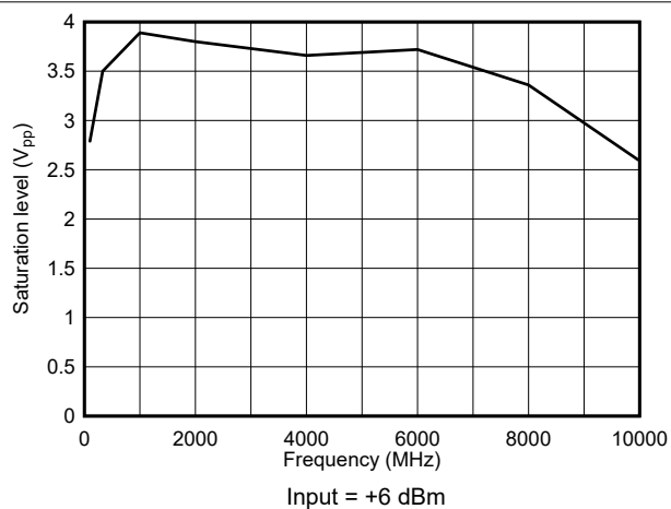
Figure 6-36. Saturation Voltage
