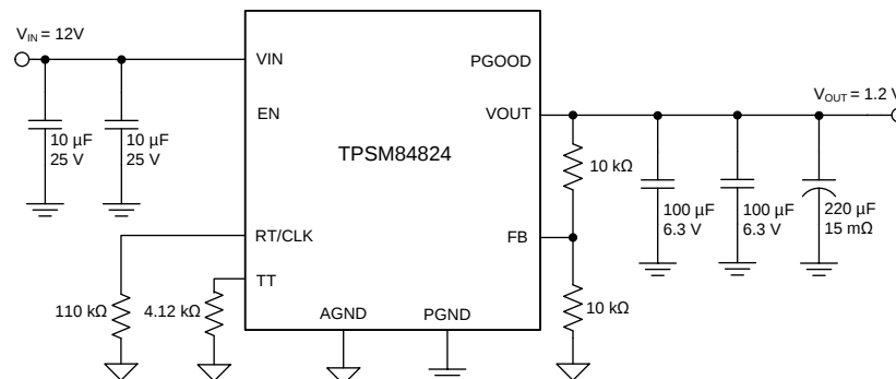
Figure 24. TPSM84824 Typical Application
