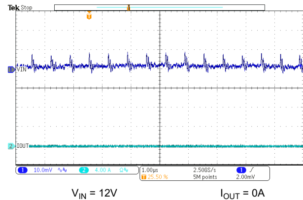
Figure 7-17. Input Ripple – No Load
