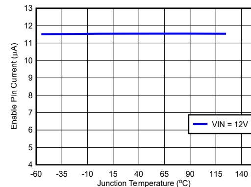
Figure 5-6. Enable Pin Current
