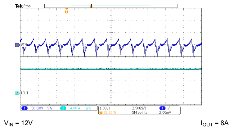
Figure 7-18. Input Ripple – 8A Load
