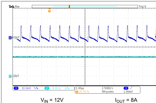
Figure 7-16. Output Ripple – 8A Load
