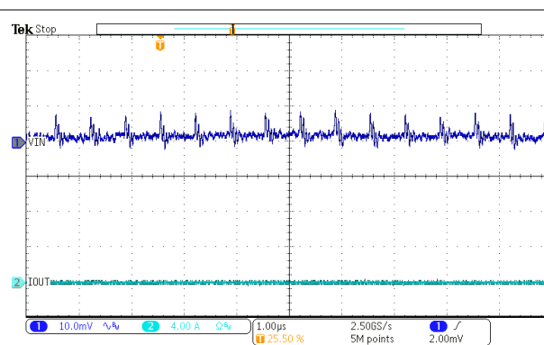
Figure 7-17. Input Ripple – No Load
