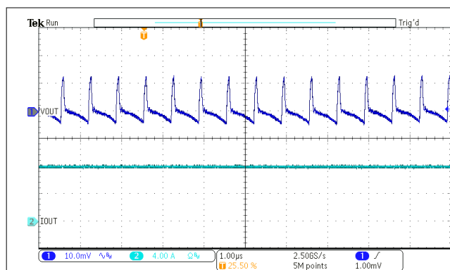
Figure 7-16. Output Ripple – 8A Load
