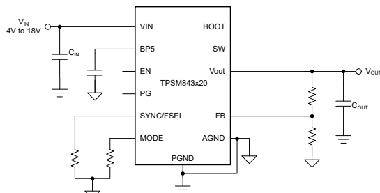
Simplified Schematic
