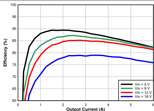
Figure 7-4. Efficiency
