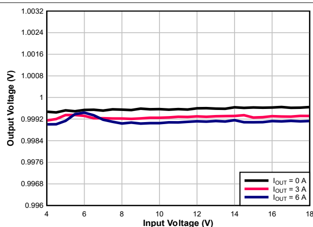
Figure 7-6. Line Regulation
