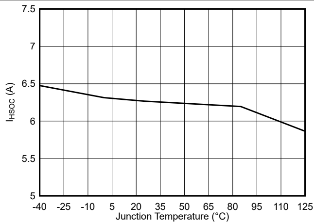
Figure 5-9. TPSM84338 High-Side Current Limit vs Junction Temperature
