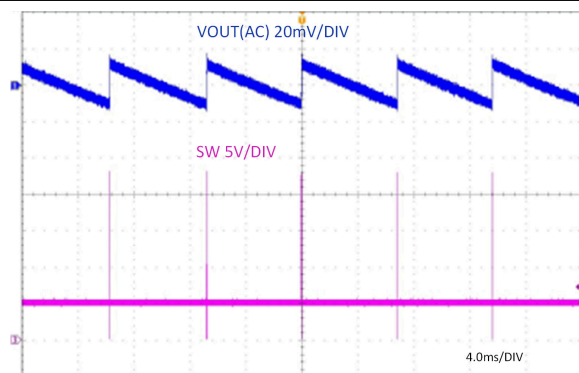
Figure 7-12. Steady State, I_{OUT} = 0A
