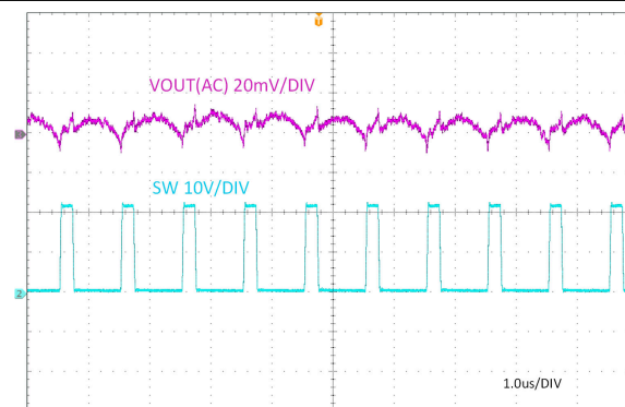
Figure 7-13. Steady State, I_{OUT} = 3A
