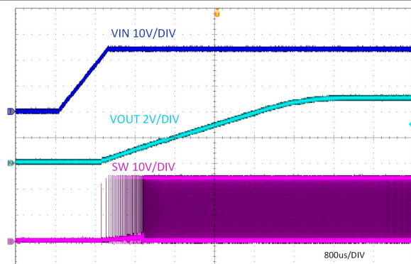
Figure 7-10. Start-Up Relative to V_{IN} , I_{OUT} = 3A
