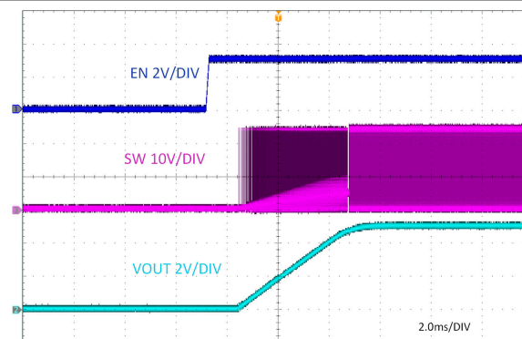
Figure 7-11. Start-Up Through EN, I_{OUT} = 3A
