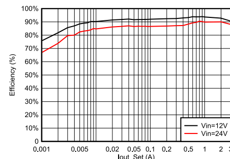
TPSM84338 Efficiency, V_{\text{OUT}} = 5\text{V} , f_{\text{SW}} = 1000\text{kHz}
