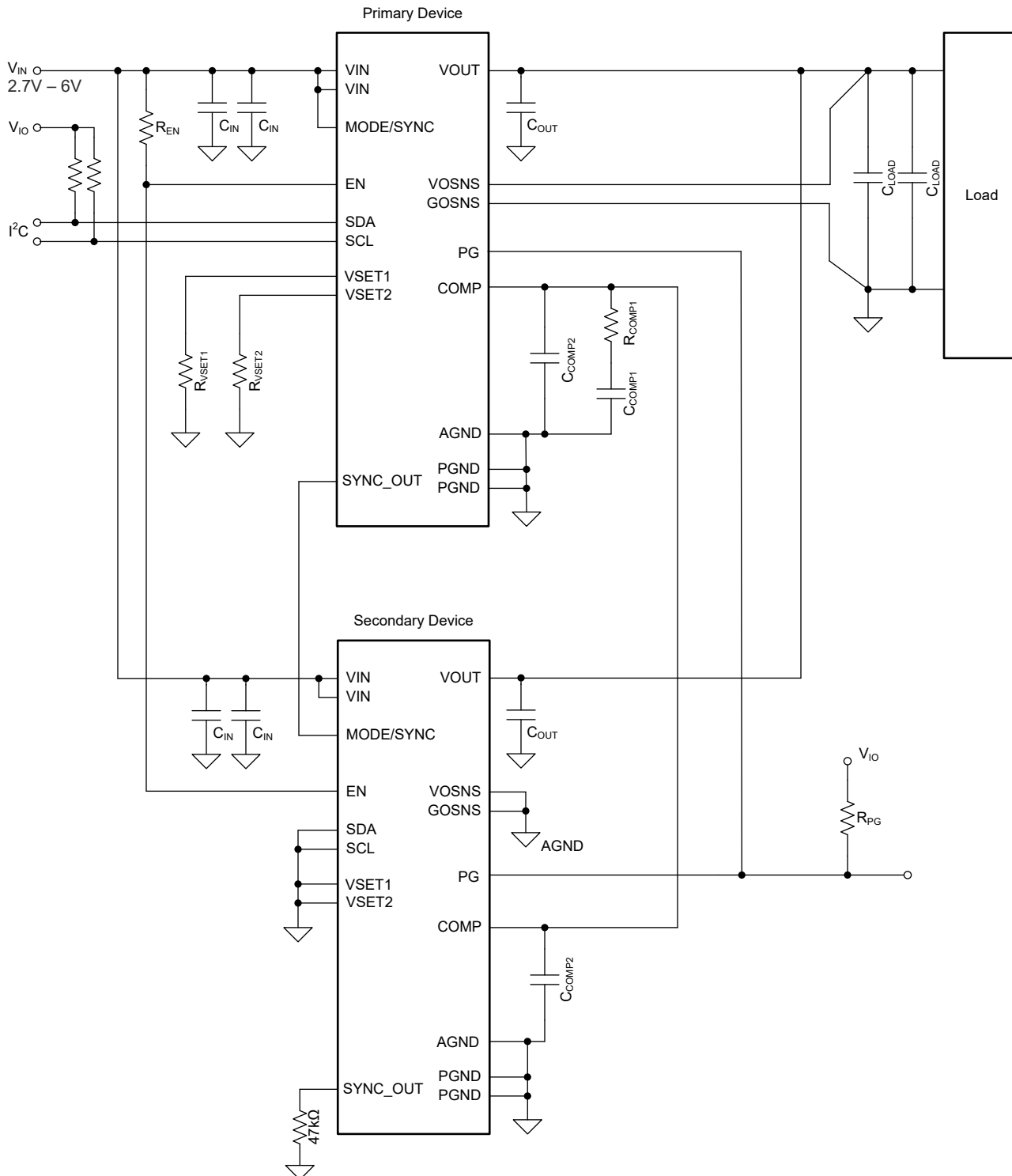
Figure 7-17. Two TPSM8287Bxx Devices in a Stacked Configuration
