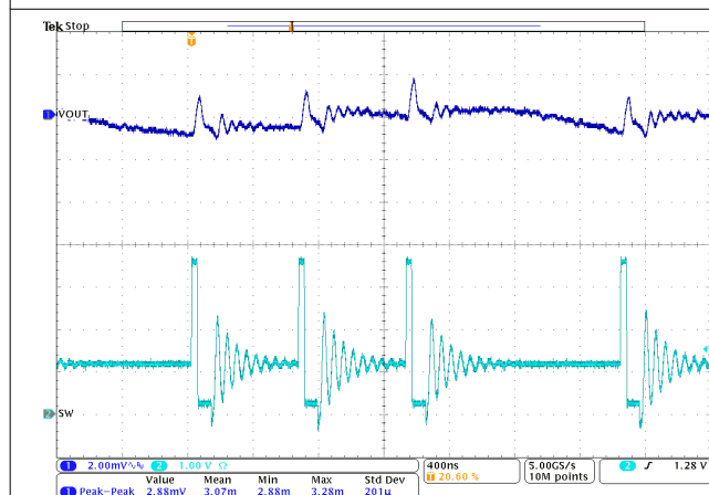
Figure 9-22. PWM-CCM Operation TPSM8287B30xx
