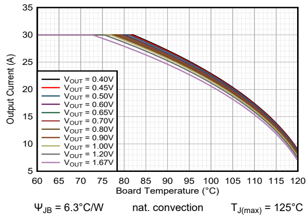
Figure 9-34. Safe Operating Area TPSM8287B30xx V_{IN} = 3.3\text{V}
