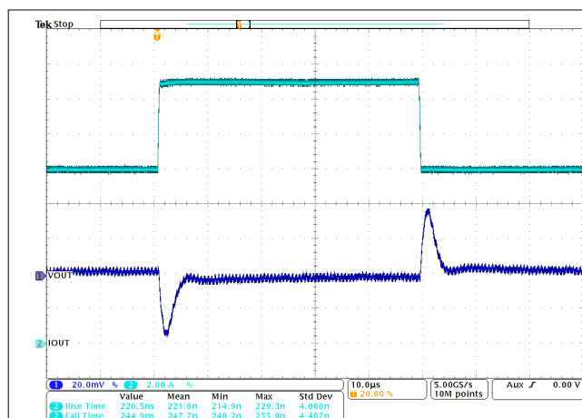
Figure 9-20. Load Transient TPSM8287B30xx
