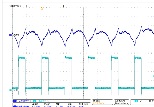
Figure 9-20. Load Transient TPSM8287B30xx
