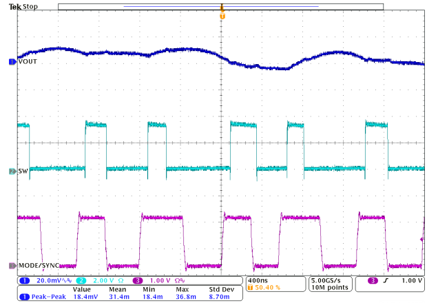
Figure 9-27. Synchronization to a Random External Clock
