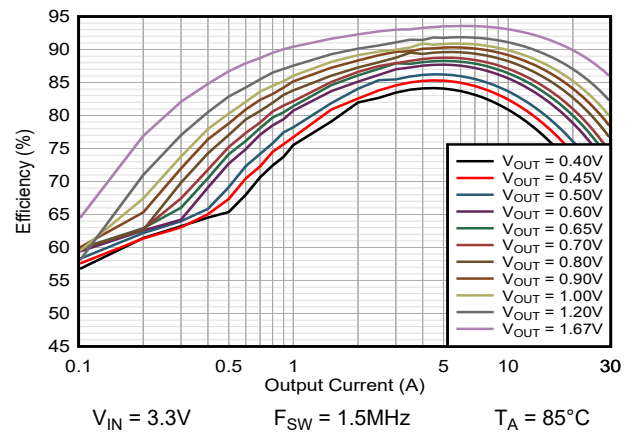
Figure 9-11. Efficiency TPSM8287B30xx PSM
