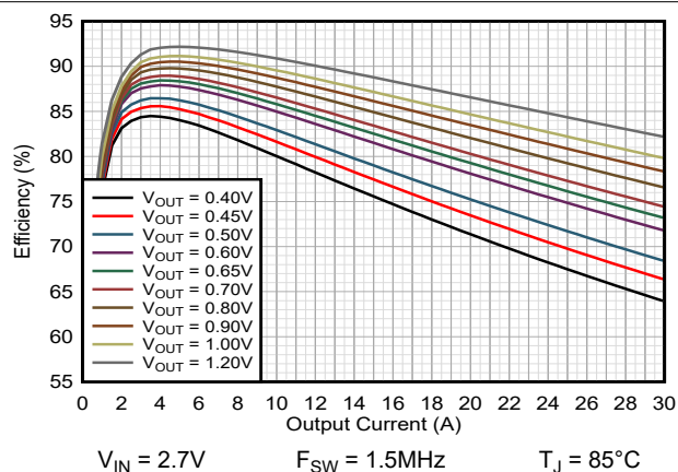
Figure 9-3. Efficiency TPSM8287B30xx FPWM
