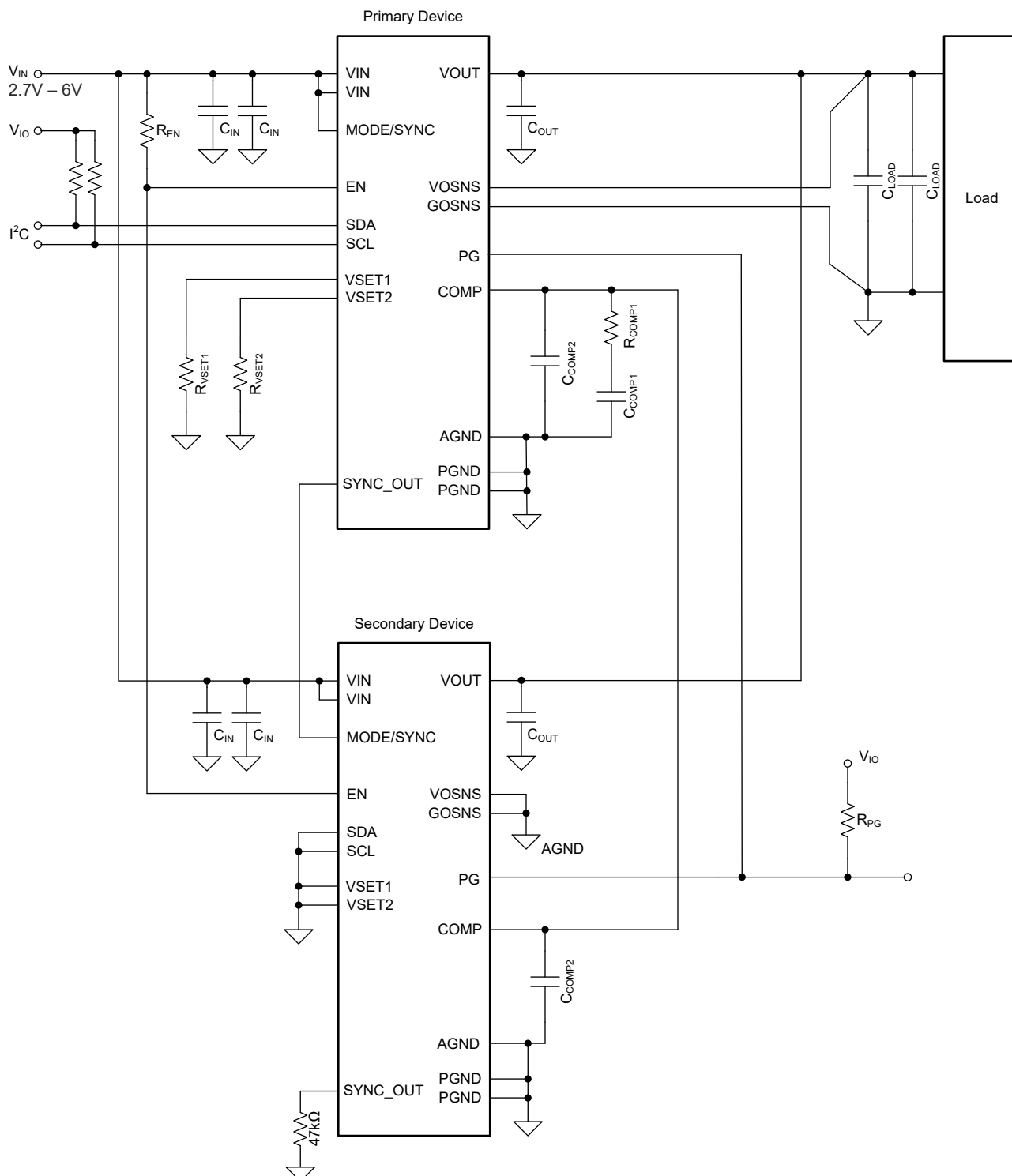
Figure 9-36. Typical Application Schematic
