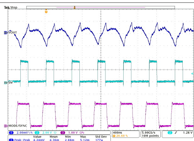
Figure 9-23. PWM-DCM Operation TPSM8287B30xx
