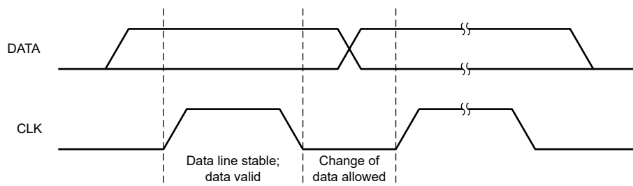
Figure 7-19. Bit Transfer on the Serial Interface
