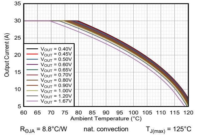
Figure 9-33. Safe Operating Area TPSM8287B30xx V_{IN} = 5.0\text{V}
