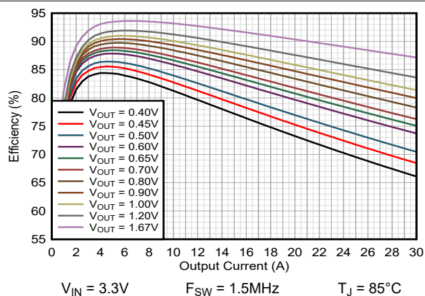
Figure 9-5. Efficiency TPSM8287B30xx FPWM
