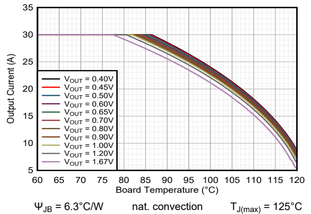
Figure 9-35. Safe Operating Area TPSM8287B30xx V_{IN} = 5.0\text{V}
