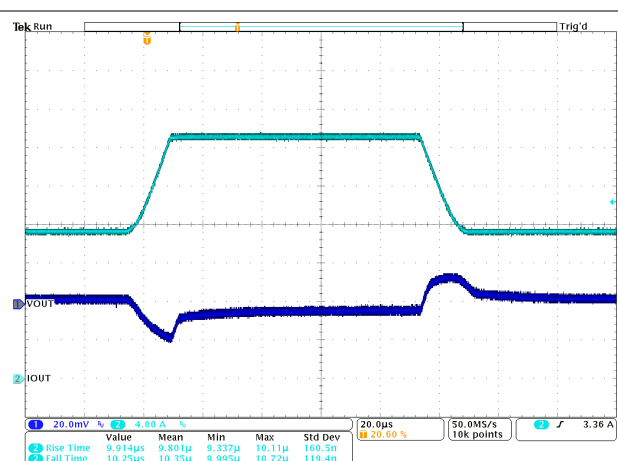
Figure 9-21. Load Transient TPSM8287B30xx
