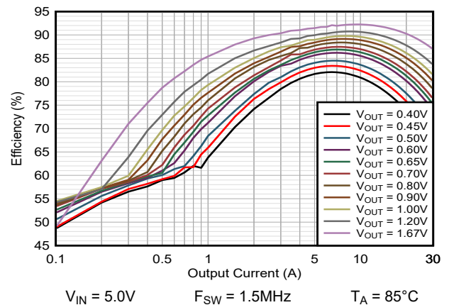
Figure 9-13. Efficiency TPSM8287B30xx PSM
