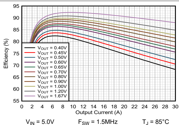
Figure 9-7. Efficiency TPSM8287B30xx FPWM
