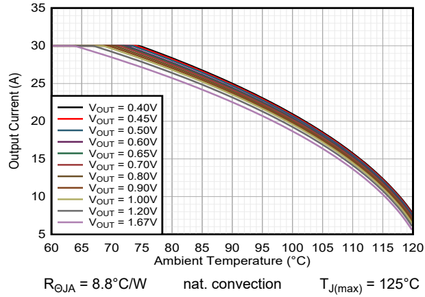
Figure 9-32. Safe Operating Area TPSM8287B30xx V_{IN} = 3.3\text{V}
