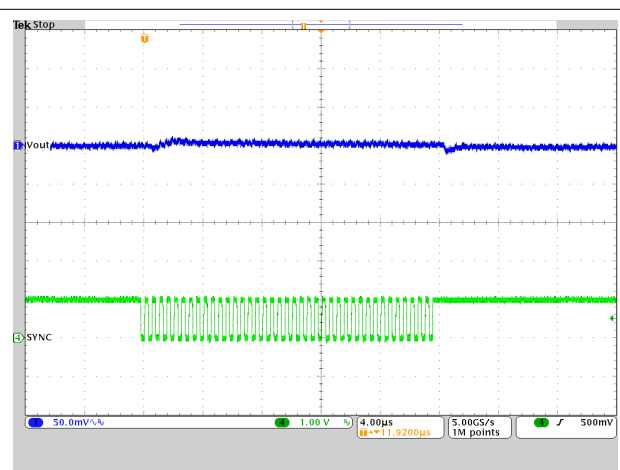
Figure 8-35. Frequency Synchronization
