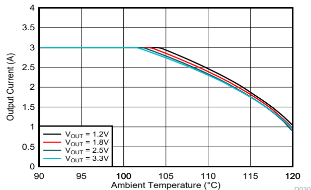
Figure 9-26. Safe Operating Area V_{IN} = 5.0V
