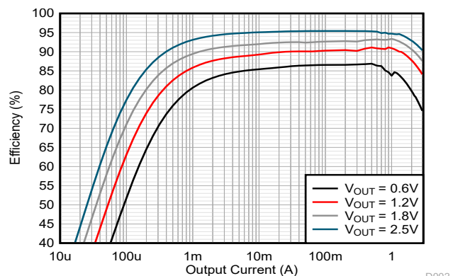
TPSM82813PVCAR Efficiency; V_{IN} = 3.3V
